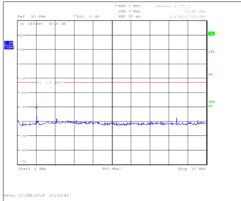
Figure 7.3.2-14: 952.5 MHz – 1GHz to 10GHz
