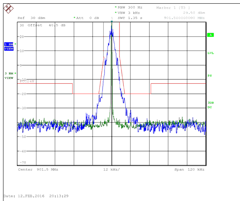
Figure 7.2.2-4: 901.5 MHz – 12.5 kHz Channel Spacing – C&amp;I Mode
