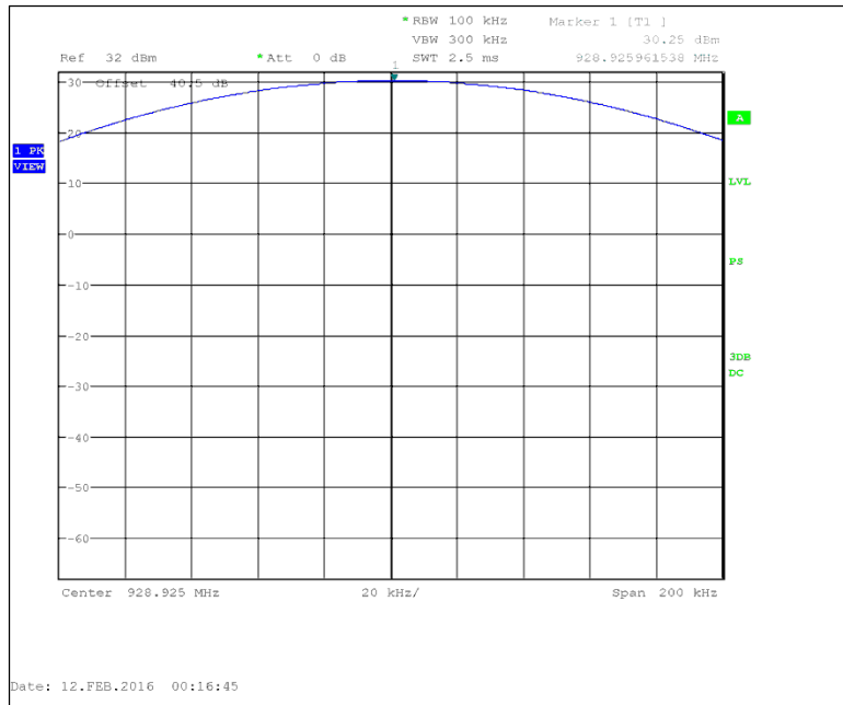
Figure 7.1.2-4: 928.925 MHz
