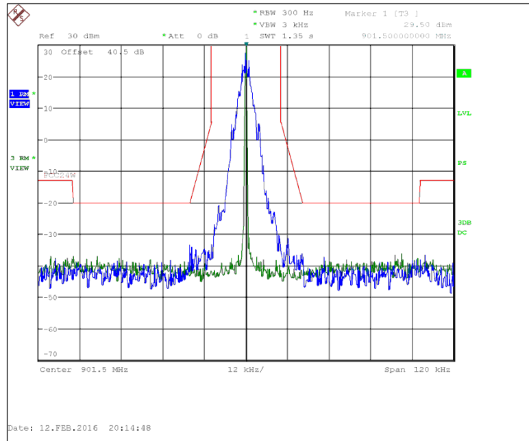
Figure 7.2.2-5: 901.5 MHz – 25 kHz Channel Spacing – C&amp;I Mode
