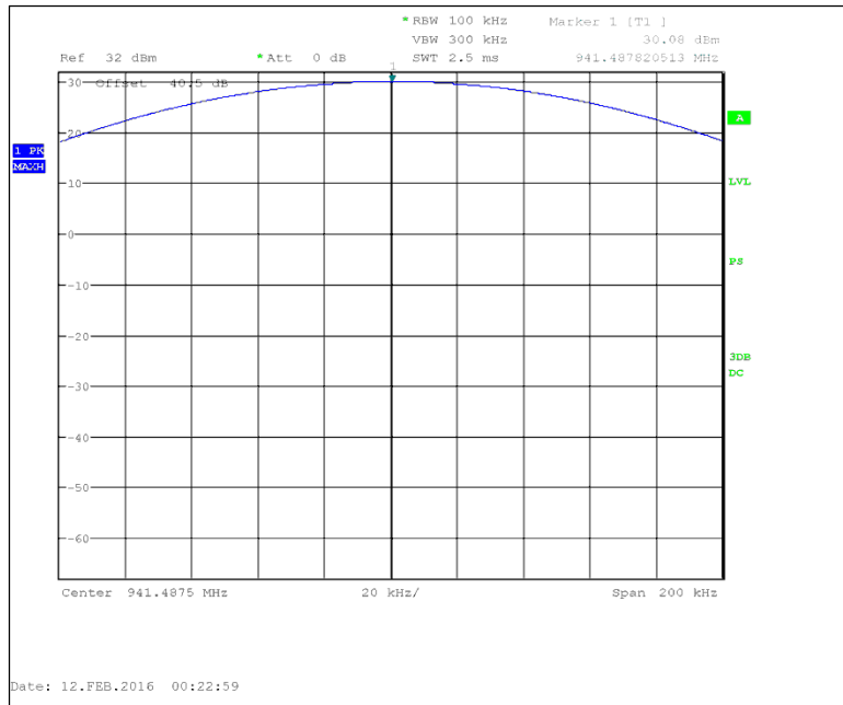
Figure 7.1.2-6: 941.4875 MHz
