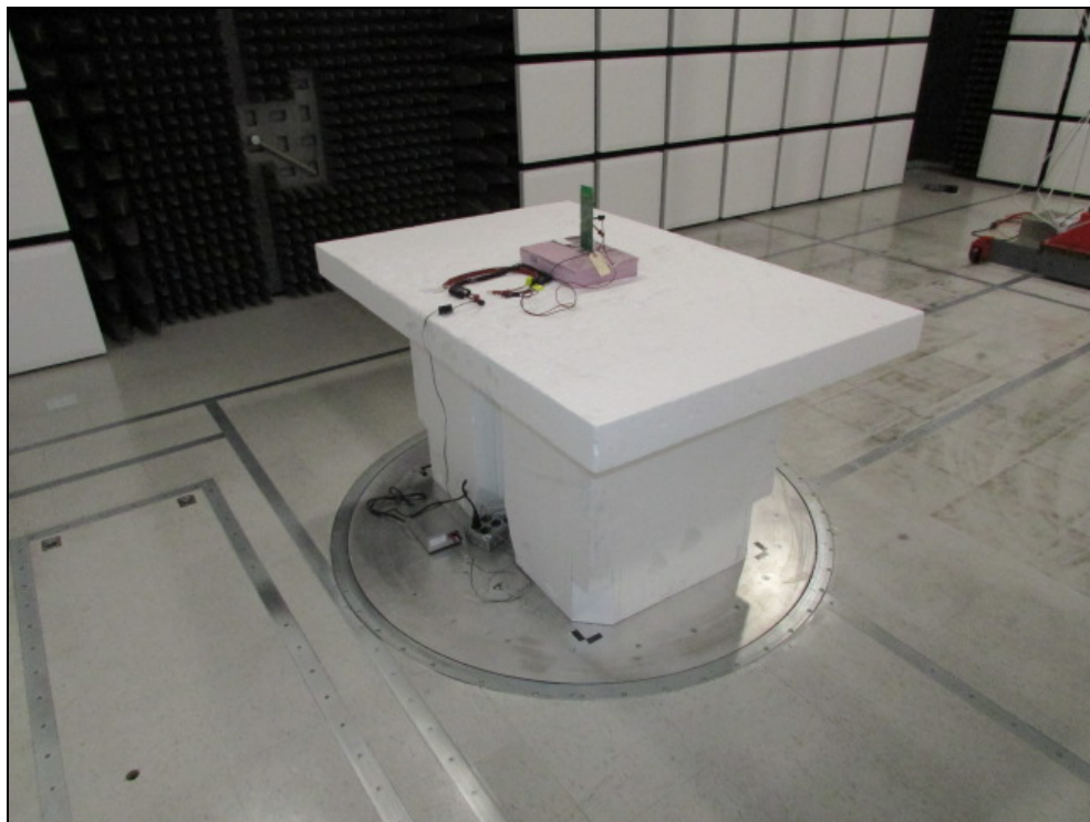
Figure 2: Rear View – Below 1 GHz
