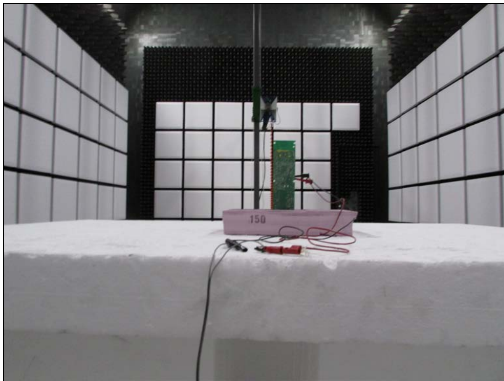
Figure 3: Rear View – Above 1 GHz
