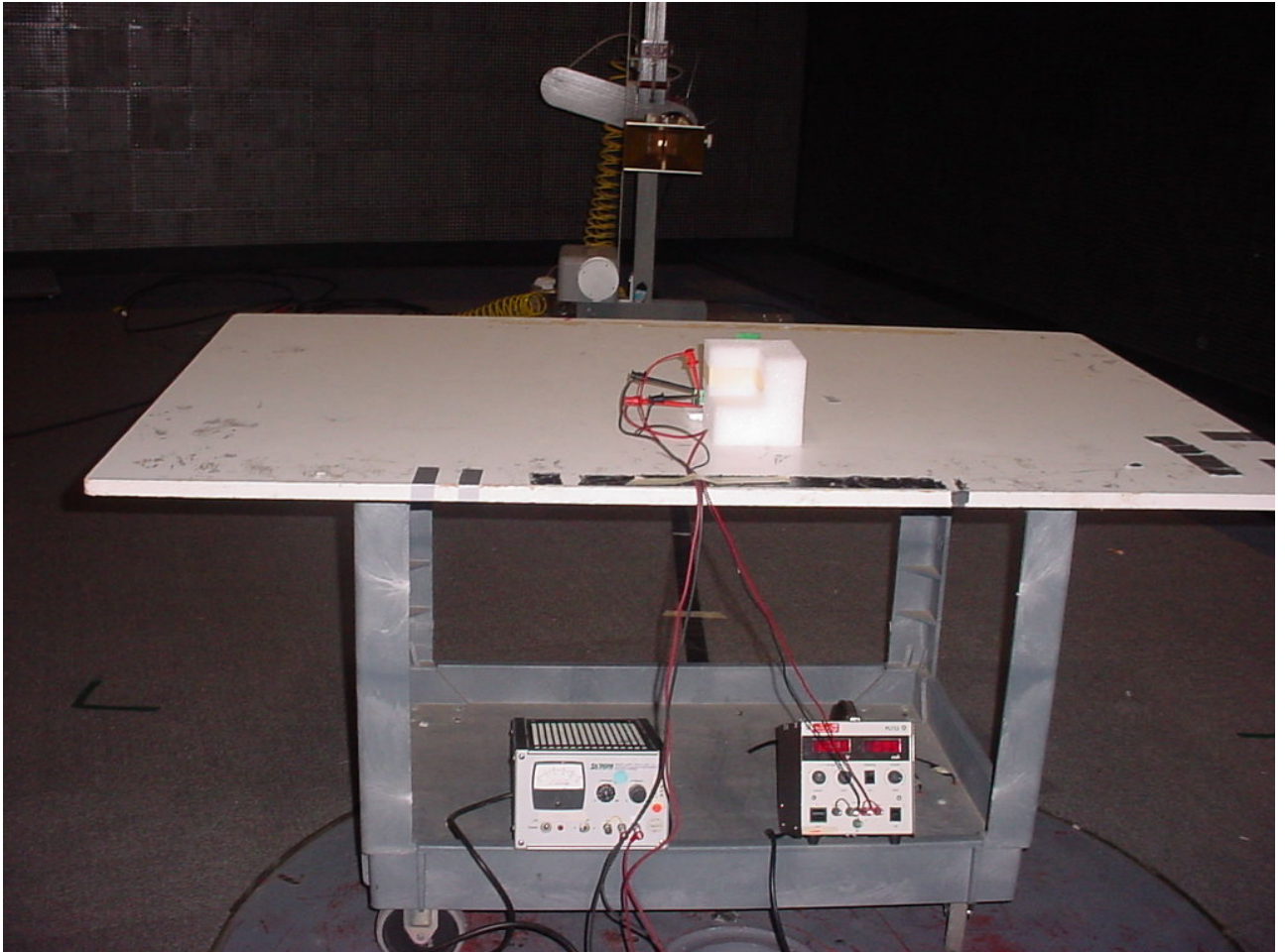
Figure 1: Radiated – Intentional
