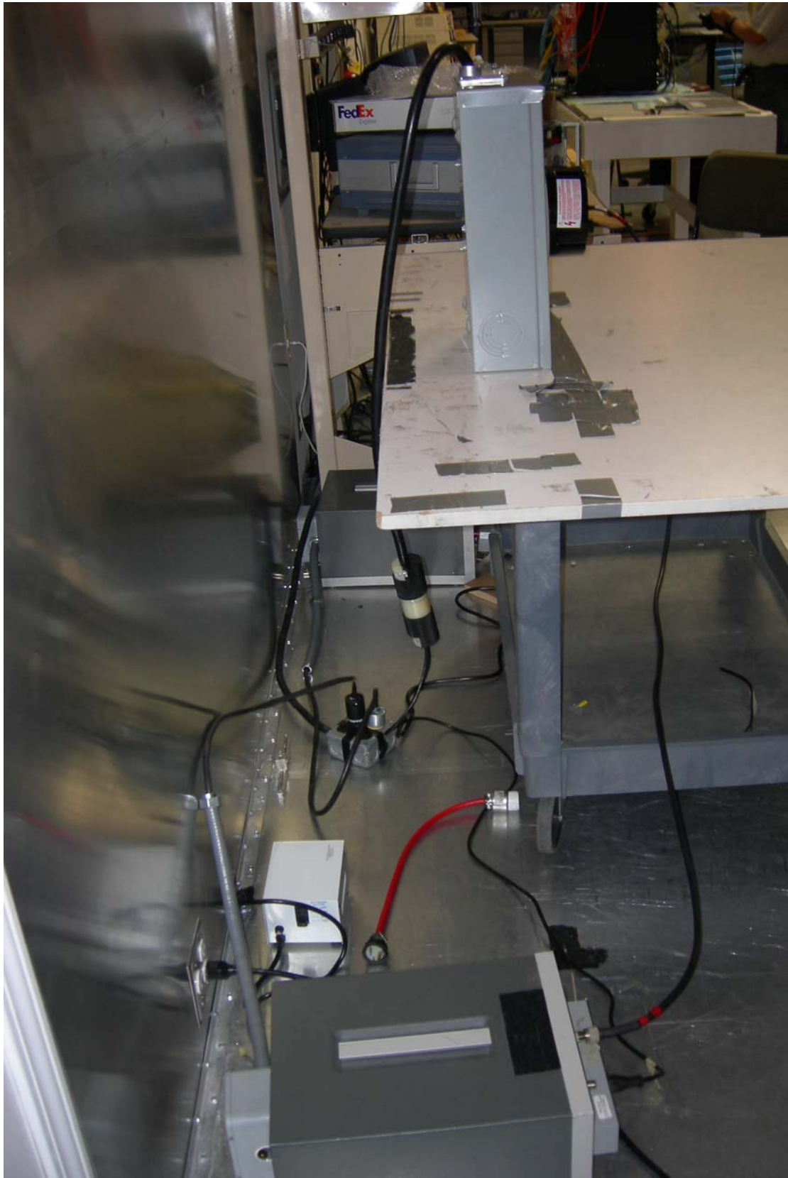
Figure 7: Conducted Emissions
