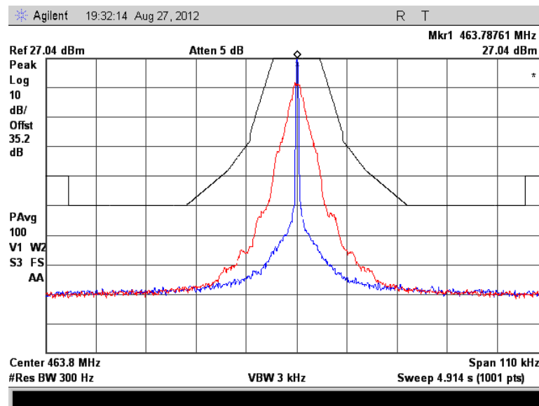
Figure 7.2.2-21: 463.7875 MHz – Priority Mode
