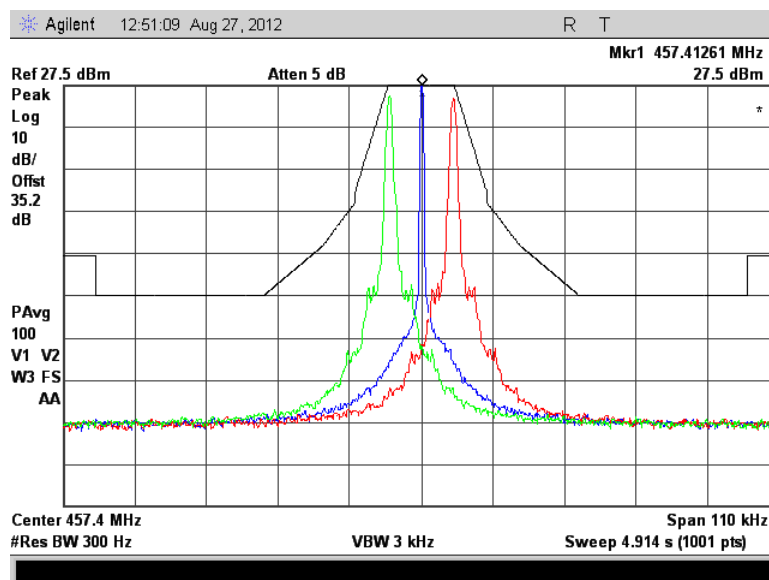
Figure 7.2.2-8: 457.4125 MHz – Boost Mode Offset Channel +/- 8 (+/- 4800)
