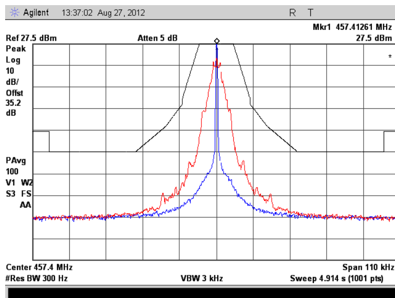
Figure 7.2.2-9: 457.4125 MHz – C&I Mode
