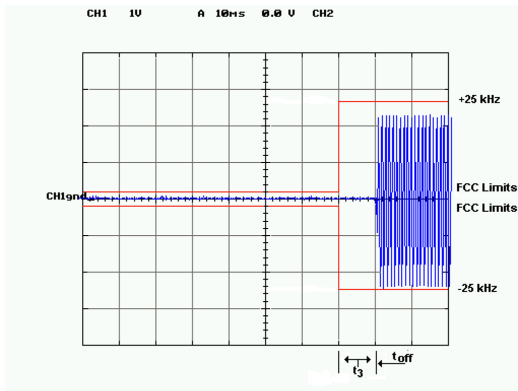
Figure 7.6.2-2: Transient Frequency Behavior – Transmitter Off
