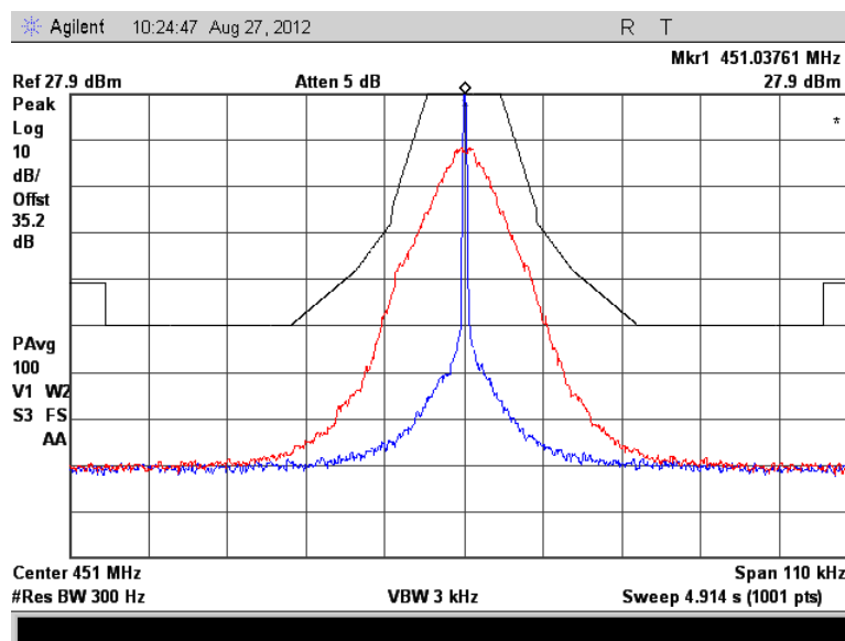
Figure 7.2.2-3: 451.0375 MHz – Double Density Mode
