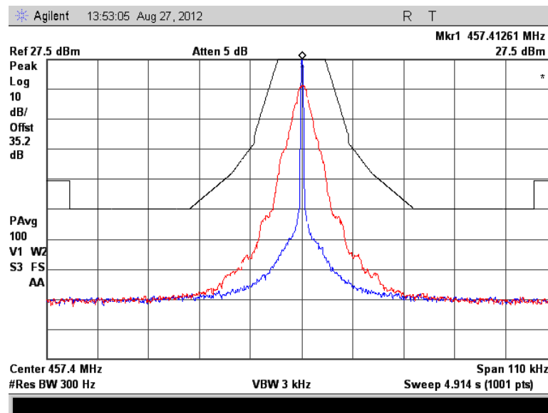
Figure 7.2.2-14: 457.4125 MHz – Priority Mode
