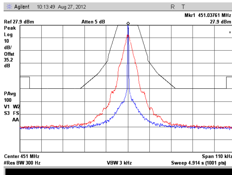
Figure 7.2.2-7: 451.0375 MHz – Priority Mode
