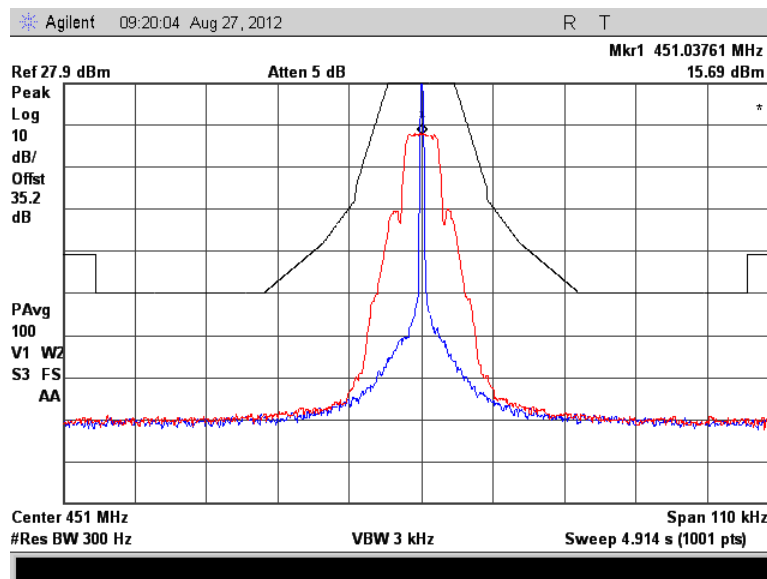
Figure 7.2.2-4: 451.0375 MHz – mPass 5k Mode
