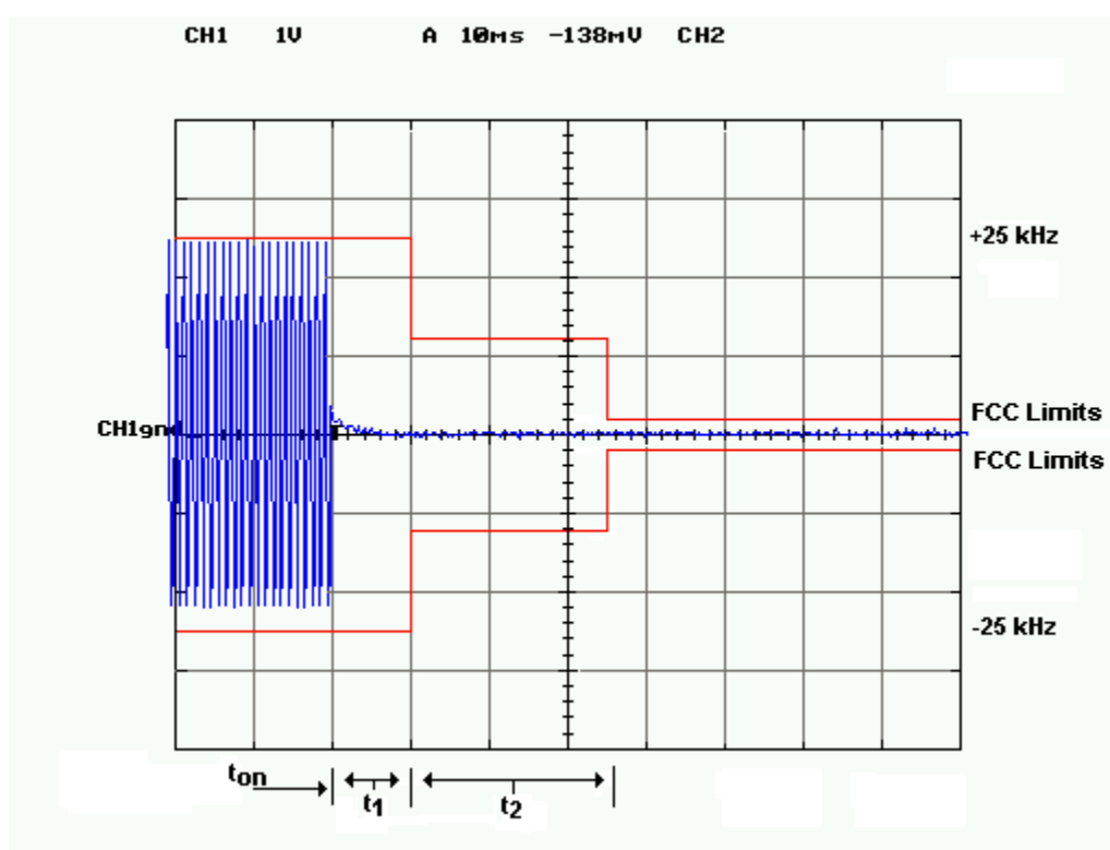
Figure 7.6.2-1: Transient Frequency Behavior – Transmitter On
