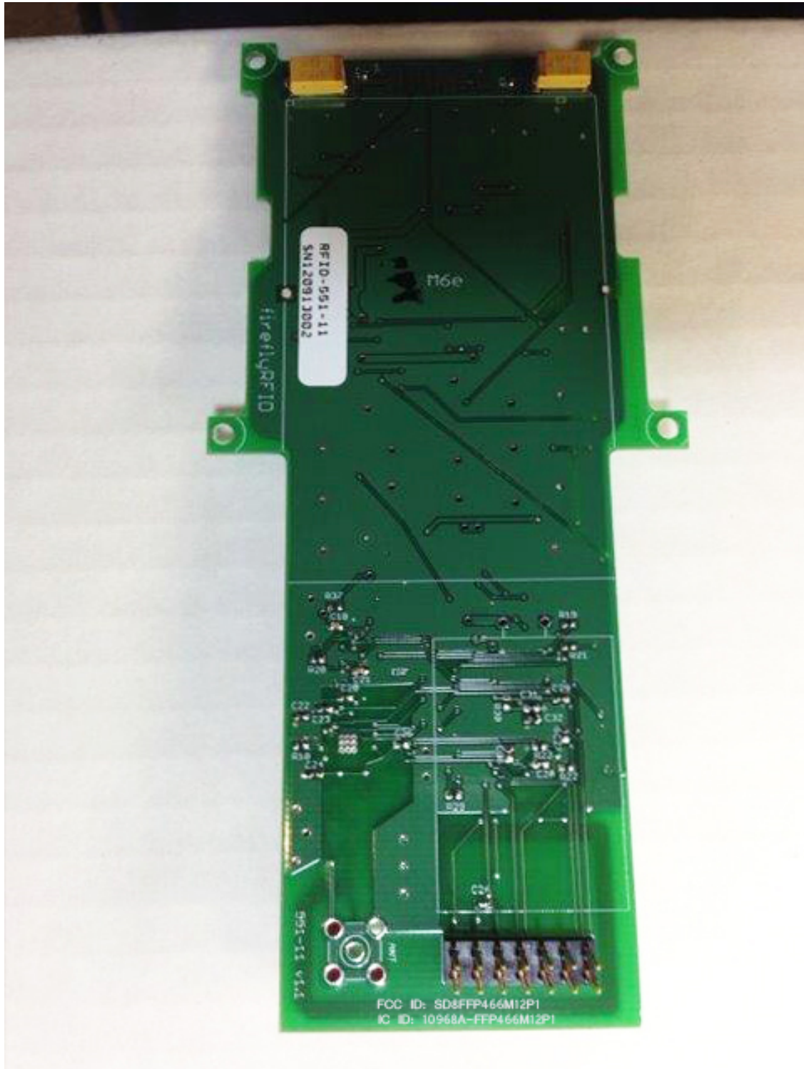
Figure 3: View of EUT without the M6e Module attached
