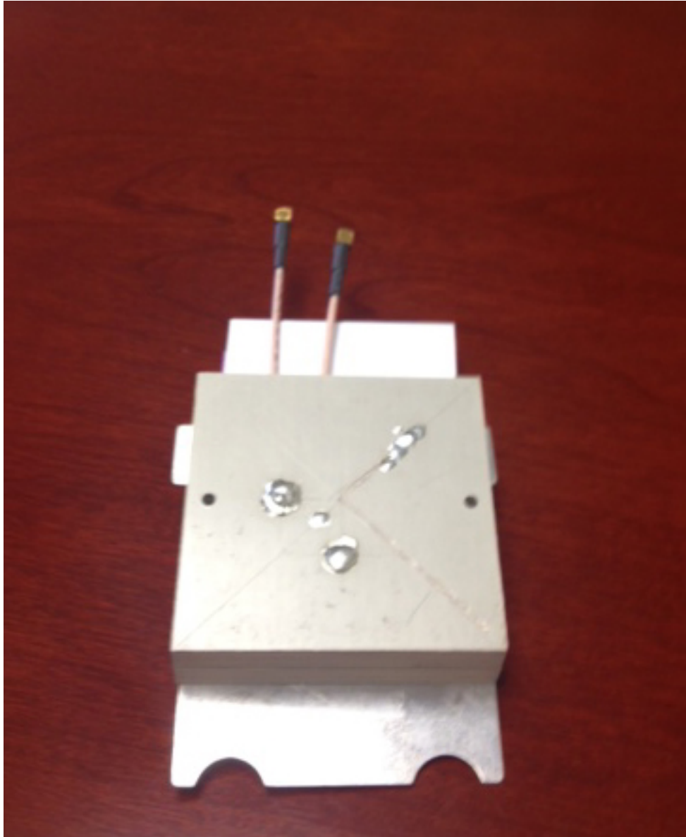
Figure 5: View of antenna package
