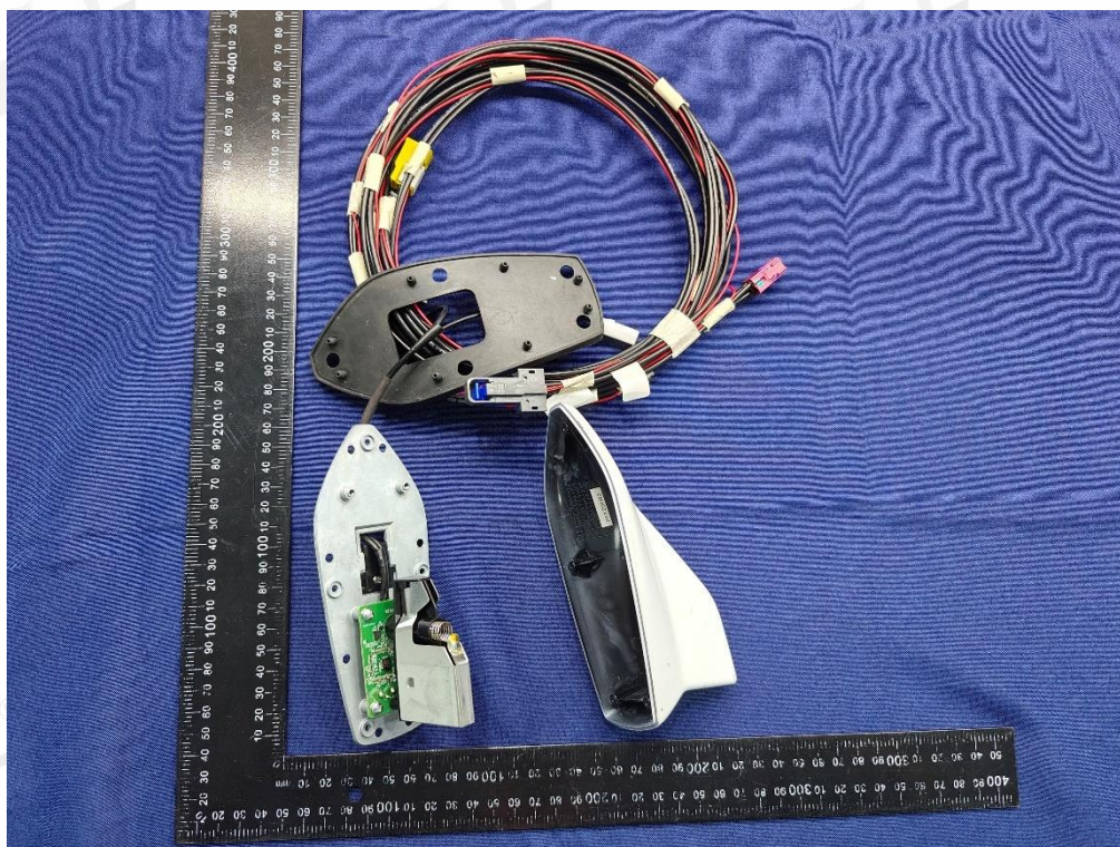
AM/FM antenna
