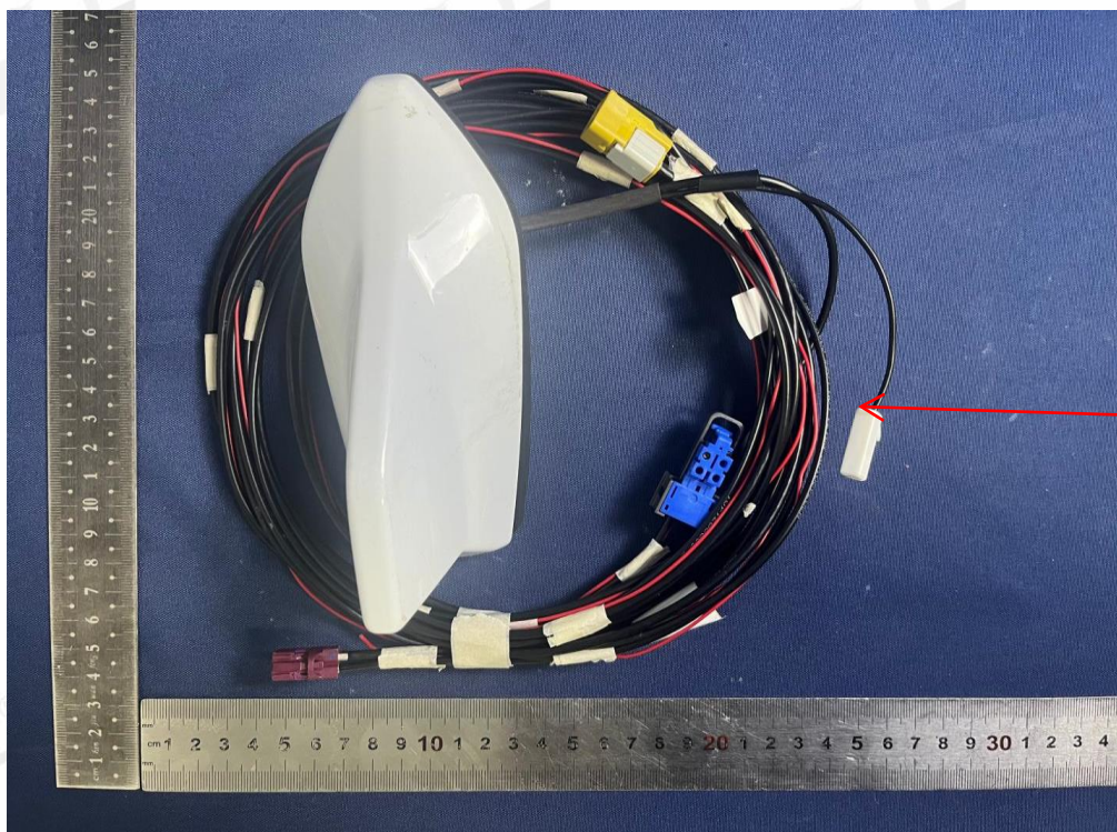
AM/FM antenna
