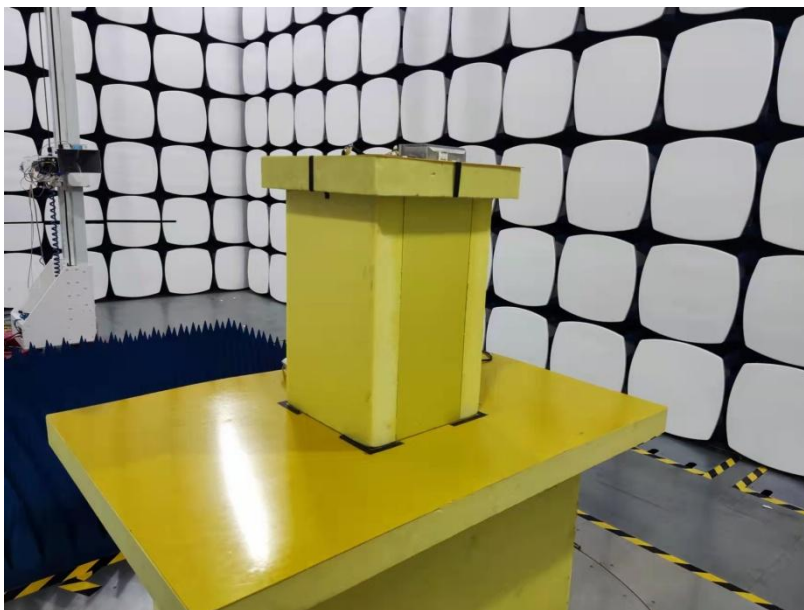
RADIATED EMISSIONS (1~18GHz)
