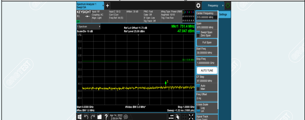
Band41-10MHz-16QAM-41540-1RB#0-Range1:30~1000MHz
