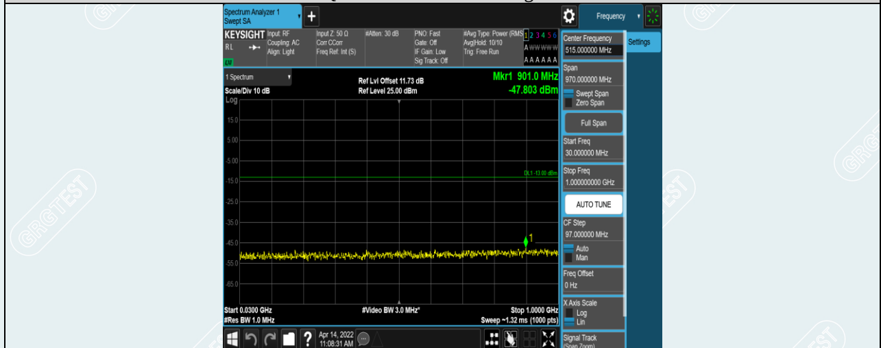
Band38-20MHz-QPSK-38150-1RB#0-Range1:30~1000MHz
