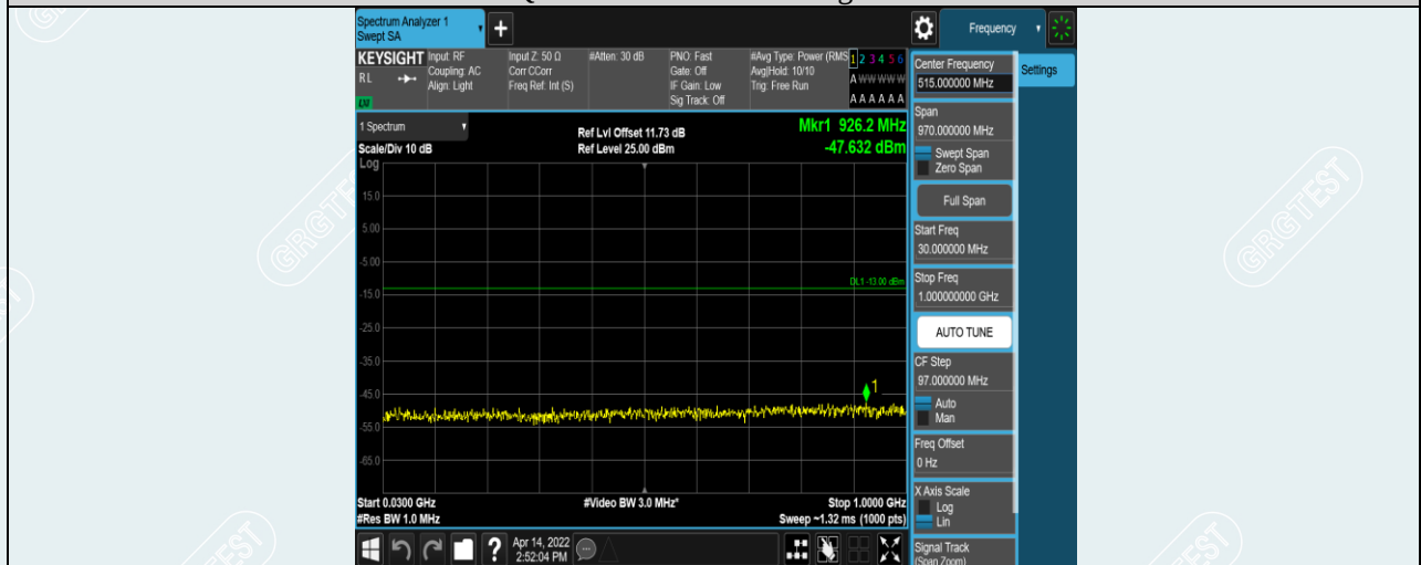
Band41-5MHz-16QAM-39675-1RB#0-Range1:30~1000MHz
