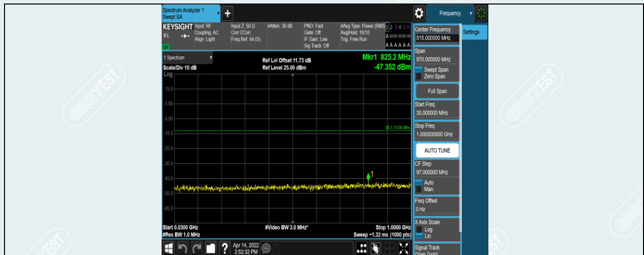
Band41-5MHz-QPSK-40620-1RB#0-Range1:30~1000MHz
