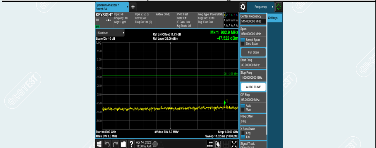
Band38-20MHz-16QAM-38150-1RB#0-Range1:30~1000MHz
