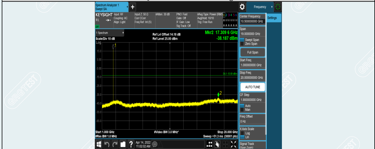
Band38-15MHz-QPSK-37825-1RB#0-Range2:1000~20000MHz
