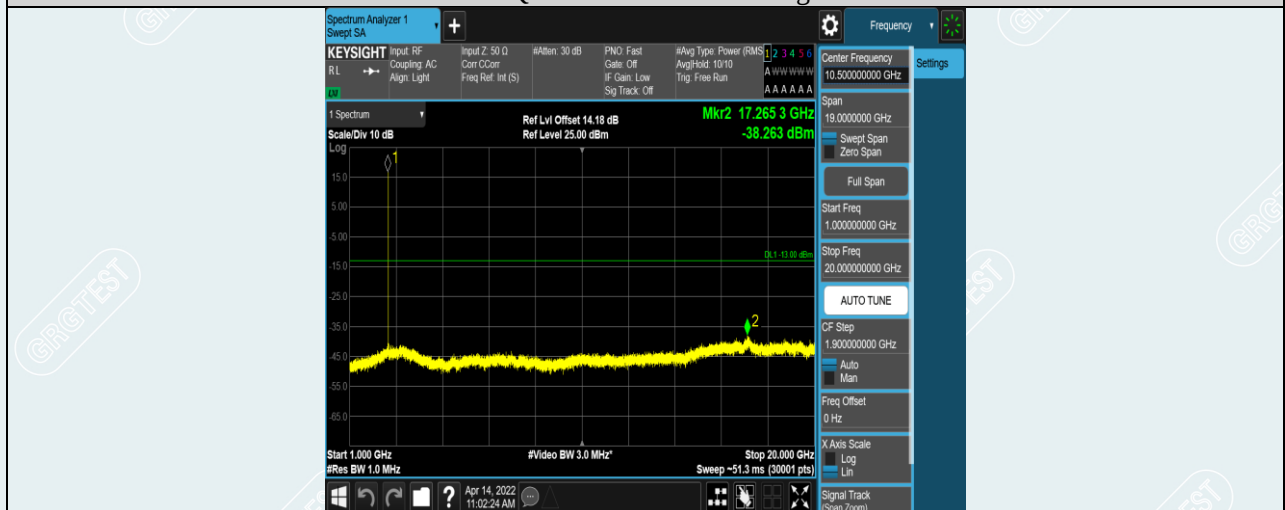
Band38-15MHz-16QAM-37825-1RB#0-Range2:1000~20000MHz
