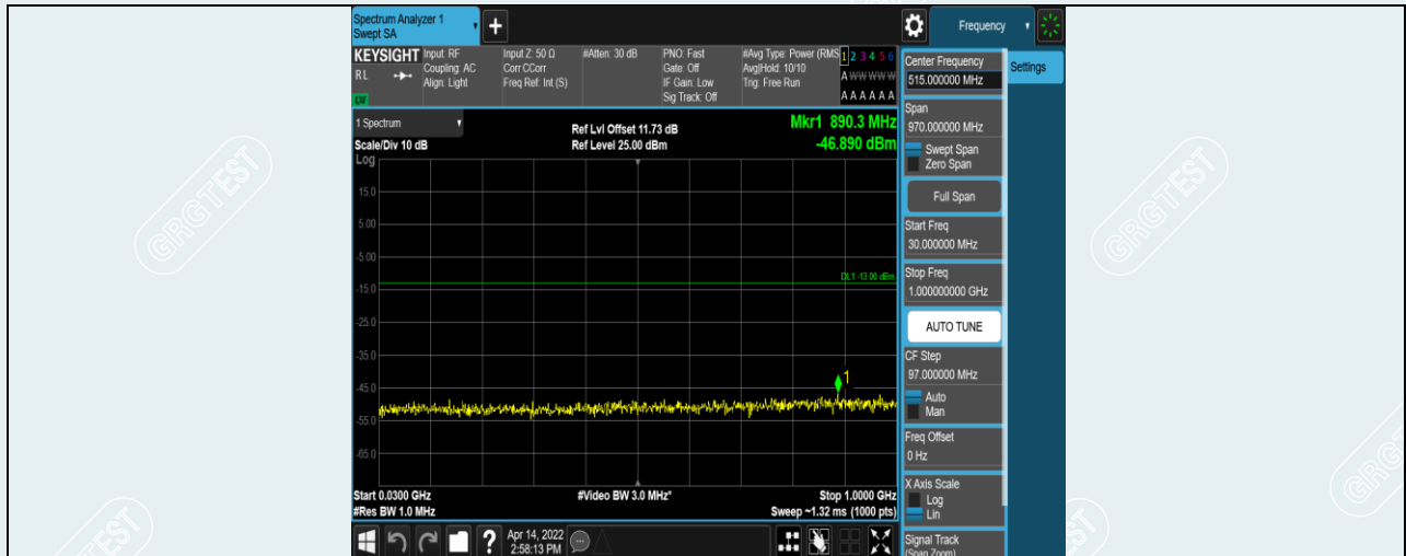
Band41-10MHz-16QAM-40620-1RB#0-Range1:30~1000MHz
