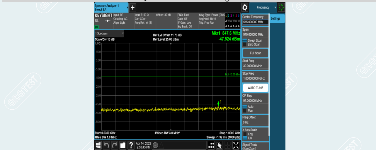
Band41-5MHz-16QAM-41565-1RB#0-Range1:30~1000MHz
