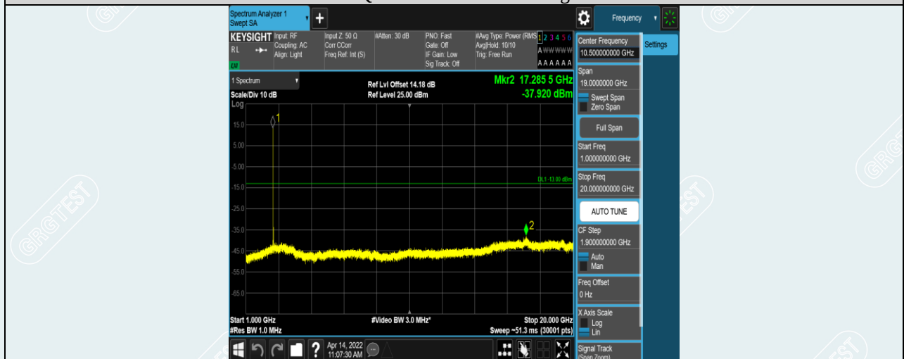
Band38-20MHz-16QAM-37850-1RB#0-Range2:1000~20000MHz
