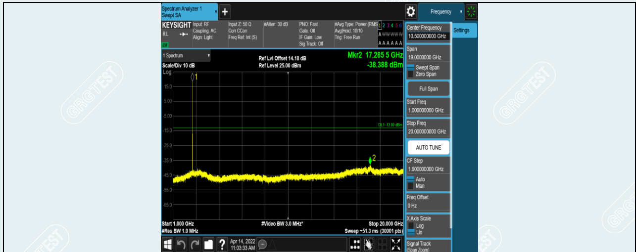
Band38-15MHz-QPSK-38175-1RB#0-Range2:1000~20000MHz
