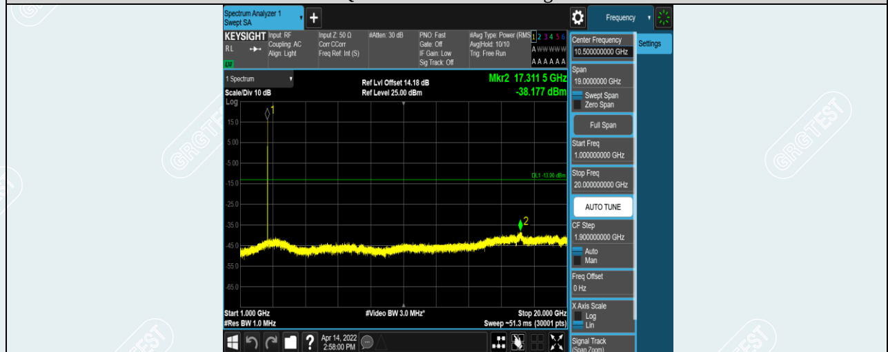
Band41-10MHz-QPSK-40620-1RB#0-Range2:1000~20000MHz
