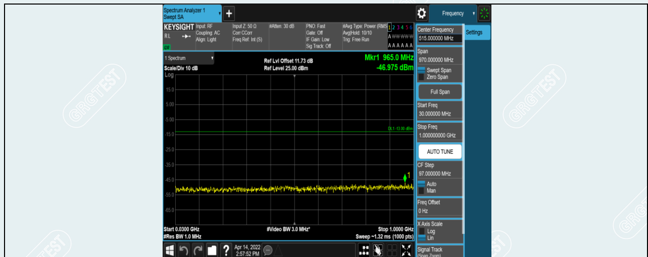
Band41-10MHz-QPSK-40620-1RB#0-Range1:30~1000MHz
