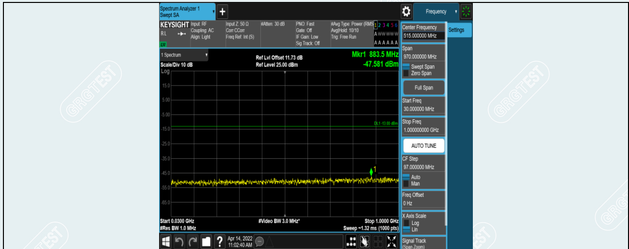
Band38-15MHz-QPSK-38000-1RB#0-Range1:30~1000MHz
