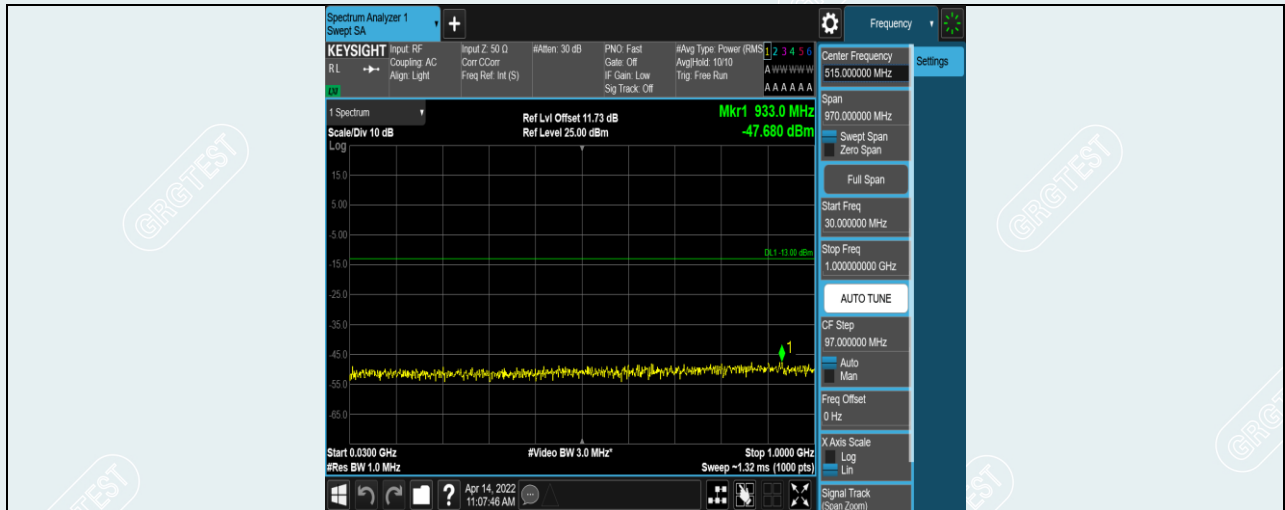
Band38-20MHz-QPSK-38000-1RB#0-Range1:30~1000MHz
