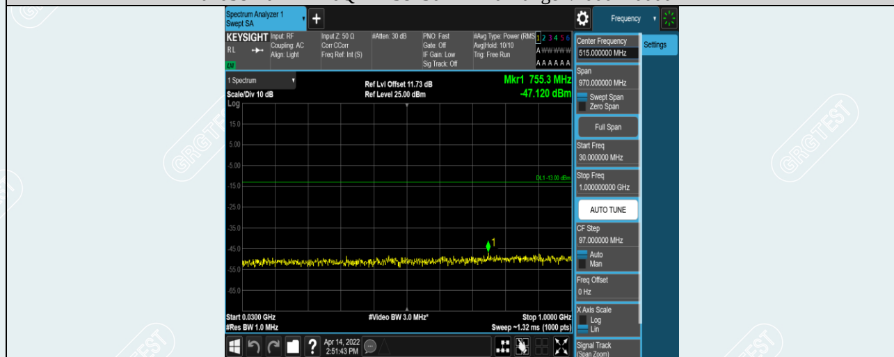
Band41-5MHz-QPSK-39675-1RB#0-Range1:30~1000MHz
