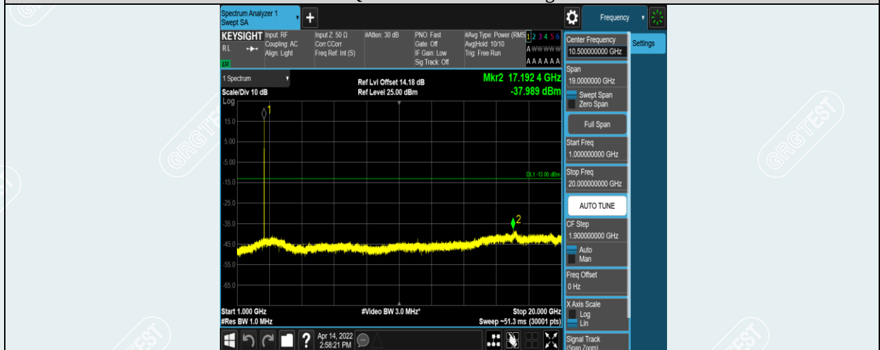
Band41-10MHz-16QAM-40620-1RB#0-Range2:1000~20000MHz
