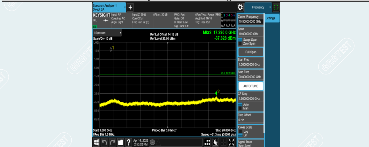
Band41-5MHz-16QAM-40620-1RB#0-Range2:1000~20000MHz
