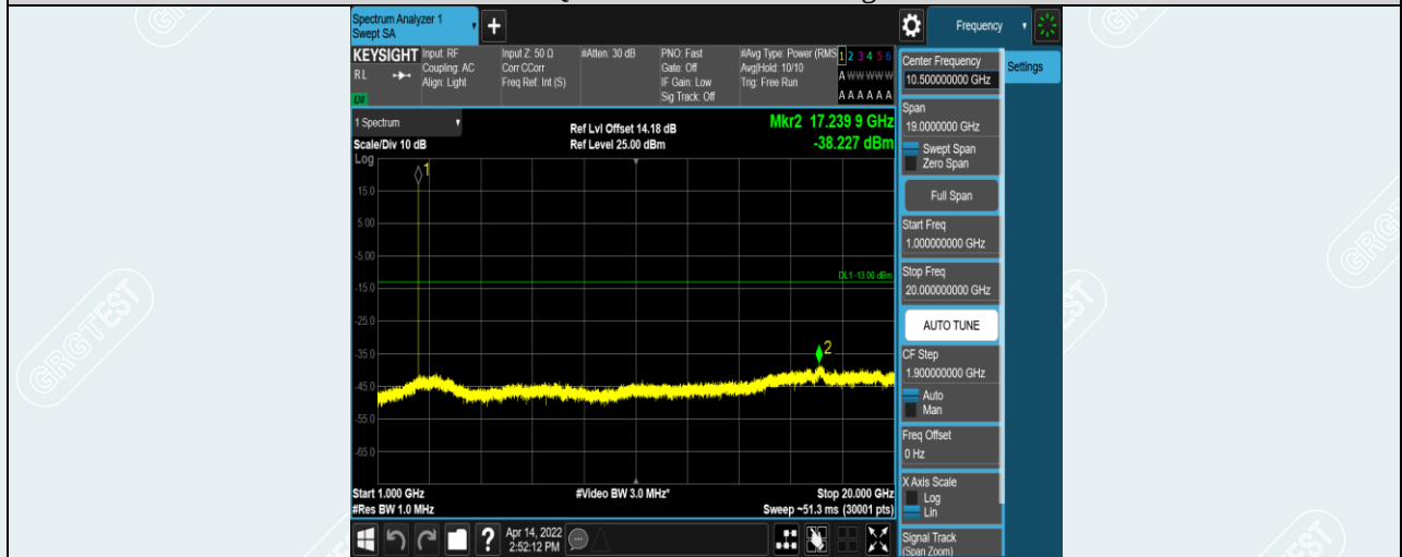
Band41-5MHz-16QAM-39675-1RB#0-Range2:1000~20000MHz
