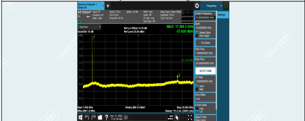
Band38-20MHz-QPSK-38000-1RB#0-Range2:1000~20000MHz
