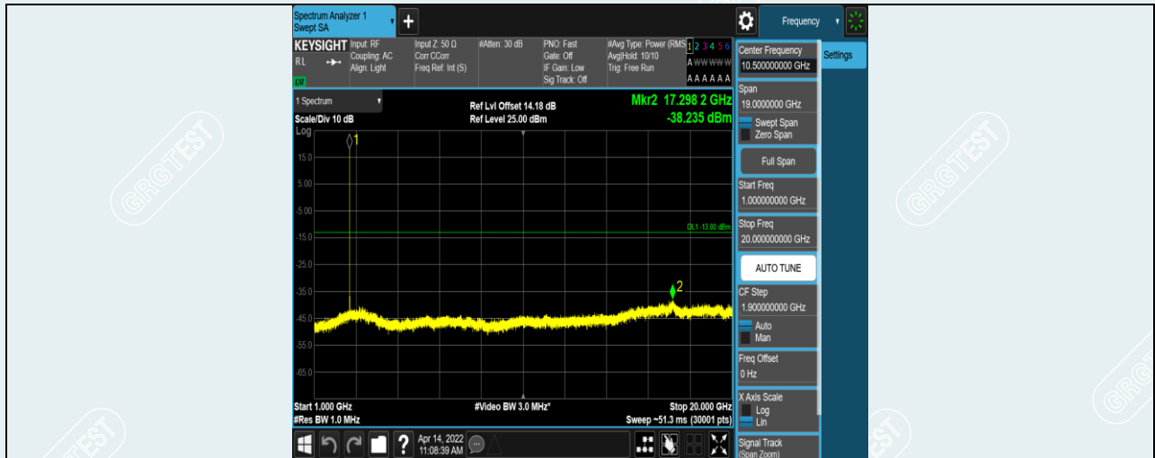
Band38-20MHz-QPSK-38150-1RB#0-Range2:1000~20000MHz
