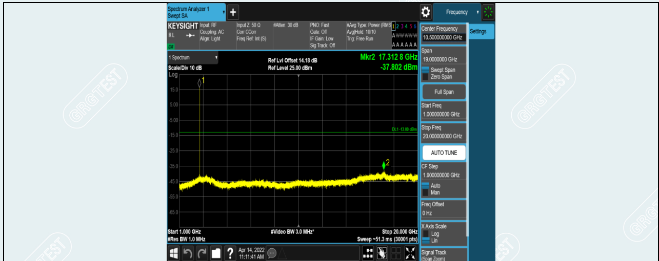
Band38-10MHz-16QAM-38200-1RB#0-Range2:1000~20000MHz
