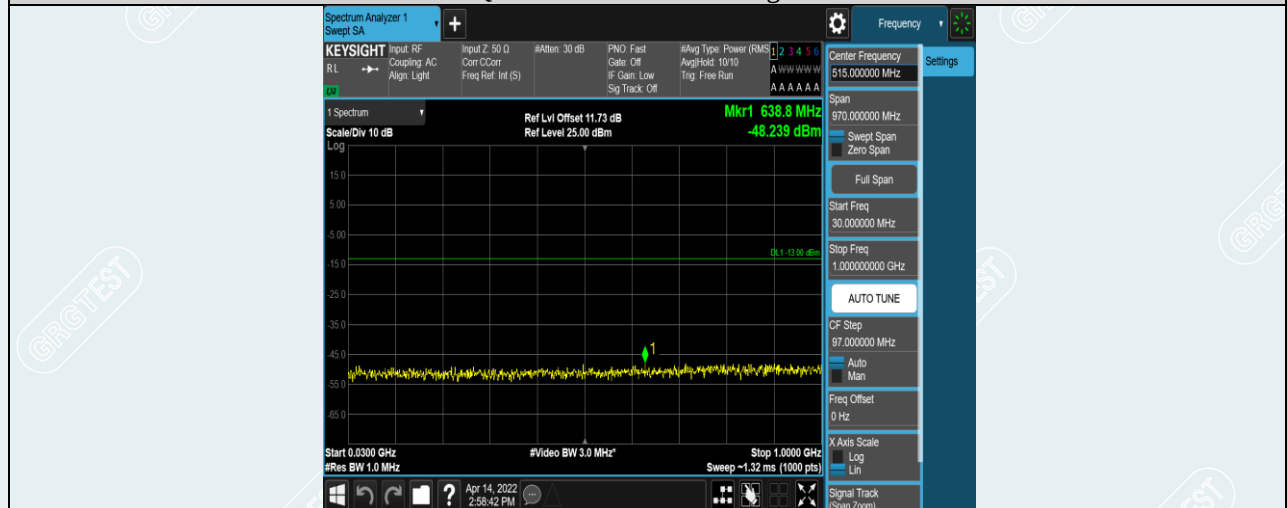
Band41-10MHz-QPSK-41540-1RB#0-Range1:30~1000MHz
