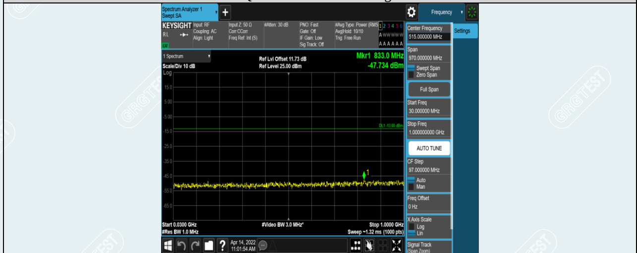
Band38-15MHz-QPSK-37825-1RB#0-Range1:30~1000MHz
