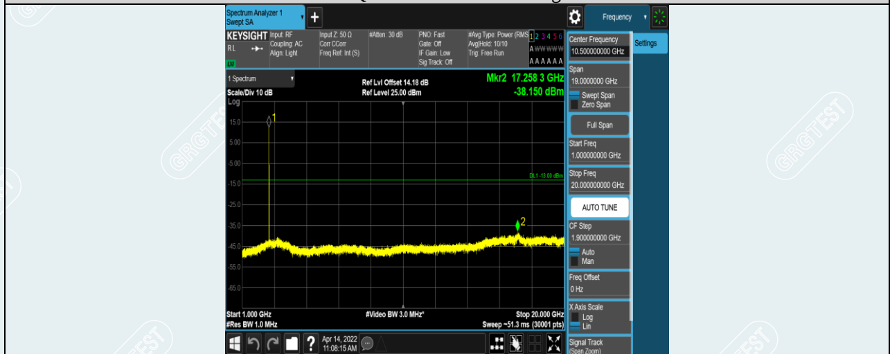
Band38-20MHz-16QAM-38000-1RB#0-Range2:1000~20000MHz
