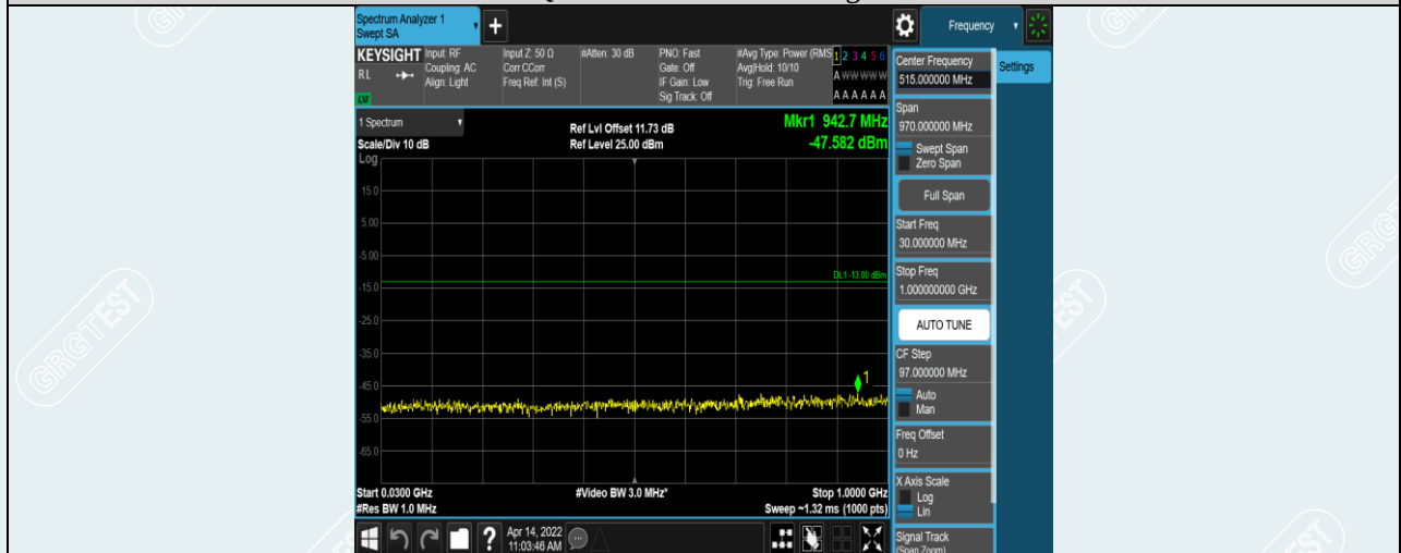
Band38-15MHz-16QAM-38175-1RB#0-Range1:30~1000MHz
