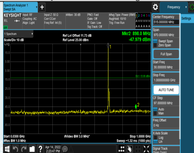
Band17-10MHz-QPSK-23800-1RB#0-Range1:30~1000MHz
