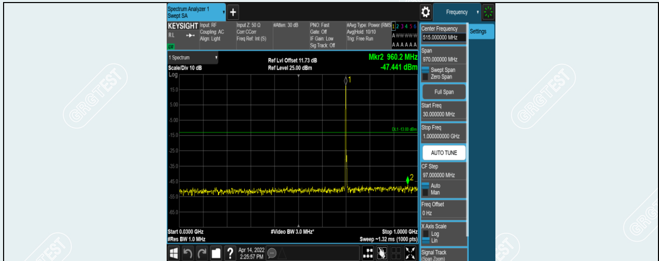
Band17-5MHz-16QAM-23790-1RB#0-Range1:30~1000MHz
