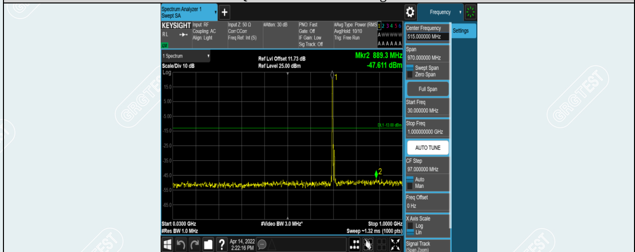
Band17-10MHz-QPSK-23780-1RB#0-Range1:30~1000MHz
