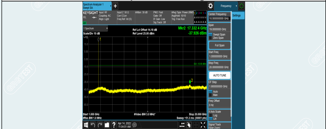
Band38-5MHz-16QAM-37775-1RB#0-Range2:1000~20000MHz
