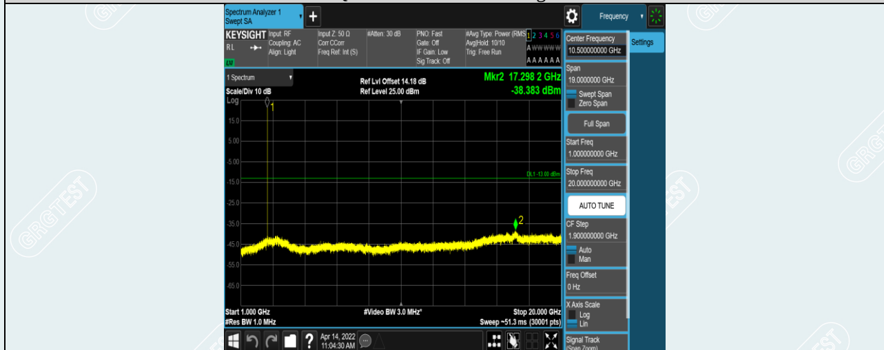
Band38-5MHz-QPSK-37775-1RB#0-Range2:1000~20000MHz
