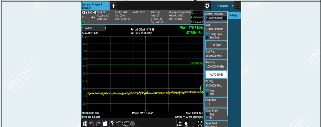
Band38-10MHz-16QAM-38200-1RB#0-Range1:30~1000MHz
