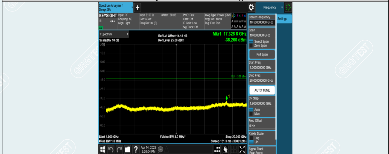
Band17-5MHz-16QAM-23790-1RB#0-Range2:1000~20000MHz
