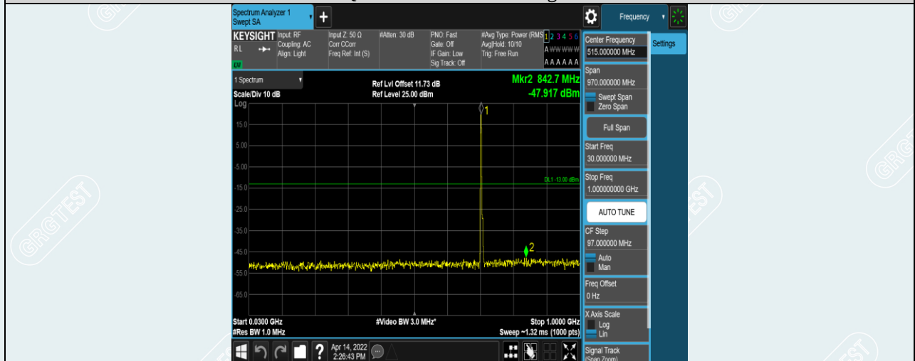
Band17-5MHz-16QAM-23825-1RB#0-Range1:30~1000MHz
