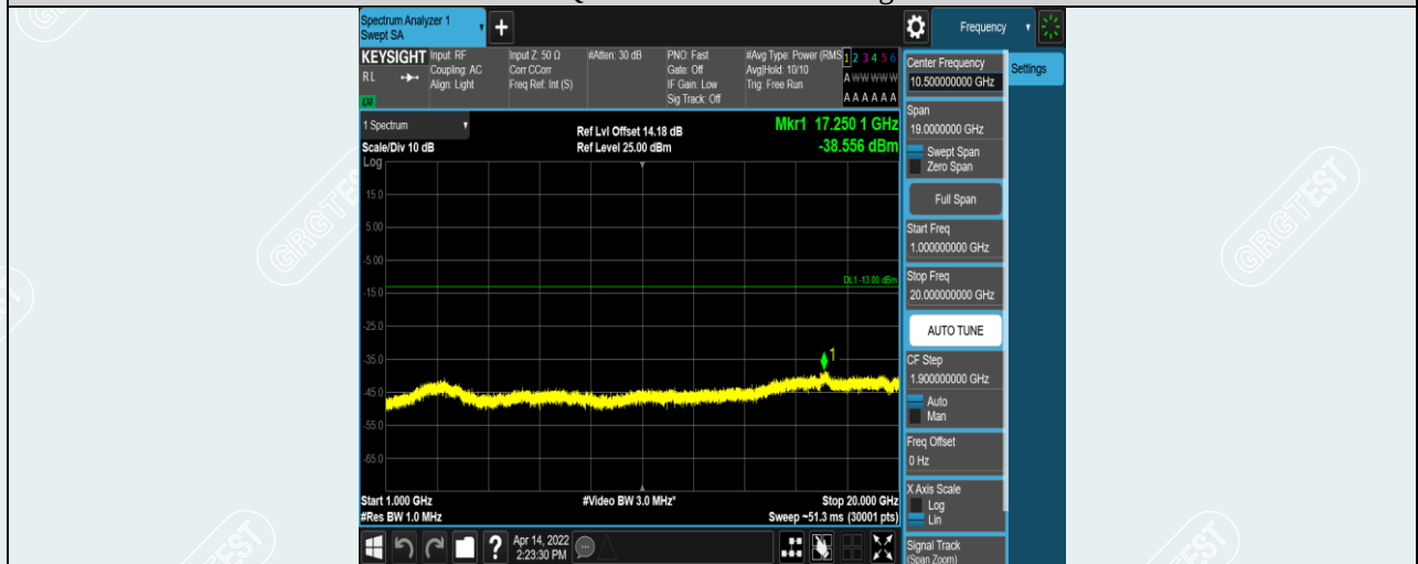
Band17-10MHz-16QAM-23790-1RB#0-Range2:1000~20000MHz
