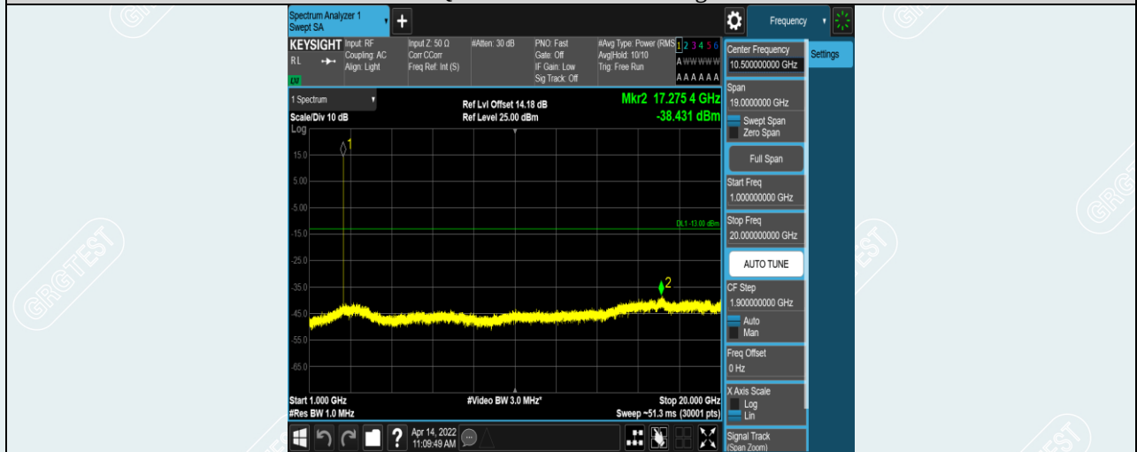
Band38-10MHz-QPSK-37800-1RB#0-Range2:1000~20000MHz
