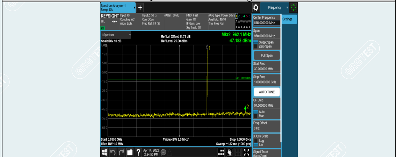
Band17-5MHz-QPSK-23755-1RB#0-Range1:30~1000MHz
