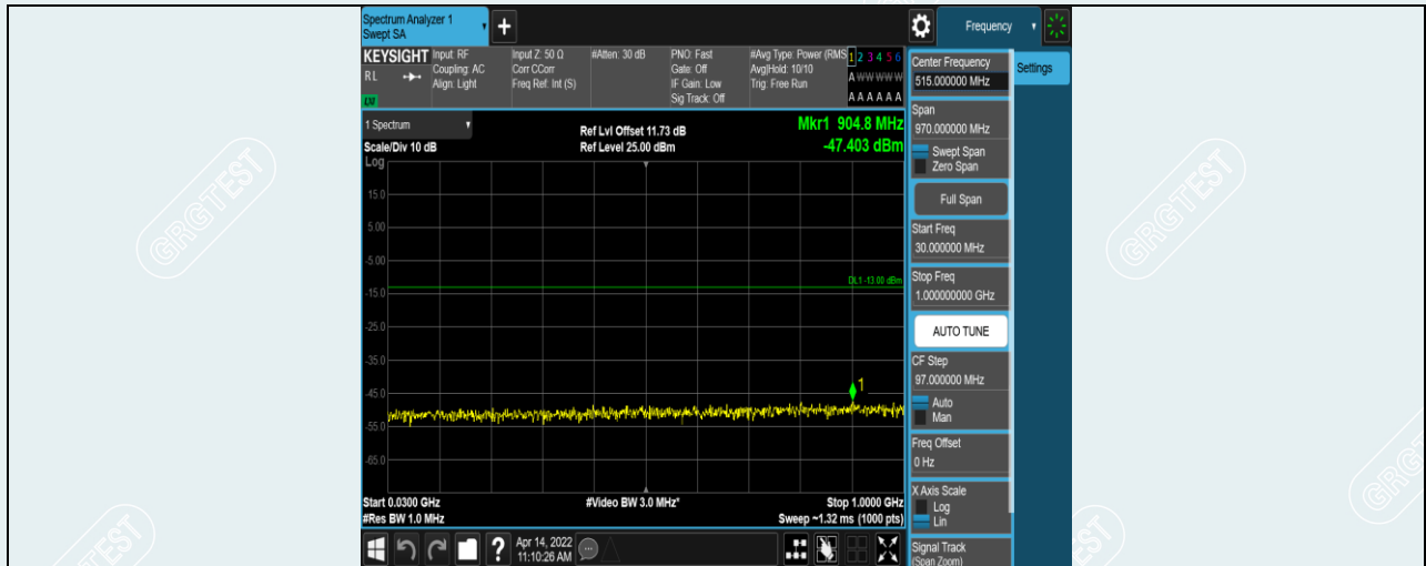
Band38-10MHz-QPSK-38000-1RB#0-Range1:30~1000MHz
