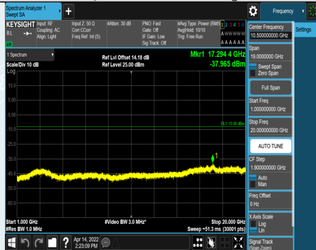
Band17-10MHz-QPSK-23790-1RB#0-Range2:1000~20000MHz
