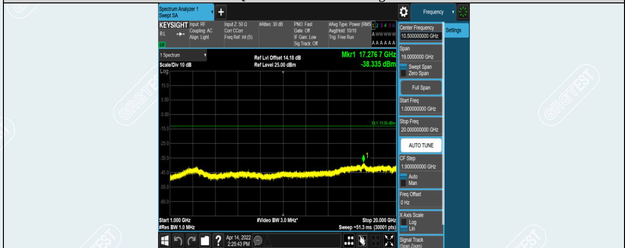
Band17-5MHz-QPSK-23790-1RB#0-Range2:1000~20000MHz
