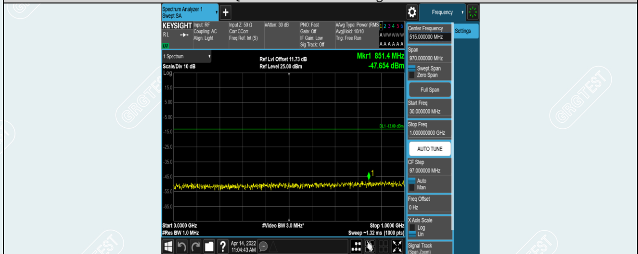
Band38-5MHz-16QAM-37775-1RB#0-Range1:30~1000MHz
