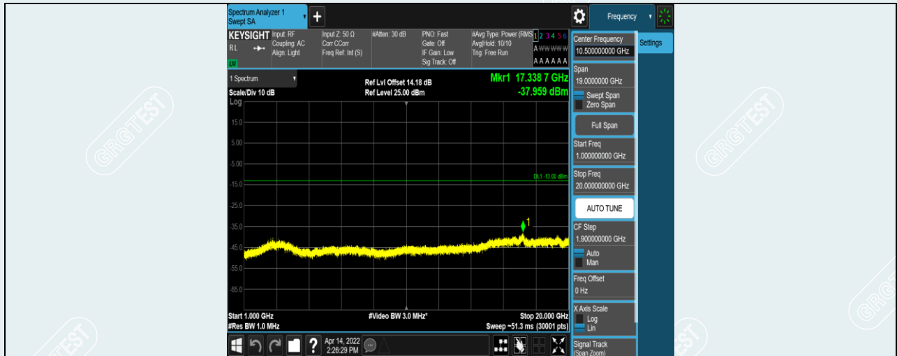
Band17-5MHz-QPSK-23825-1RB#0-Range2:1000~20000MHz
