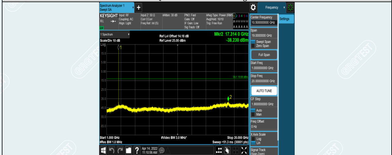
Band38-10MHz-16QAM-38000-1RB#0-Range2:1000~20000MHz
