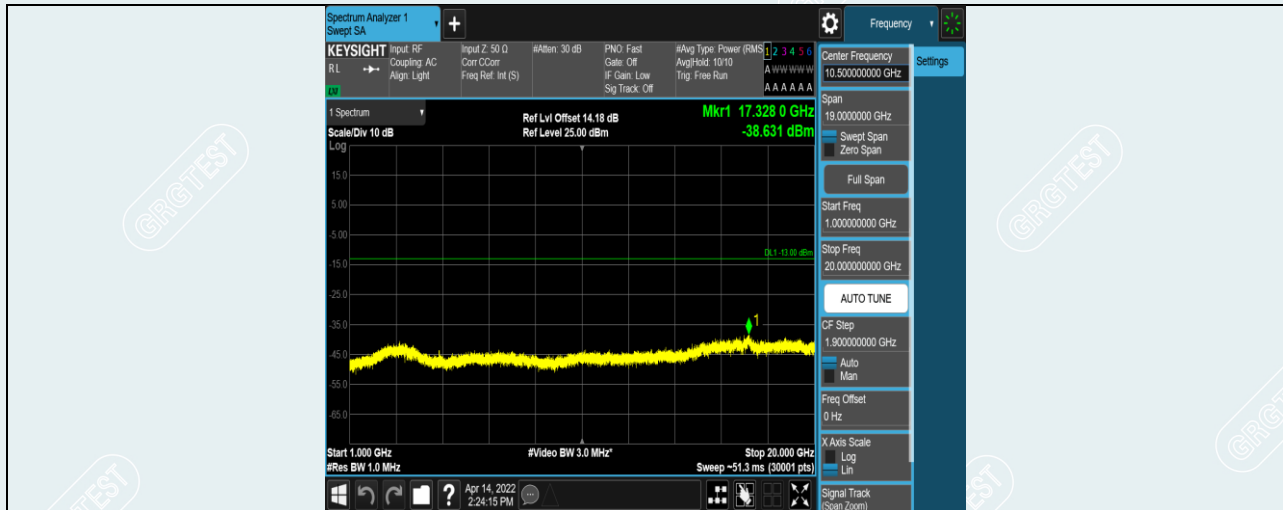
Band17-10MHz-16QAM-23800-1RB#0-Range2:1000~20000MHz
