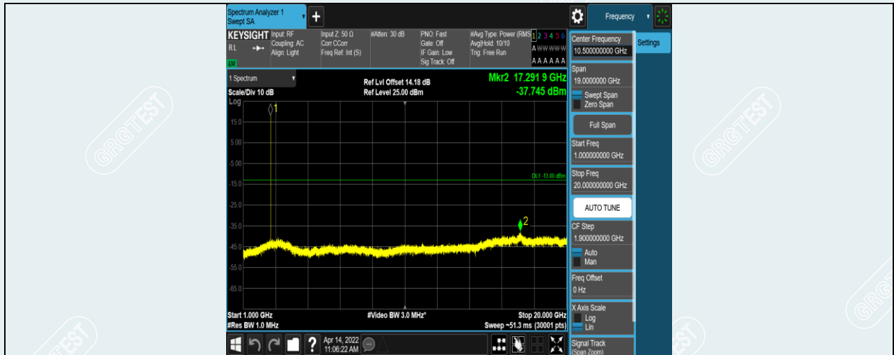
Band38-5MHz-16QAM-38225-1RB#0-Range2:1000~20000MHz
