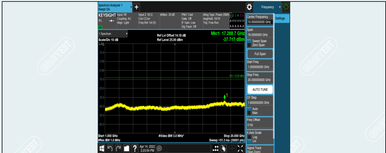
Band17-10MHz-QPSK-23800-1RB#0-Range2:1000~20000MHz
