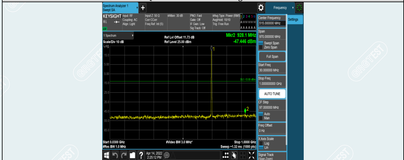
Band17-5MHz-16QAM-23755-1RB#0-Range1:30~1000MHz
