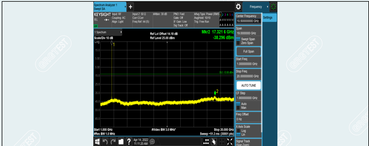
Band38-10MHz-QPSK-38200-1RB#0-Range2:1000~20000MHz
