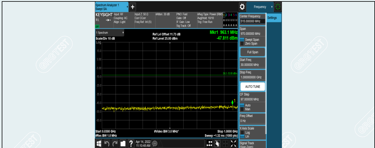
Band38-10MHz-16QAM-38000-1RB#0-Range1:30~1000MHz
