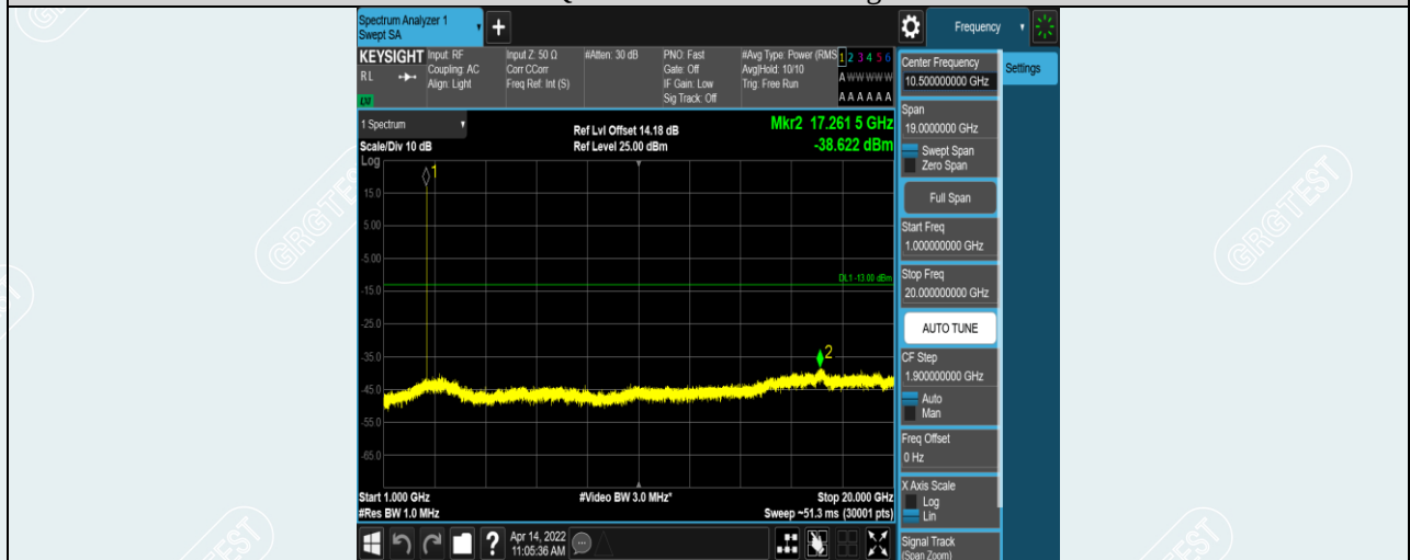
Band38-5MHz-16QAM-38000-1RB#0-Range2:1000~20000MHz
