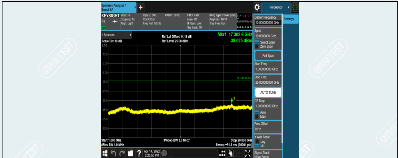
Band17-5MHz-16QAM-23825-1RB#0-Range2:1000~20000MHz
