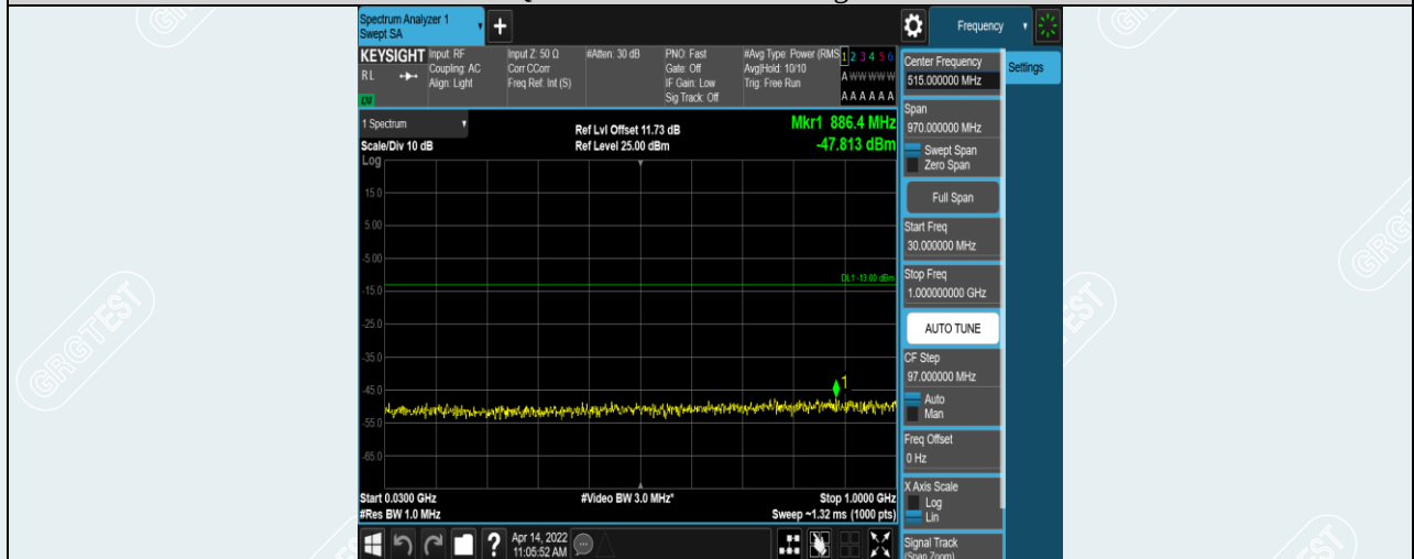
Band38-5MHz-QPSK-38225-1RB#0-Range1:30~1000MHz
