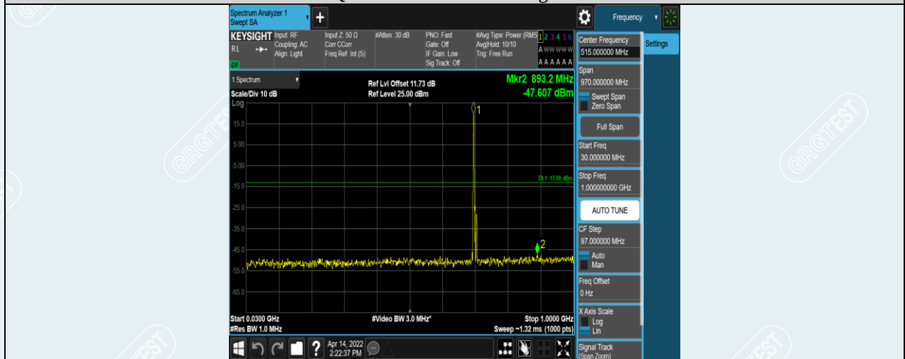
Band17-10MHz-16QAM-23780-1RB#0-Range1:30~1000MHz
