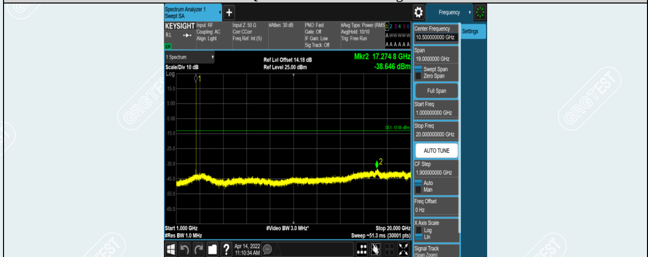
Band38-10MHz-QPSK-38000-1RB#0-Range2:1000~20000MHz
