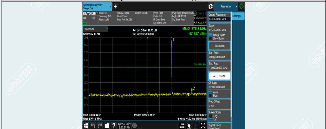
Band17-5MHz-QPSK-23825-1RB#0-Range1:30~1000MHz
