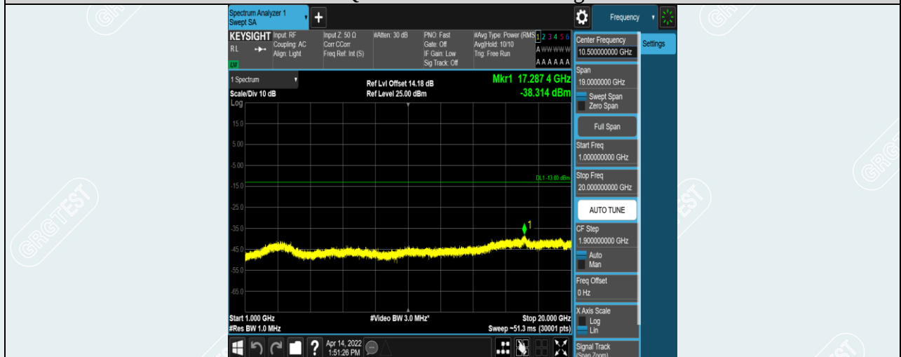
Band13-10MHz-16QAM-23230-1RB#0-Range5:1000~20000MHz
