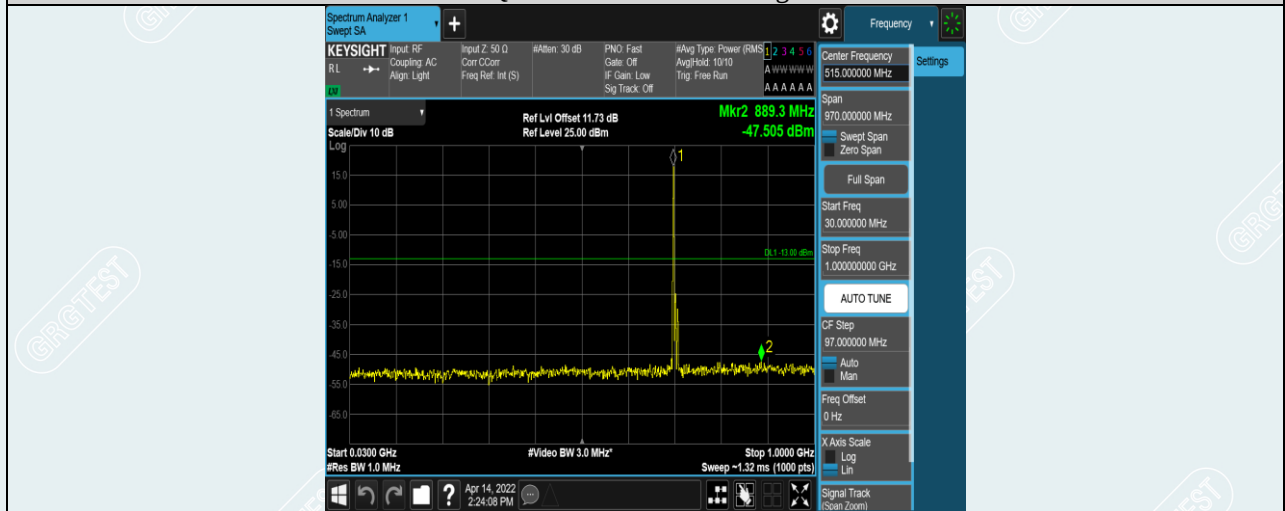
Band17-10MHz-16QAM-23800-1RB#0-Range1:30~1000MHz
