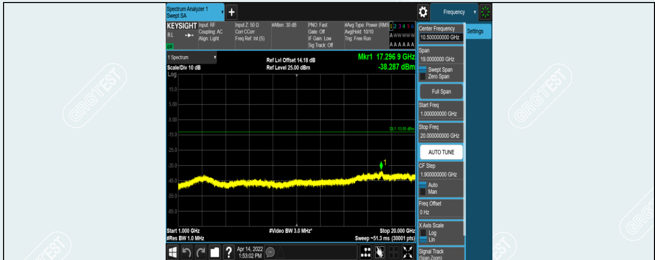
Band13-5MHz-16QAM-23205-1RB#0-Range5:1000~20000MHz
