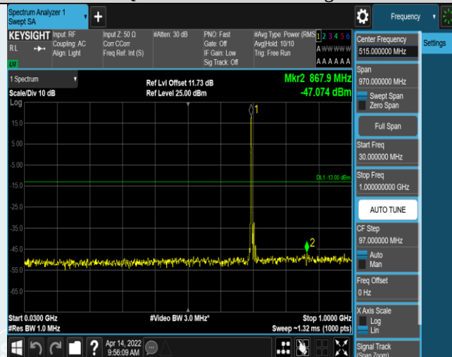
Band12-10MHz-16QAM-23095-1RB#0-Range1:30~1000MHz
