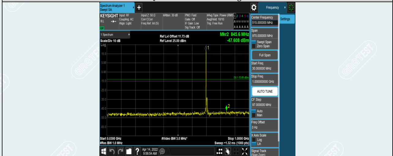
Band12-10MHz-16QAM-23130-1RB#0-Range1:30~1000MHz
