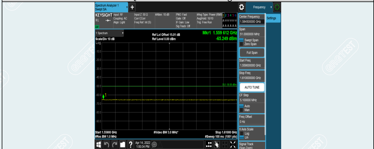
Band13-10MHz-QPSK-23230-1RB#0-Range3:1559~1610MHz
