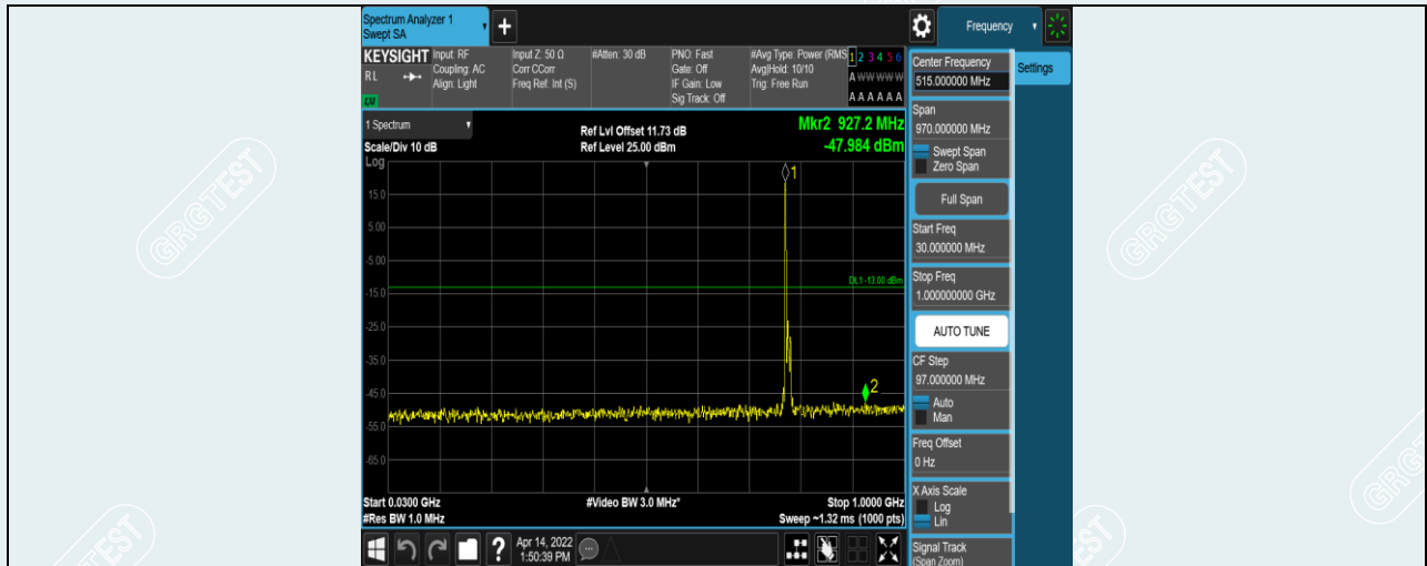
Band13-10MHz-QPSK-23230-1RB#0-Range4:30~1000MHz
