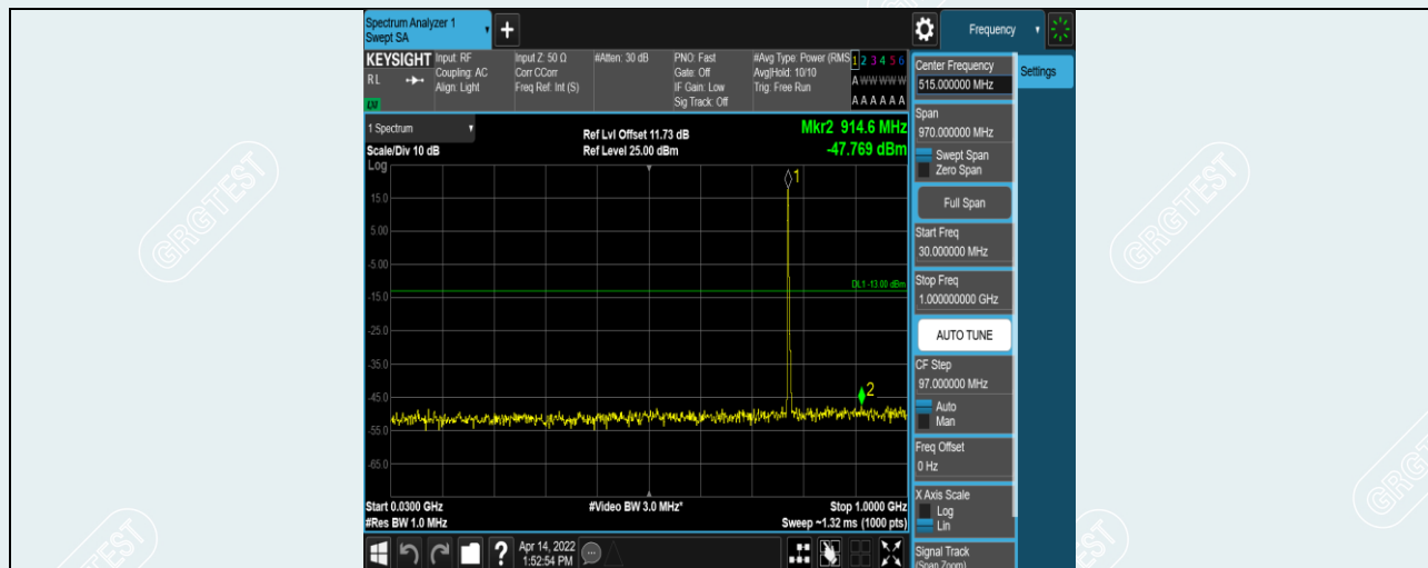
Band13-5MHz-16QAM-23205-1RB#0-Range4:30~1000MHz
