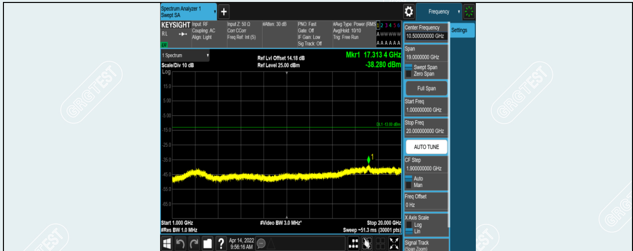
Band12-10MHz-16QAM-23095-1RB#0-Range2:1000~20000MHz
