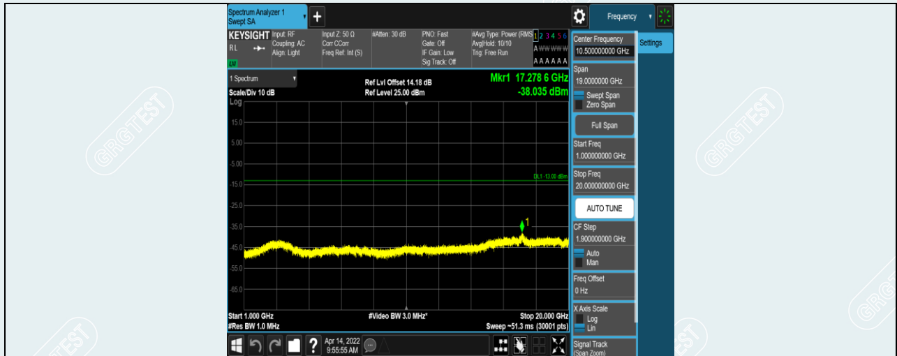
Band12-10MHz-QPSK-23095-1RB#0-Range2:1000~20000MHz
