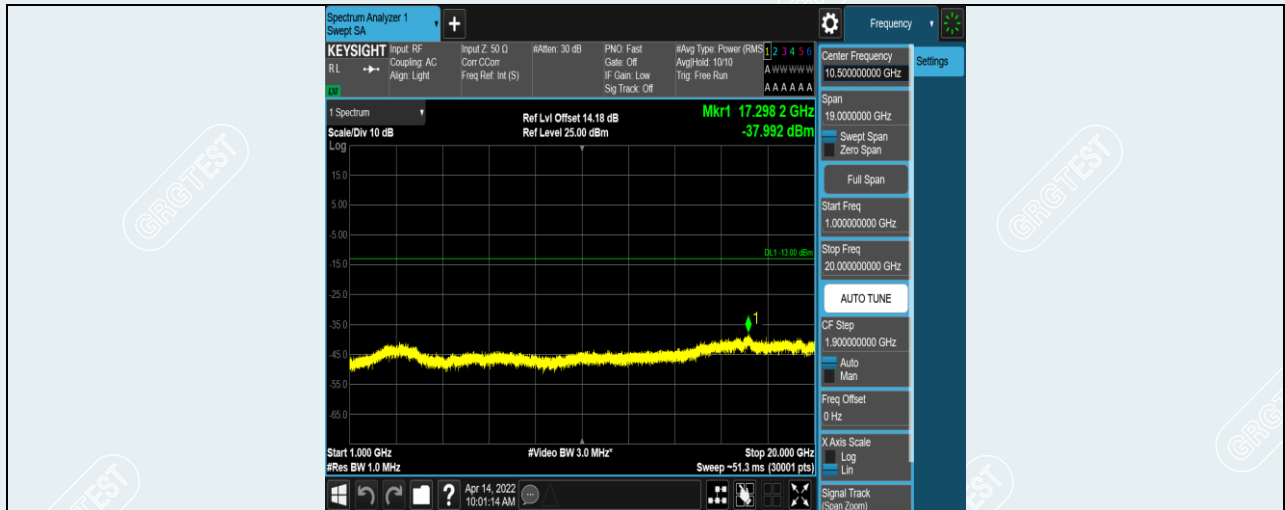
Band12-5MHz-16QAM-23095-1RB#0-Range2:1000~20000MHz
