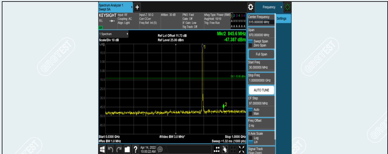
Band12-5MHz-16QAM-23035-1RB#0-Range1:30~1000MHz
