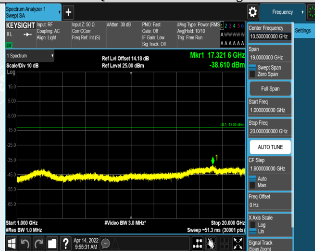
Band12-10MHz-16QAM-23060-1RB#0-Range2:1000~20000MHz
