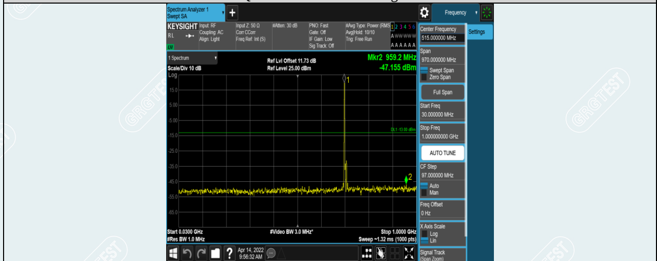
Band12-10MHz-QPSK-23130-1RB#0-Range1:30~1000MHz
