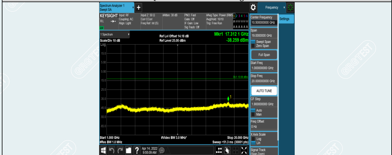
Band12-10MHz-QPSK-23060-1RB#0-Range2:1000~20000MHz
