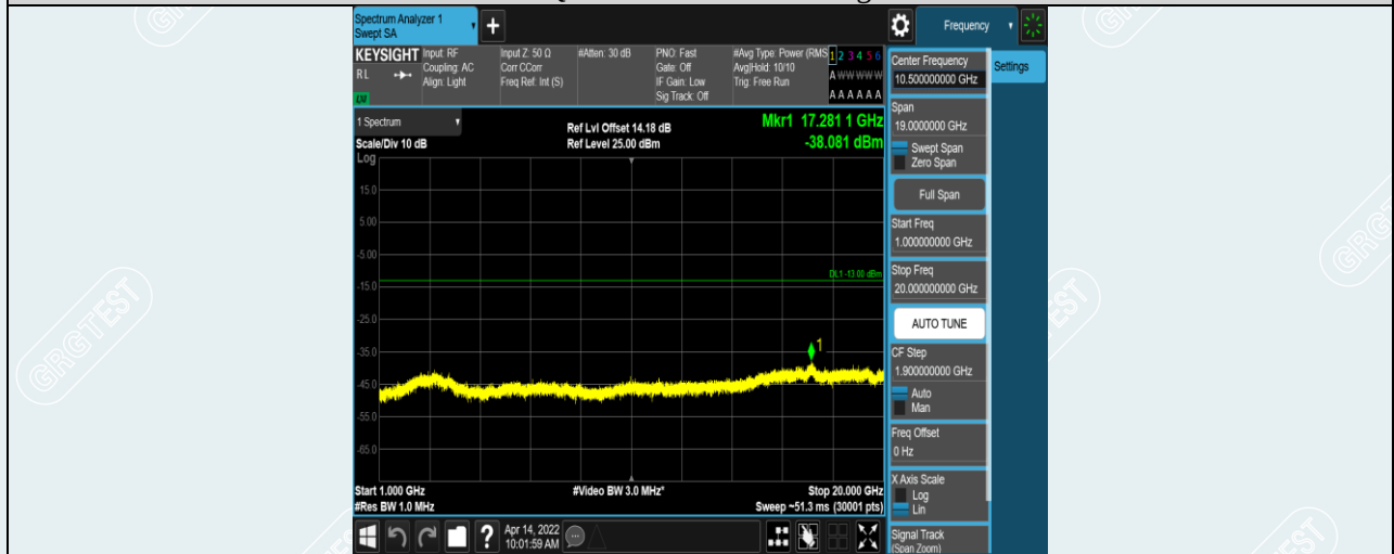
Band12-5MHz-16QAM-23155-1RB#0-Range2:1000~20000MHz
