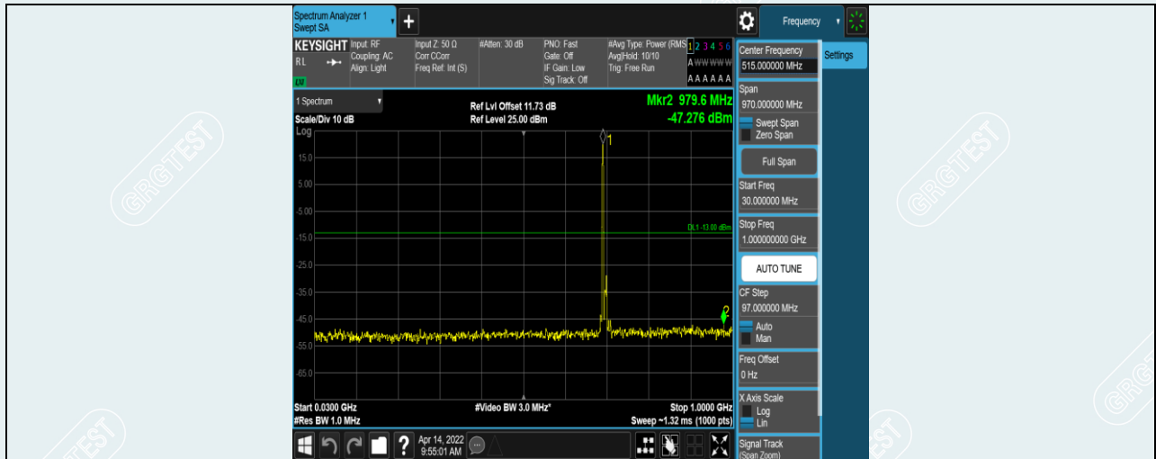
Band12-10MHz-QPSK-23060-1RB#0-Range1:30~1000MHz
