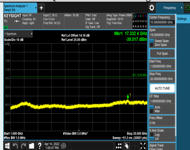
Band13-5MHz-16QAM-23255-1RB#0-Range5:1000~20000MHz
