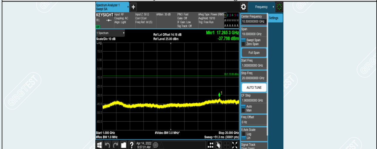
Band12-10MHz-16QAM-23130-1RB#0-Range2:1000~20000MHz
