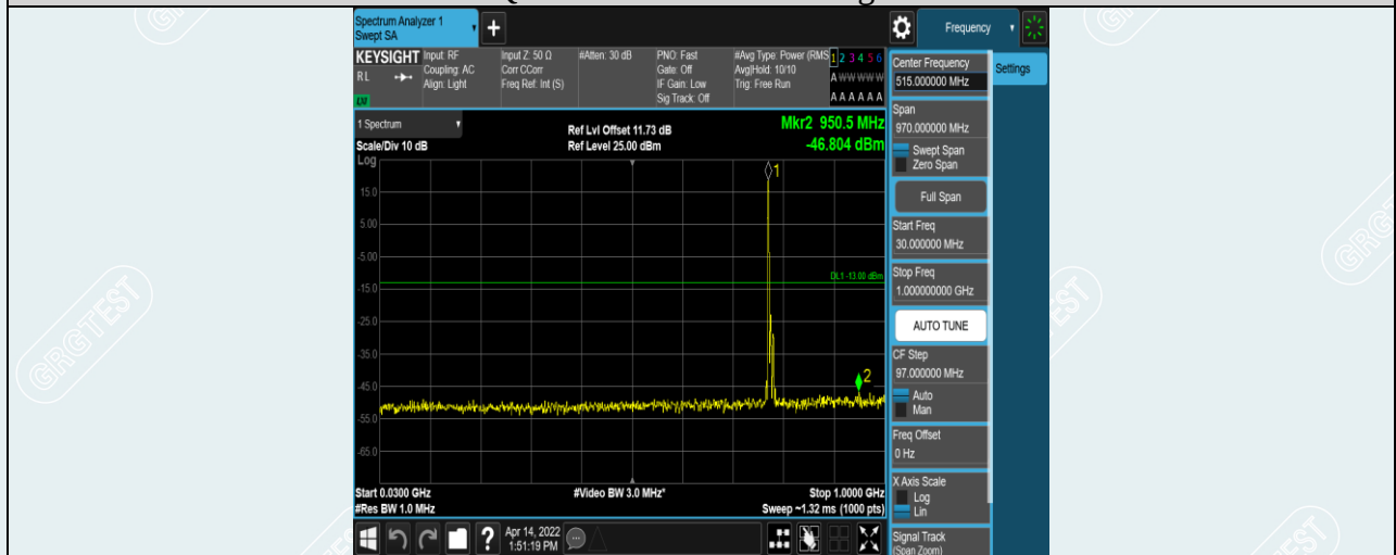
Band13-10MHz-16QAM-23230-1RB#0-Range4:30~1000MHz
