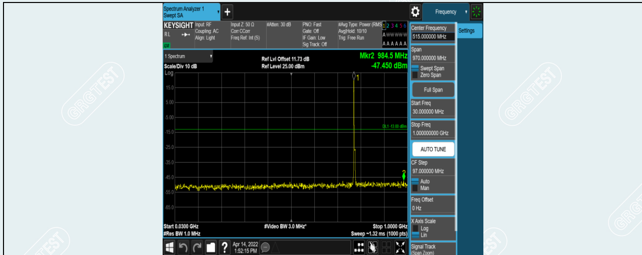
Band13-5MHz-QPSK-23205-1RB#0-Range4:30~1000MHz
