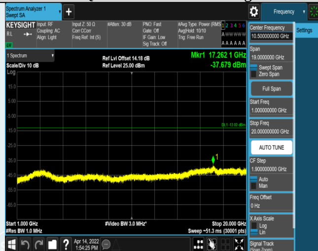
Band13-5MHz-16QAM-23230-1RB#0-Range5:1000~20000MHz
