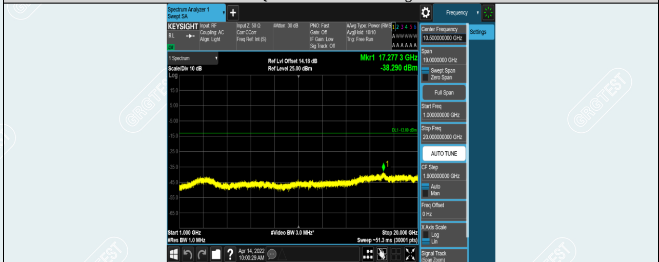
Band12-5MHz-16QAM-23035-1RB#0-Range2:1000~20000MHz
