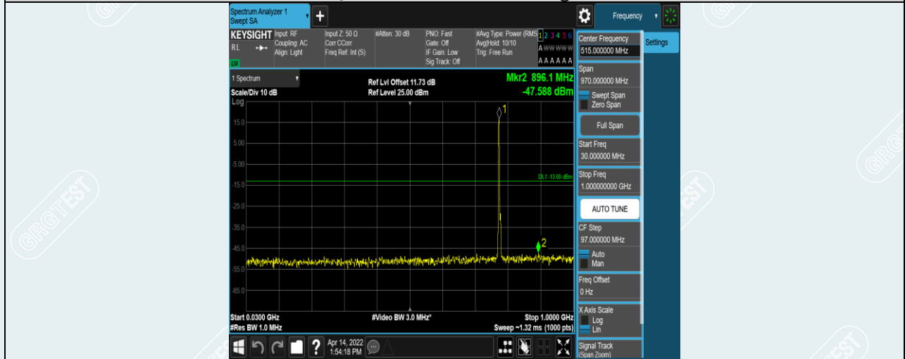
Band13-5MHz-16QAM-23230-1RB#0-Range4:30~1000MHz
