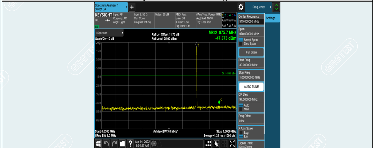
Band12-3MHz-16QAM-23165-1RB#0-Range1:30~1000MHz
