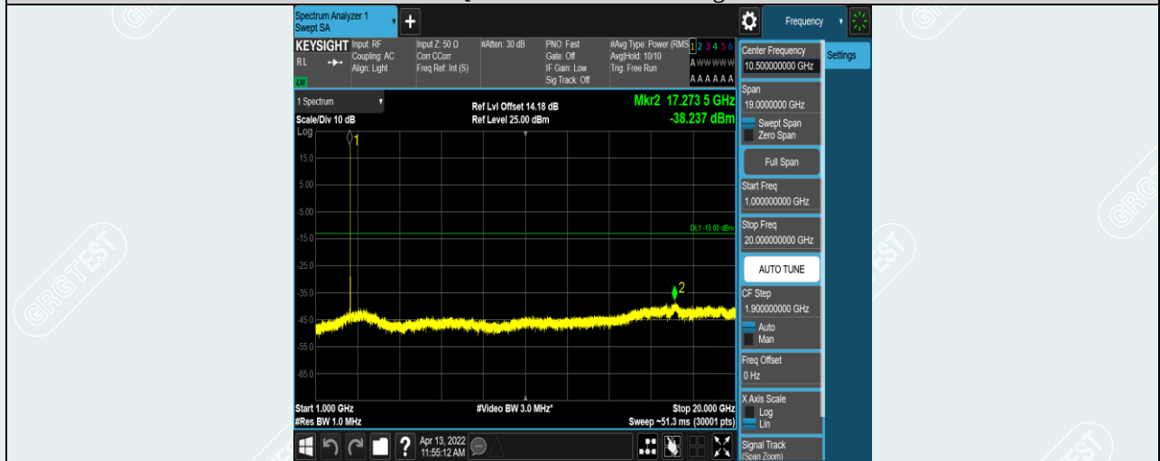
Band7-15MHz-16QAM-21375-1RB#0-Range2:1000~20000MHz
