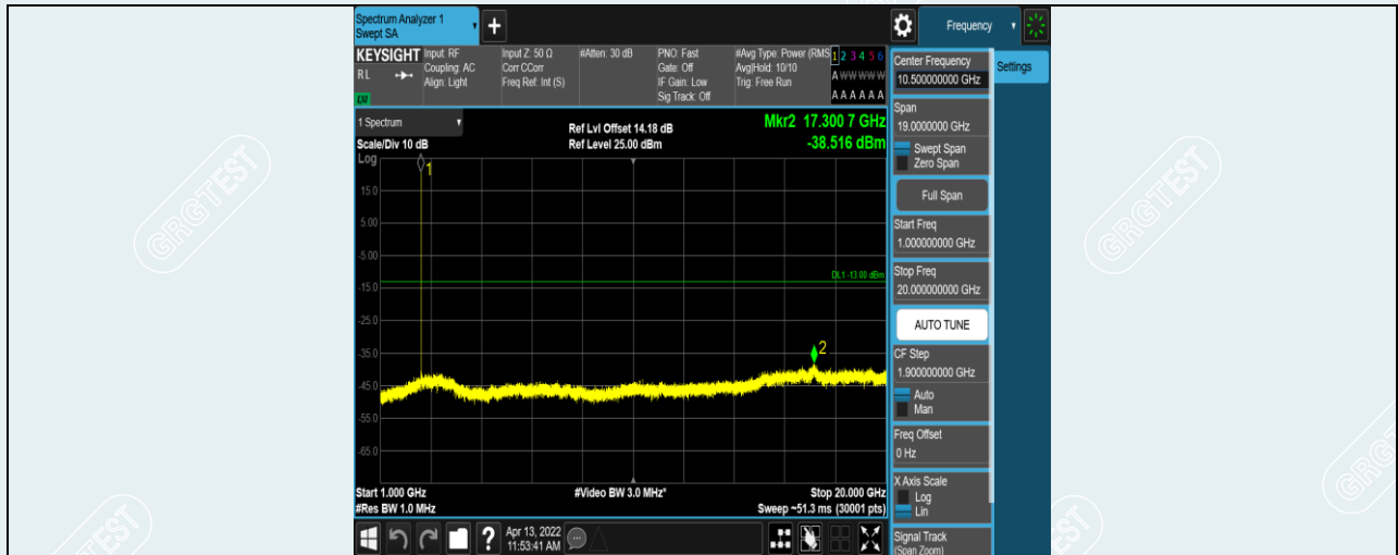
Band7-15MHz-16QAM-21100-1RB#0-Range2:1000~20000MHz
