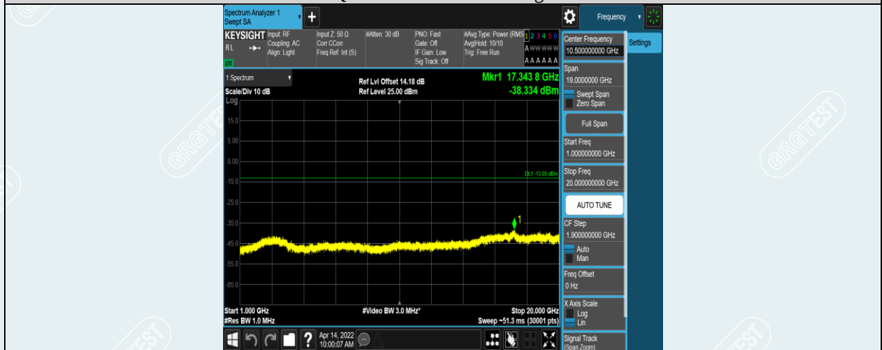
Band12-5MHz-QPSK-23035-1RB#0-Range2:1000~20000MHz
