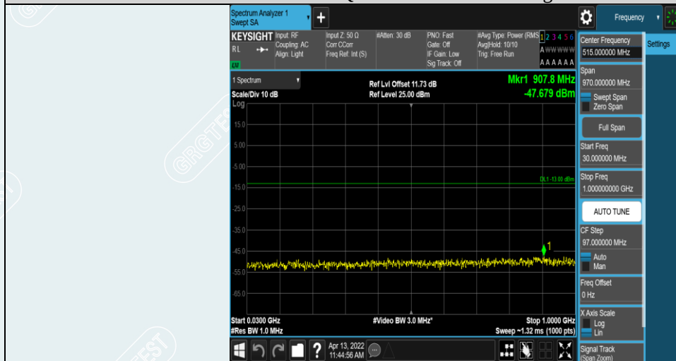
Band7-20MHz-16QAM-21350-1RB#0-Range1:30~1000MHz
