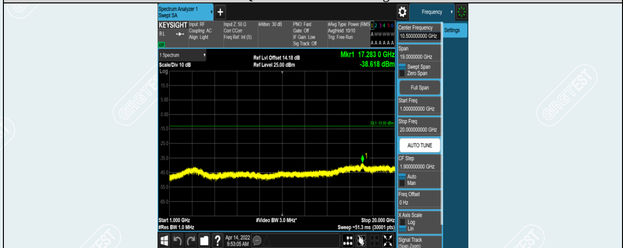
Band12-3MHz-16QAM-23025-1RB#0-Range2:1000~20000MHz
