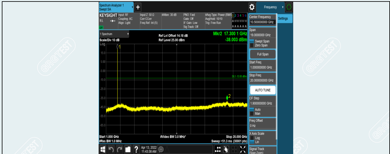
Band7-20MHz-16QAM-21100-1RB#0-Range2:1000~20000MHz
