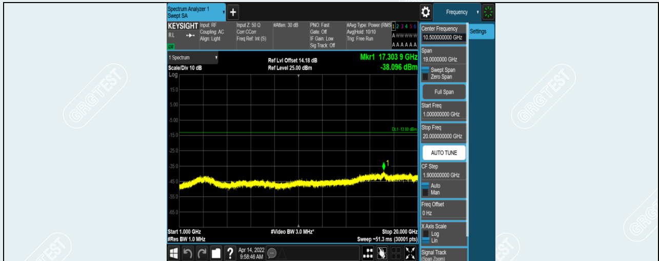
Band12-1.4MHz-16QAM-23095-1RB#0-Range2:1000~20000MHz
