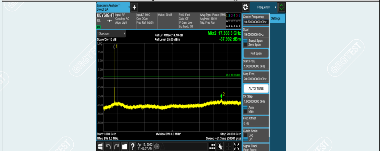
Band7-20MHz-16QAM-20850-1RB#0-Range2:1000~20000MHz
