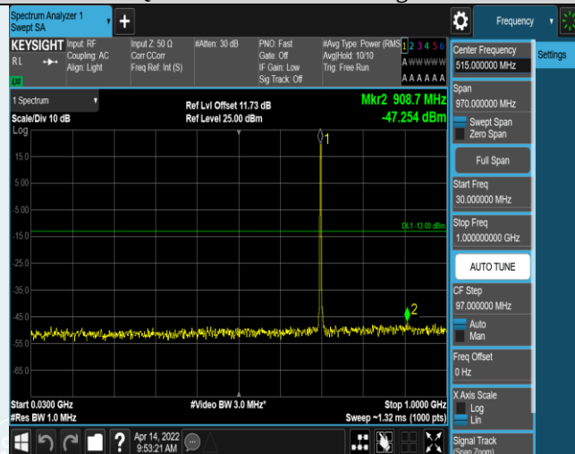
Band12-3MHz-QPSK-23095-1RB#0-Range1:30~1000MHz
