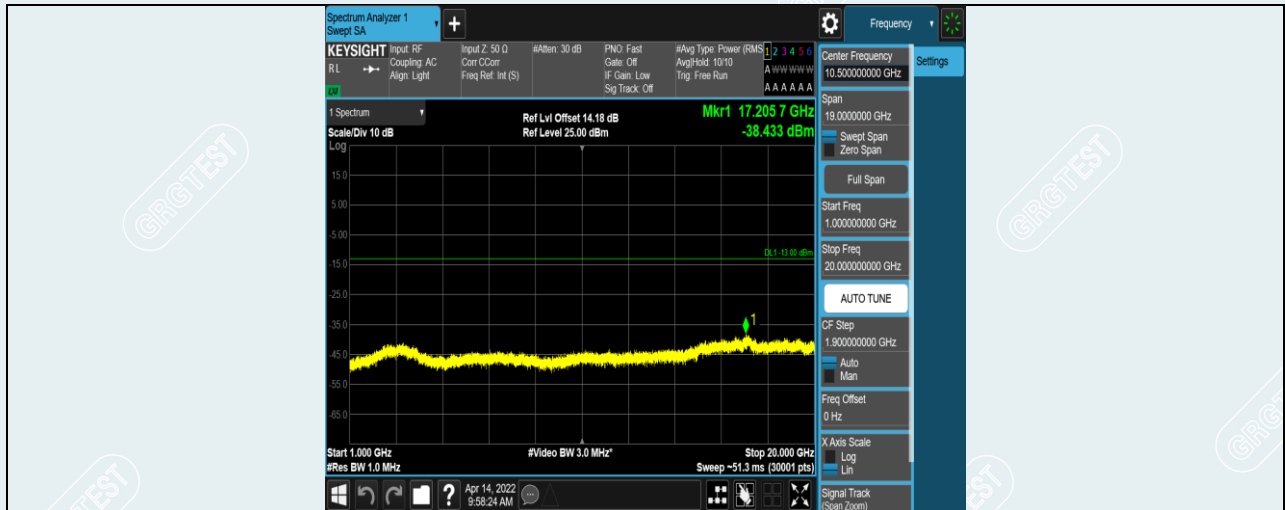
Band12-1.4MHz-QPSK-23095-1RB#0-Range2:1000~20000MHz
