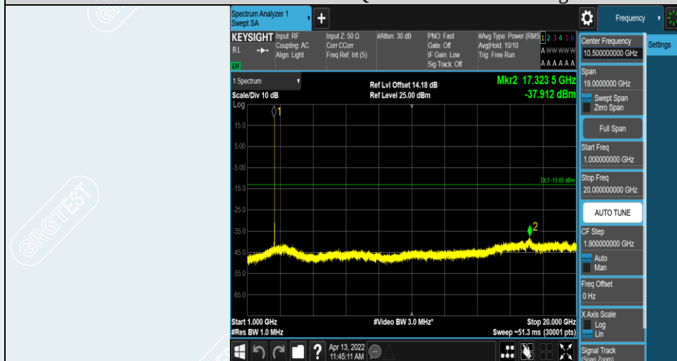
Band7-20MHz-16QAM-21350-1RB#0-Range2:1000~20000MHz
