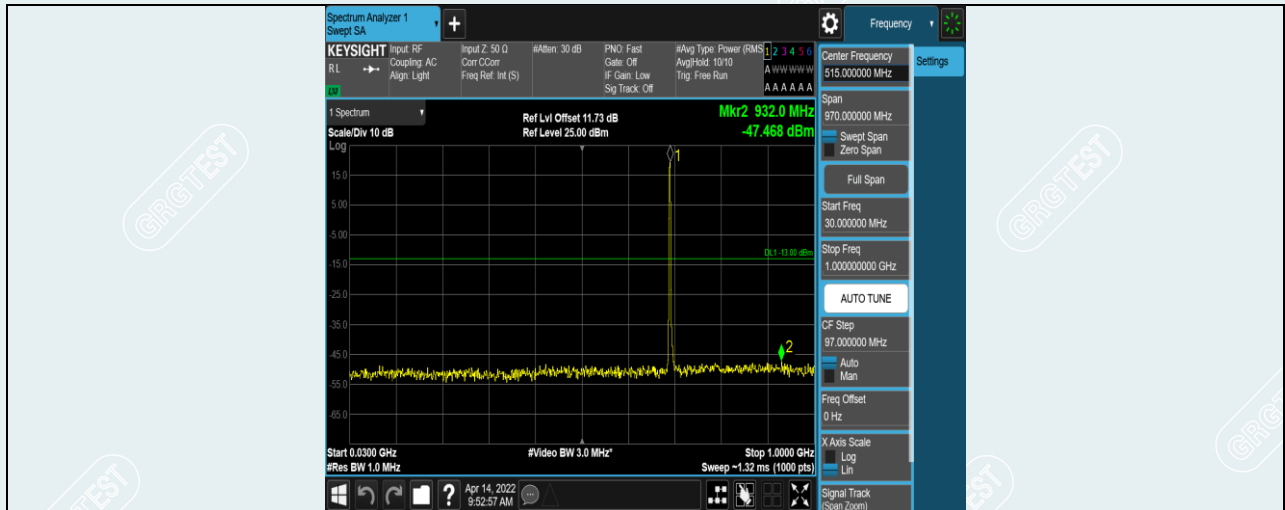
Band12-3MHz-16QAM-23025-1RB#0-Range1:30~1000MHz
