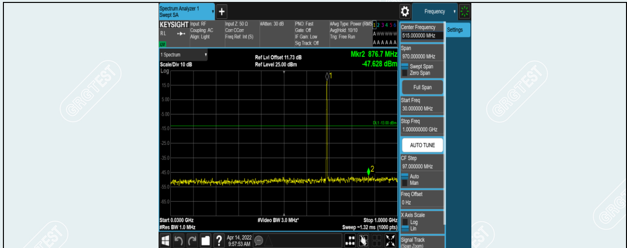
Band12-1.4MHz-16QAM-23017-1RB#0-Range1:30~1000MHz
