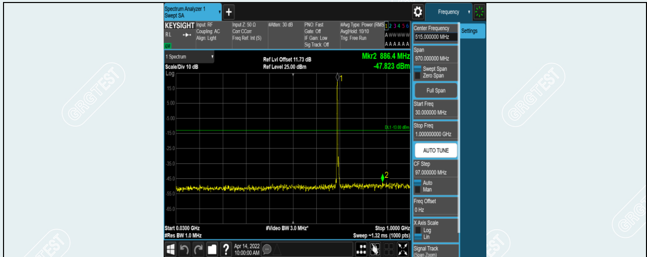
Band12-5MHz-QPSK-23035-1RB#0-Range1:30~1000MHz
