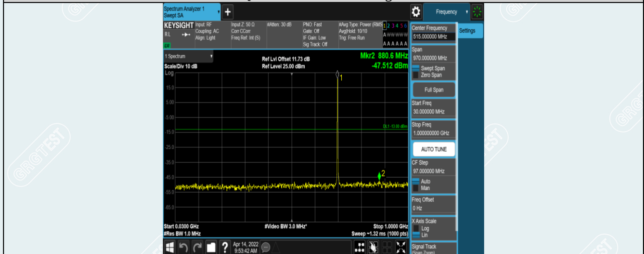
Band12-3MHz-16QAM-23095-1RB#0-Range1:30~1000MHz
