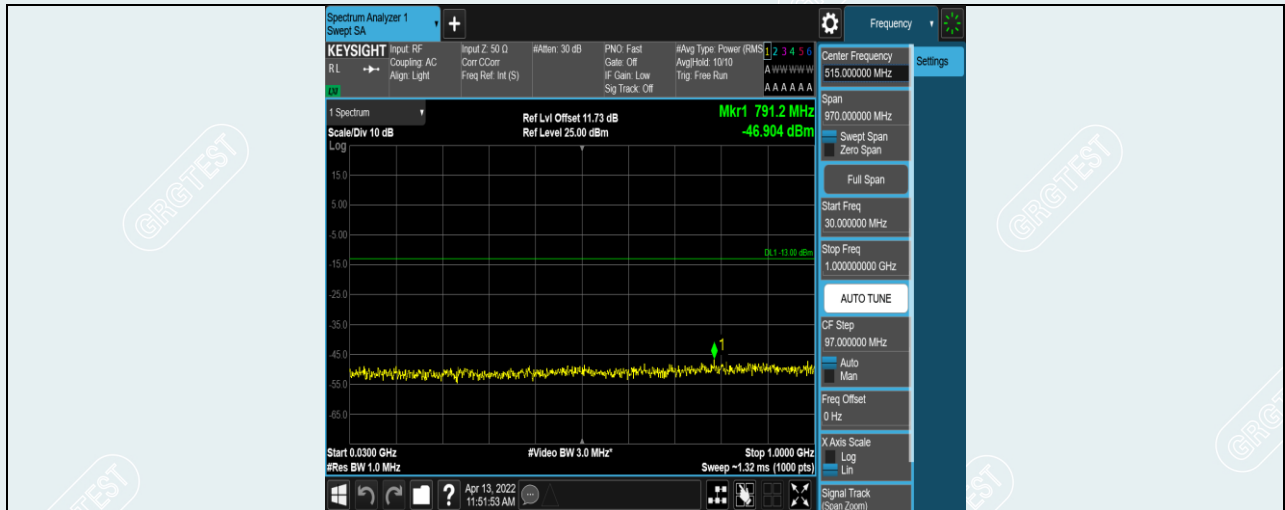
Band7-15MHz-16QAM-20825-1RB#0-Range1:30~1000MHz
