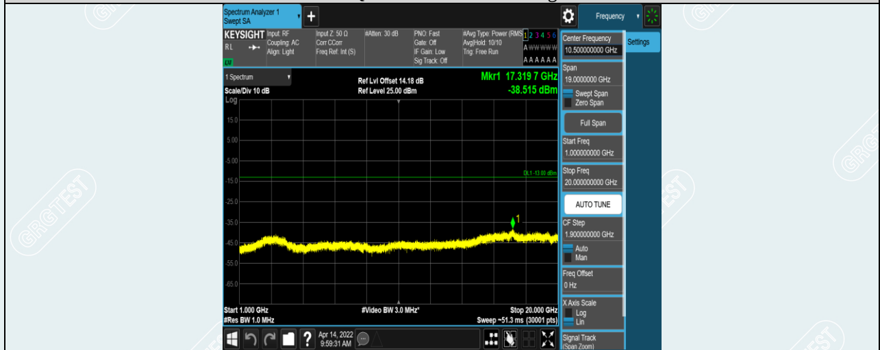
Band12-1.4MHz-16QAM-23173-1RB#0-Range2:1000~20000MHz
