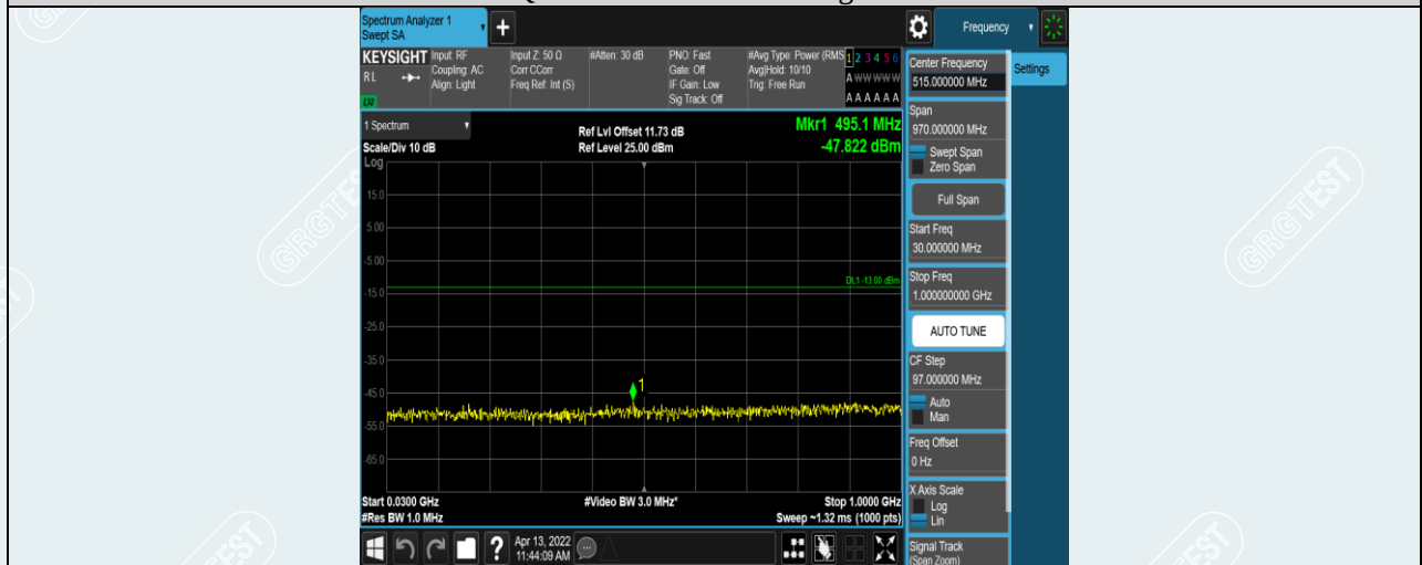
Band7-20MHz-QPSK-21350-1RB#0-Range1:30~1000MHz
