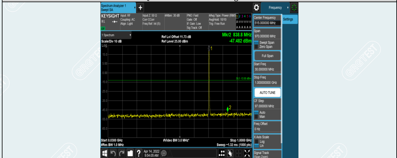
Band12-3MHz-QPSK-23165-1RB#0-Range1:30~1000MHz
