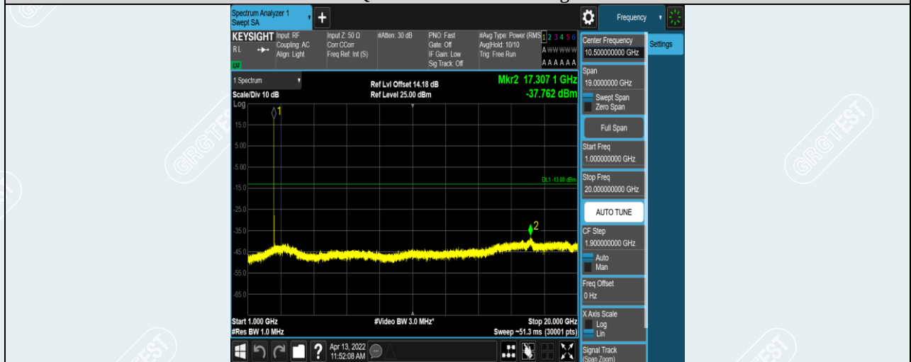
Band7-15MHz-16QAM-20825-1RB#0-Range2:1000~20000MHz
