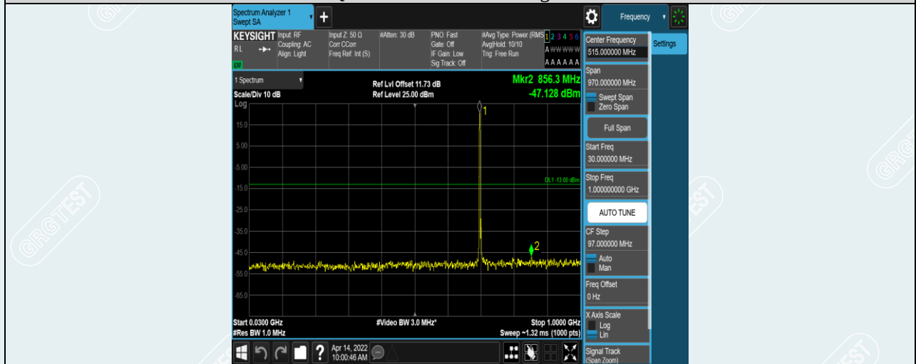
Band12-5MHz-QPSK-23095-1RB#0-Range1:30~1000MHz
