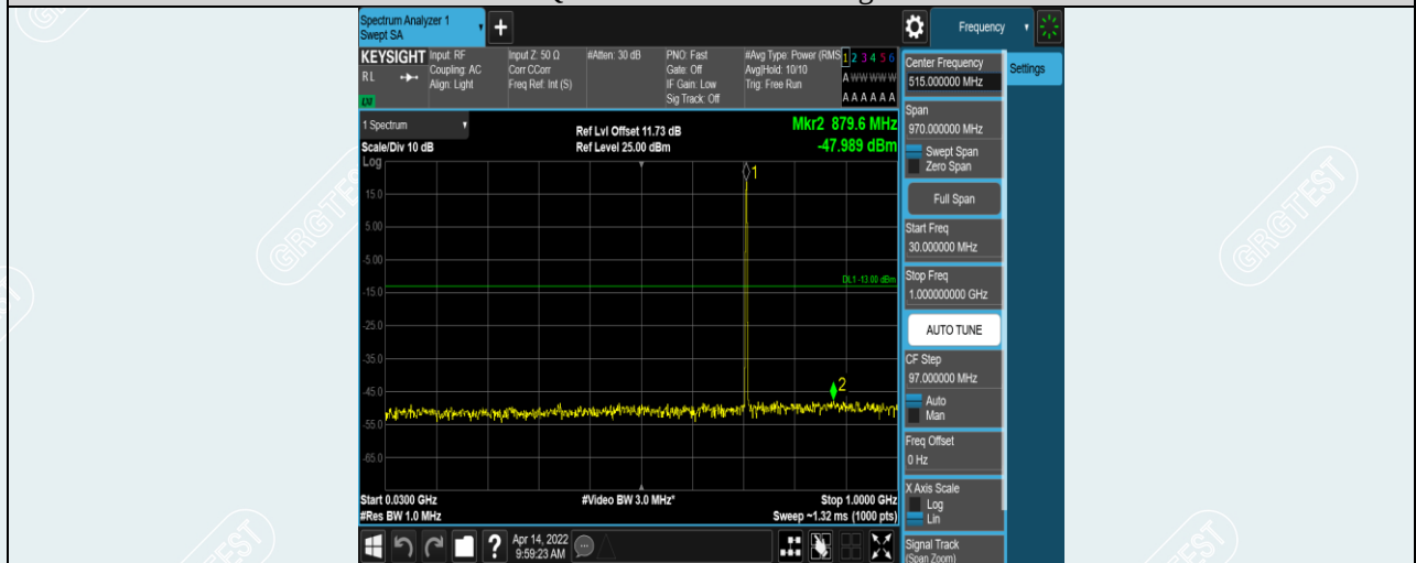
Band12-1.4MHz-16QAM-23173-1RB#0-Range1:30~1000MHz
