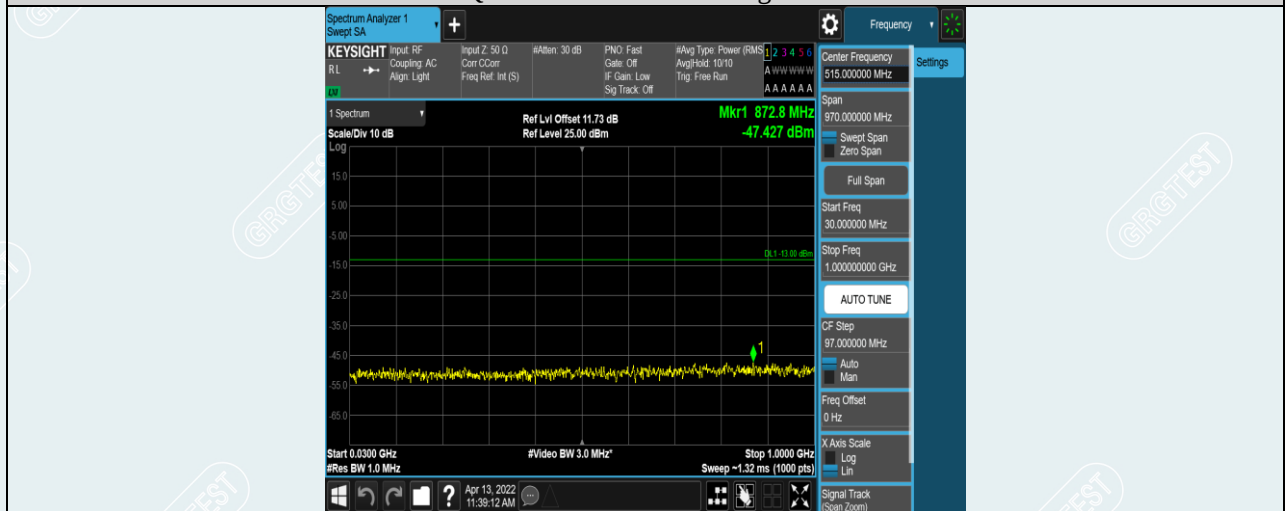
Band7-10MHz-QPSK-21400-1RB#0-Range1:30~1000MHz
