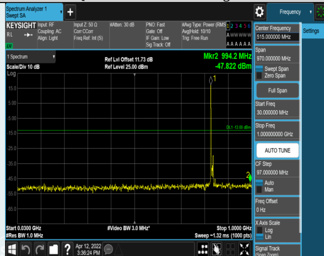
Band5-10MHz-QPSK-20525-1RB#0-Range1:30~1000MHz
