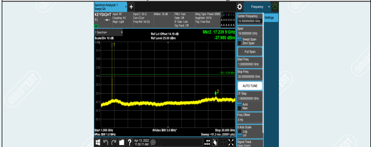
Band7-5MHz-16QAM-21425-1RB#0-Range2:1000~20000MHz
