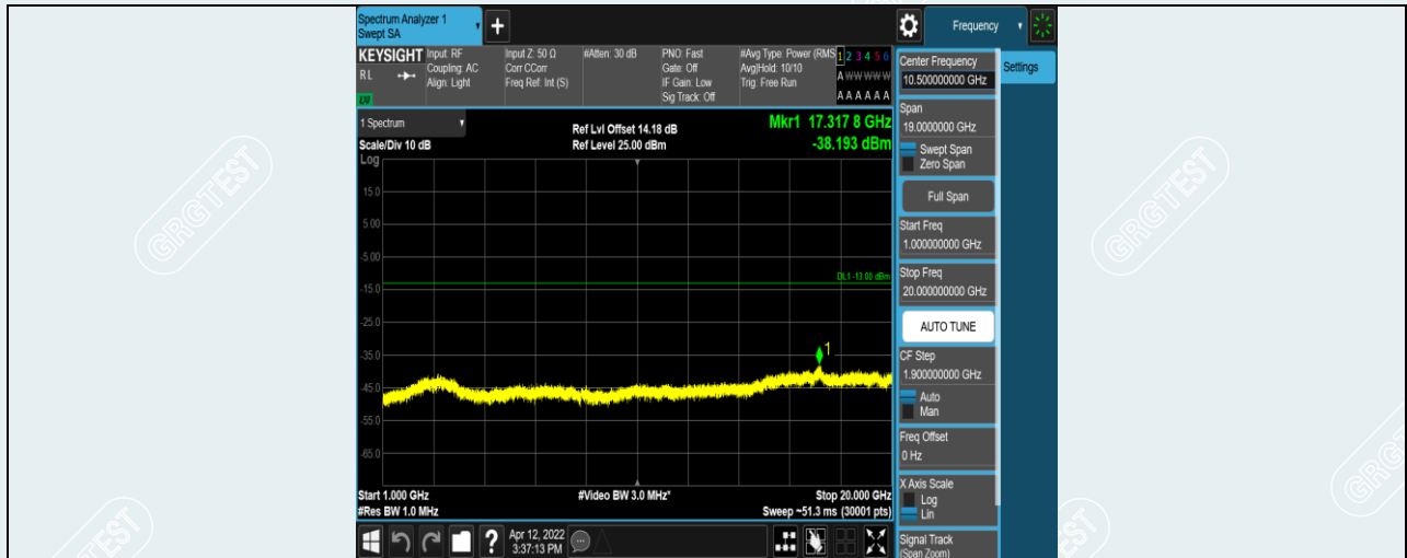
Band5-10MHz-16QAM-20525-1RB#0-Range2:1000~20000MHz
