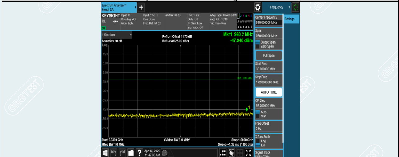
Band7-5MHz-QPSK-21100-1RB#0-Range1:30~1000MHz
