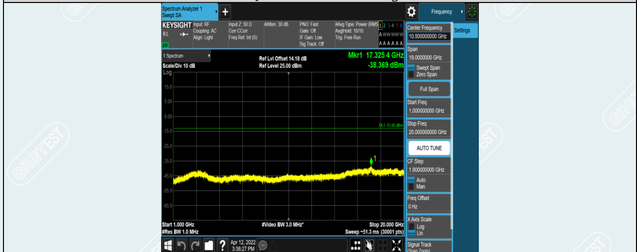
Band5-10MHz-16QAM-20600-1RB#0-Range2:1000~20000MHz
