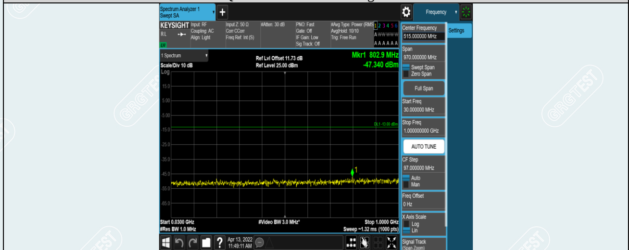
Band7-5MHz-QPSK-21425-1RB#0-Range1:30~1000MHz
