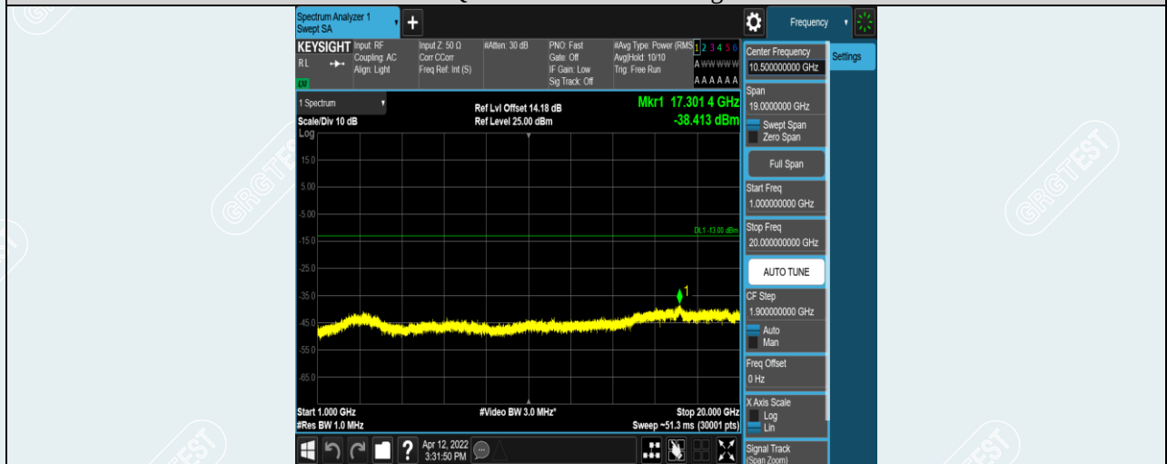
Band5-5MHz-16QAM-20425-1RB#0-Range2:1000~20000MHz
