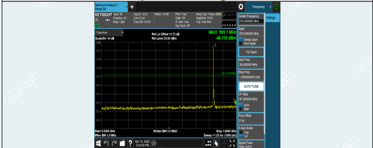
Band5-5MHz-16QAM-20525-1RB#0-Range1:30~1000MHz
