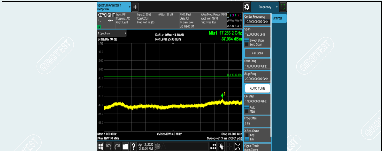
Band5-5MHz-16QAM-20525-1RB#0-Range2:1000~20000MHz
