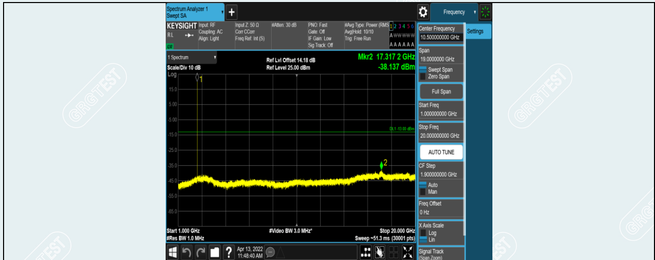
Band7-5MHz-16QAM-21100-1RB#0-Range2:1000~20000MHz
