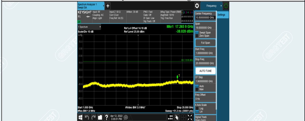
Band5-10MHz-16QAM-20450-1RB#0-Range2:1000~20000MHz
