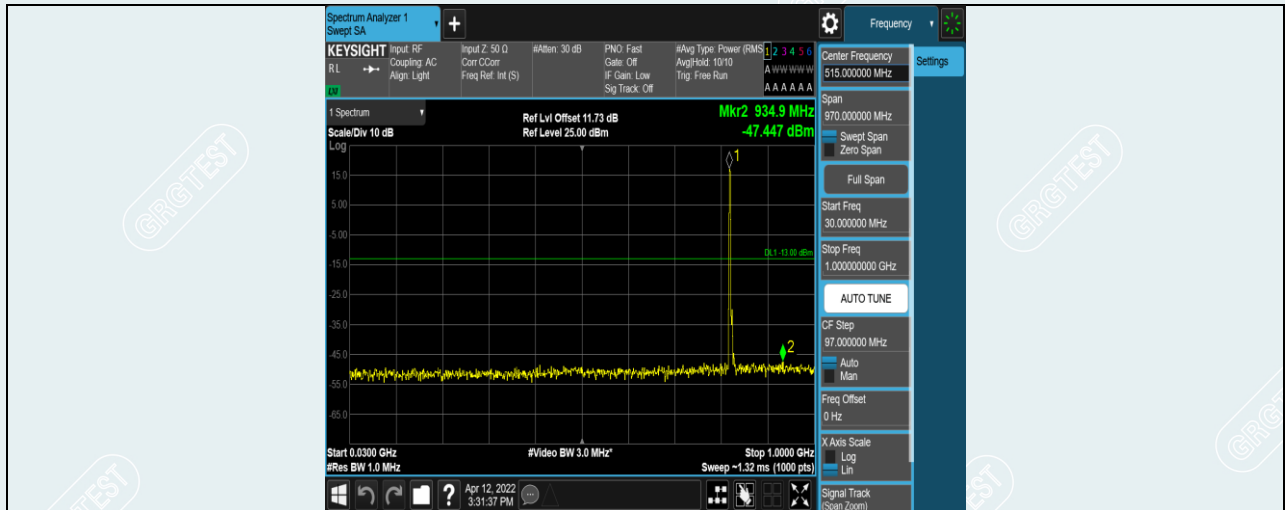
Band5-5MHz-16QAM-20425-1RB#0-Range1:30~1000MHz
