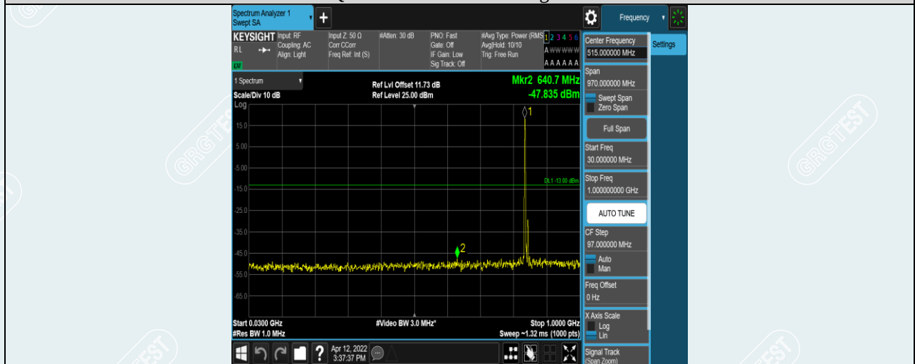
Band5-10MHz-QPSK-20600-1RB#0-Range1:30~1000MHz
