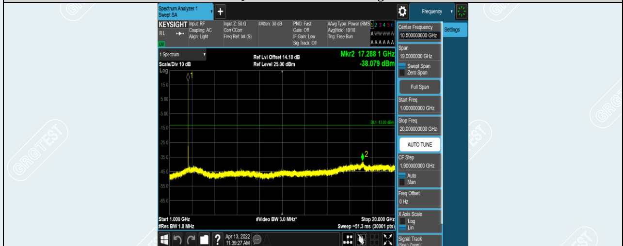
Band7-10MHz-QPSK-21400-1RB#0-Range2:1000~20000MHz
