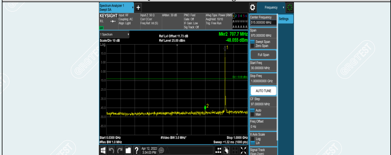
Band5-5MHz-16QAM-20625-1RB#0-Range1:30~1000MHz
