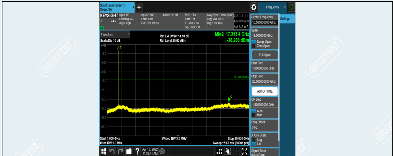
Band7-10MHz-16QAM-21100-1RB#0-Range2:1000~20000MHz
