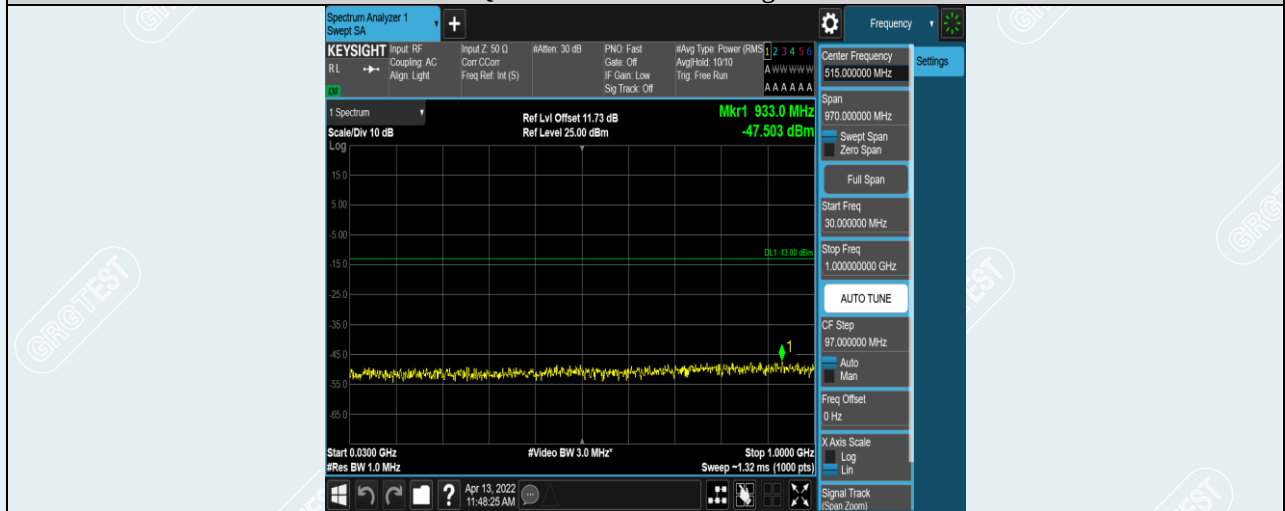
Band7-5MHz-16QAM-21100-1RB#0-Range1:30~1000MHz
