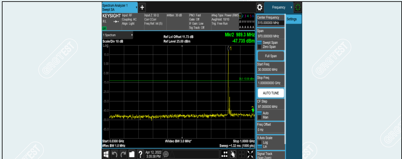
Band5-10MHz-16QAM-20450-1RB#0-Range1:30~1000MHz
