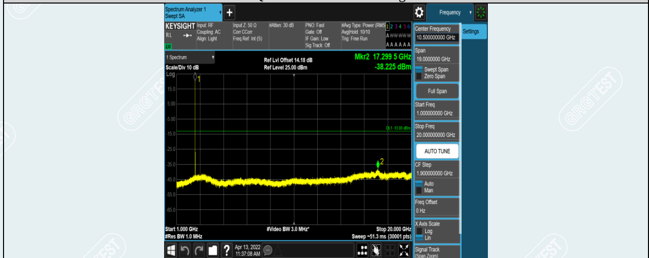
Band7-10MHz-16QAM-20800-1RB#0-Range2:1000~20000MHz
