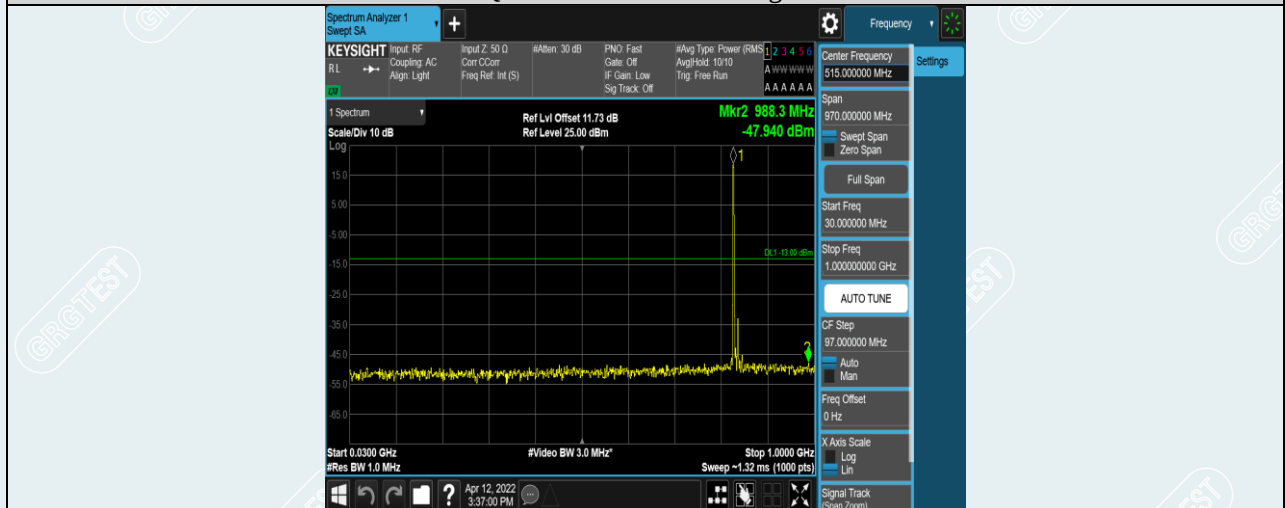
Band5-10MHz-16QAM-20525-1RB#0-Range1:30~1000MHz
