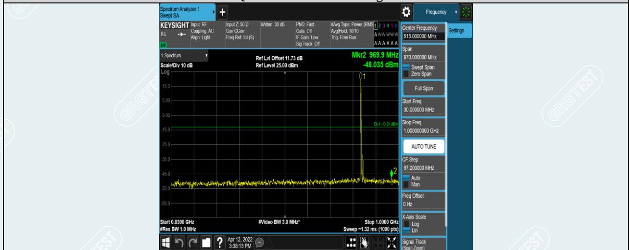
Band5-10MHz-16QAM-20600-1RB#0-Range1:30~1000MHz
