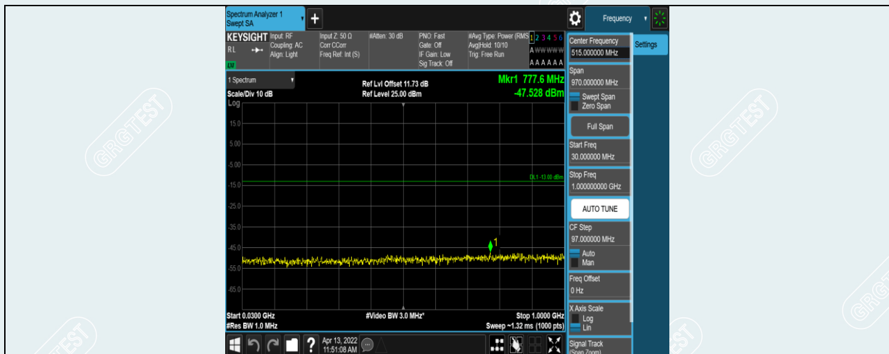
Band7-15MHz-QPSK-20825-1RB#0-Range1:30~1000MHz
