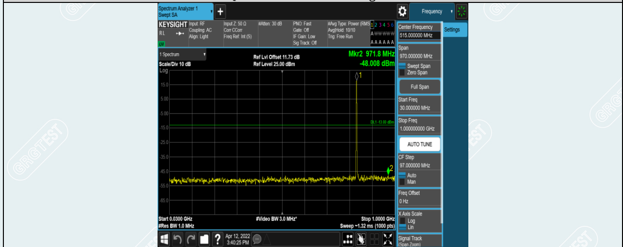
Band5-1.4MHz-QPSK-20525-1RB#0-Range1:30~1000MHz
