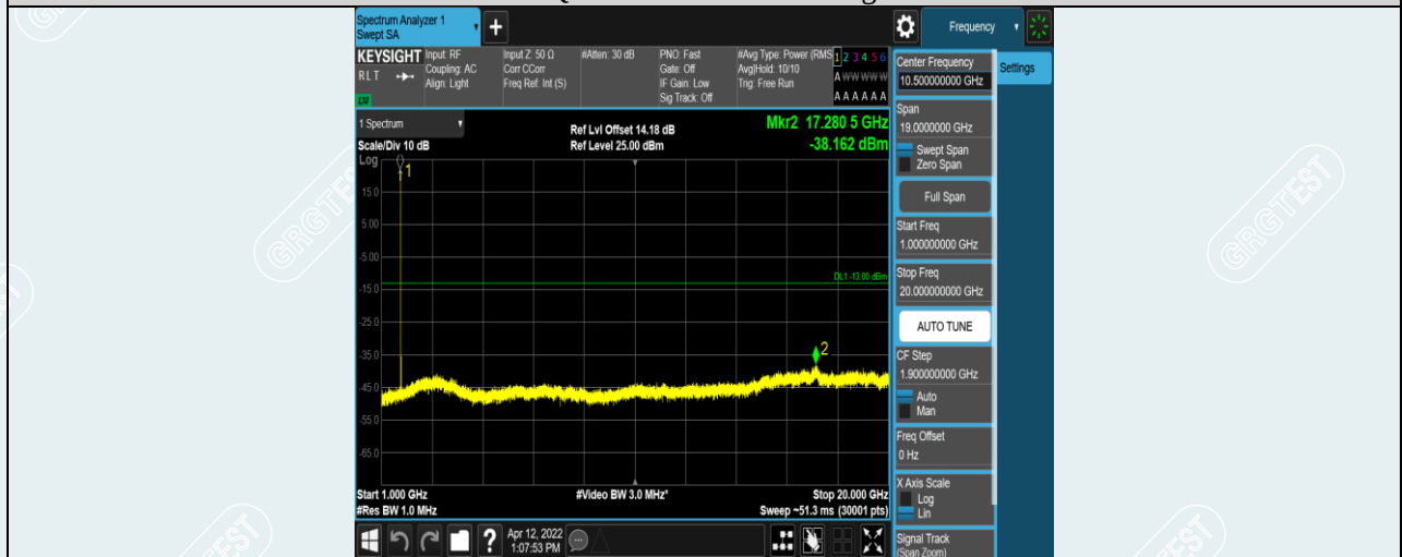
Band4-15MHz-16QAM-20025-1RB#0-Range2:1000~20000MHz
