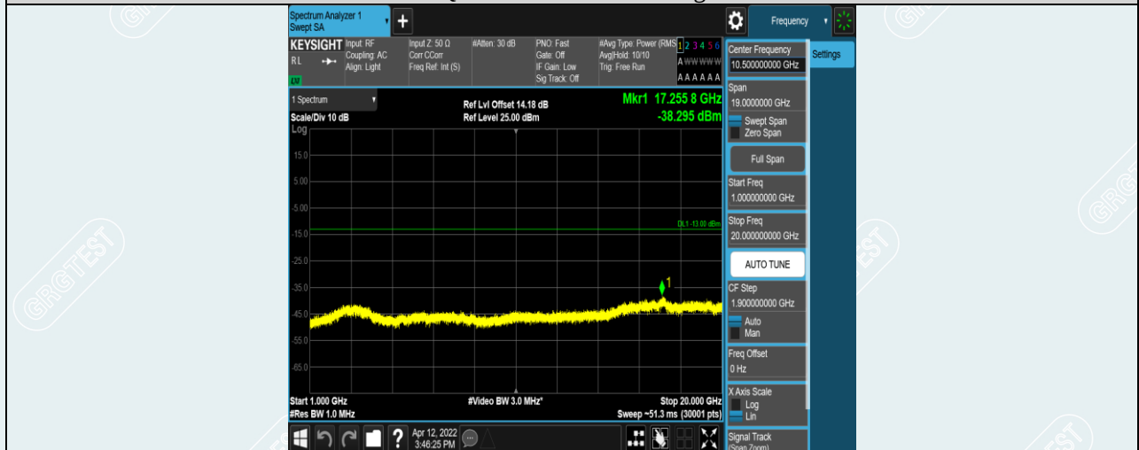
Band5-3MHz-16QAM-20635-1RB#0-Range2:1000~20000MHz
