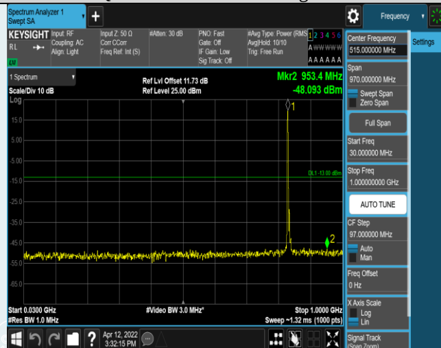
Band5-5MHz-QPSK-20525-1RB#0-Range1:30~1000MHz
