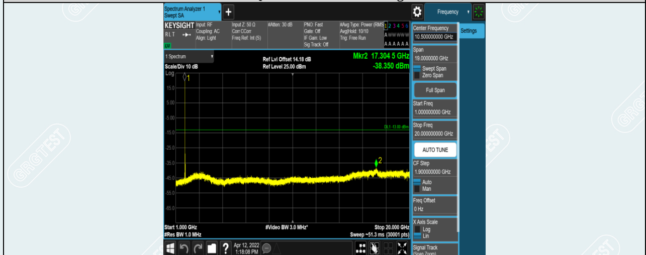
Band4-20MHz-16QAM-20300-1RB#0-Range2:1000~20000MHz
