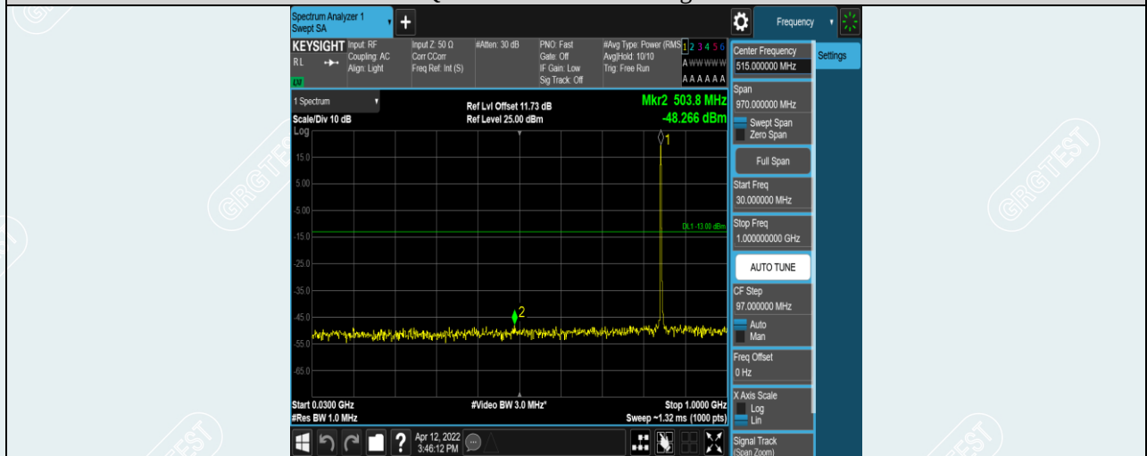
Band5-3MHz-16QAM-20635-1RB#0-Range1:30~1000MHz
