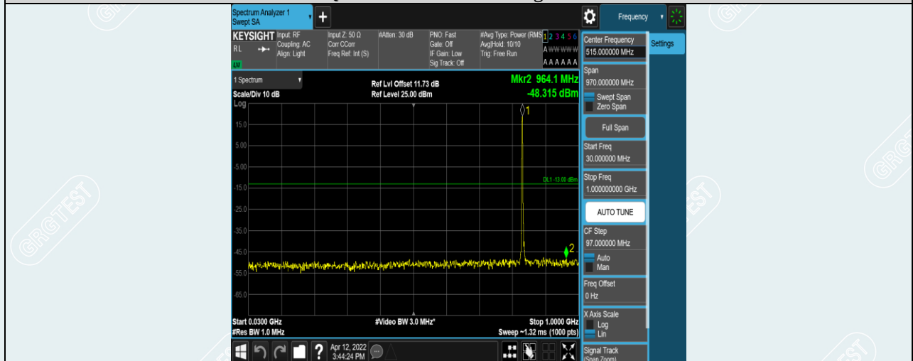
Band5-3MHz-QPSK-20525-1RB#0-Range1:30~1000MHz
