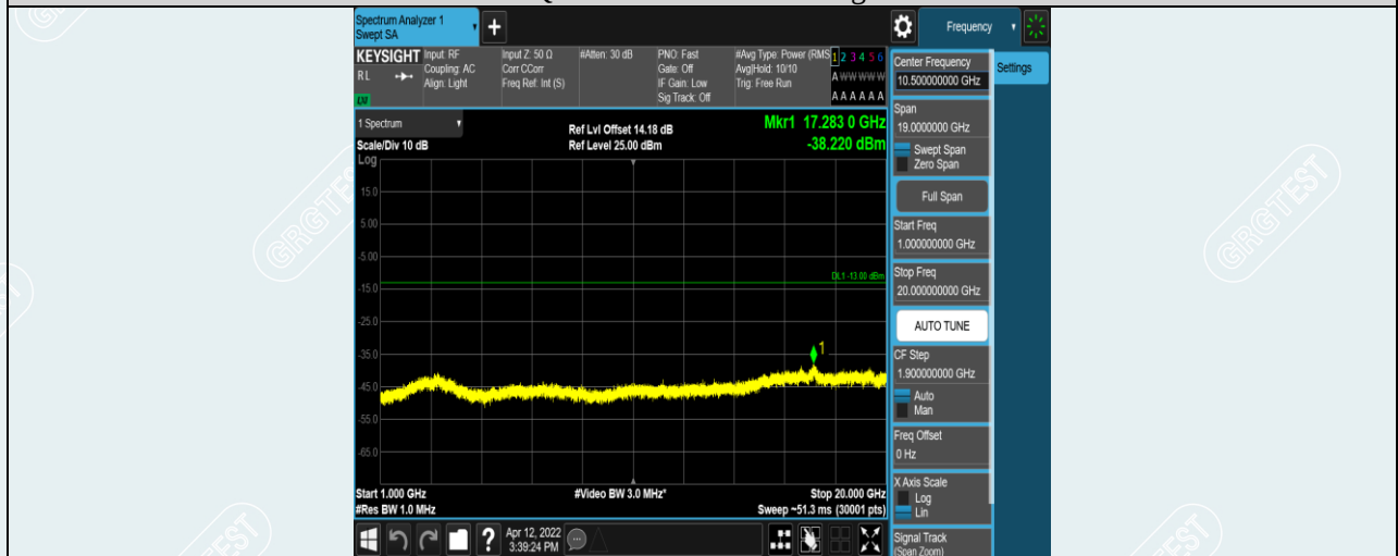
Band5-1.4MHz-QPSK-20407-1RB#0-Range2:1000~20000MHz
