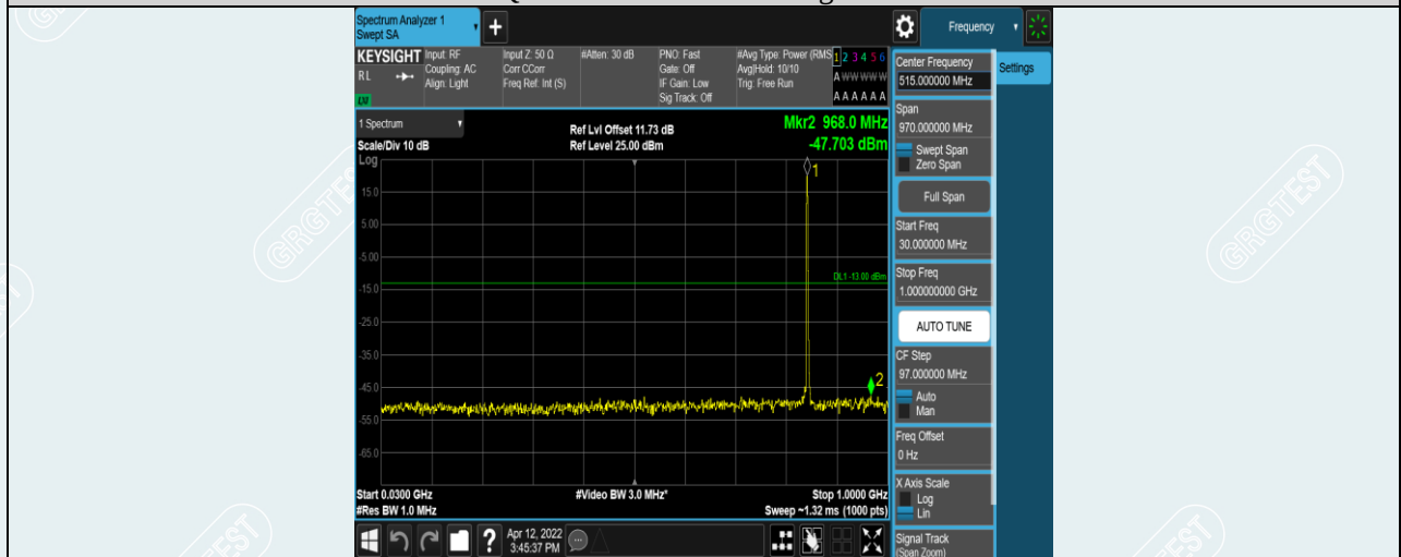
Band5-3MHz-QPSK-20635-1RB#0-Range1:30~1000MHz
