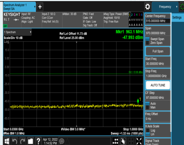
Band4-20MHz-QPSK-20050-1RB#0-Range1:30~1000MHz
