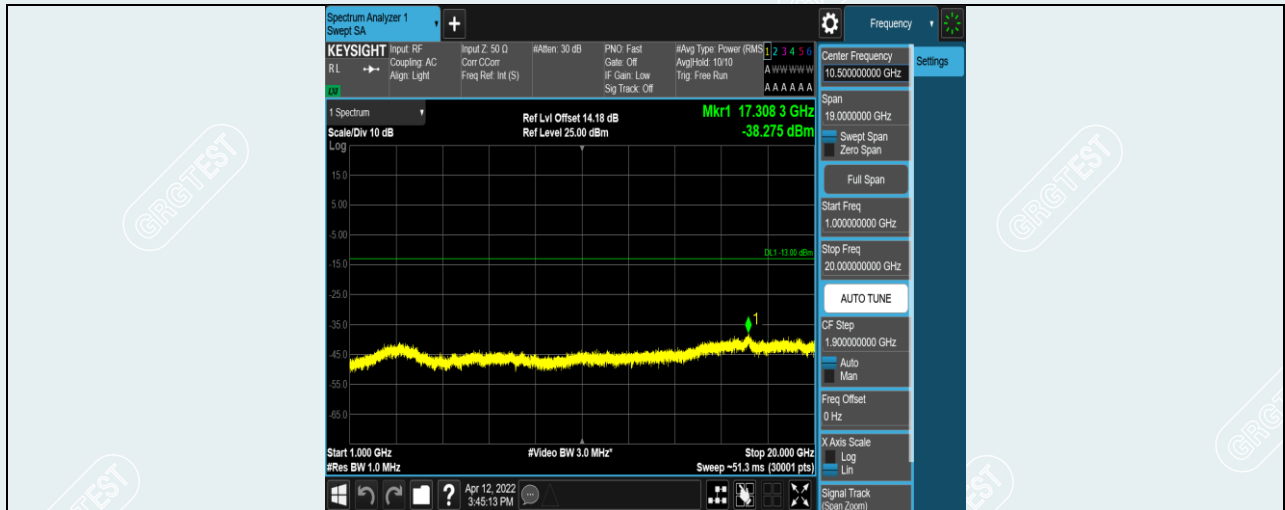
Band5-3MHz-16QAM-20525-1RB#0-Range2:1000~20000MHz
