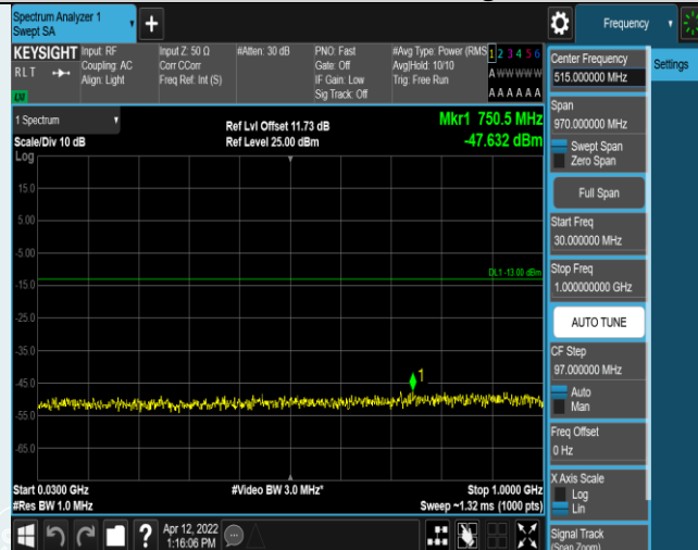
Band4-20MHz-QPSK-20175-1RB#0-Range1:30~1000MHz
