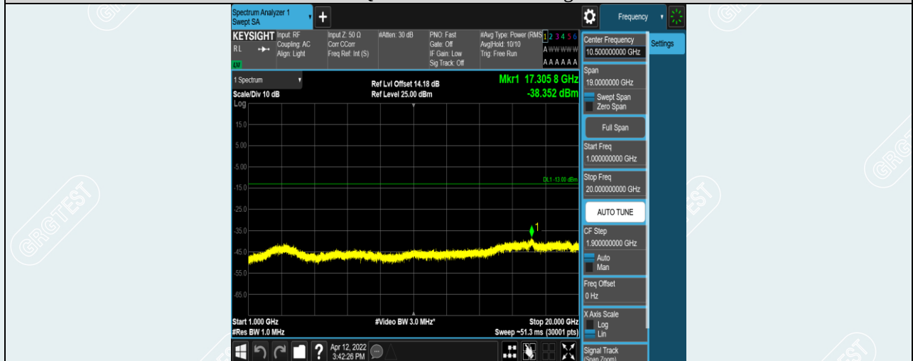
Band5-1.4MHz-16QAM-20643-1RB#0-Range2:1000~20000MHz
