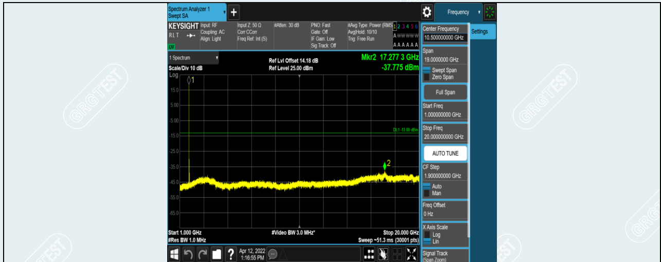
Band4-20MHz-16QAM-20175-1RB#0-Range2:1000~20000MHz
