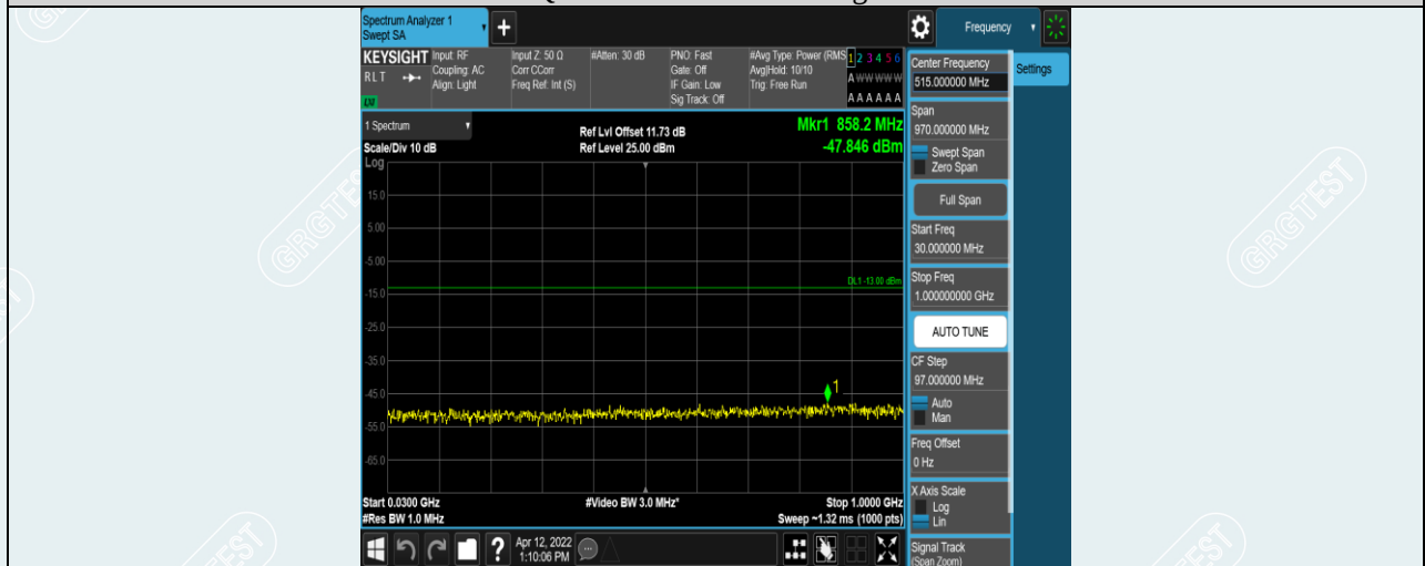
Band4-15MHz-16QAM-20325-1RB#0-Range1:30~1000MHz
