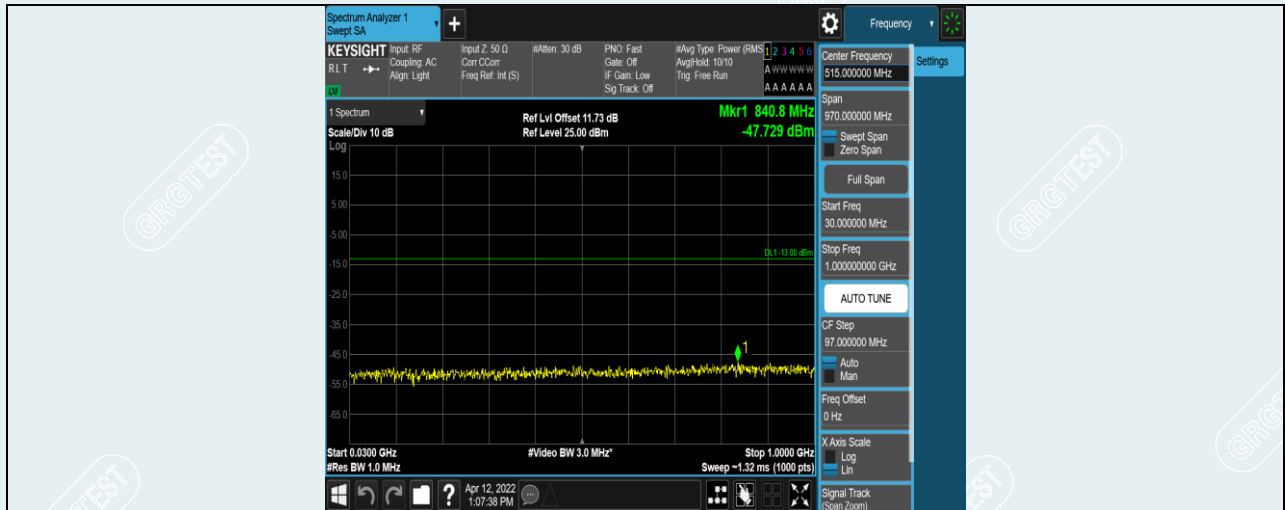
Band4-15MHz-16QAM-20025-1RB#0-Range1:30~1000MHz
