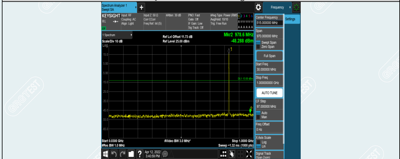
Band5-1.4MHz-16QAM-20525-1RB#0-Range1:30~1000MHz
