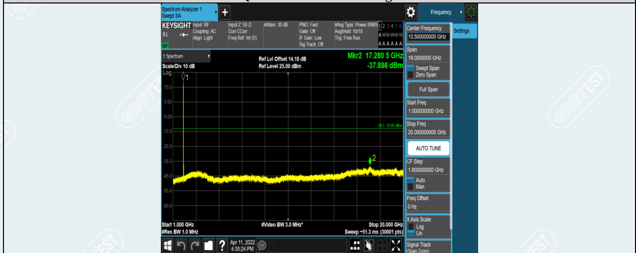
Band2-15MHz-QPSK-18675-1RB#0-Range2:1000~20000MHz
