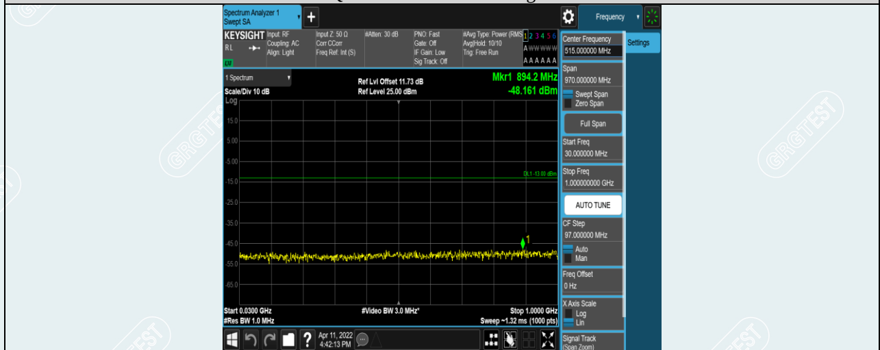
Band2-10MHz-16QAM-19150-1RB#0-Range1:30~1000MHz
