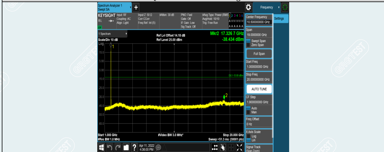
Band2-15MHz-16QAM-18675-1RB#0-Range2:1000~20000MHz
