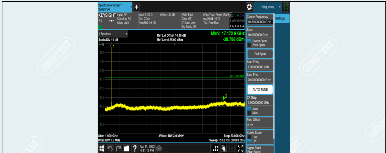
Band2-10MHz-16QAM-18900-1RB#0-Range2:1000~20000MHz
