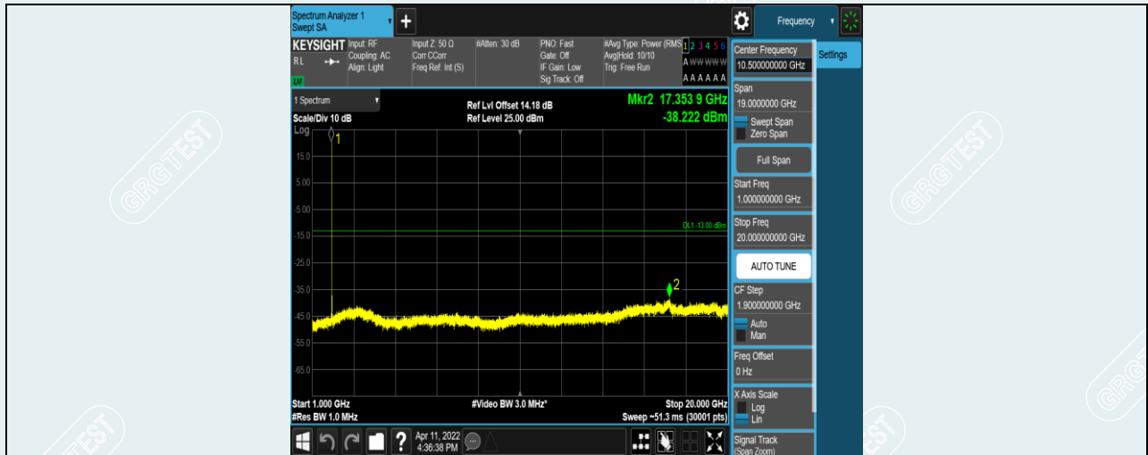
Band2-15MHz-QPSK-18900-1RB#0-Range2:1000~20000MHz
