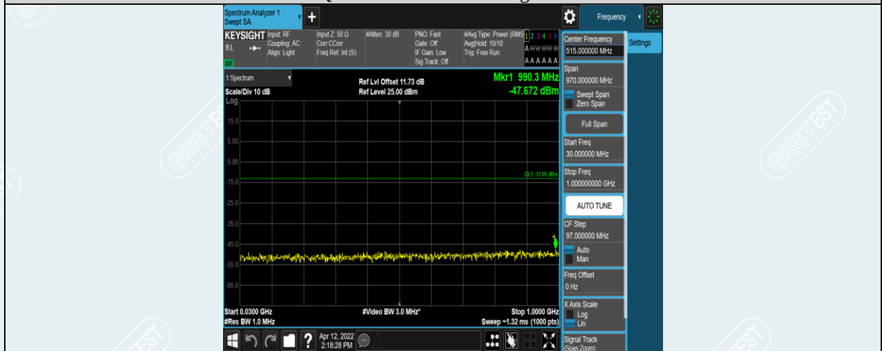
Band2-20MHz-QPSK-19100-1RB#0-Range1:30~1000MHz
