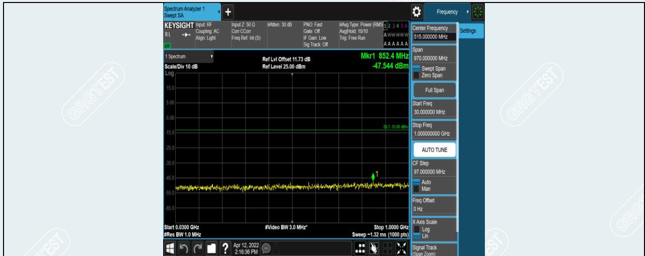
Band2-20MHz-16QAM-18700-1RB#0-Range1:30~1000MHz
