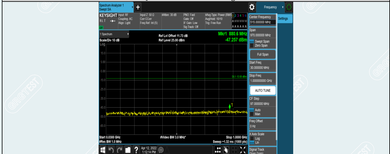
Band4-1.4MHz-QPSK-20175-1RB#0-Range1:30~1000MHz
