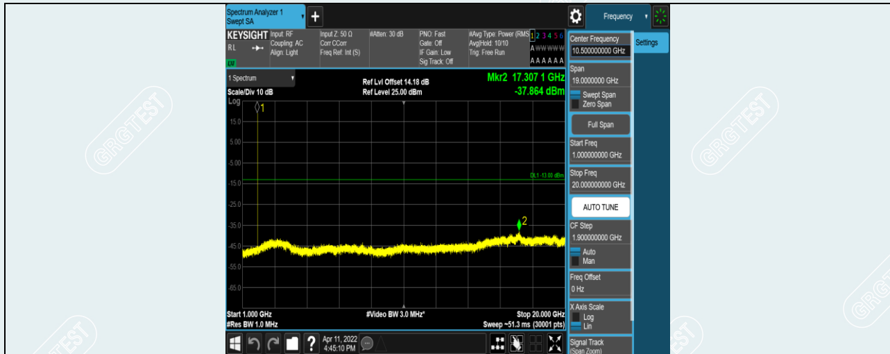
Band2-5MHz-16QAM-18900-1RB#0-Range2:1000~20000MHz
