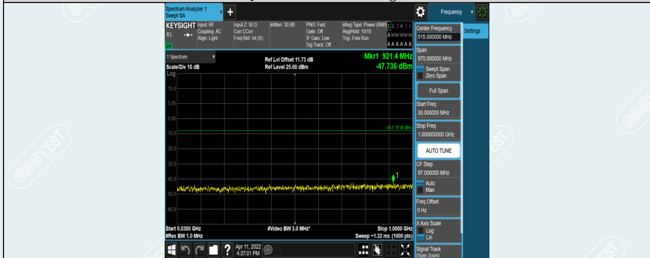
Band2-15MHz-16QAM-18900-1RB#0-Range1:30~1000MHz
