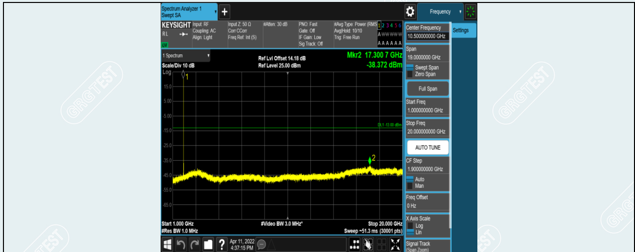
Band2-15MHz-16QAM-18900-1RB#0-Range2:1000~20000MHz
