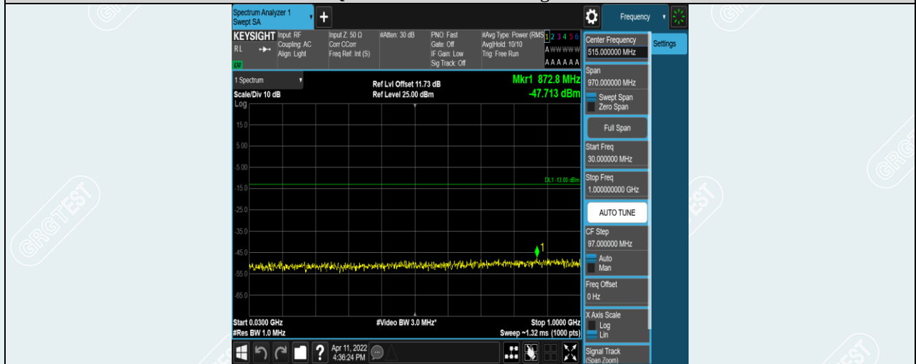
Band2-15MHz-QPSK-18900-1RB#0-Range1:30~1000MHz
