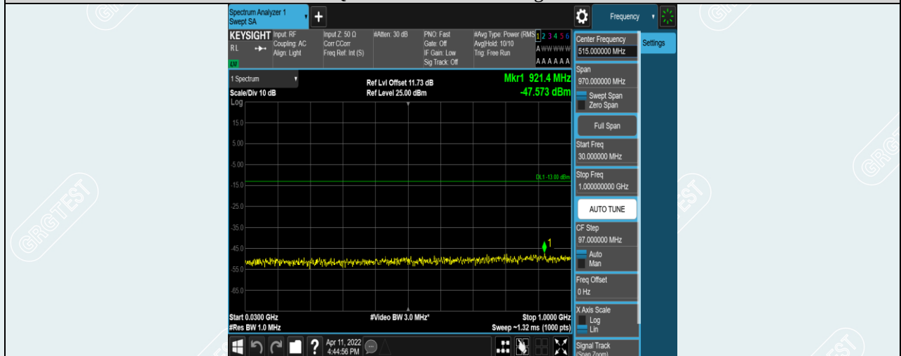
Band2-5MHz-16QAM-18900-1RB#0-Range1:30~1000MHz
