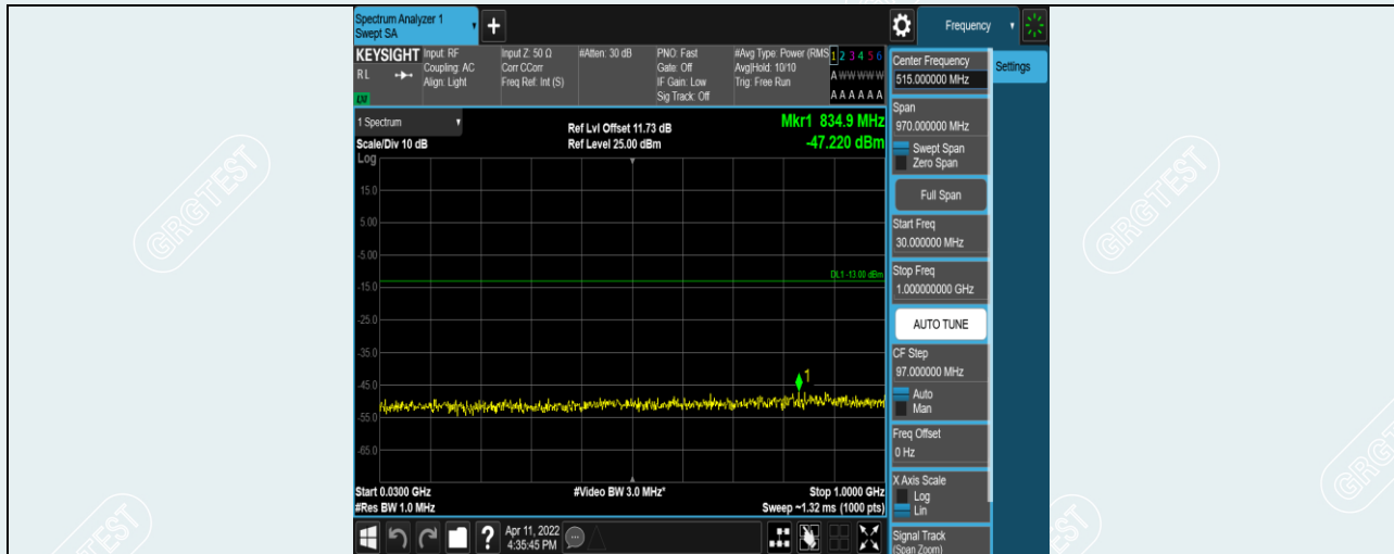
Band2-15MHz-16QAM-18675-1RB#0-Range1:30~1000MHz
