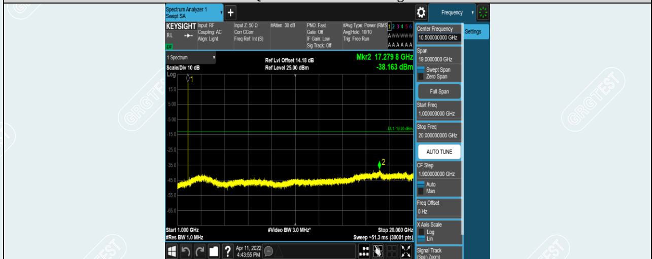
Band2-5MHz-16QAM-18625-1RB#0-Range2:1000~20000MHz
