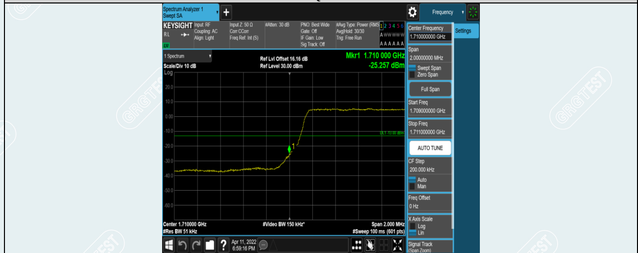
Band4-3MHz-16QAM-19965-15RB#0
