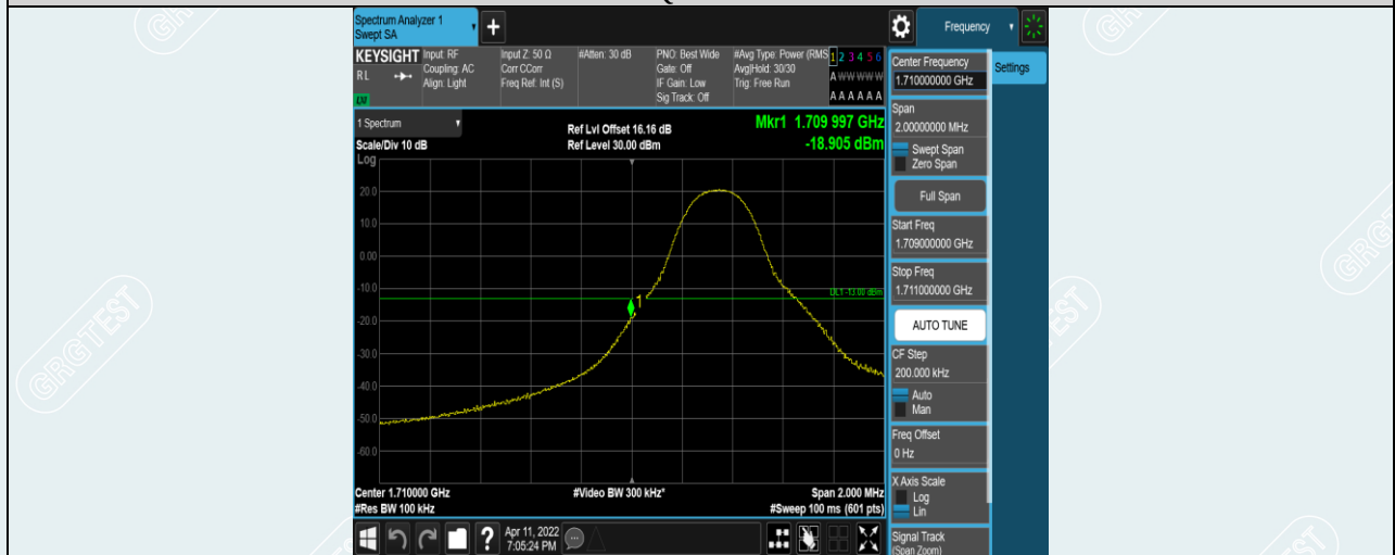
Band4-5MHz-16QAM-19975-1RB#0
