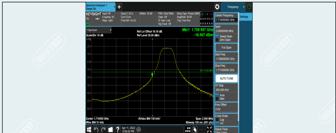
Band4-3MHz-16QAM-19965-1RB#0
