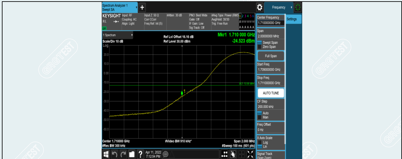
Band4-15MHz-16QAM-20025-1RB#0
