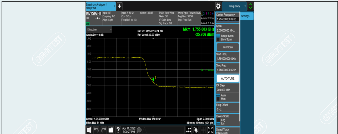
Band4-3MHz-16QAM-20385-15RB#0
