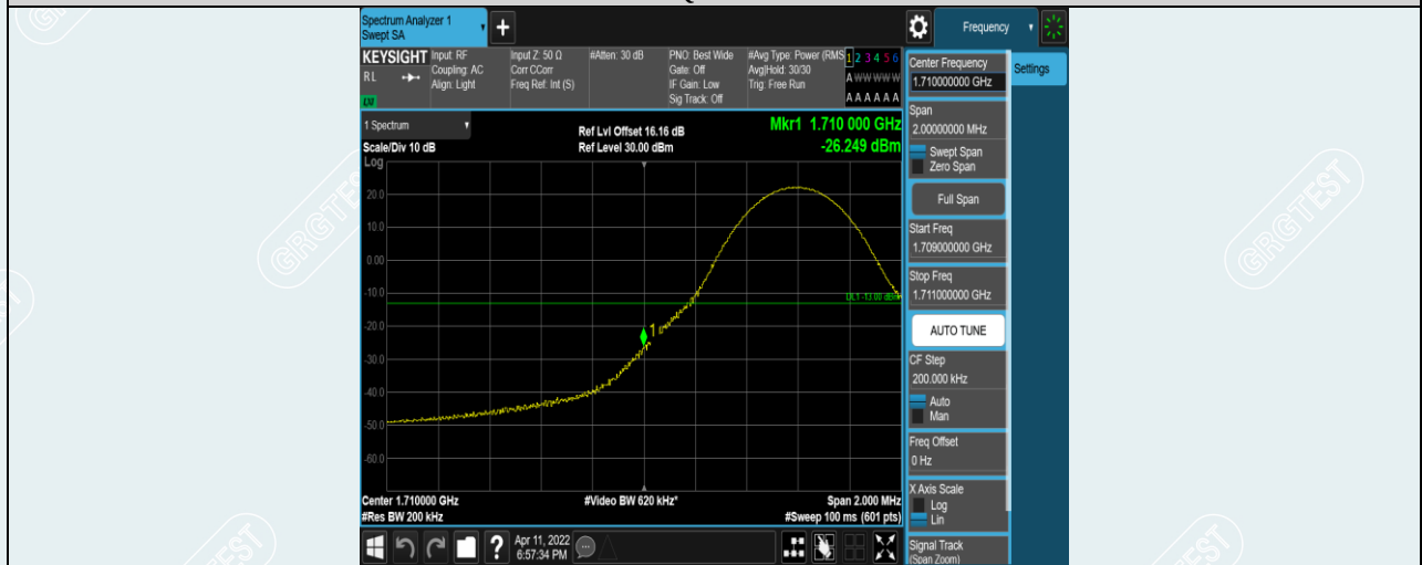
Band4-10MHz-16QAM-20000-1RB#0
