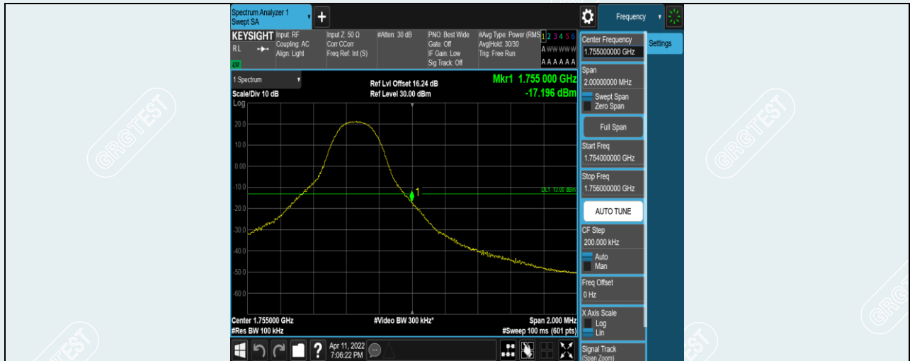
Band4-5MHz-QPSK-20375-1RB#24
