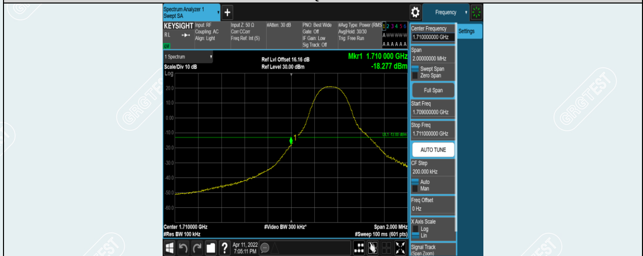
Band4-5MHz-QPSK-19975-1RB#0
