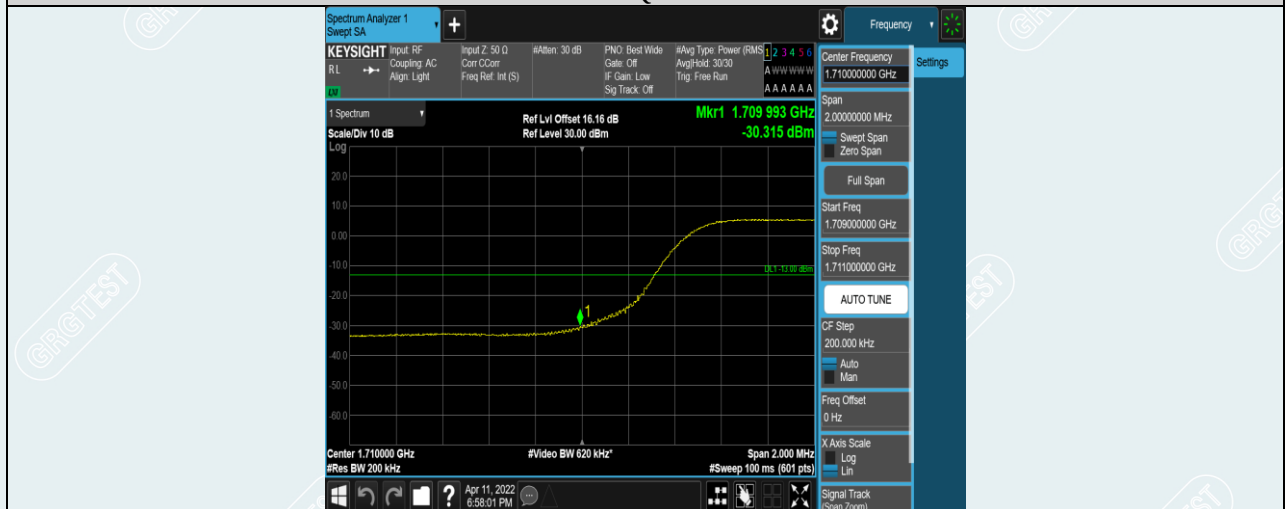
Band4-10MHz-16QAM-20000-50RB#0
