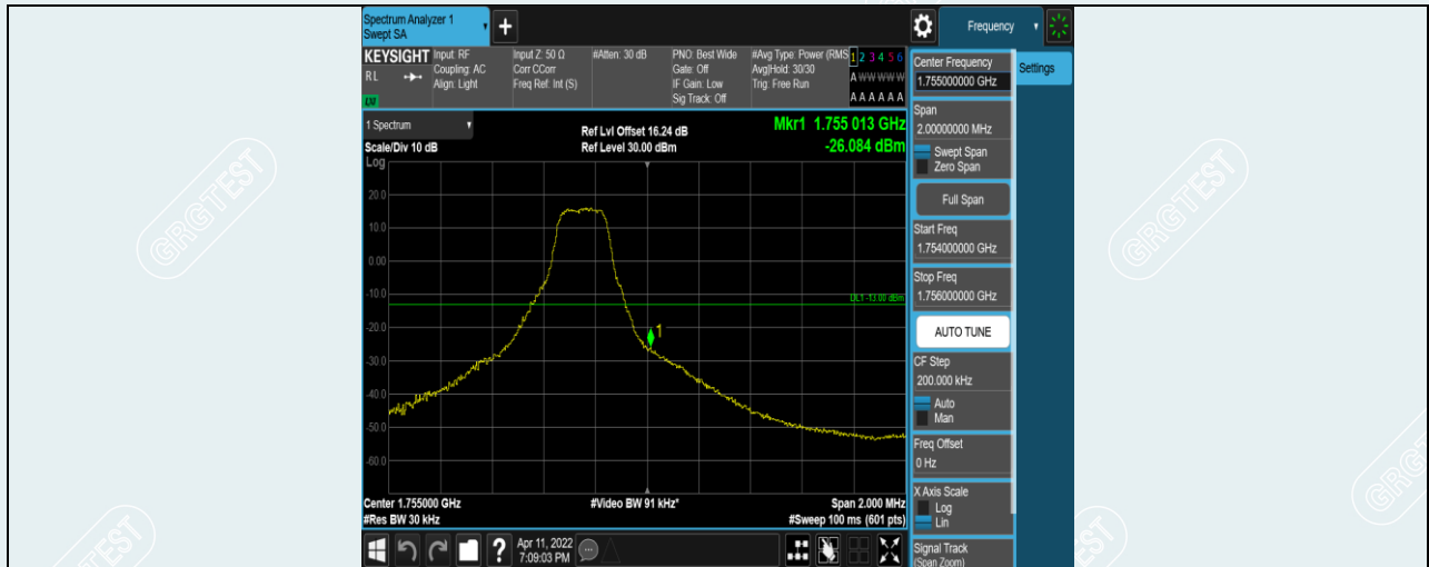
Band4-1.4MHz-16QAM-20393-1RB#5
