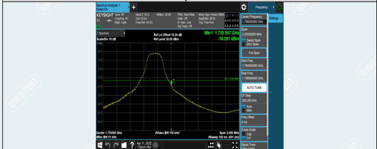
Band4-3MHz-16QAM-20385-1RB#14
