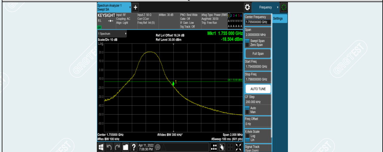
Band4-5MHz-16QAM-20375-1RB#24
