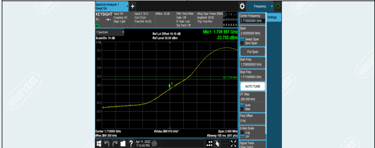
Band4-15MHz-QPSK-20025-1RB#0
