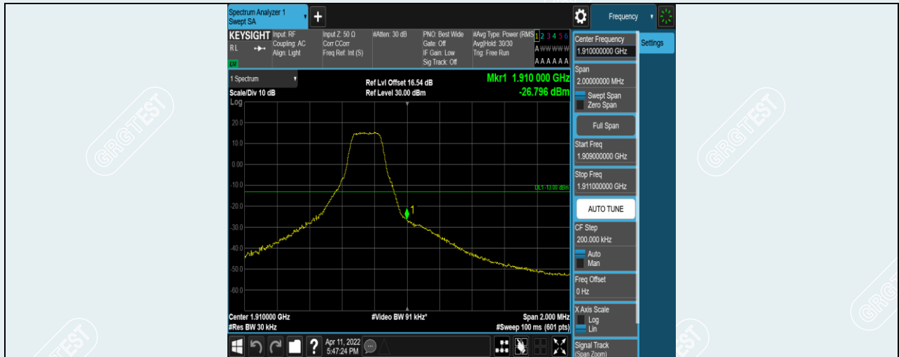
Band2-1.4MHz-16QAM-19193-1RB#5
