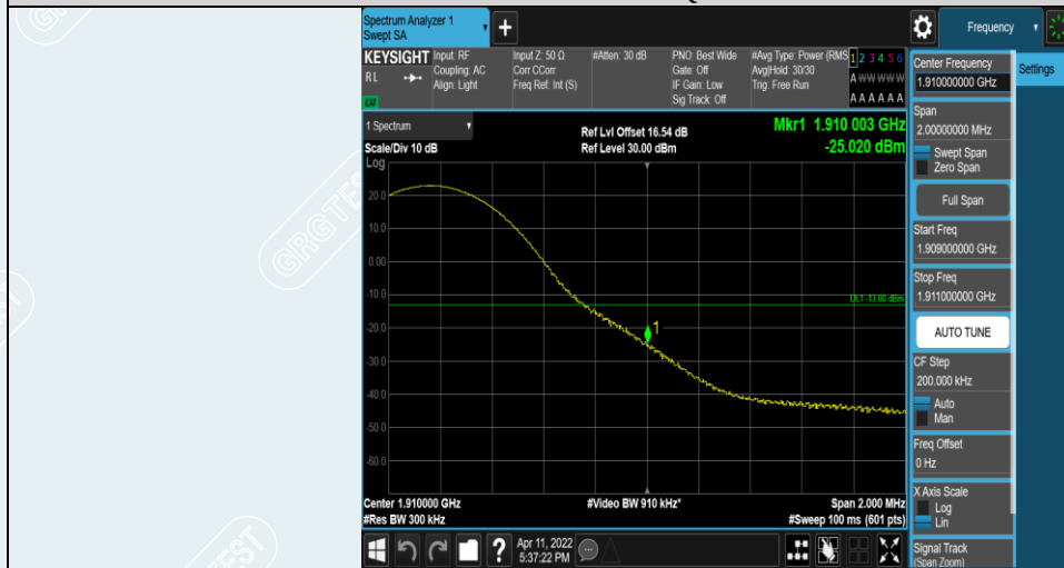
Band2-15MHz-QPSK-19125-1RB#74
