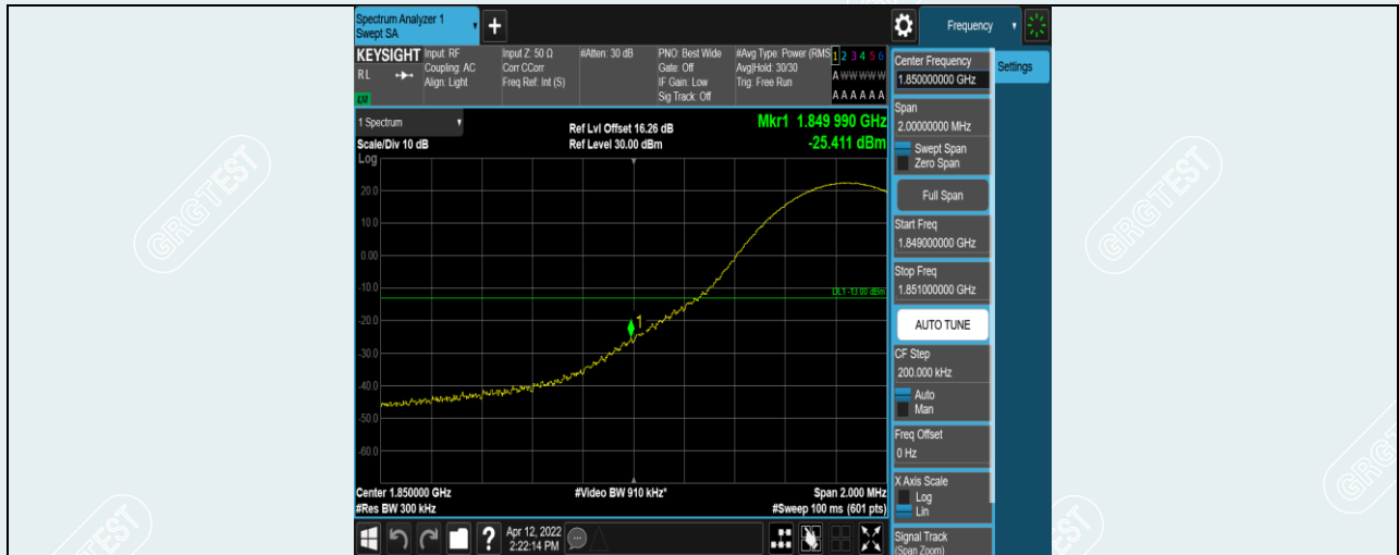
Band2-15MHz-16QAM-18675-1RB#0
