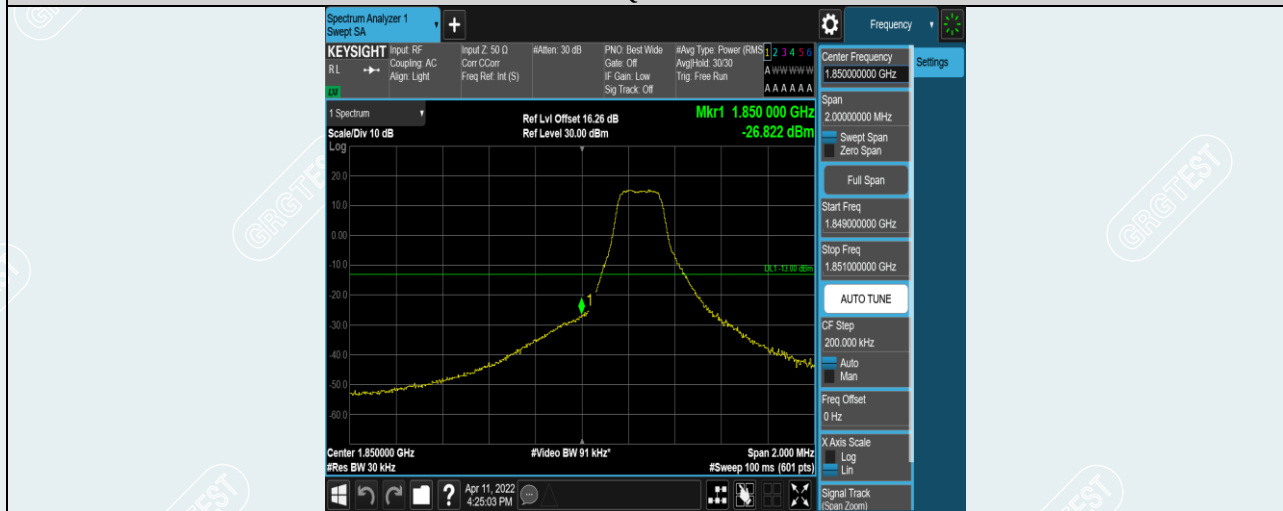
Band2-1.4MHz-16QAM-18607-1RB#0
