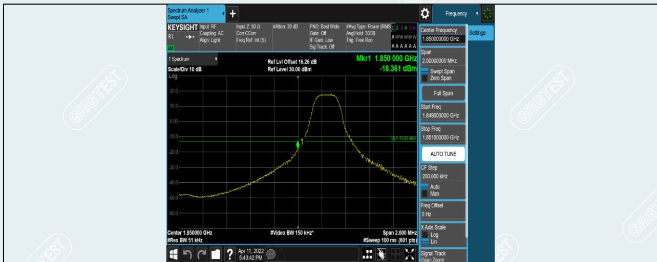
Band2-3MHz-16QAM-18615-1RB#0
