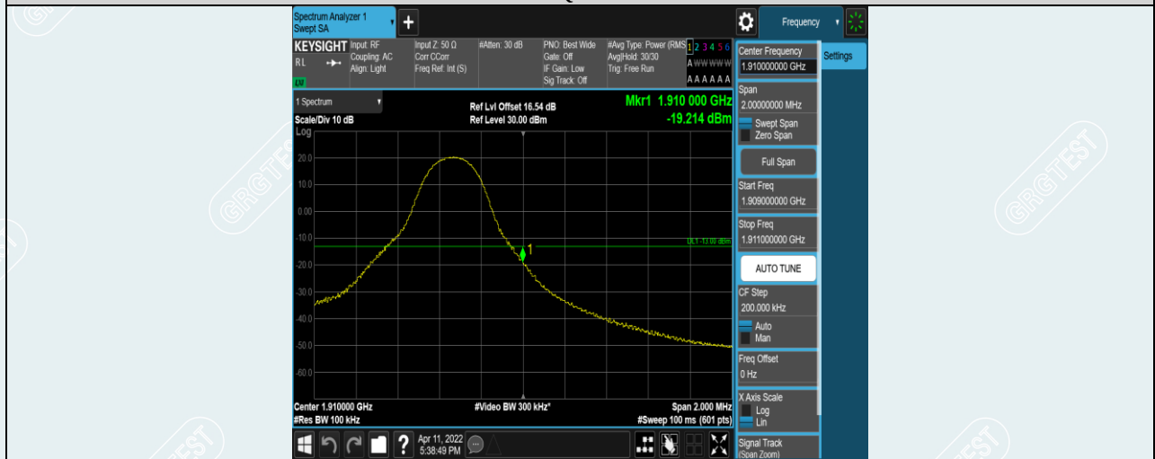
Band2-5MHz-16QAM-19175-1RB#24
