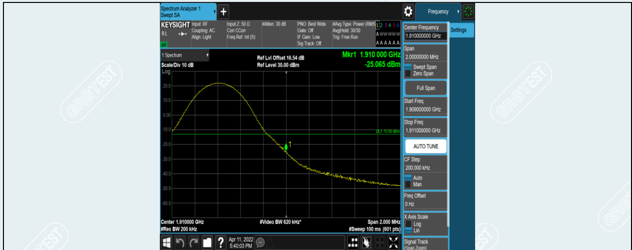
Band2-10MHz-16QAM-19150-1RB#49
