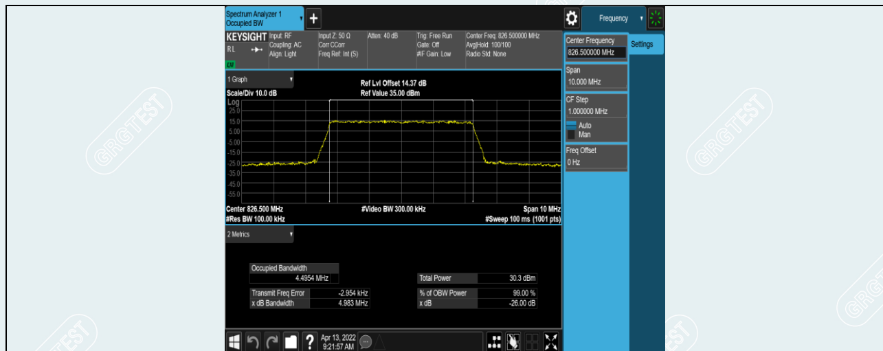
Band5-5MHz-16QAM-20425-25RB#0
