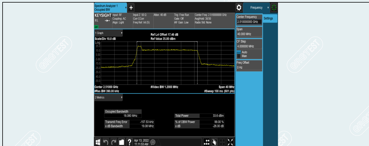
Band7-20MHz-QPSK-20850-100RB#0
