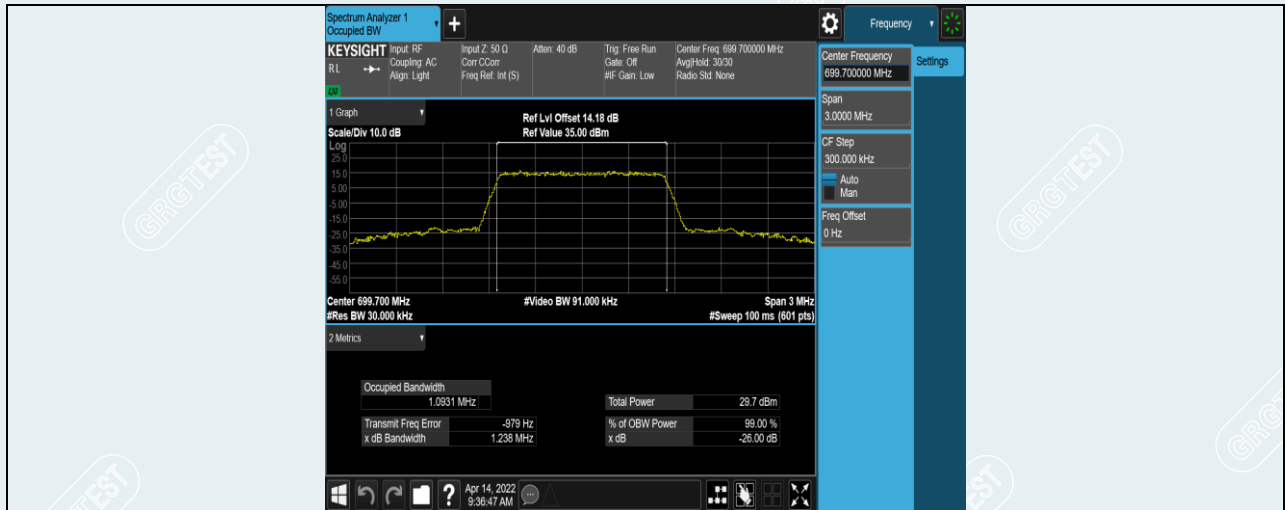
Band12-1.4MHz-16QAM-23017-6RB#0
