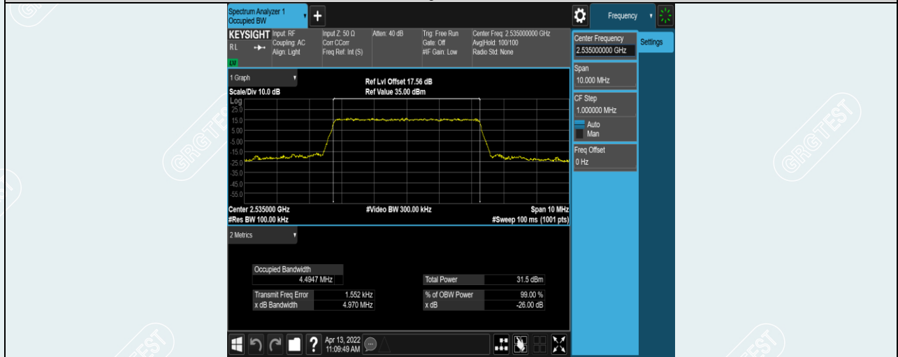
Band7-5MHz-QPSK-21100-25RB#0
