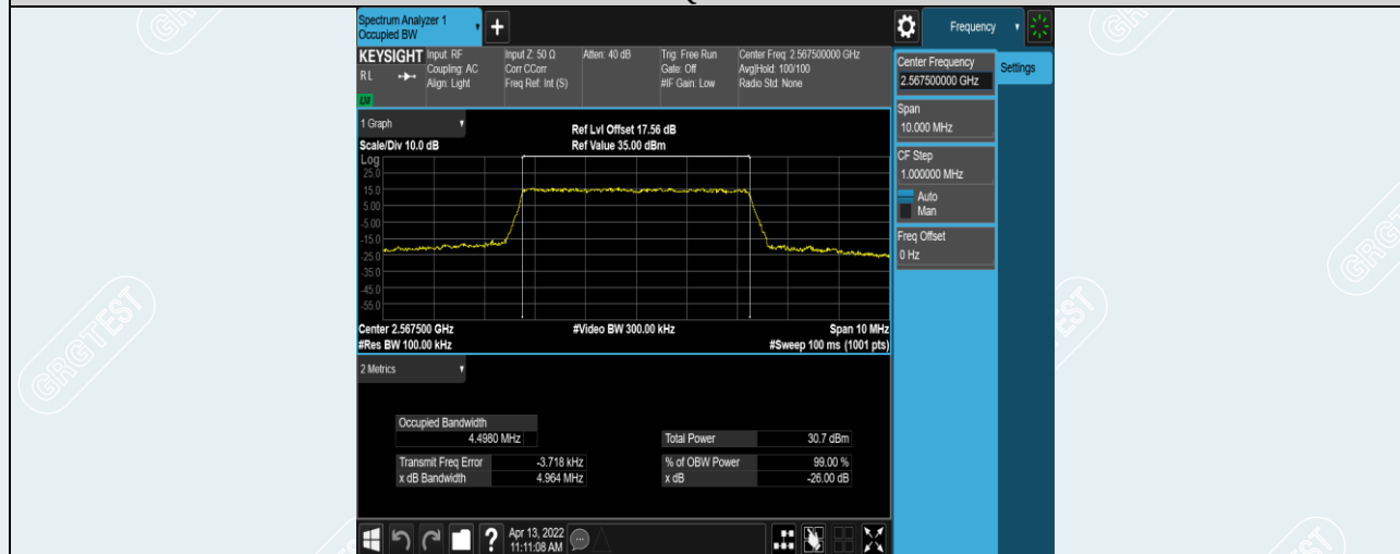
Band7-5MHz-16QAM-21425-25RB#0
