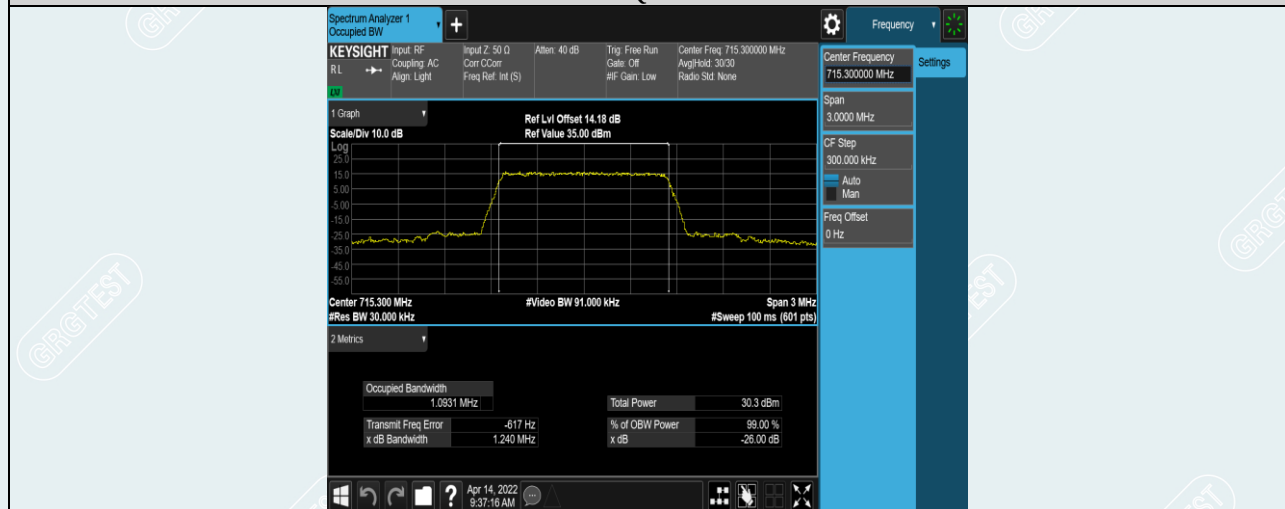
Band12-1.4MHz-QPSK-23173-6RB#0
