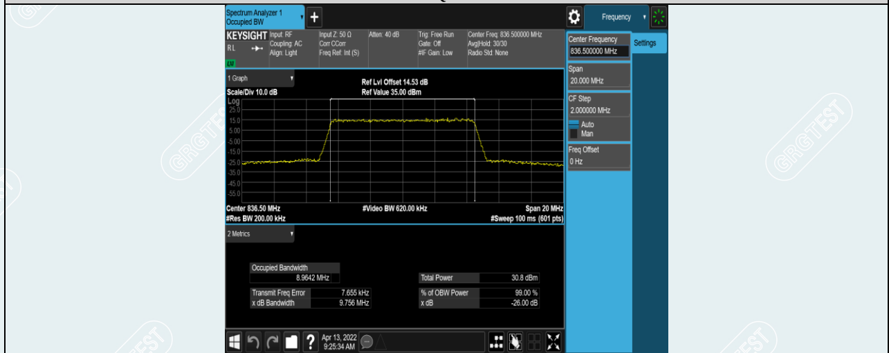
Band5-10MHz-16QAM-20525-50RB#0
