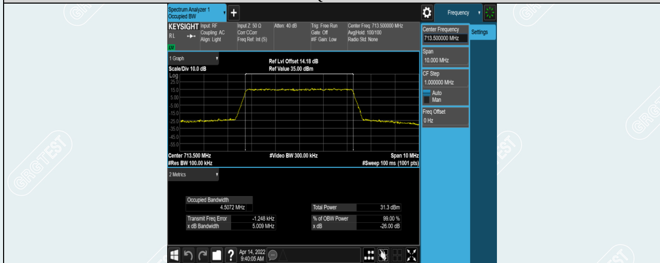
Band12-5MHz-QPSK-23155-25RB#0
