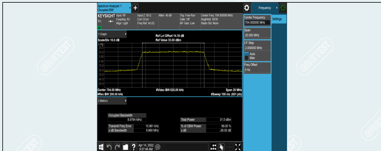
Band12-10MHz-QPSK-23060-50RB#0
