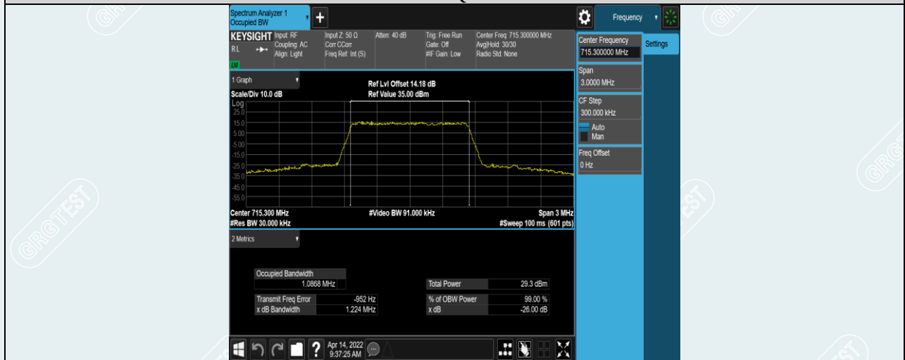
Band12-1.4MHz-16QAM-23173-6RB#0
