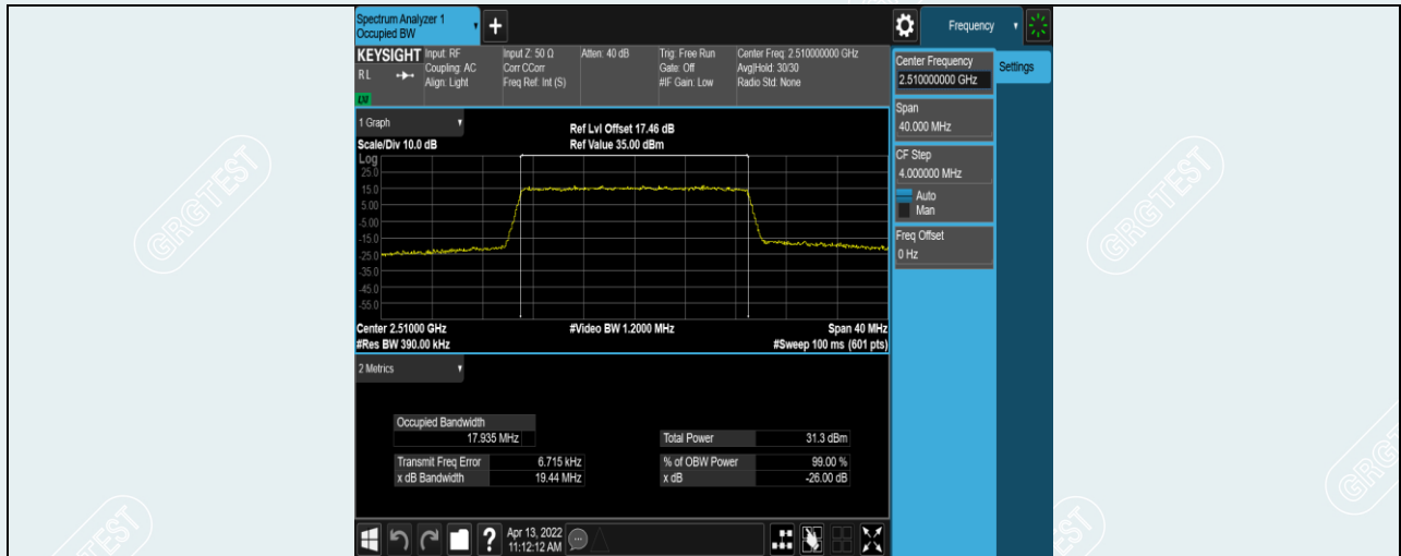
Band7-20MHz-16QAM-20850-100RB#0
