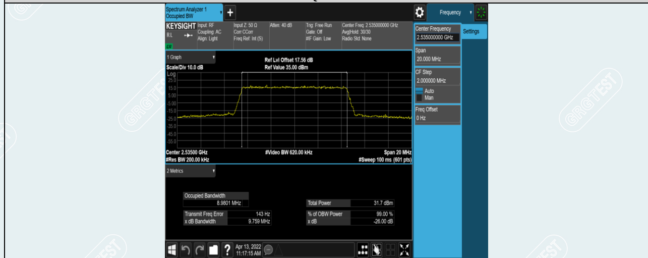
Band7-10MHz-QPSK-21100-50RB#0
