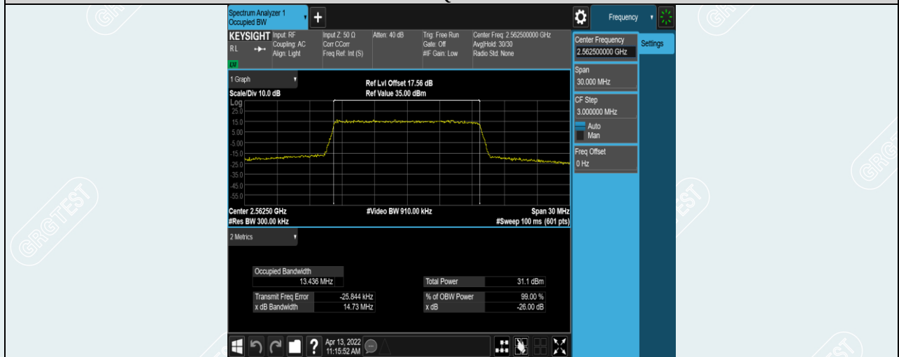
Band7-15MHz-16QAM-21375-75RB#0
