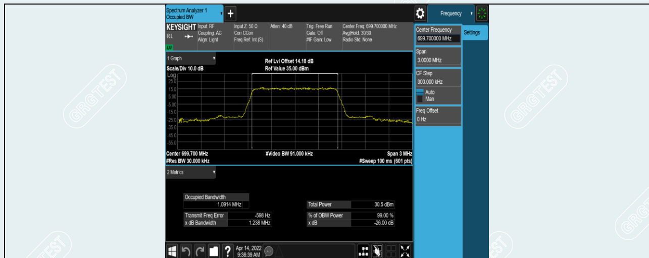
Band12-1.4MHz-QPSK-23017-6RB#0
