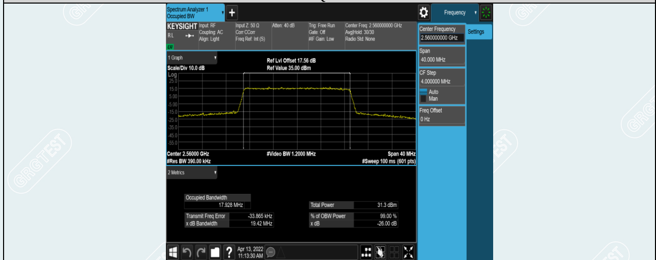
Band7-20MHz-16QAM-21350-100RB#0
