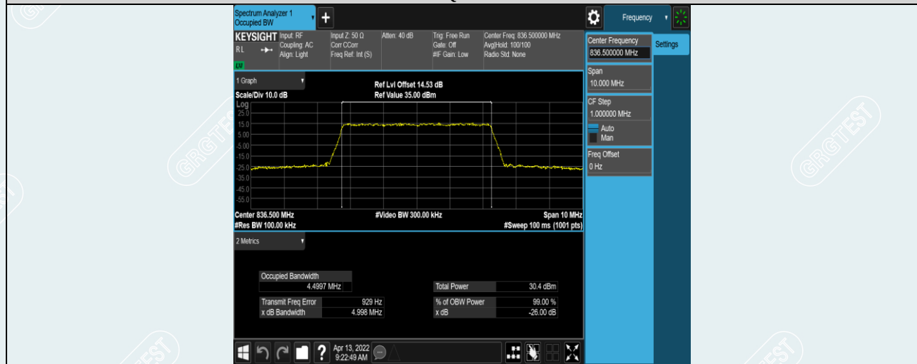
Band5-5MHz-16QAM-20525-25RB#0
