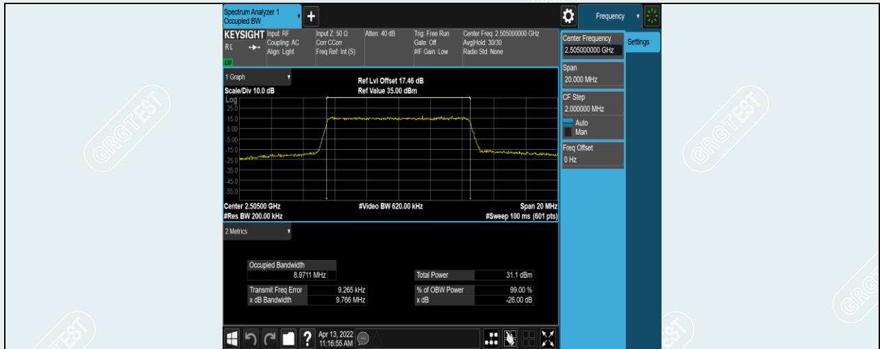
Band7-10MHz-16QAM-20800-50RB#0
