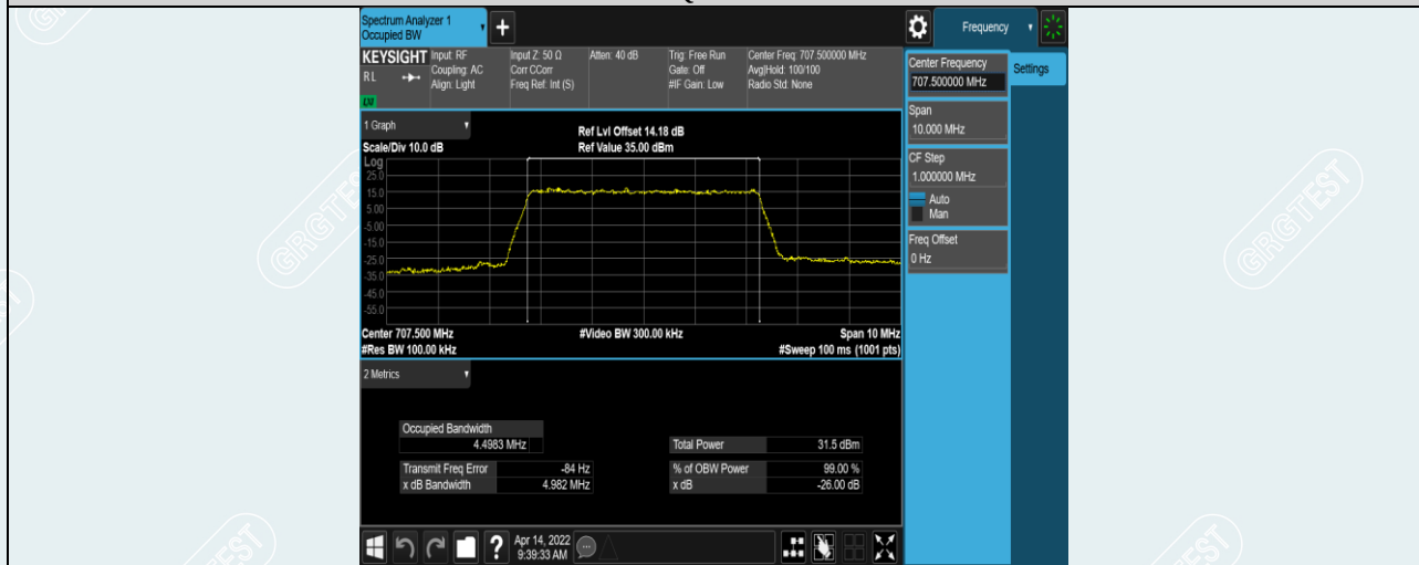
Band12-5MHz-QPSK-23095-25RB#0
