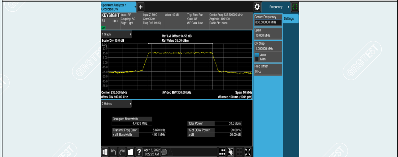
Band5-5MHz-QPSK-20525-25RB#0
