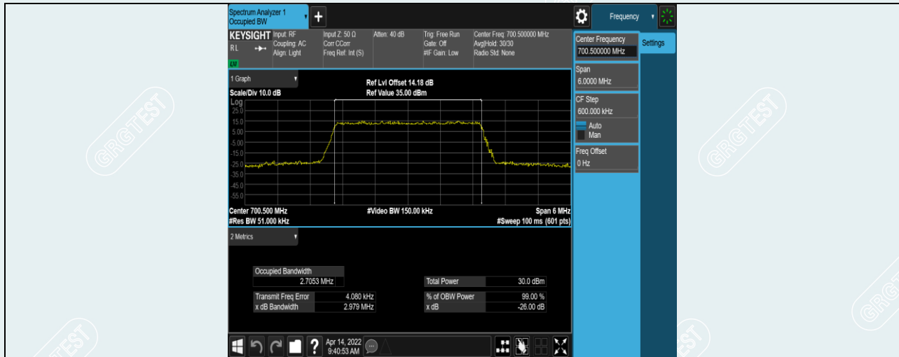
Band12-3MHz-16QAM-23025-15RB#0
