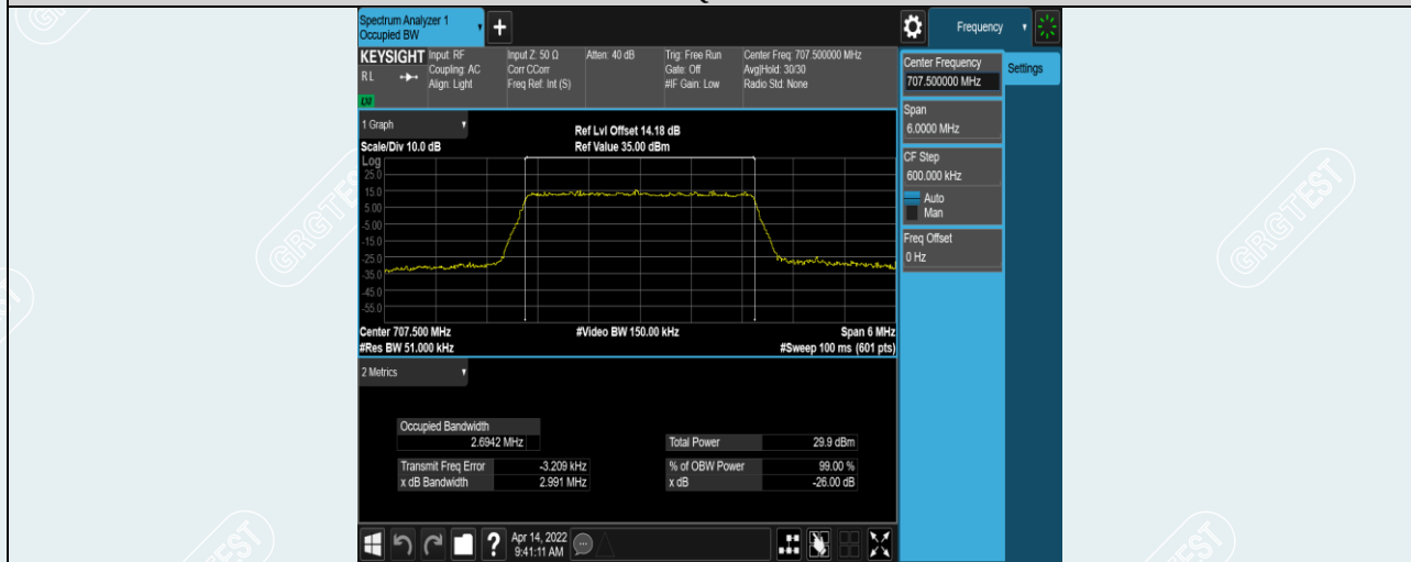
Band12-3MHz-16QAM-23095-15RB#0
