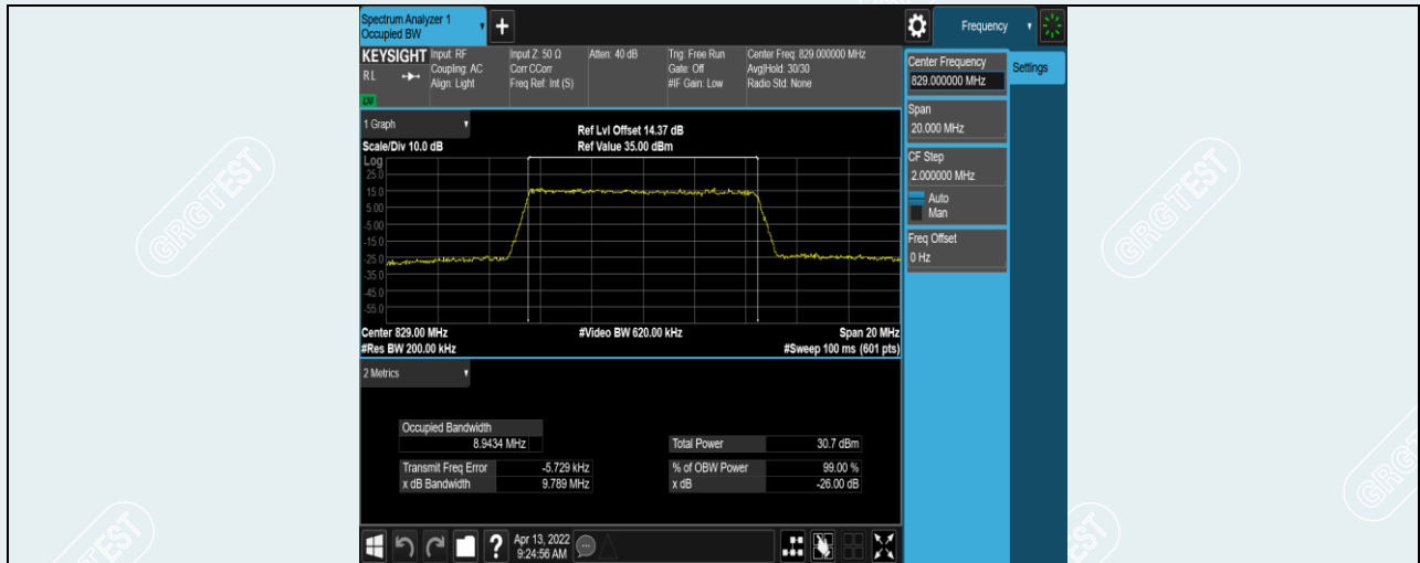
Band5-10MHz-16QAM-20450-50RB#0
