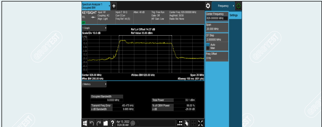
Band5-10MHz-QPSK-20450-50RB#0
