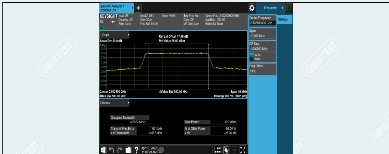
Band7-5MHz-16QAM-20775-25RB#0
