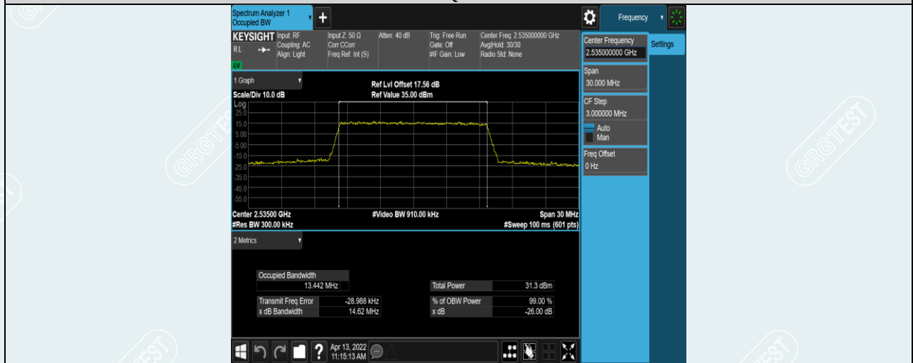
Band7-15MHz-16QAM-21100-75RB#0
