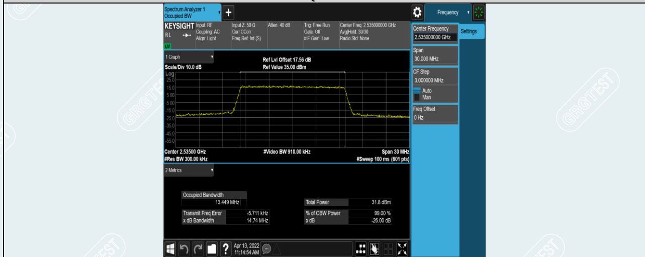
Band7-15MHz-QPSK-21100-75RB#0
