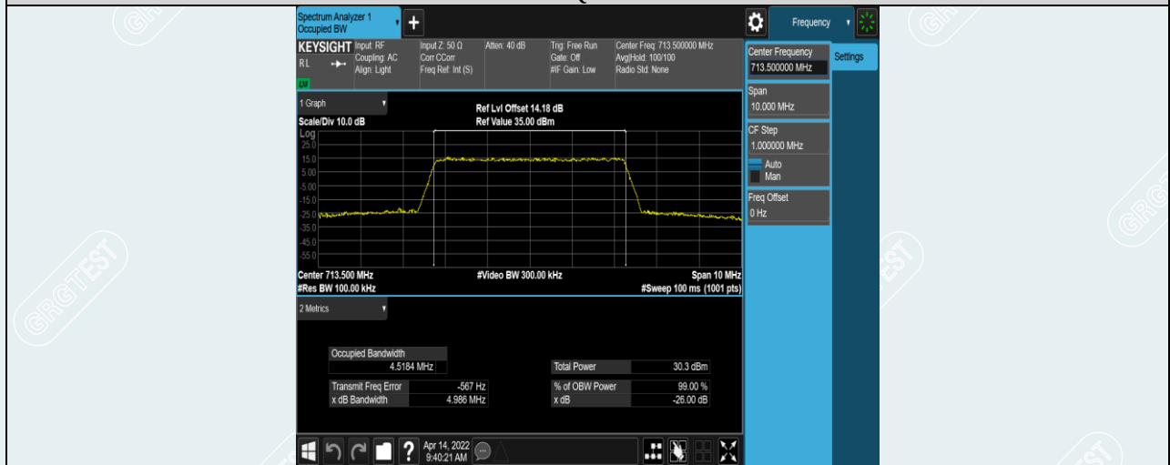
Band12-5MHz-16QAM-23155-25RB#0
