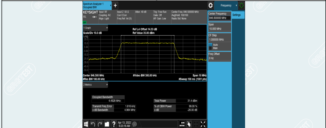
Band5-5MHz-QPSK-20625-25RB#0
