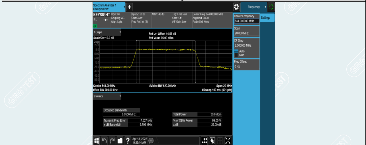
Band5-10MHz-16QAM-20600-50RB#0
