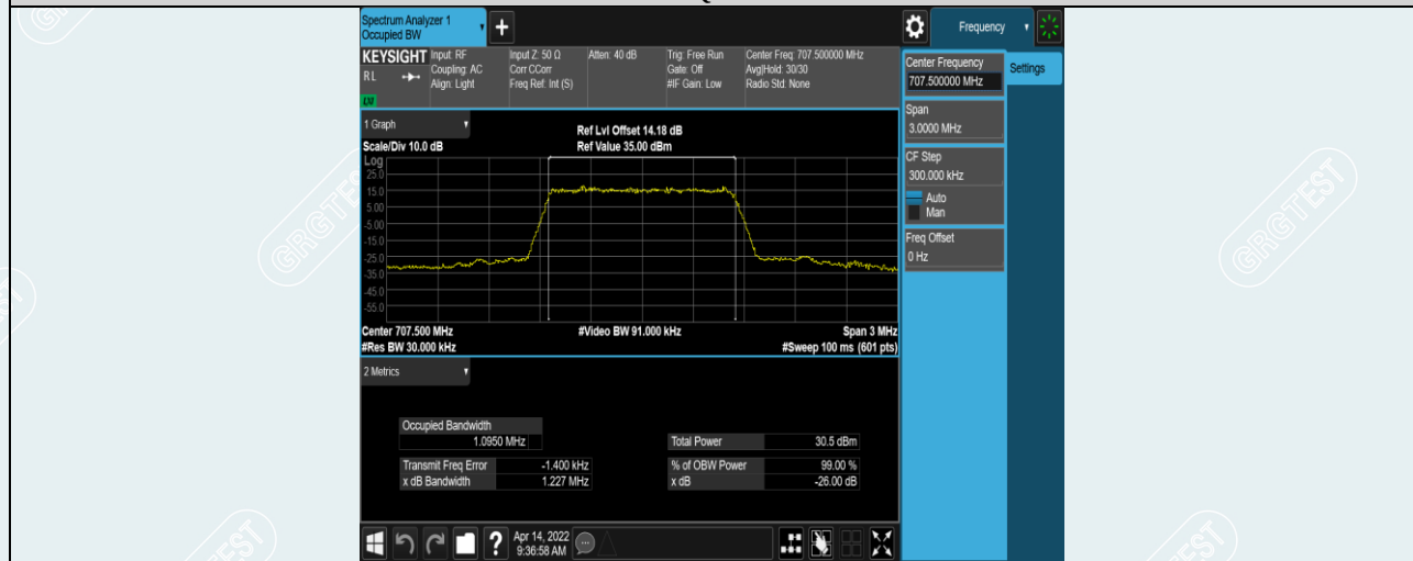
Band12-1.4MHz-QPSK-23095-6RB#0
