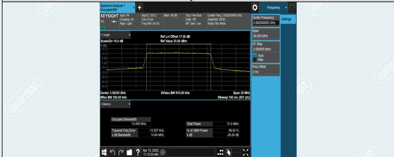
Band7-15MHz-QPSK-21375-75RB#0
