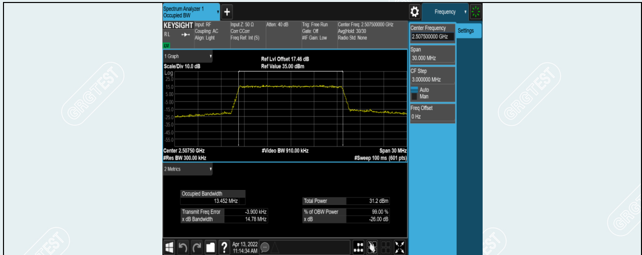
Band7-15MHz-16QAM-20825-75RB#0
