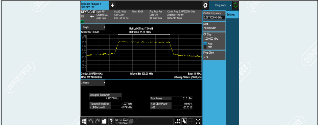
Band7-5MHz-QPSK-21425-25RB#0
