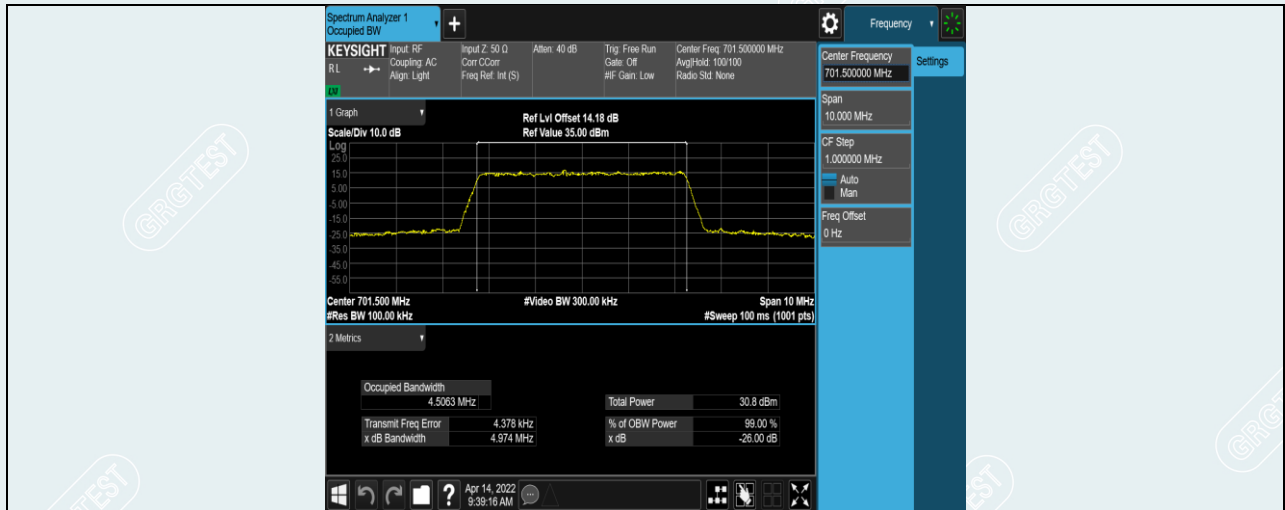
Band12-5MHz-16QAM-23035-25RB#0
