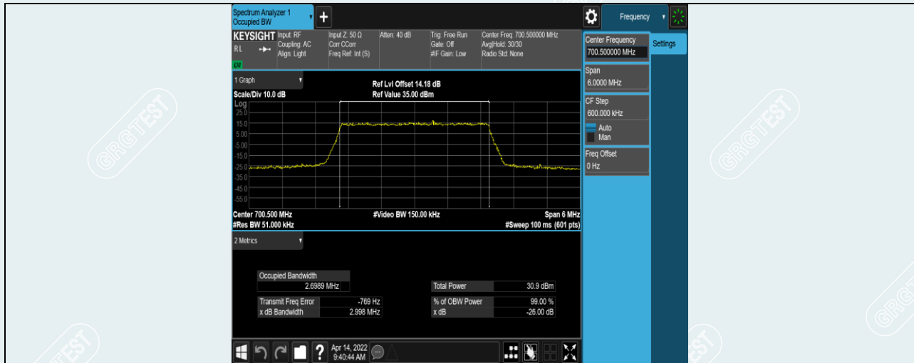
Band12-3MHz-QPSK-23025-15RB#0
