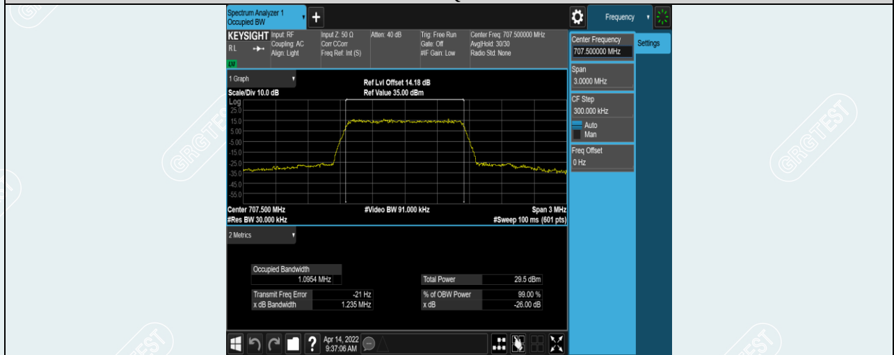
Band12-1.4MHz-16QAM-23095-6RB#0
