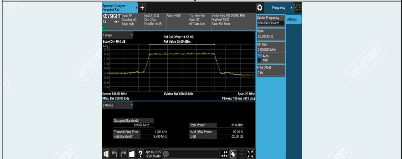
Band5-10MHz-QPSK-20525-50RB#0
