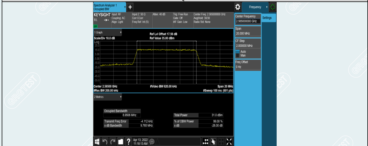
Band7-10MHz-16QAM-21400-50RB#0
