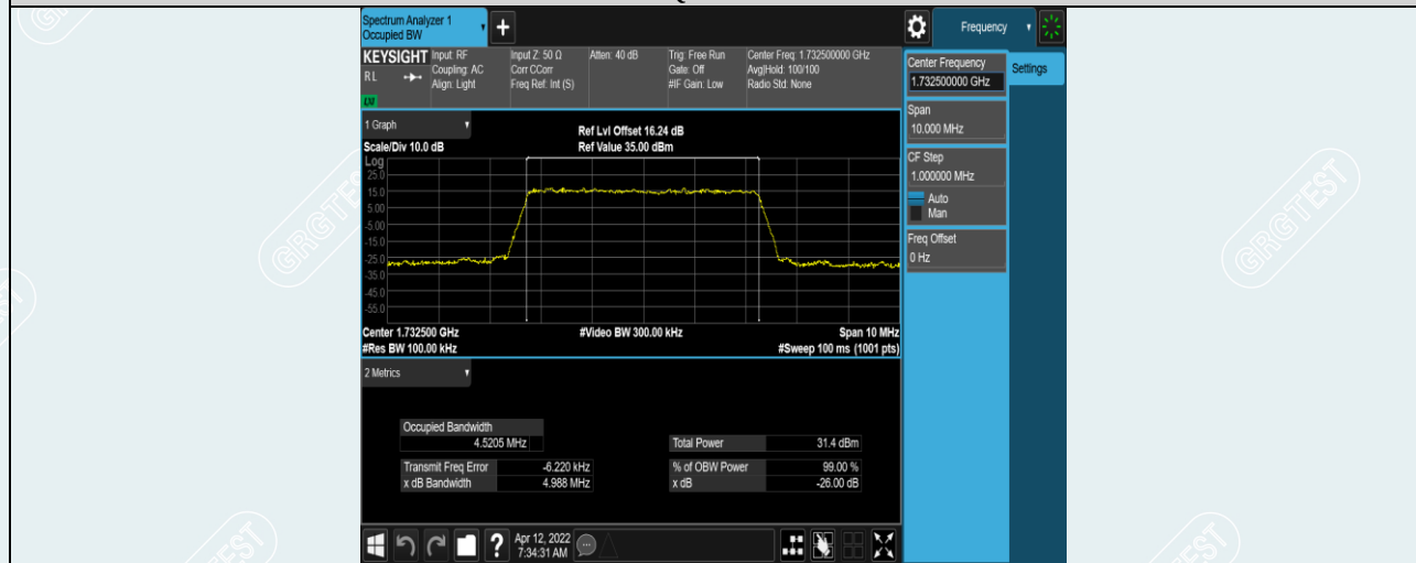
Band4-5MHz-QPSK-20175-25RB#0
