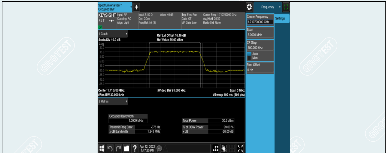
Band4-1.4MHz-QPSK-19957-6RB#0
