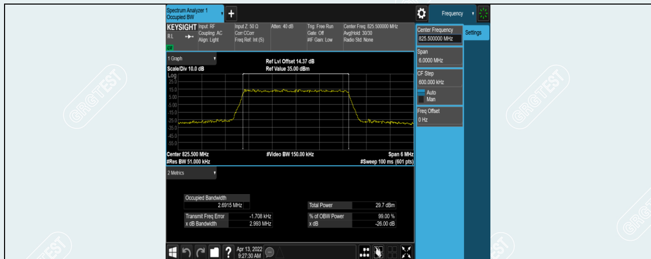
Band5-3MHz-16QAM-20415-15RB#0
