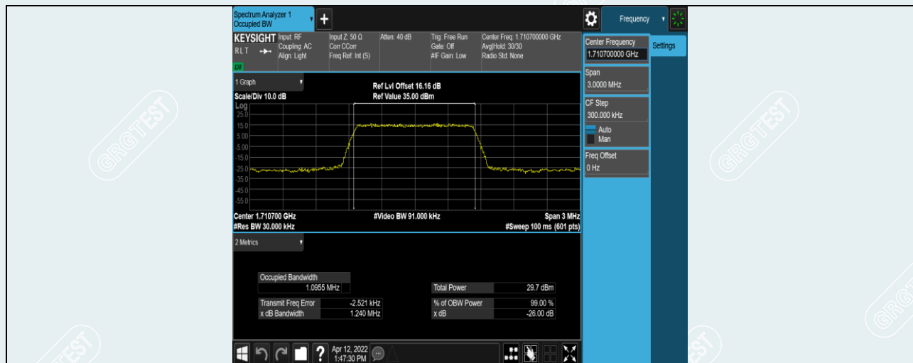
Band4-1.4MHz-16QAM-19957-6RB#0
