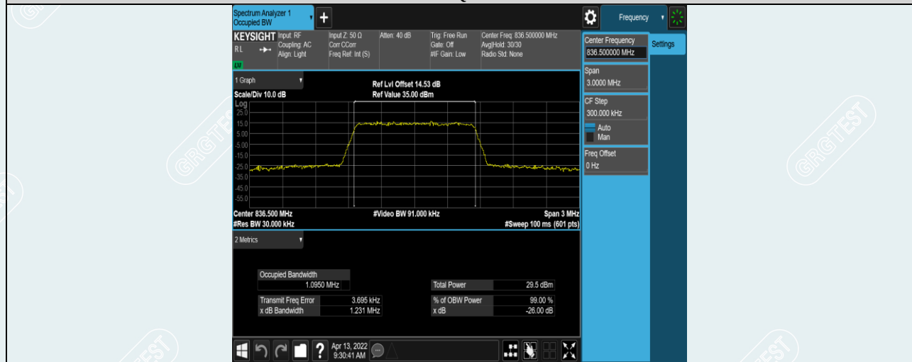
Band5-1.4MHz-16QAM-20525-6RB#0
