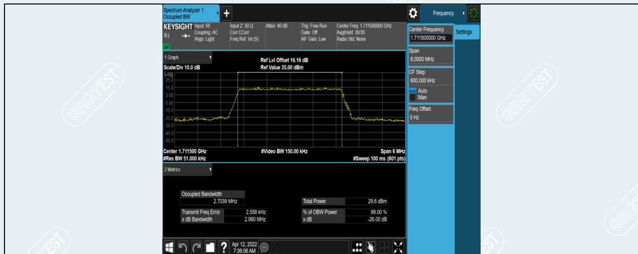
Band4-3MHz-16QAM-19965-15RB#0
