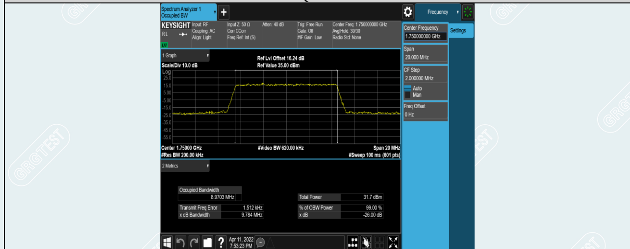
Band4-10MHz-QPSK-20350-50RB#0
