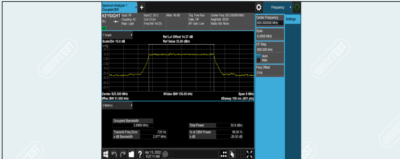
Band5-3MHz-QPSK-20415-15RB#0
