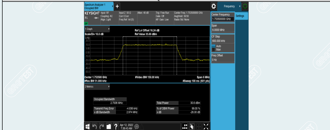
Band4-3MHz-QPSK-20385-15RB#0
