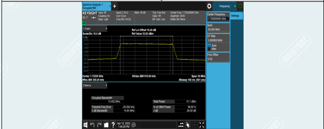
Band4-15MHz-16QAM-20175-75RB#0
