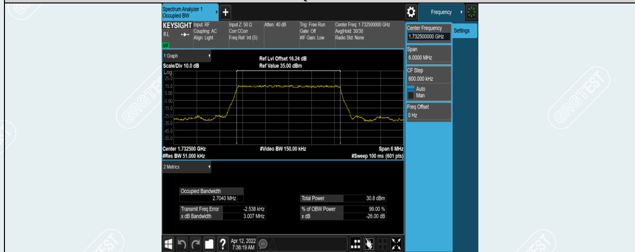
Band4-3MHz-QPSK-20175-15RB#0
