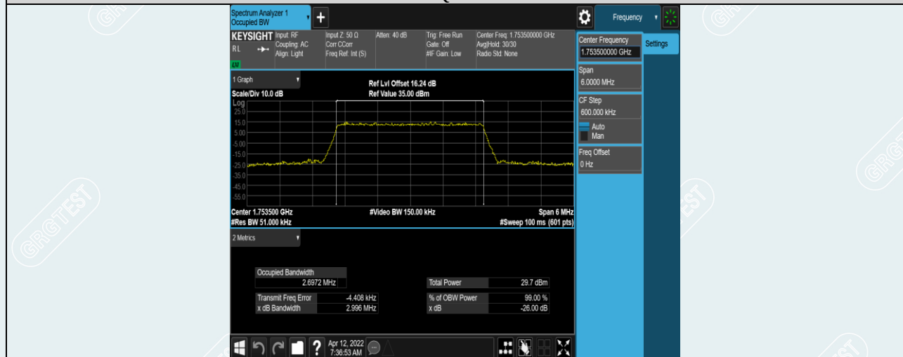
Band4-3MHz-16QAM-20385-15RB#0
