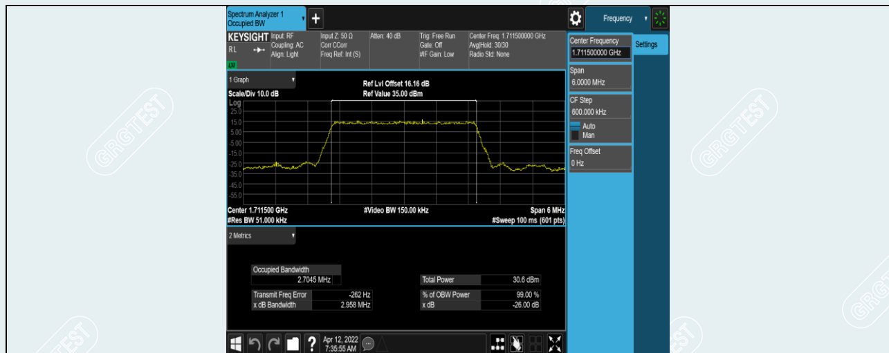
Band4-3MHz-QPSK-19965-15RB#0
