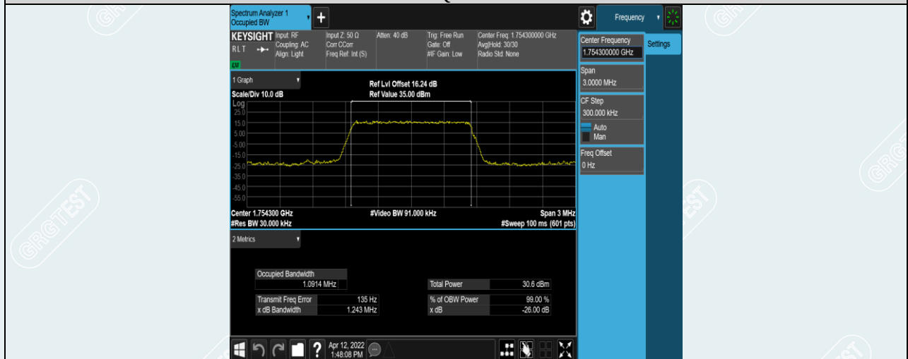
Band4-1.4MHz-QPSK-20393-6RB#0
