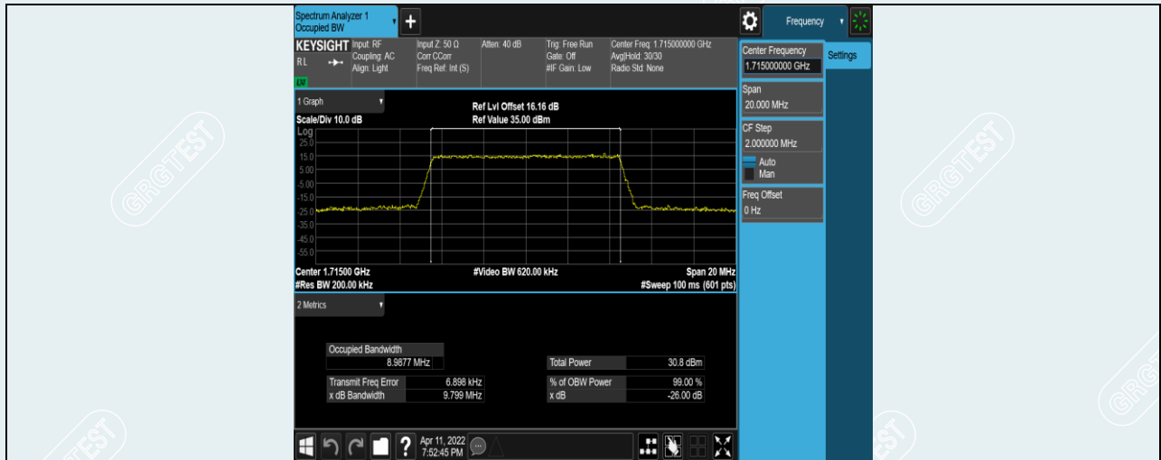
Band4-10MHz-16QAM-20000-50RB#0
