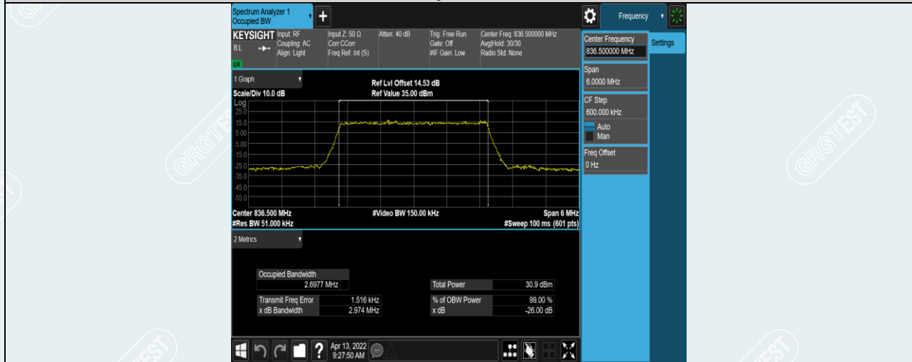
Band5-3MHz-QPSK-20525-15RB#0
