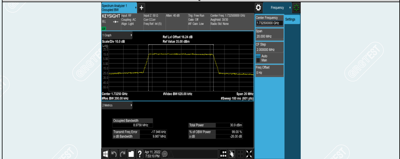
Band4-10MHz-16QAM-20175-50RB#0
