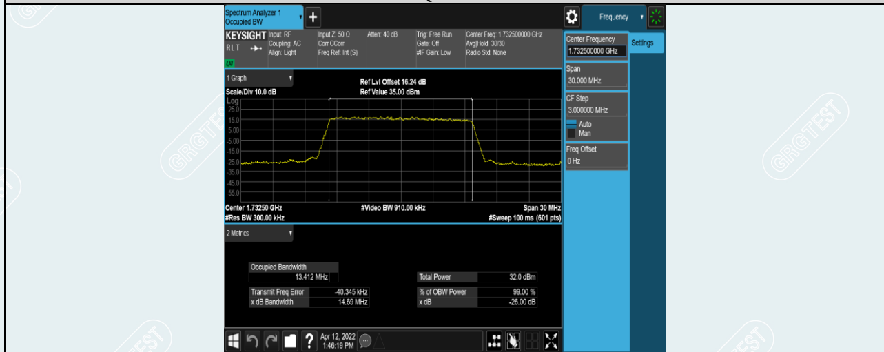
Band4-15MHz-QPSK-20175-75RB#0
