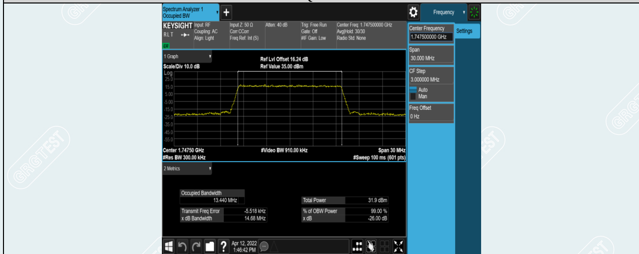
Band4-15MHz-QPSK-20325-75RB#0
