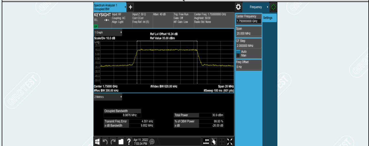
Band4-10MHz-16QAM-20350-50RB#0
