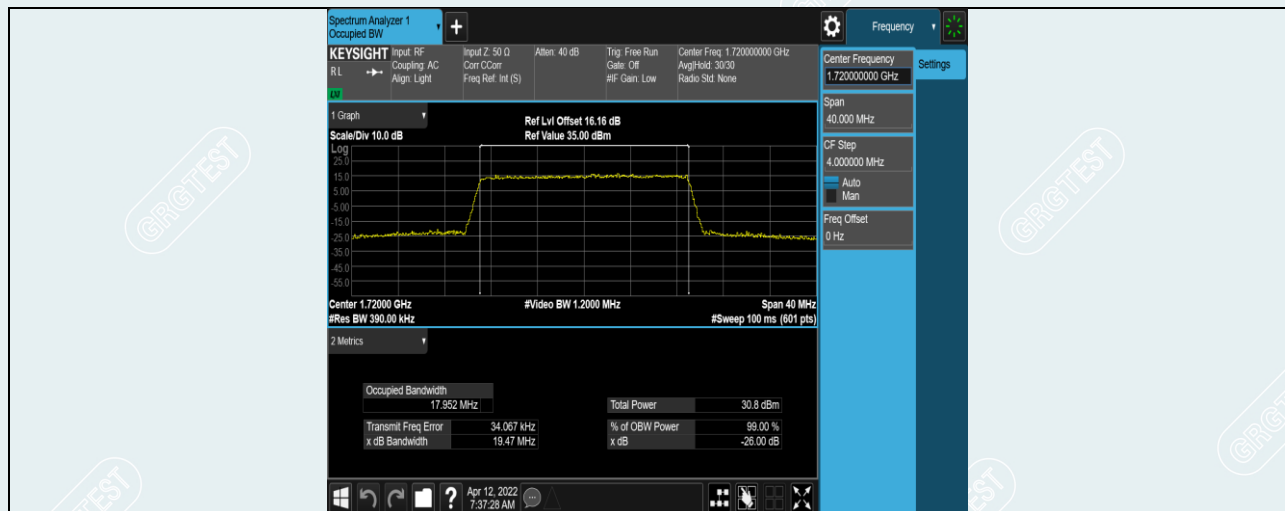
Band4-20MHz-16QAM-20050-100RB#0
