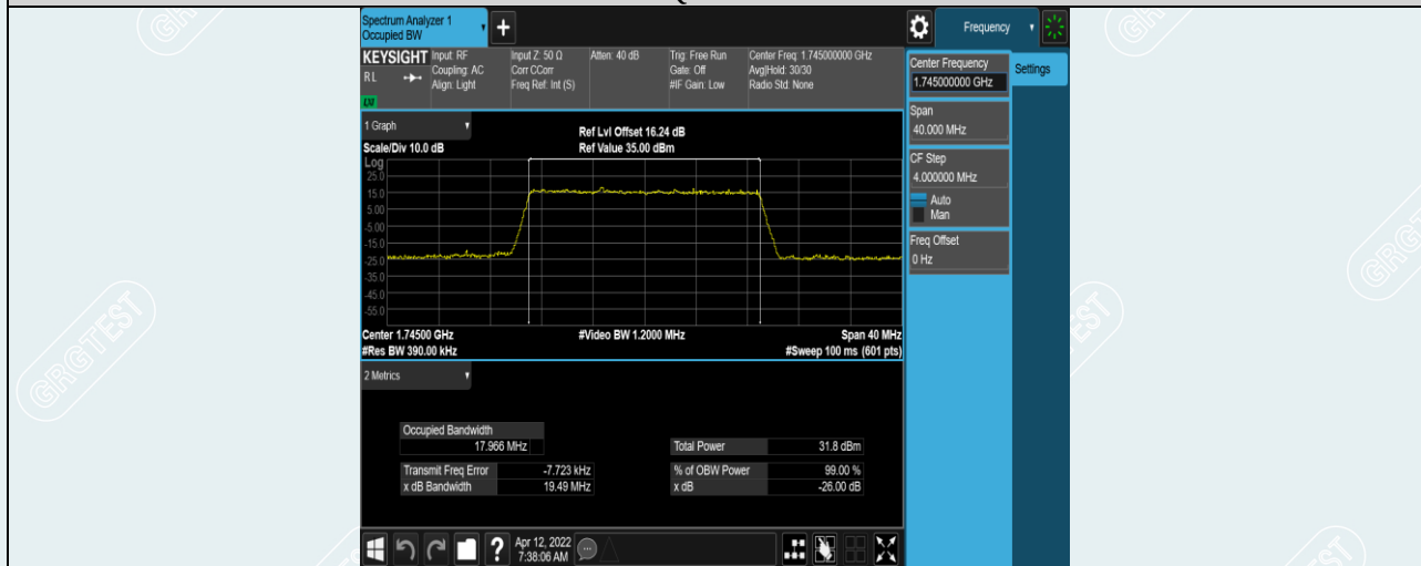
Band4-20MHz-QPSK-20300-100RB#0
