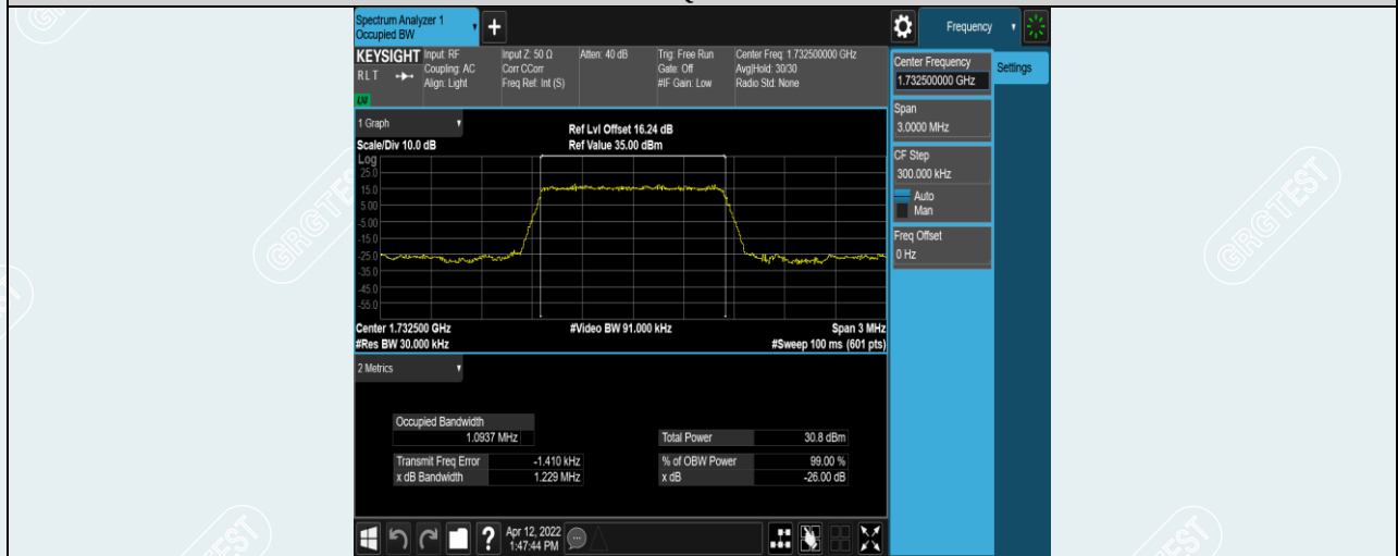
Band4-1.4MHz-QPSK-20175-6RB#0
