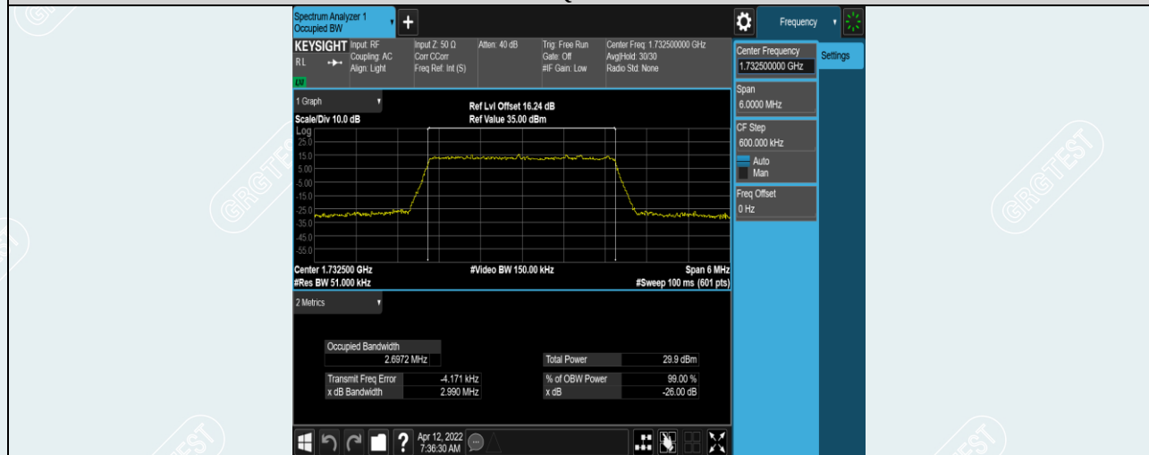
Band4-3MHz-16QAM-20175-15RB#0
