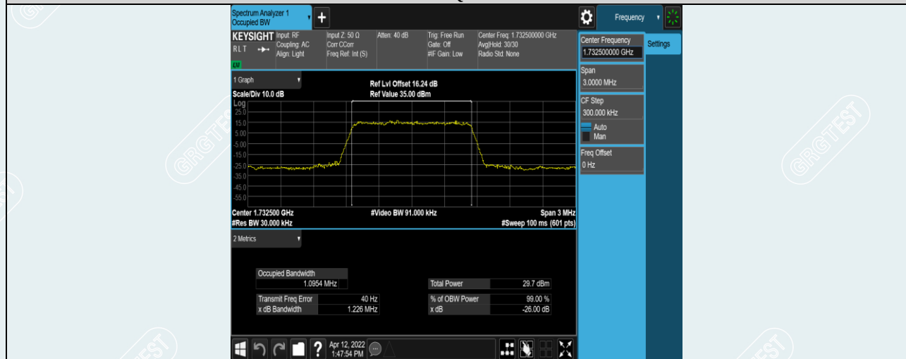
Band4-1.4MHz-16QAM-20175-6RB#0
