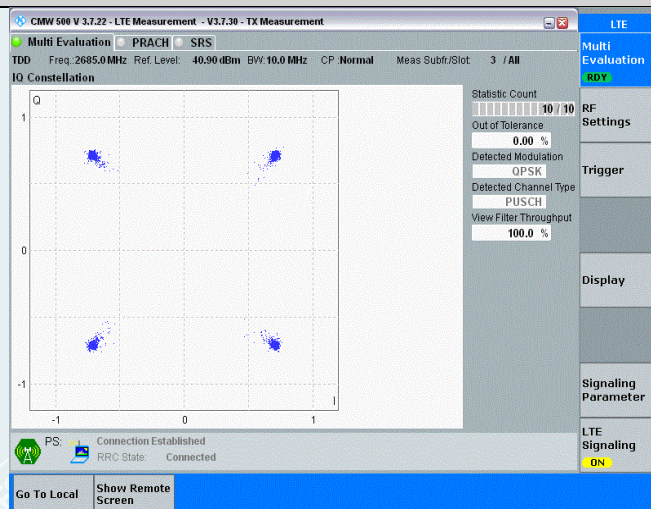
Band41-10MHz-QPSK-41540-50RB#0
