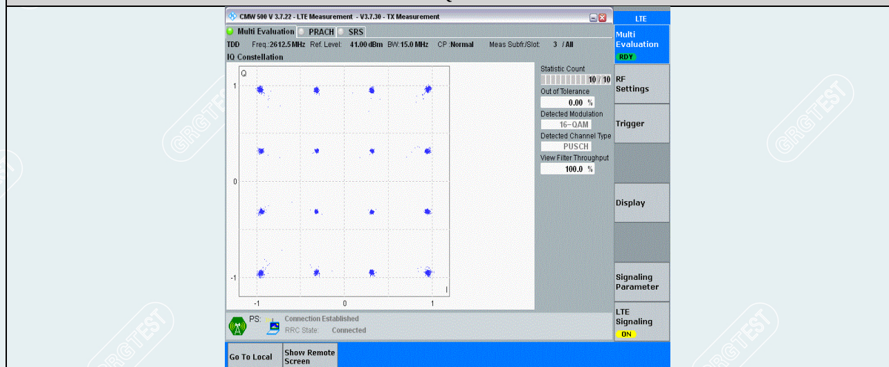
Band38-15MHz-16QAM-38175-75RB#0
