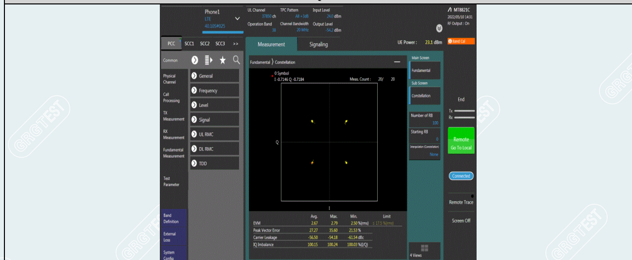
Band38-20MHz-QPSK-37850-100RB#0
