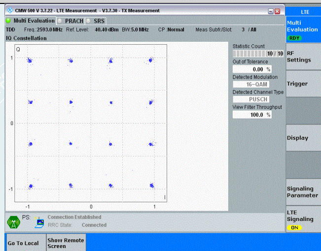
Band41-5MHz-16QAM-40620-25RB#0
