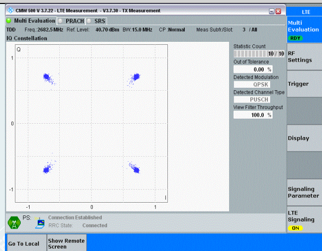
Band41-15MHz-QPSK-41515-75RB#0
