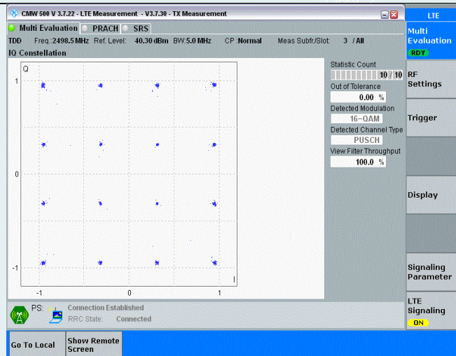
Band41-5MHz-16QAM-39675-25RB#0
