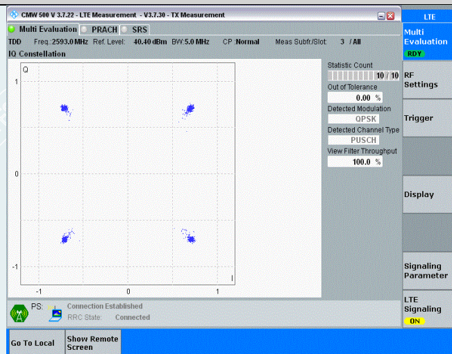
Band41-5MHz-QPSK-40620-25RB#0
