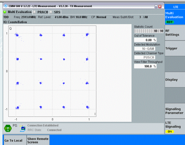
Band41-10MHz-16QAM-40620-50RB#0
