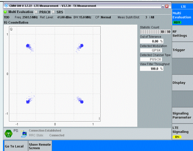
Band41-15MHz-QPSK-39725-75RB#0
