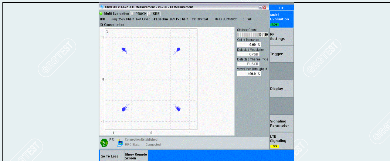
Band38-15MHz-QPSK-38000-75RB#0
