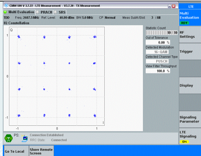
Band41-5MHz-16QAM-41565-25RB#0
