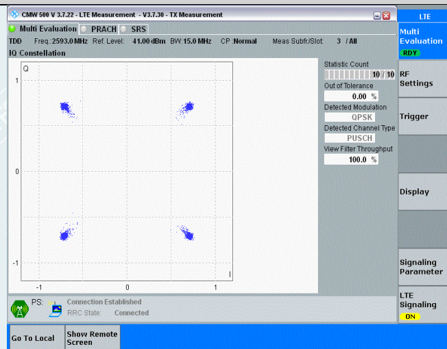
Band41-15MHz-QPSK-40620-75RB#0
