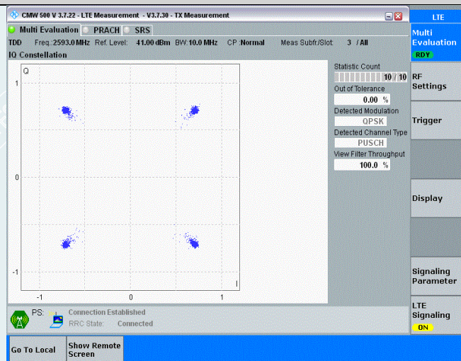
Band41-10MHz-QPSK-40620-50RB#0
