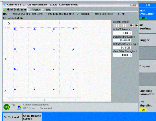
Band41-10MHz-16QAM-39700-50RB#0
