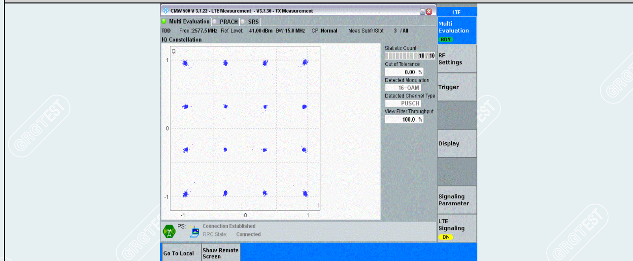
Band38-15MHz-16QAM-37825-75RB#0
