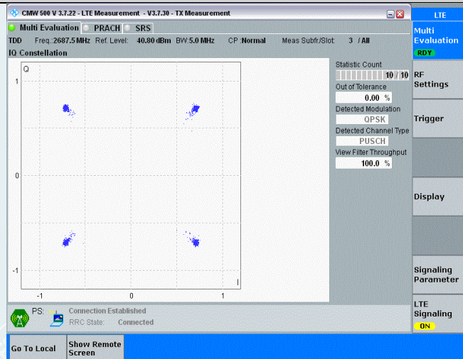
Band41-5MHz-QPSK-41565-25RB#0
