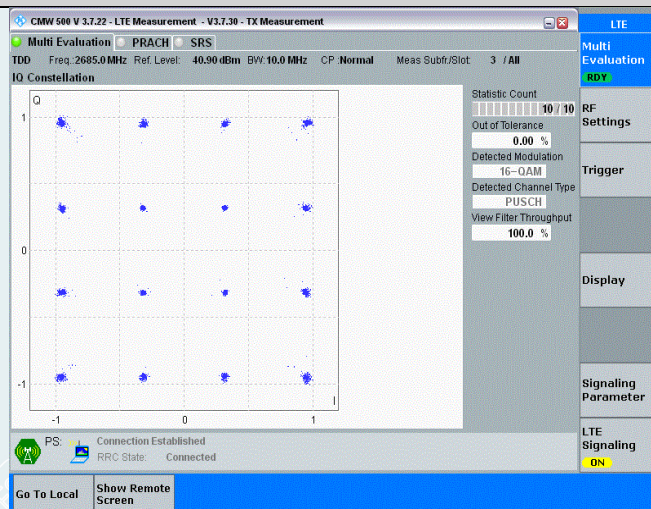
Band41-10MHz-16QAM-41540-50RB#0
