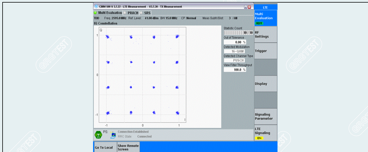
Band38-15MHz-16QAM-38000-75RB#0
