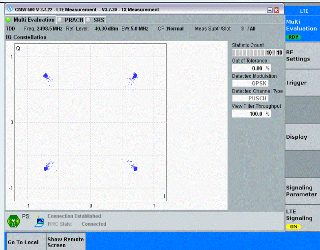
Band41-5MHz-QPSK-39675-25RB#0
