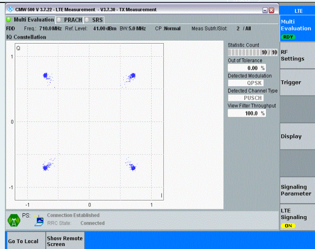
Band17-5MHz-QPSK-23790-25RB#0
