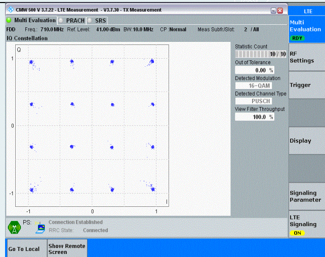
Band17-10MHz-16QAM-23790-50RB#0
