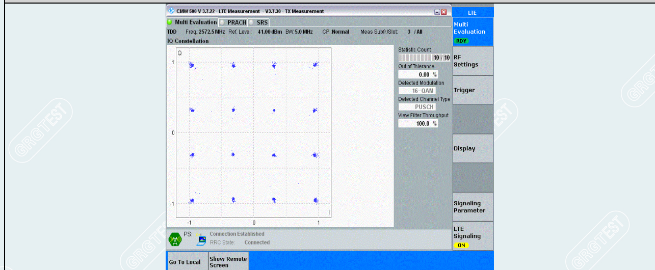
Band38-5MHz-16QAM-37775-25RB#0
