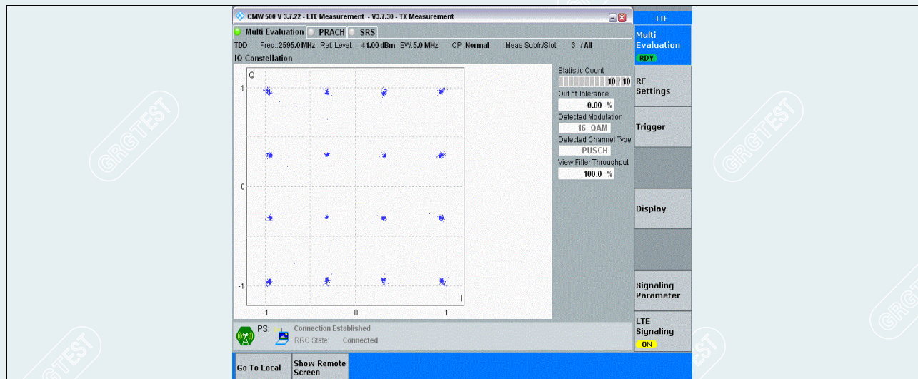
Band38-5MHz-16QAM-38000-25RB#0
