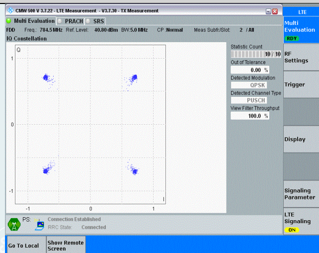
Band13-5MHz-QPSK-23255-25RB#0
