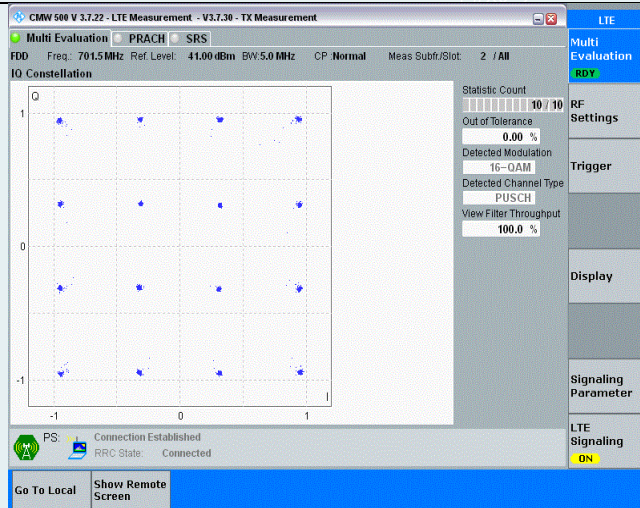
Band12-5MHz-16QAM-23035-25RB#0
