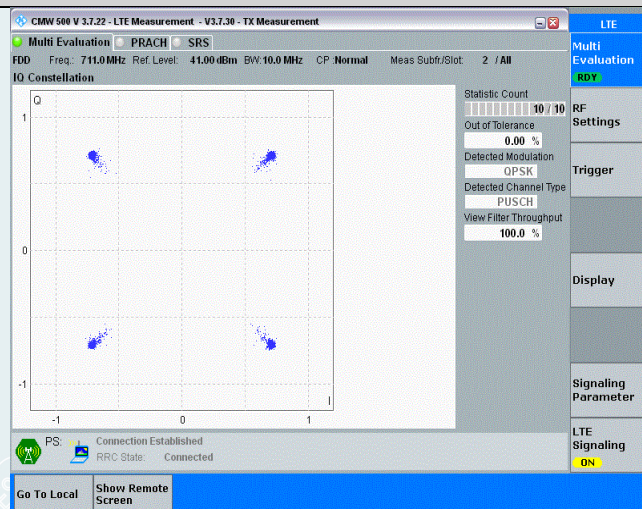
Band12-10MHz-QPSK-23130-50RB#0
