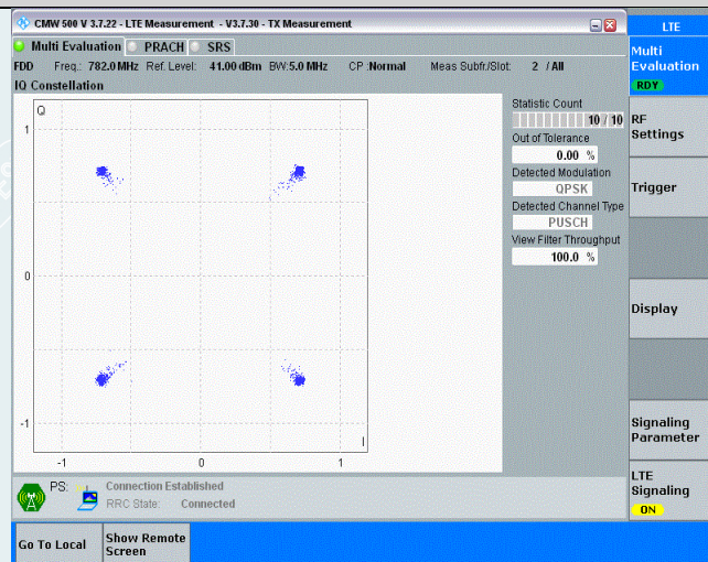
Band13-5MHz-QPSK-23230-25RB#0
