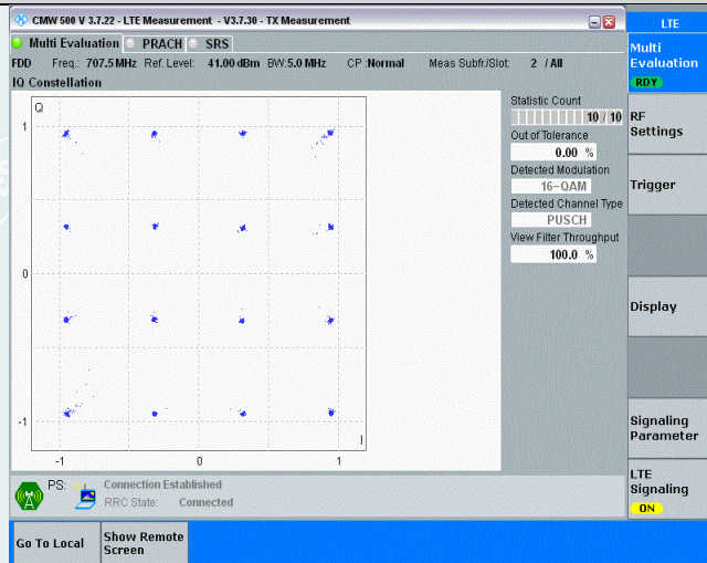
Band12-5MHz-16QAM-23095-25RB#0
