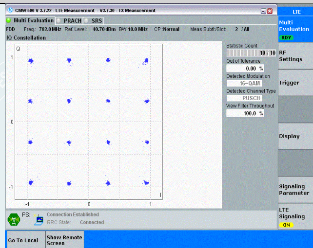
Band13-10MHz-16QAM-23230-50RB#0
