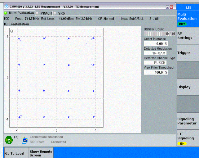
Band12-3MHz-16QAM-23165-15RB#0
