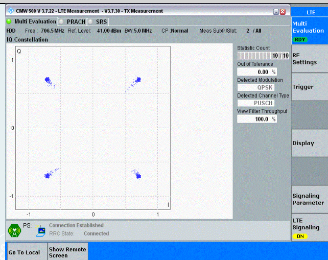
Band17-5MHz-QPSK-23755-25RB#0
