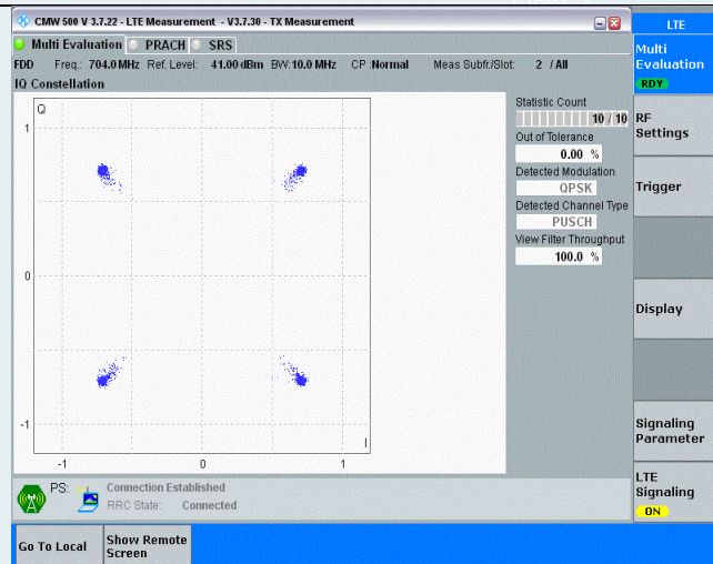
Band12-10MHz-QPSK-23060-50RB#0
