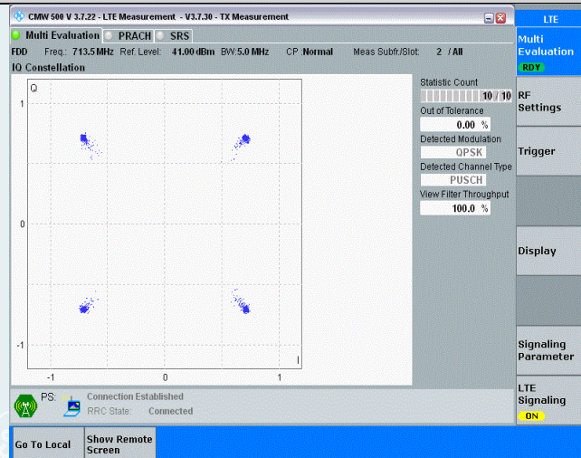
Band12-5MHz-QPSK-23155-25RB#0
