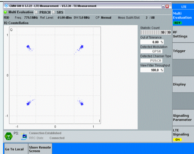
Band13-5MHz-QPSK-23205-25RB#0
