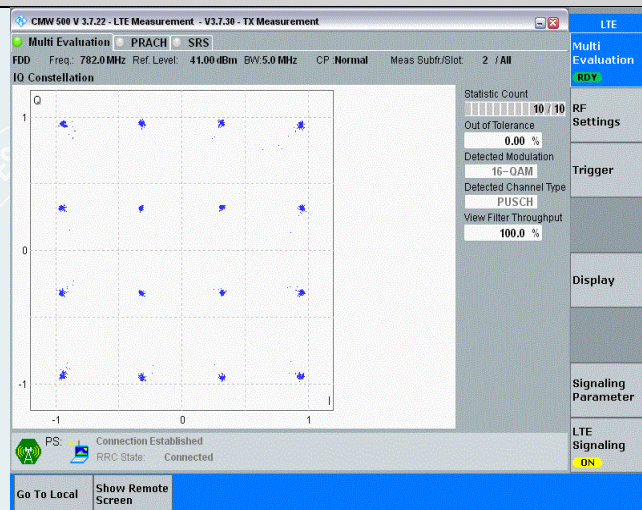
Band13-5MHz-16QAM-23230-25RB#0
