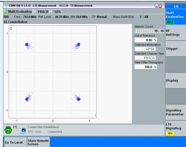
Band13-10MHz-QPSK-23230-50RB#0
