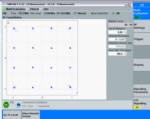
Band12-10MHz-16QAM-23095-50RB#0
