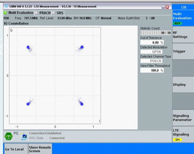
Band12-10MHz-QPSK-23095-50RB#0
