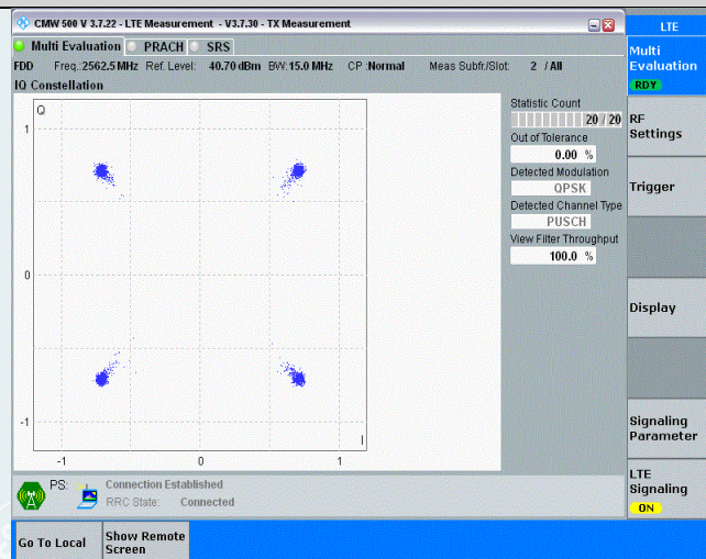
Band7-15MHz-QPSK-21375-75RB#0
