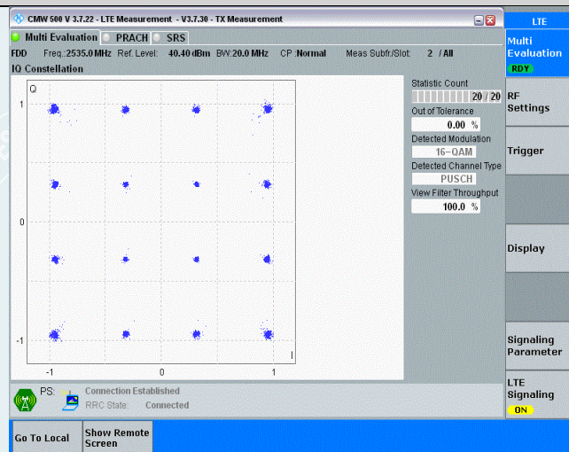
Band7-20MHz-16QAM-21100-100RB#0
