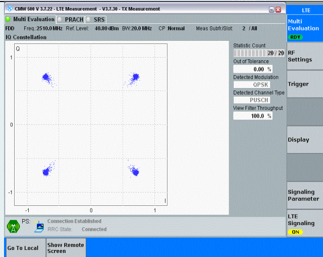
Band7-20MHz-QPSK-20850-100RB#0
