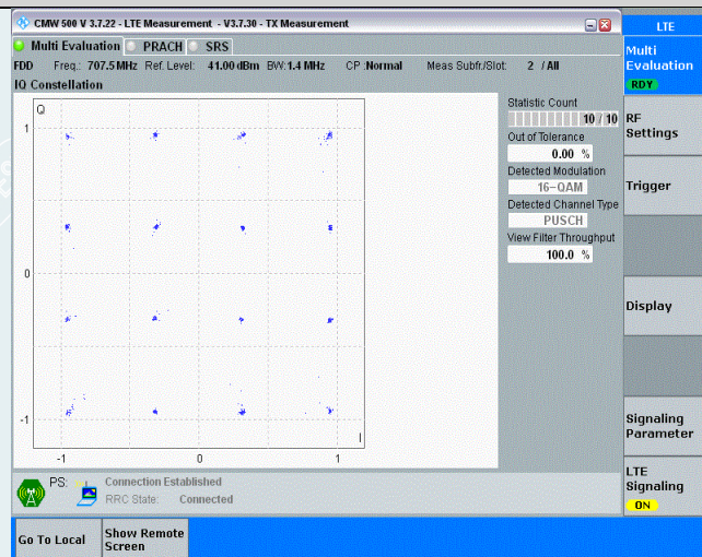
Band12-1.4MHz-16QAM-23095-6RB#0
