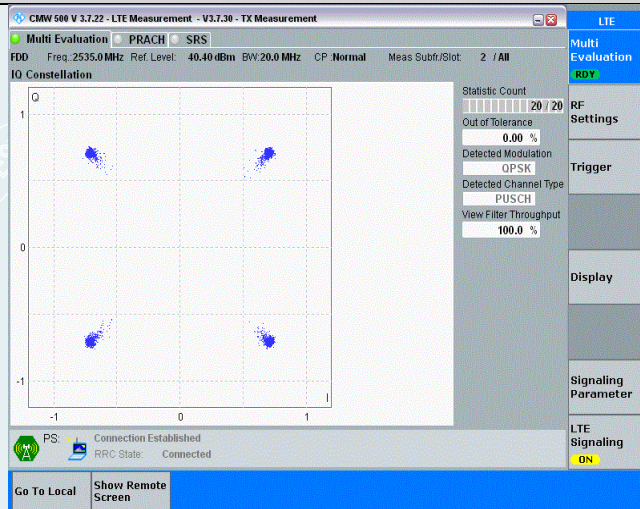
Band7-20MHz-QPSK-21100-100RB#0
