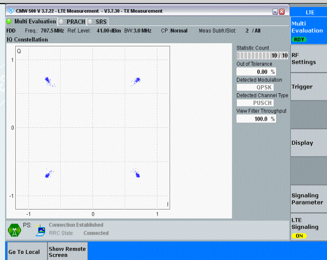
Band12-3MHz-QPSK-23095-15RB#0
