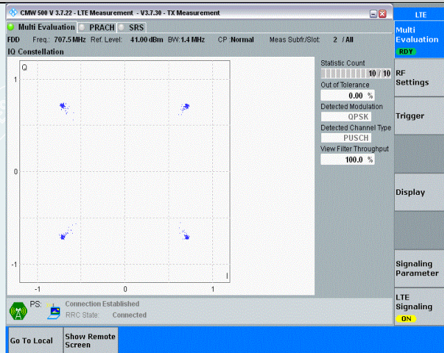
Band12-1.4MHz-QPSK-23095-6RB#0
