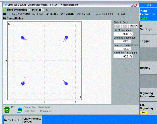
Band7-15MHz-QPSK-20825-75RB#0
