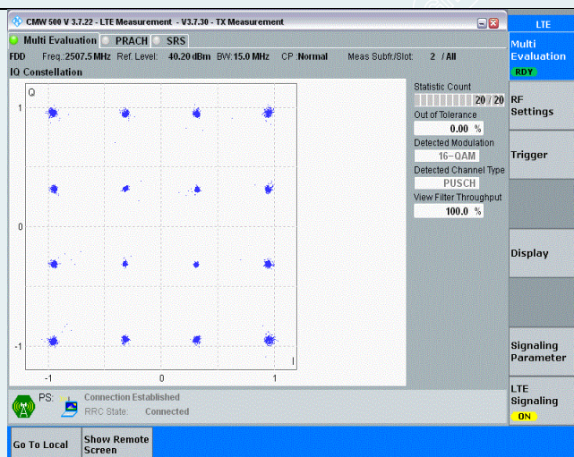
Band7-15MHz-16QAM-20825-75RB#0
