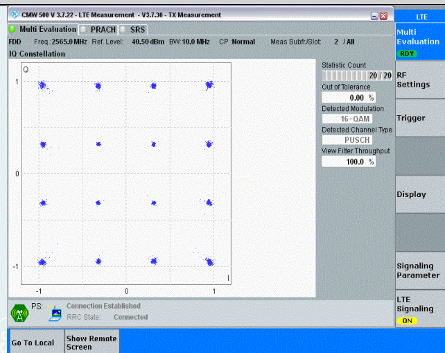
Band7-10MHz-16QAM-21400-50RB#0
