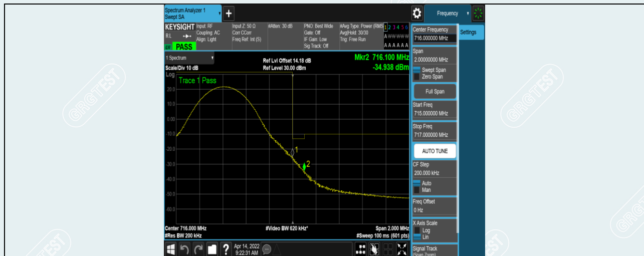
Band12-10MHz-16QAM-23130-1RB#49
