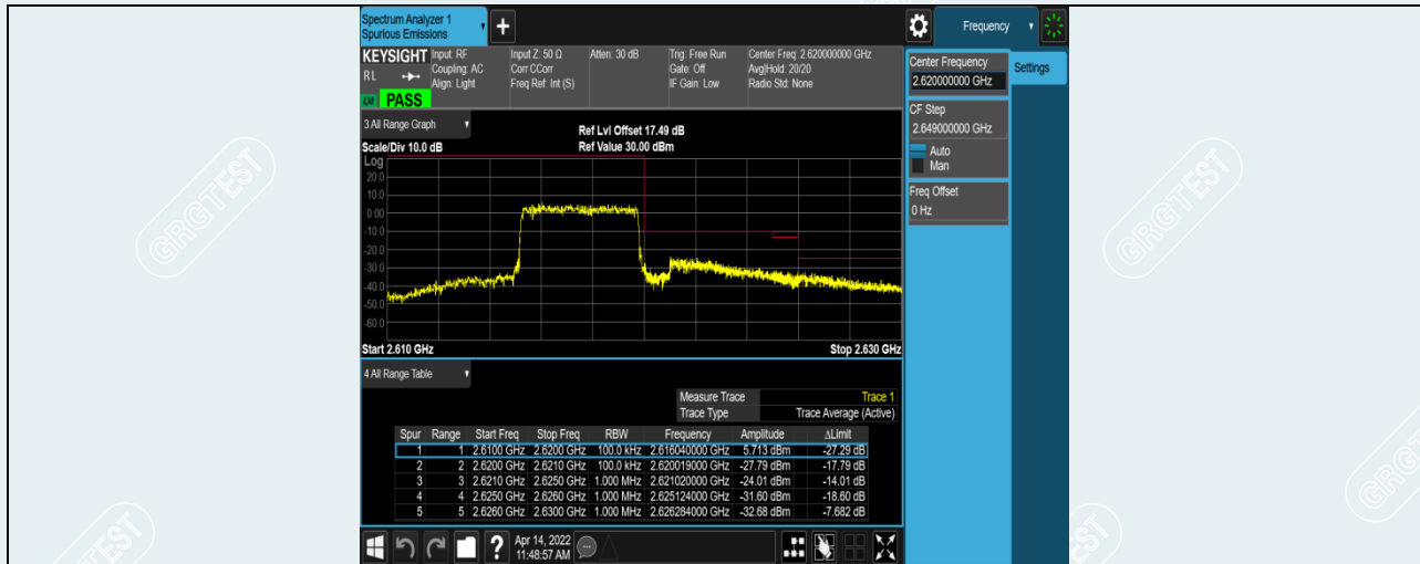
Band38-5MHz-16QAM-38225-25RB#0
