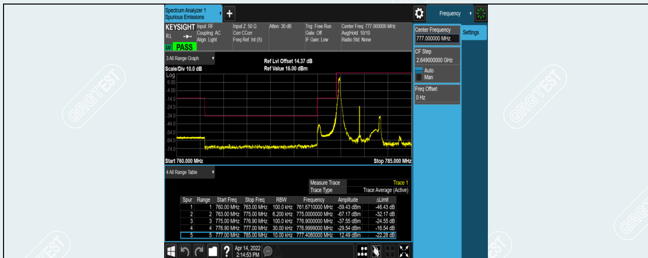
Band13-5MHz-16QAM-23205-1RB#0
