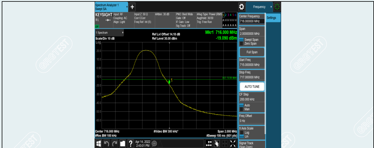
Band17-5MHz-QPSK-23825-1RB#24
