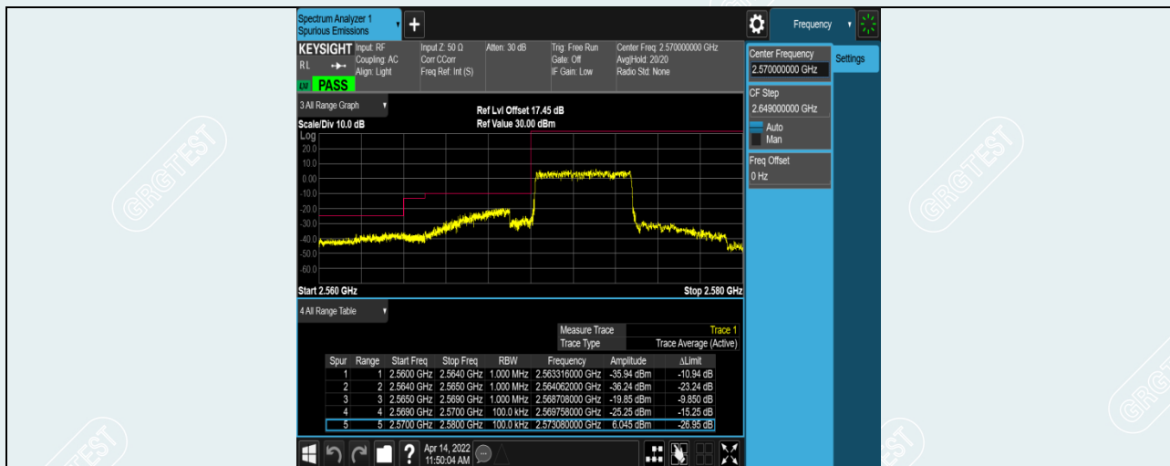
Band38-5MHz-QPSK-37775-25RB#0
