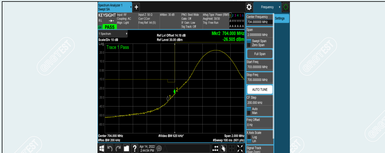
Band17-10MHz-QPSK-23780-1RB#0
