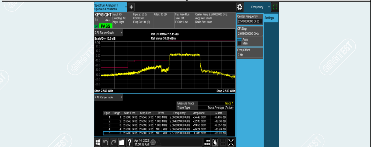
Band38-5MHz-16QAM-37775-25RB#0
