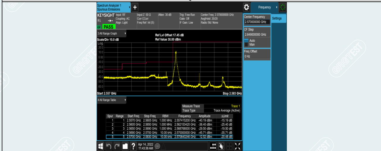
Band38-10MHz-QPSK-37800-1RB#0
