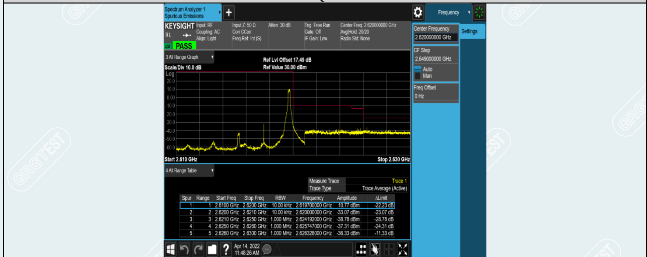
Band38-5MHz-16QAM-38225-1RB#24
