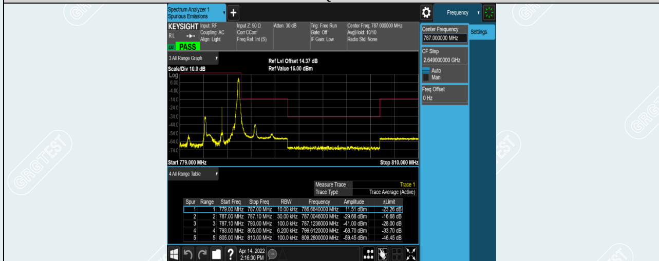
Band13-5MHz-16QAM-23255-1RB#24
