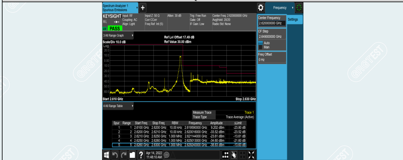
Band38-5MHz-QPSK-38225-1RB#24
