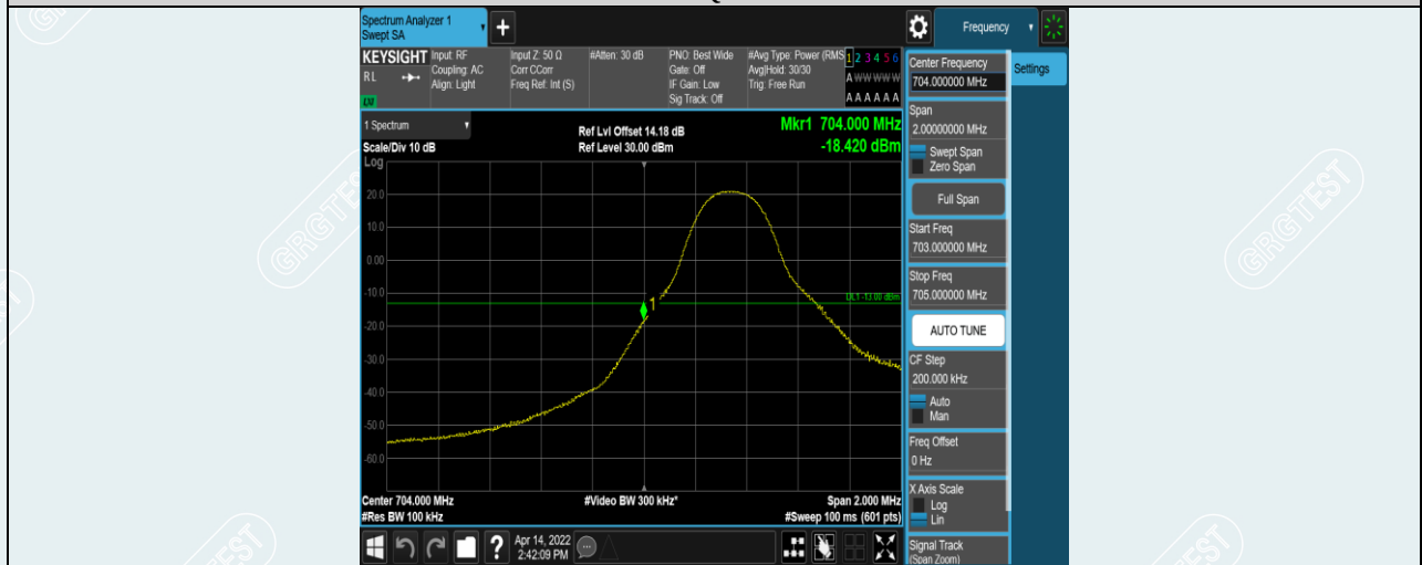
Band17-5MHz-QPSK-23755-1RB#0
