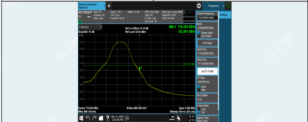
Band17-5MHz-16QAM-23825-1RB#24
