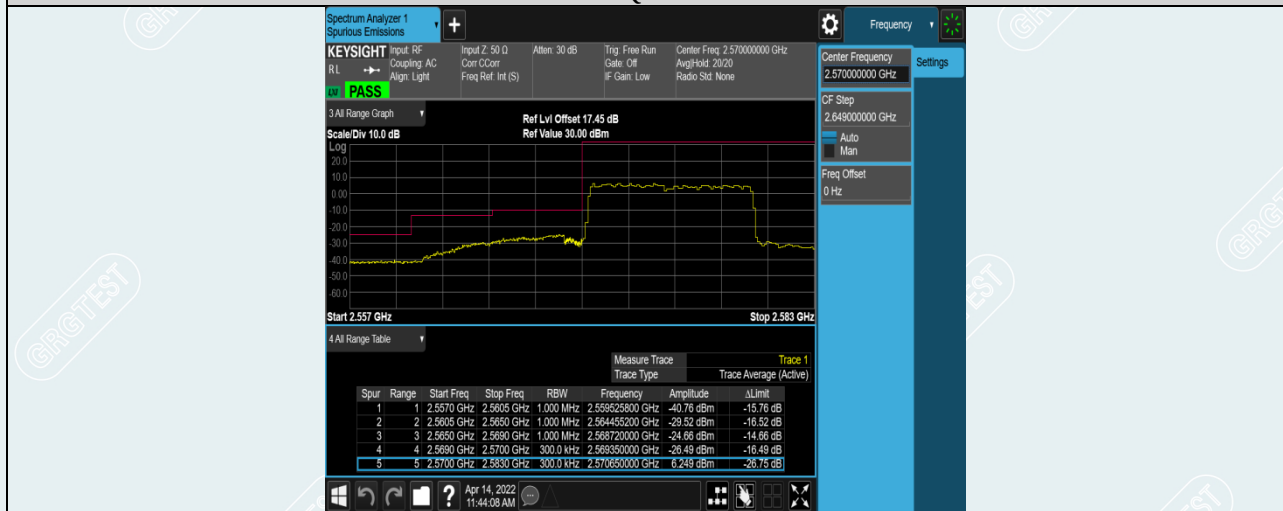
Band38-10MHz-QPSK-37800-50RB#0
