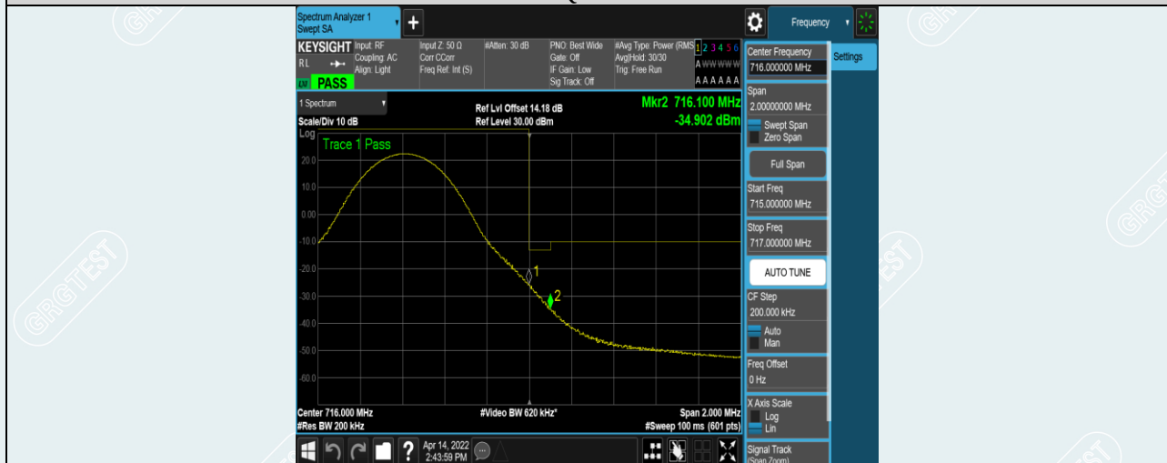
Band17-10MHz-QPSK-23800-1RB#49
