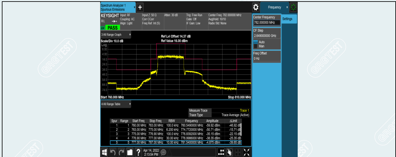
Band13-10MHz-16QAM-23230-50RB#0
