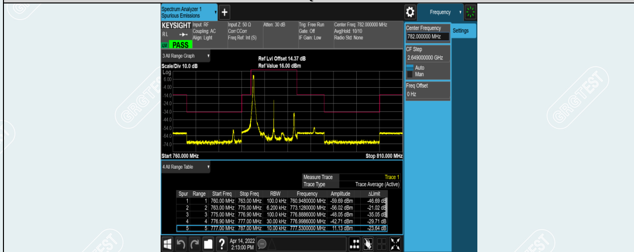
Band13-10MHz-16QAM-23230-1RB#0
