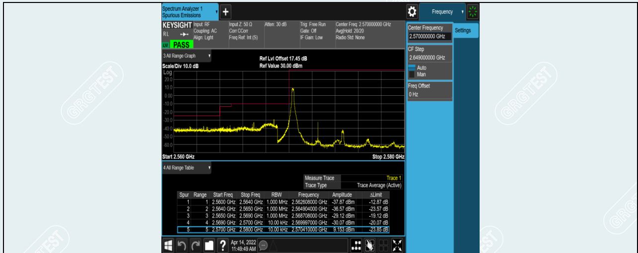
Band38-5MHz-16QAM-37775-1RB#0
