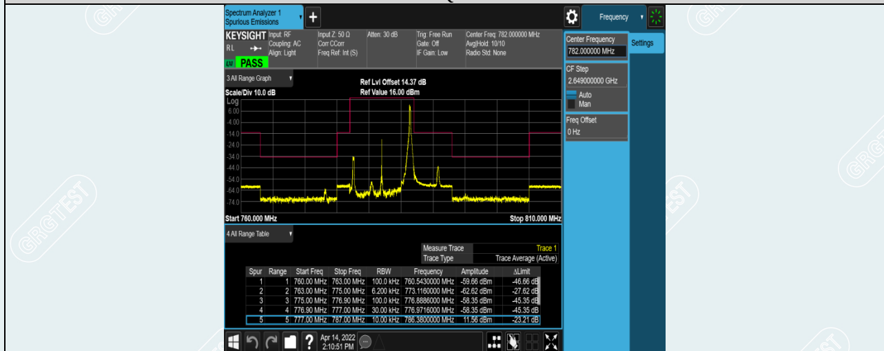
Band13-10MHz-16QAM-23230-1RB#49
