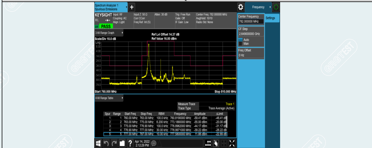
Band13-10MHz-QPSK-23230-1RB#0
