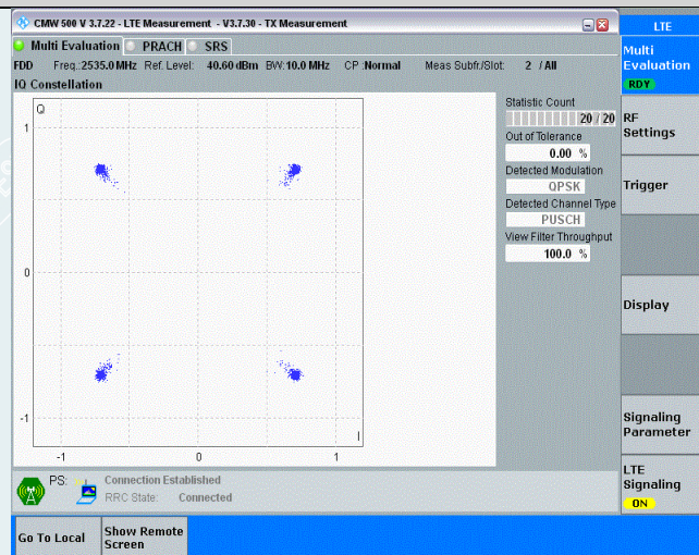
Band7-10MHz-QPSK-21100-50RB#0
