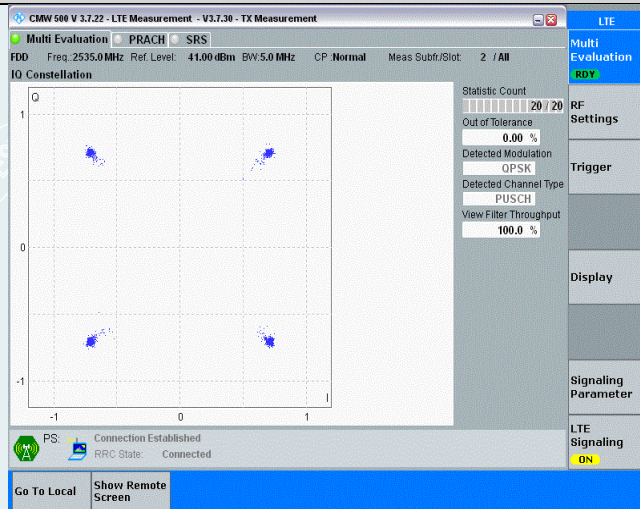
Band7-5MHz-QPSK-21100-25RB#0
