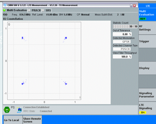
Band5-1.4MHz-QPSK-20525-6RB#0
