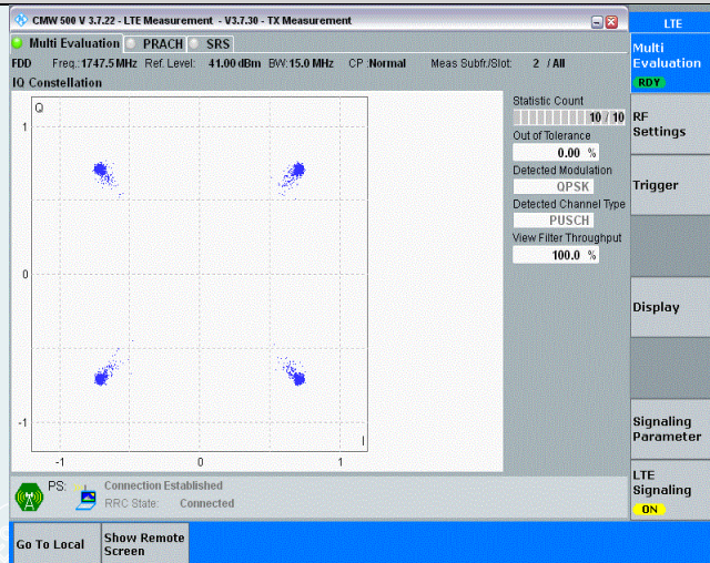
Band4-15MHz-QPSK-20325-75RB#0
