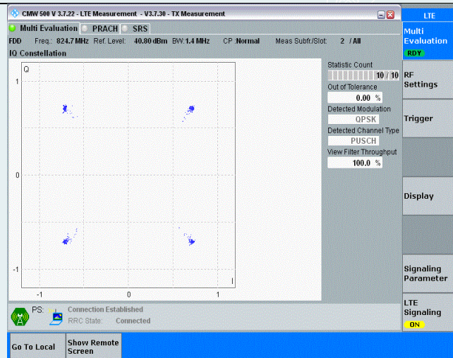
Band5-1.4MHz-QPSK-20407-6RB#0
