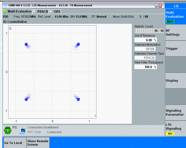
Band4-15MHz-QPSK-20175-75RB#0
