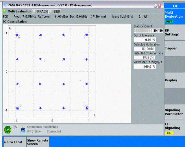
Band4-15MHz-16QAM-20325-75RB#0
