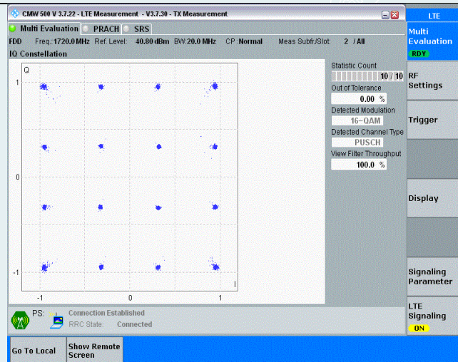
Band4-20MHz-16QAM-20050-100RB#0
