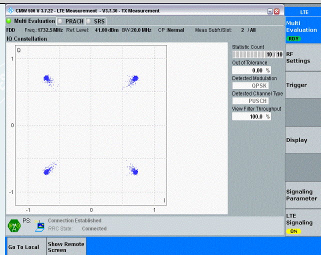
Band4-20MHz-QPSK-20175-100RB#0
