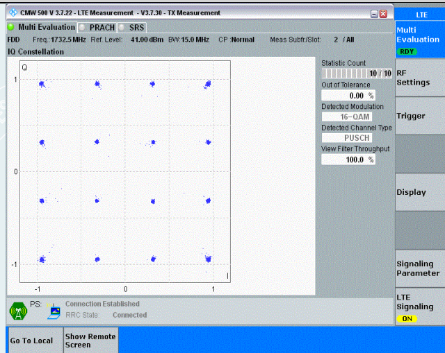
Band4-15MHz-16QAM-20175-75RB#0
