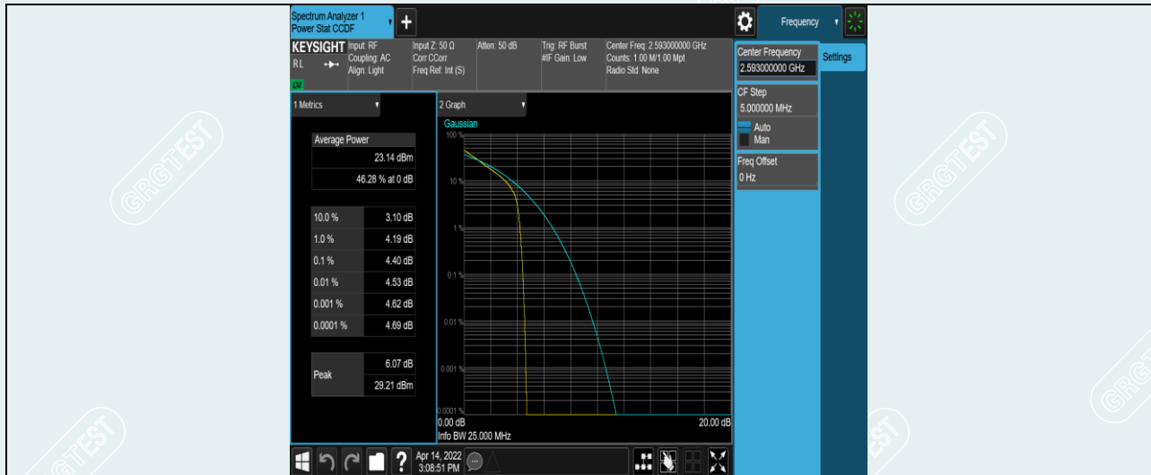
Band41-15MHz-QPSK-40620-75RB#0
