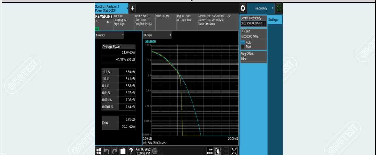
Band41-15MHz-16QAM-41515-75RB#0
