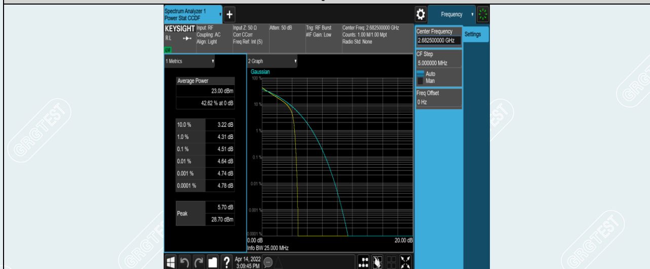
Band41-15MHz-QPSK-41515-75RB#0
