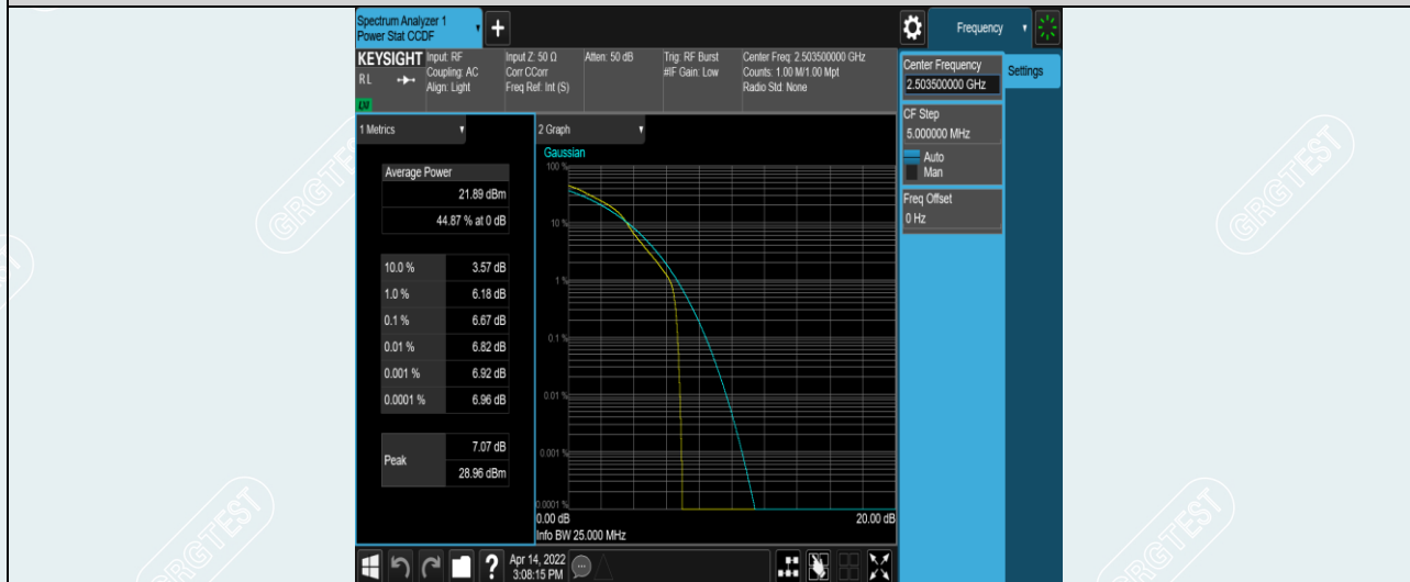
Band41-15MHz-16QAM-39725-75RB#0
