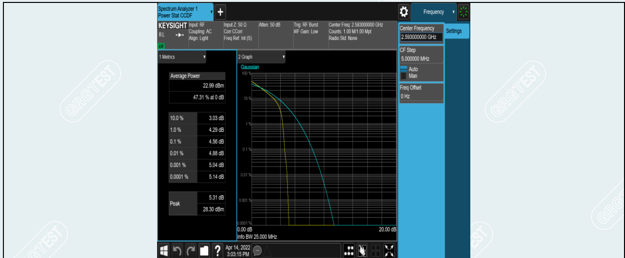
Band41-20MHz-QPSK-40620-100RB#0
