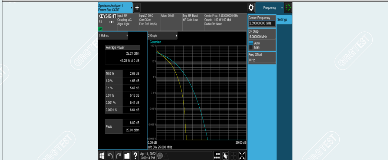
Band41-15MHz-QPSK-41515-1RB#0
