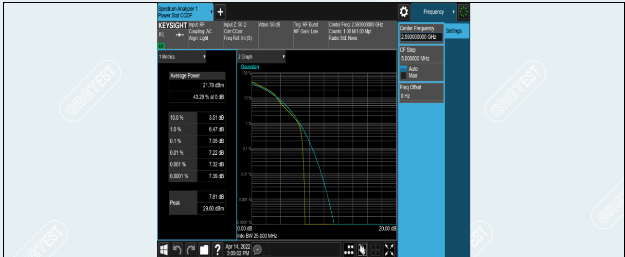
Band41-15MHz-16QAM-40620-75RB#0
