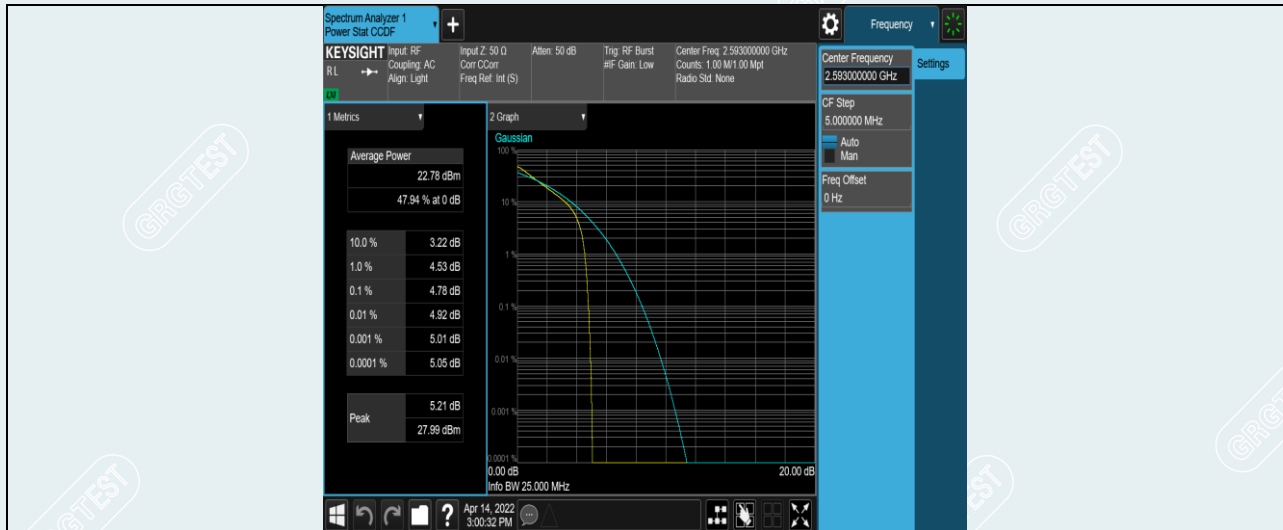
Band41-10MHz-QPSK-40620-50RB#0
