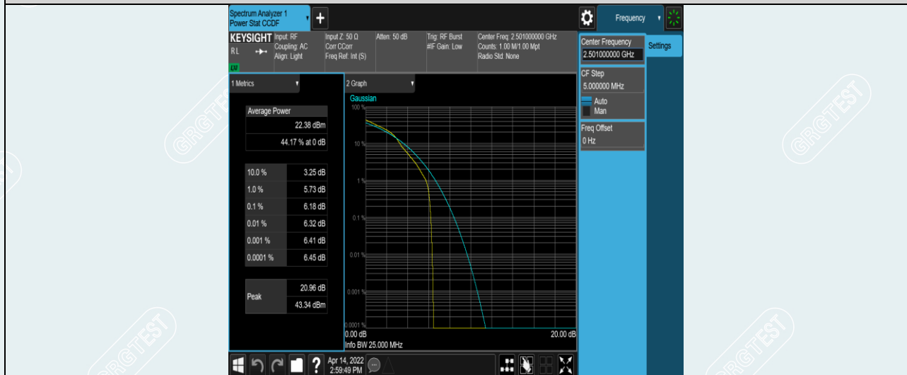
Band41-10MHz-16QAM-39700-50RB#0
