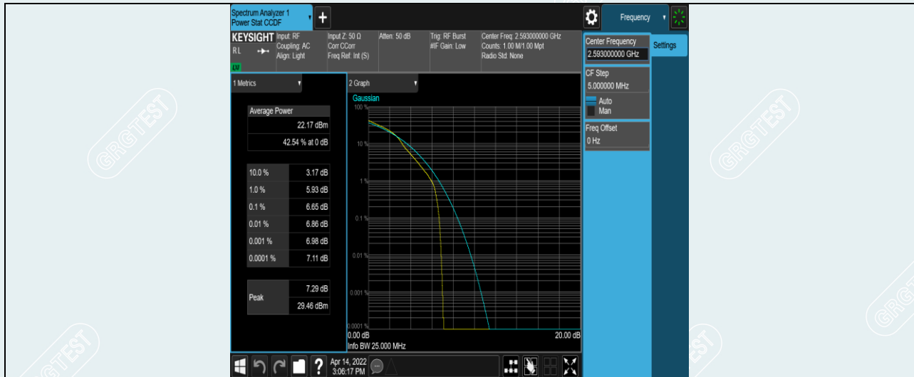
Band41-5MHz-16QAM-40620-25RB#0
