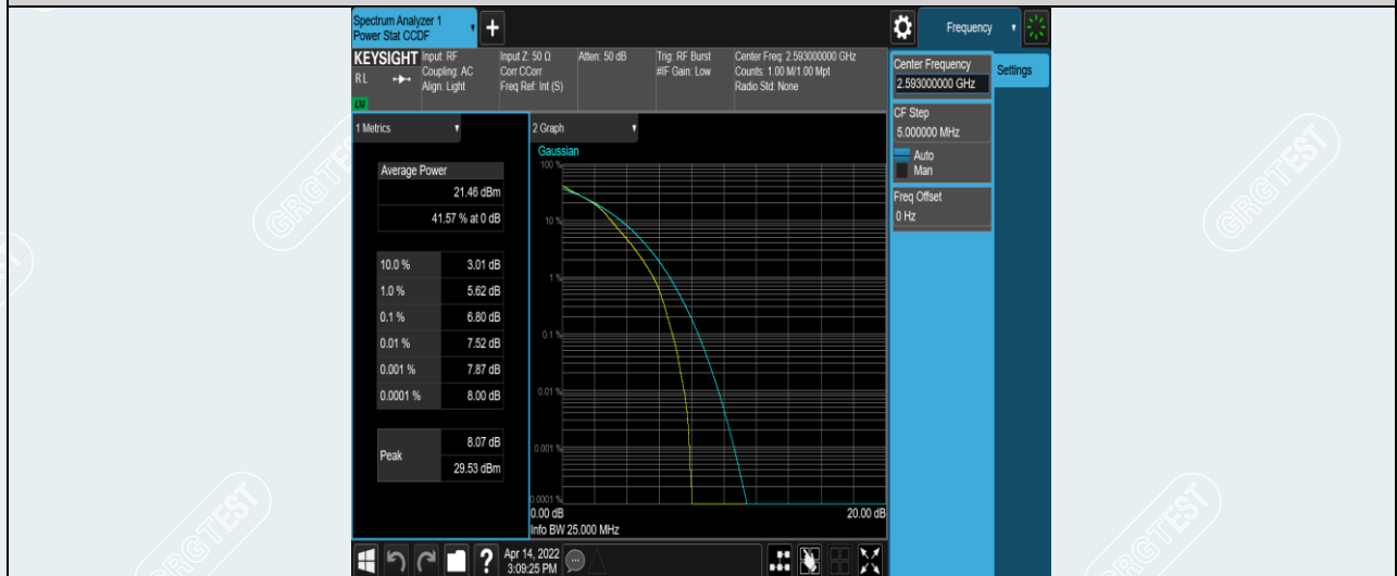
Band41-15MHz-16QAM-41515-1RB#0
