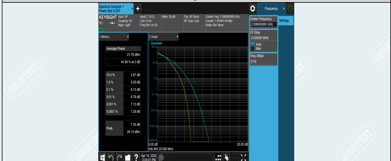
Band41-20MHz-16QAM-40620-1RB#0
