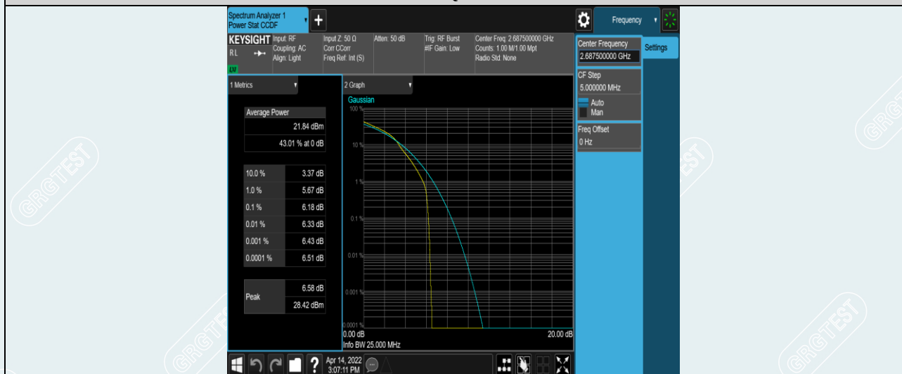
Band41-5MHz-16QAM-41565-25RB#0
