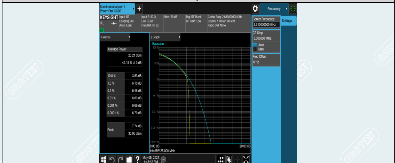
Band38-20MHz-16QAM-38150-1RB#0
