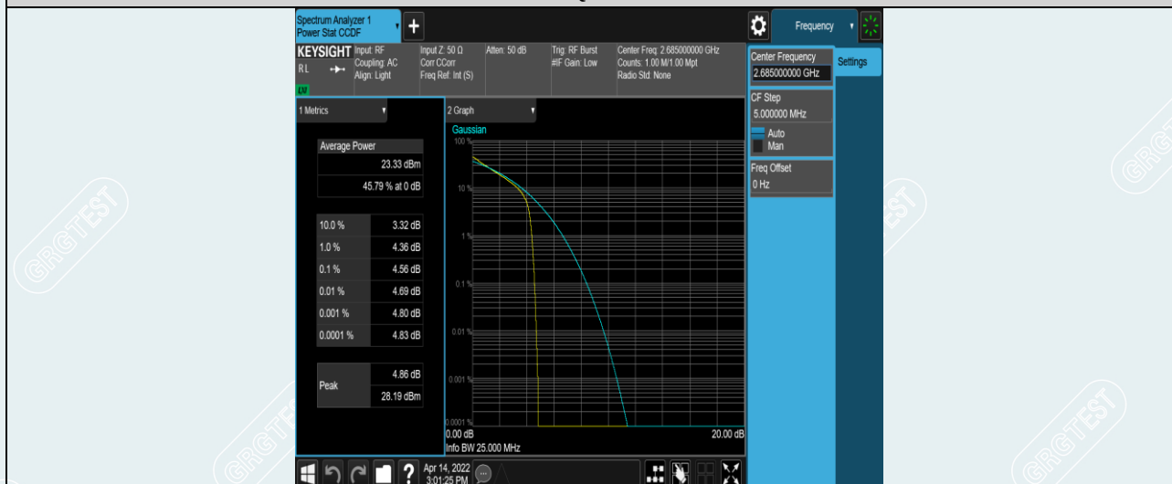
Band41-10MHz-QPSK-41540-50RB#0
