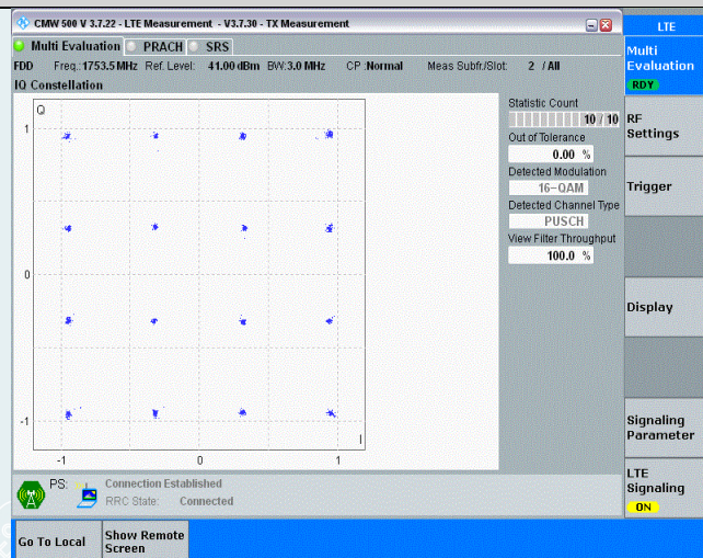
Band4-3MHz-16QAM-20385-15RB#0
