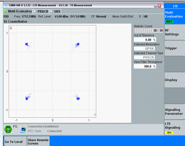
Band4-5MHz-QPSK-20375-25RB#0
