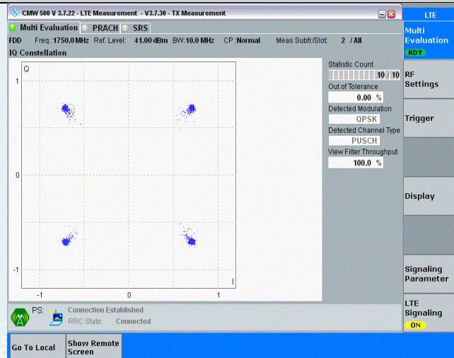
Band4-10MHz-QPSK-20350-50RB#0
