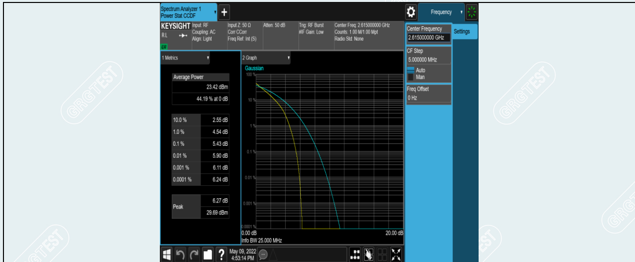
Band38-10MHz-QPSK-38200-50RB#0
