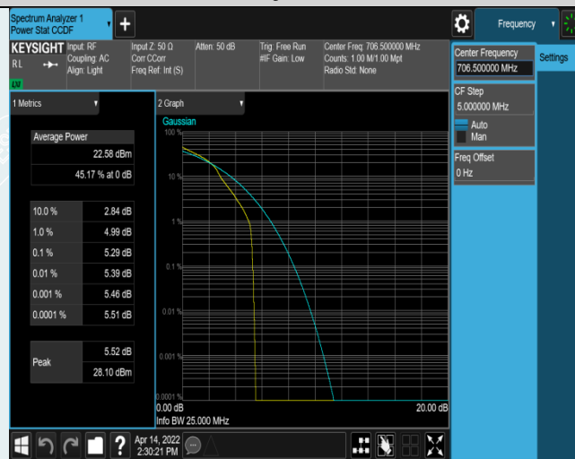
Band17-5MHz-16QAM-23755-1RB#0
