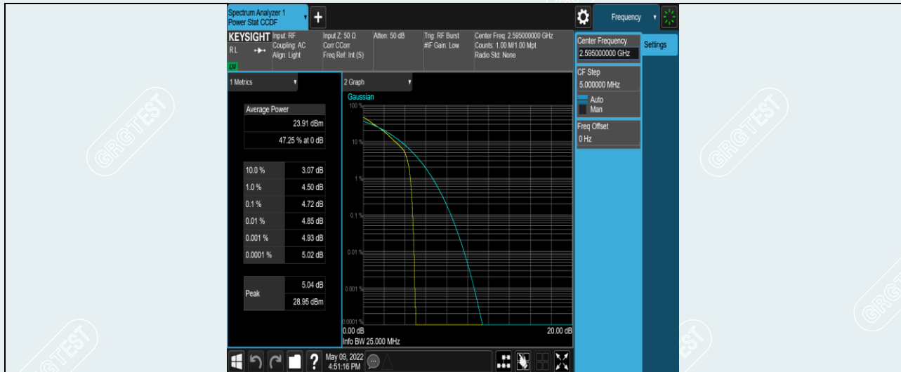
Band38-10MHz-QPSK-38000-1RB#0
