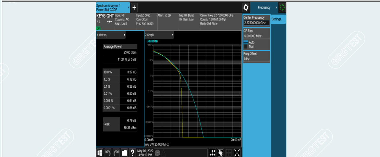
Band38-10MHz-16QAM-37800-1RB#0
