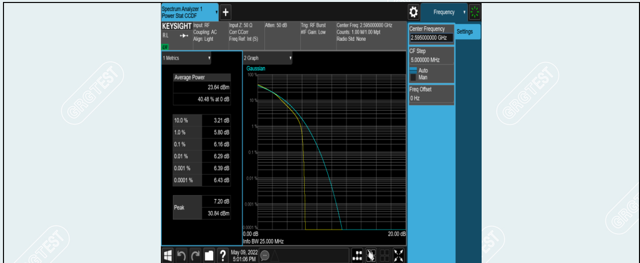
Band38-15MHz-16QAM-38000-1RB#0
