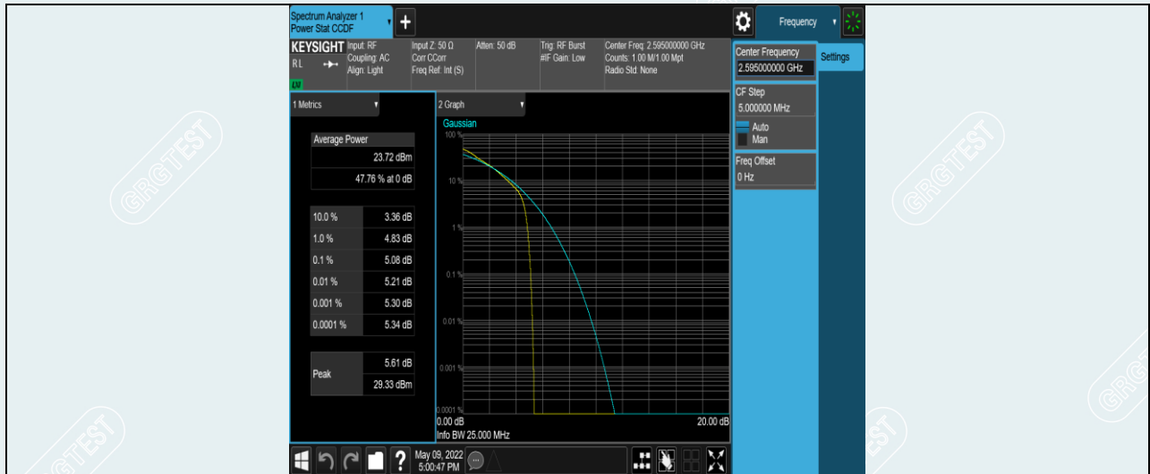
Band38-15MHz-QPSK-38000-1RB#0
