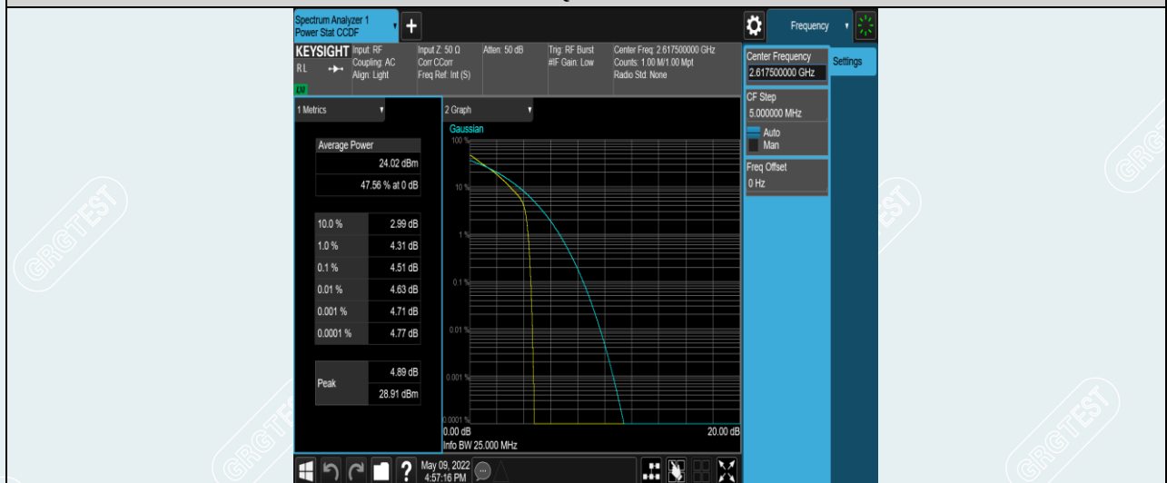
Band38-5MHz-QPSK-38225-1RB#0
