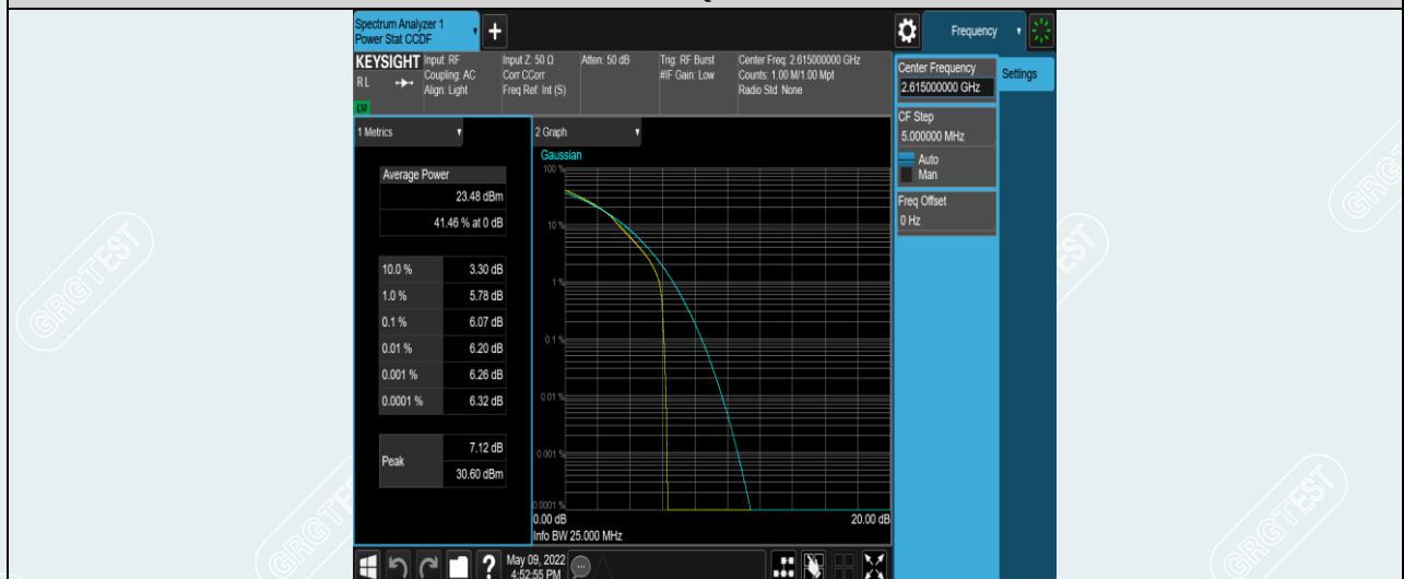
Band38-10MHz-16QAM-38200-1RB#0
