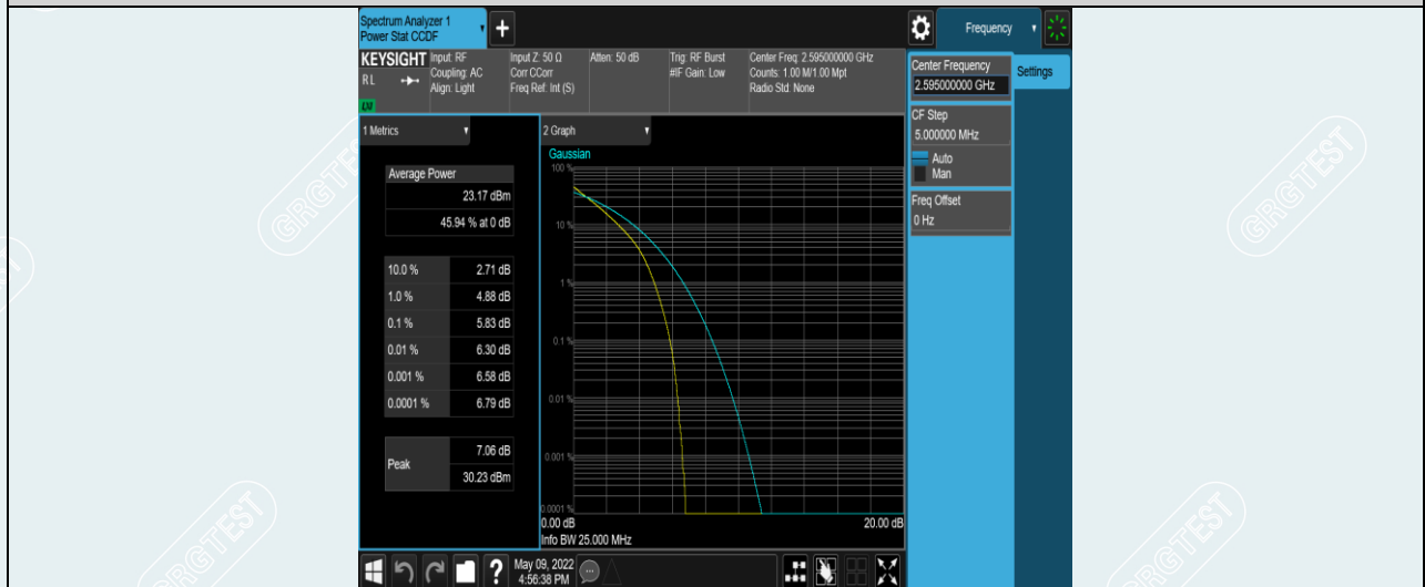
Band38-5MHz-QPSK-38000-25RB#0
