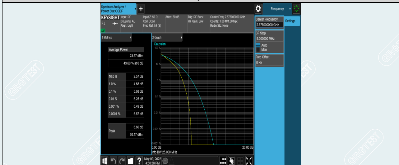
Band38-10MHz-QPSK-37800-50RB#0
