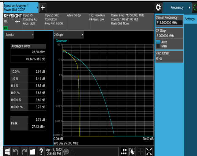
Band17-5MHz-QPSK-23825-1RB#0
