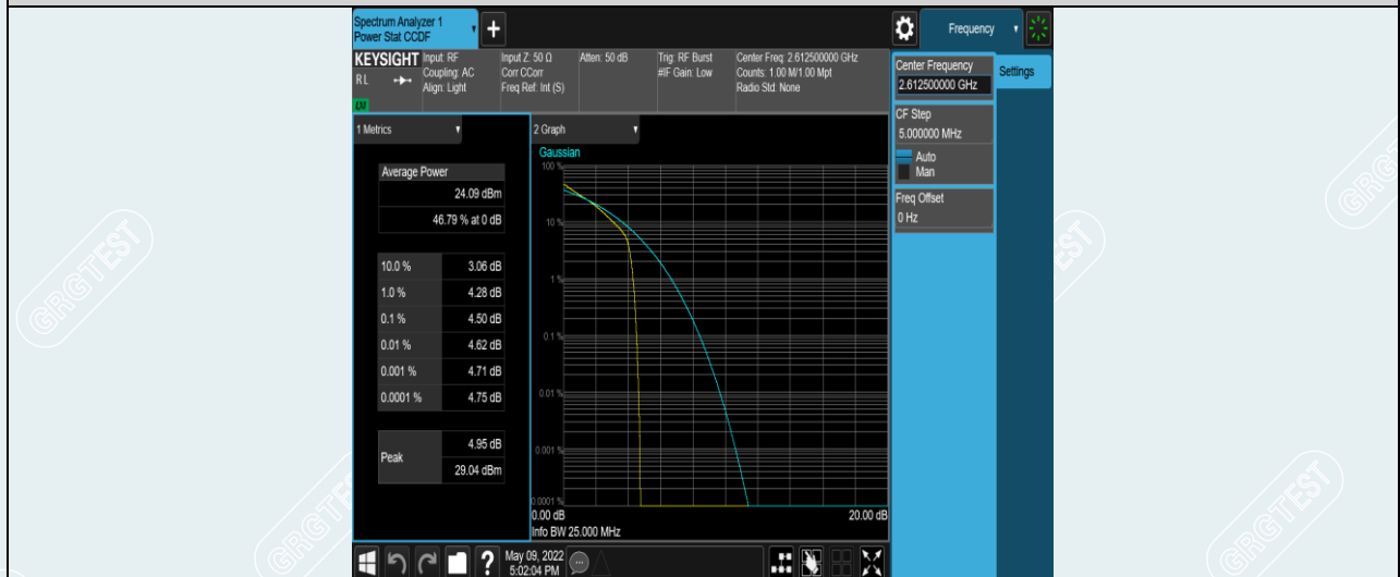
Band38-15MHz-QPSK-38175-1RB#0
