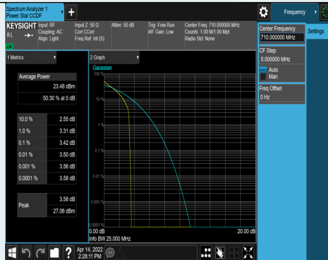
Band17-10MHz-QPSK-23790-1RB#0
