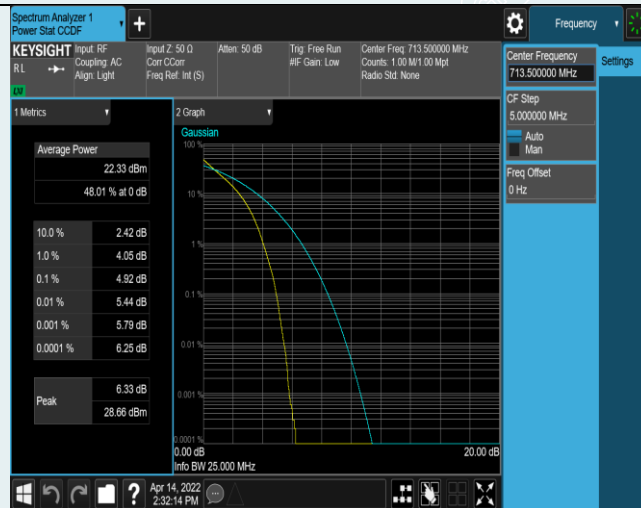
Band17-5MHz-QPSK-23825-25RB#0
