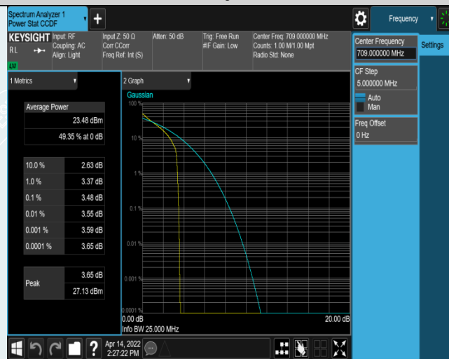
Band17-10MHz-QPSK-23780-1RB#0
