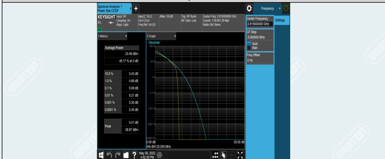
Band38-10MHz-QPSK-38200-1RB#0
