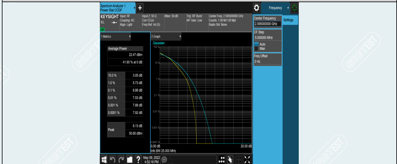
Band38-10MHz-16QAM-38000-50RB#0
