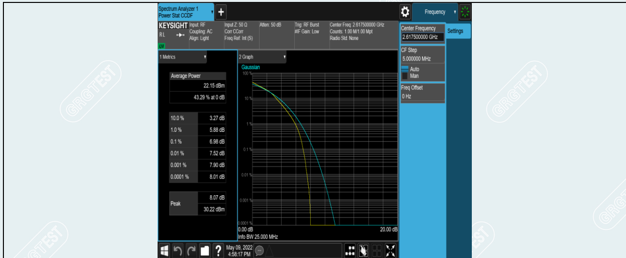
Band38-5MHz-16QAM-38225-25RB#0
