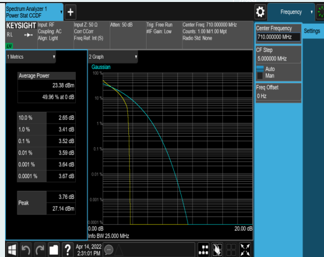
Band17-5MHz-QPSK-23790-1RB#0
