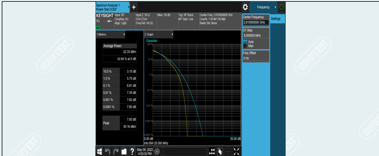
Band38-10MHz-16QAM-38200-50RB#0
