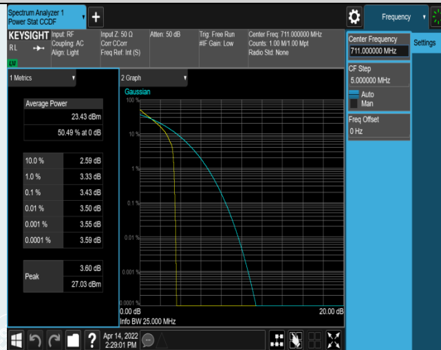
Band17-10MHz-QPSK-23800-1RB#0
