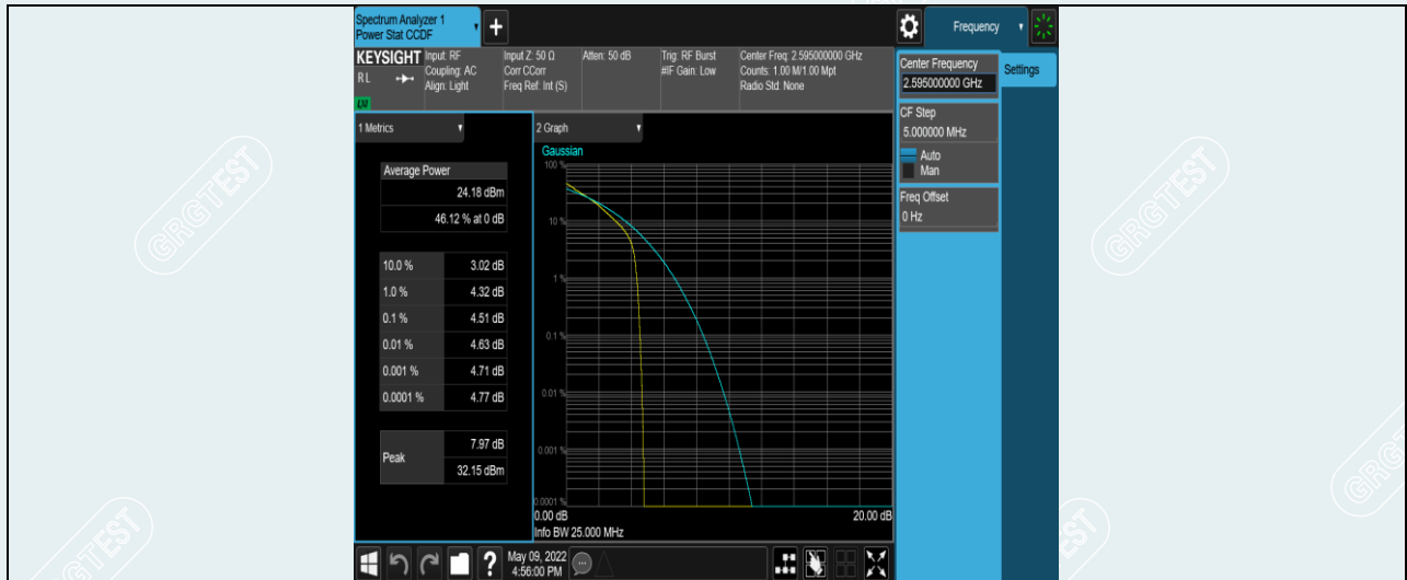
Band38-5MHz-QPSK-38000-1RB#0
