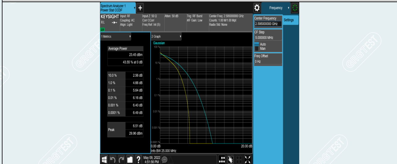
Band38-10MHz-QPSK-38000-50RB#0
