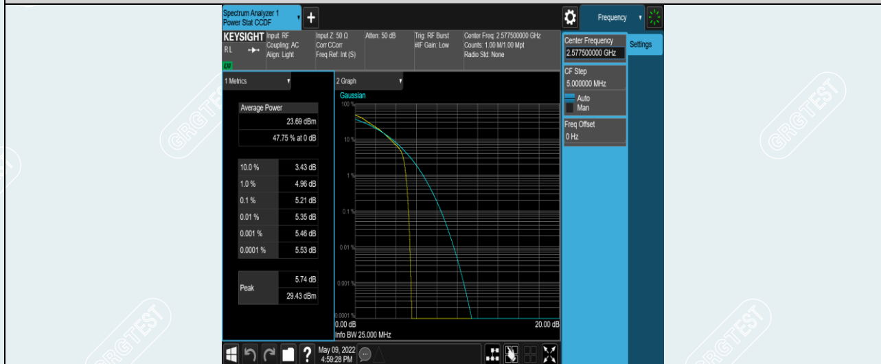
Band38-15MHz-QPSK-37825-1RB#0
