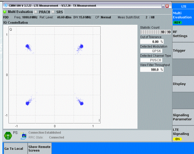
Band2-15MHz-QPSK-18900-75RB#0
