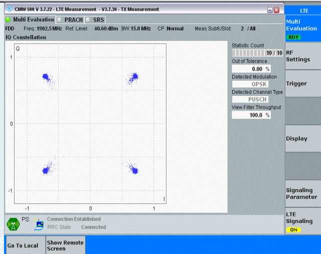
Band2-15MHz-QPSK-19125-75RB#0
