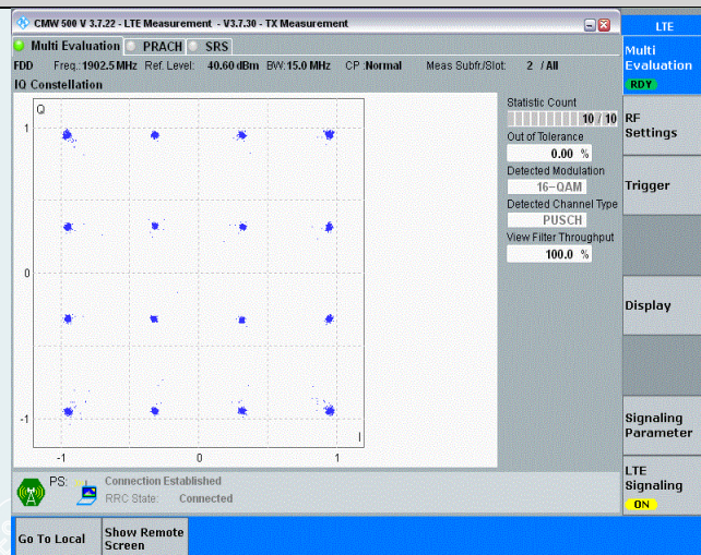
Band2-15MHz-16QAM-19125-75RB#0
