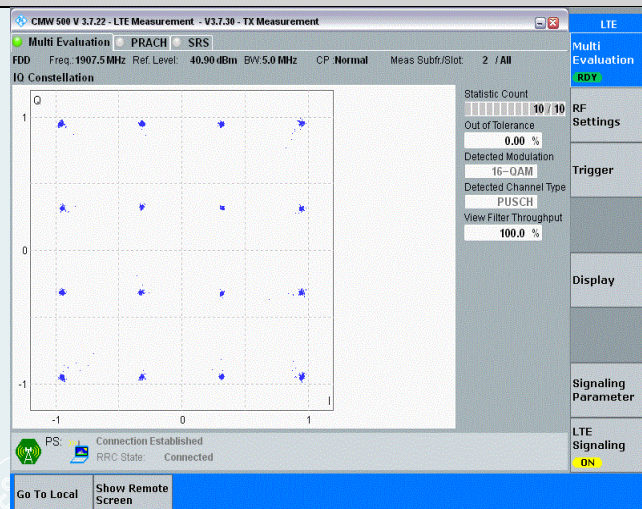
Band2-5MHz-16QAM-19175-25RB#0
