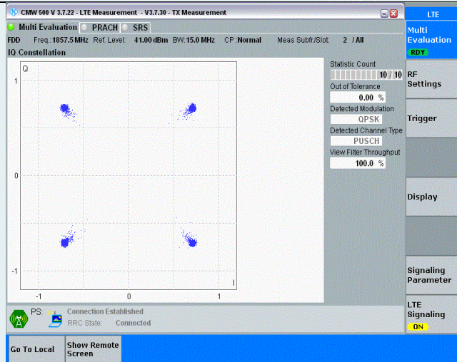
Band2-15MHz-QPSK-18675-75RB#0
