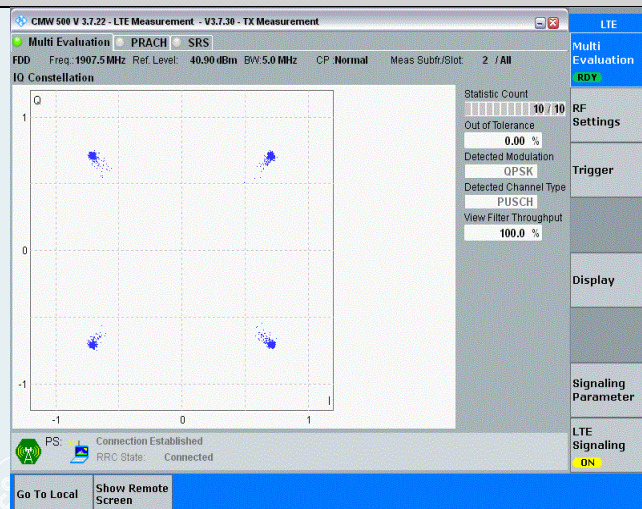
Band2-5MHz-QPSK-19175-25RB#0
