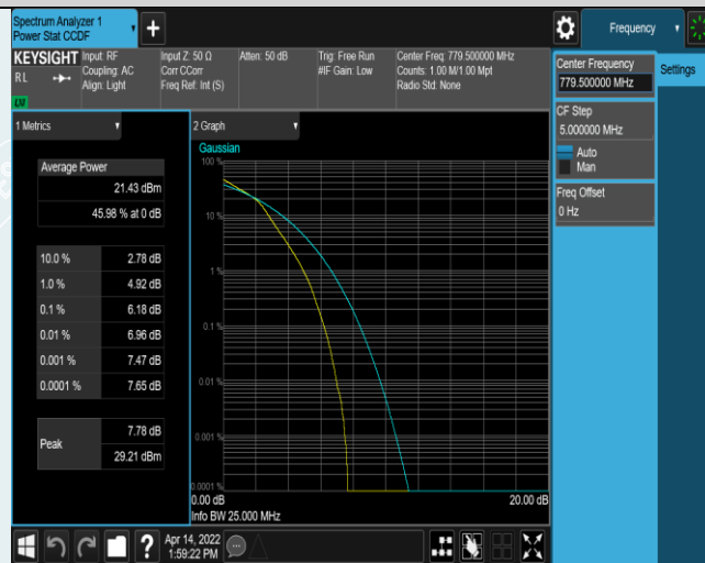
Band13-5MHz-16QAM-23205-25RB#0
