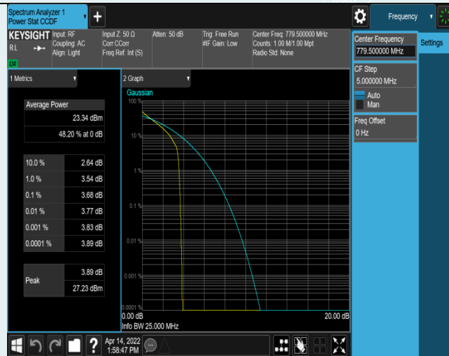
Band13-5MHz-QPSK-23205-1RB#0
