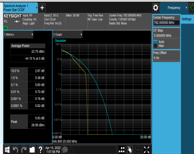
Band13-10MHz-16QAM-23230-1RB#0
