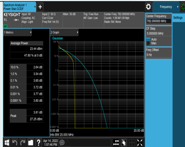
Band13-10MHz-QPSK-23230-1RB#0
