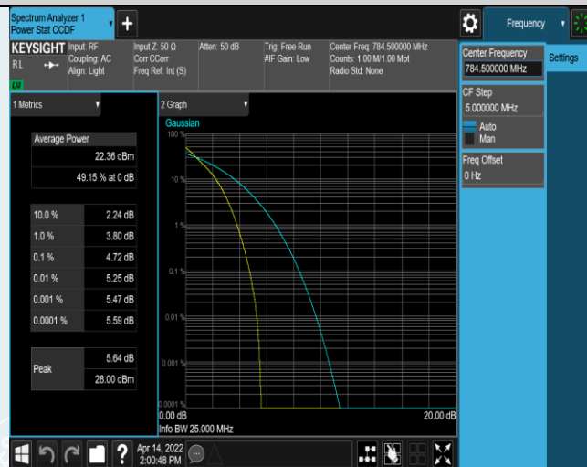
Band13-5MHz-QPSK-23255-25RB#0
