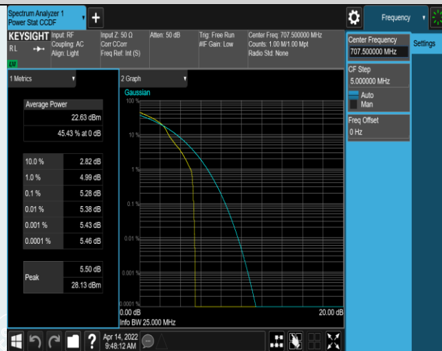
Band12-10MHz-16QAM-23095-1RB#0
