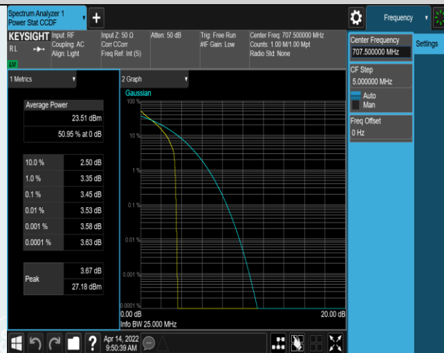
Band12-3MHz-QPSK-23095-1RB#0
