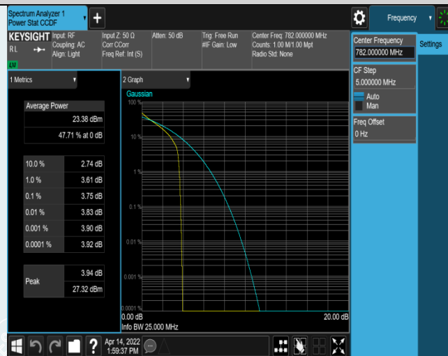
Band13-5MHz-QPSK-23230-1RB#0
