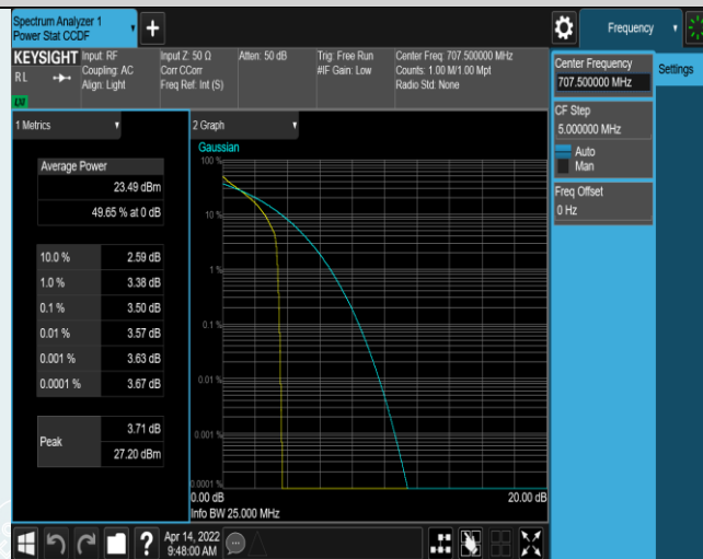
Band12-10MHz-QPSK-23095-1RB#0
