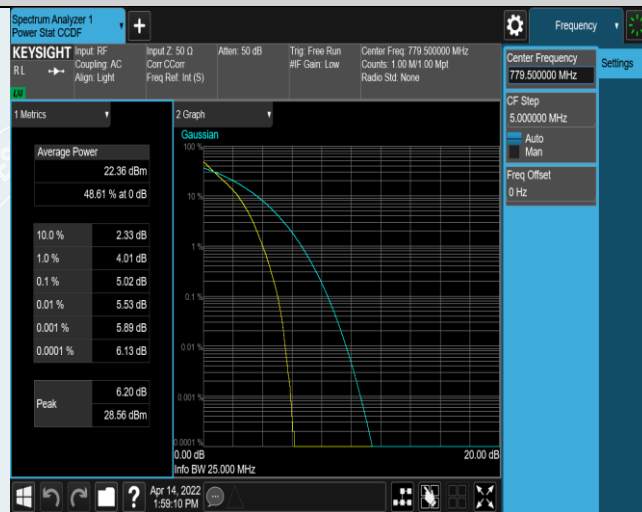
Band13-5MHz-QPSK-23205-25RB#0
