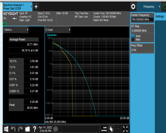
Band13-5MHz-16QAM-23255-1RB#0
