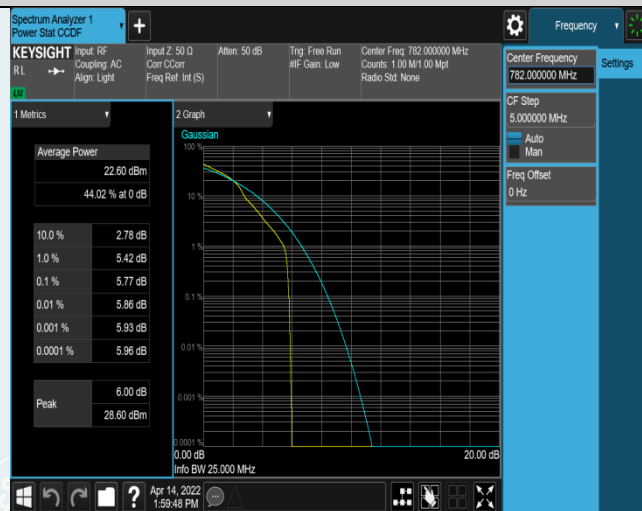
Band13-5MHz-16QAM-23230-1RB#0
