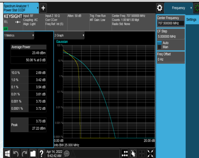
Band12-5MHz-QPSK-23095-1RB#0
