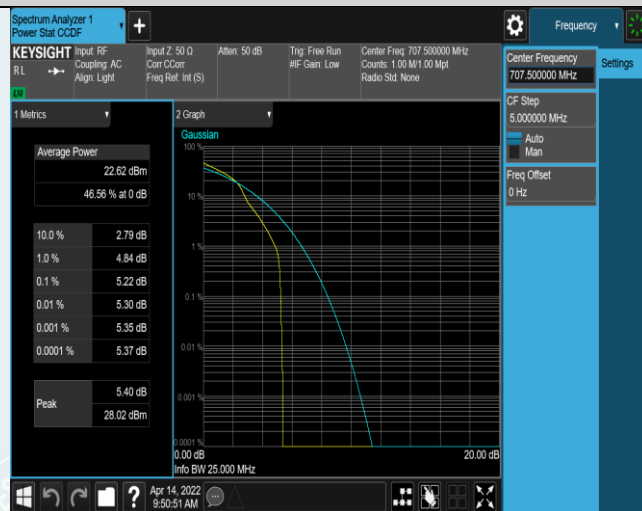
Band12-3MHz-16QAM-23095-1RB#0
