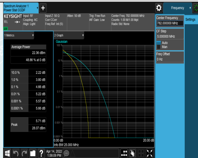
Band13-10MHz-QPSK-23230-50RB#0
