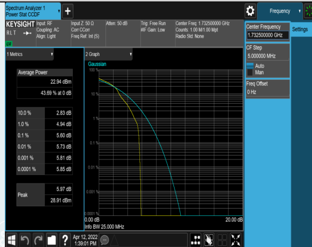
Band4-3MHz-16QAM-20175-1RB#0
