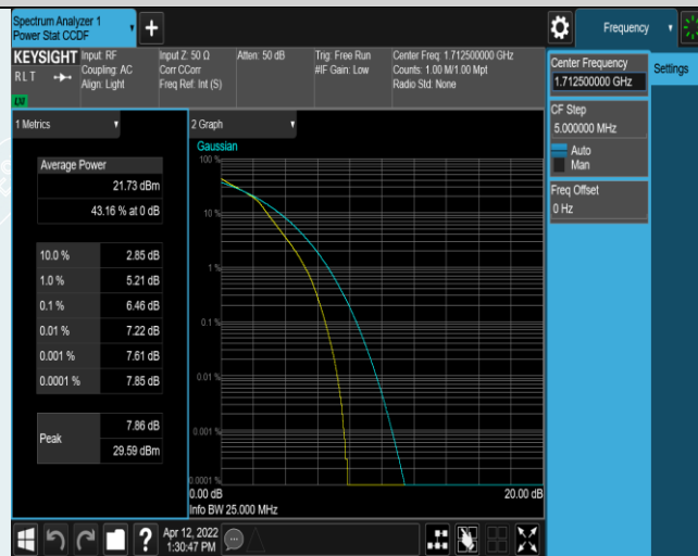
Band4-5MHz-16QAM-19975-25RB#0
