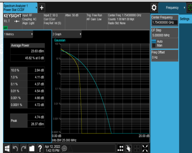
Band4-1.4MHz-QPSK-20393-1RB#0
