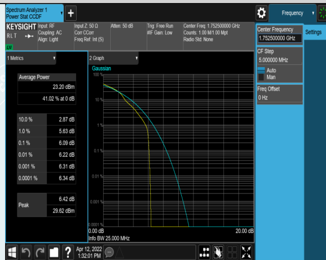
Band4-5MHz-16QAM-20375-1RB#0
