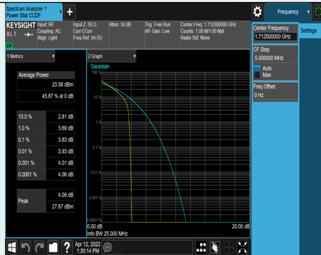
Band4-5MHz-QPSK-19975-1RB#0
