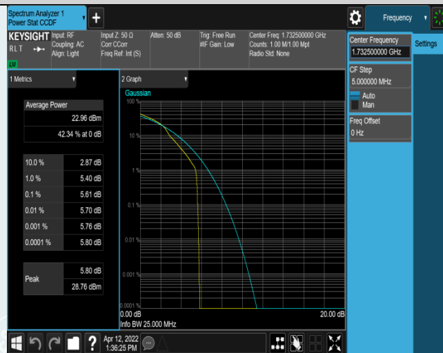
Band4-15MHz-16QAM-20175-1RB#0
