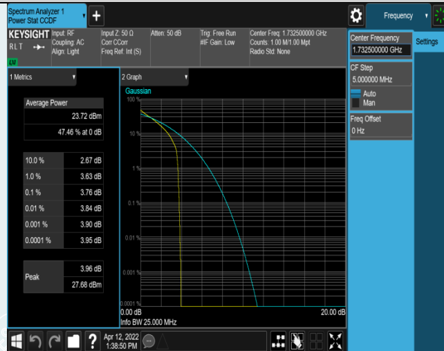
Band4-3MHz-QPSK-20175-1RB#0
