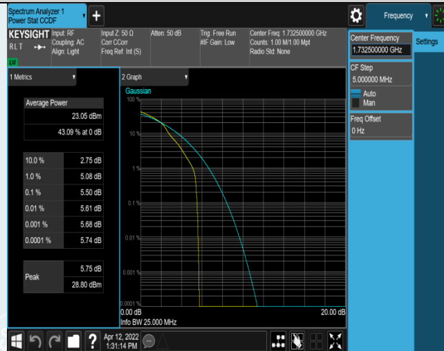
Band4-5MHz-16QAM-20175-1RB#0
