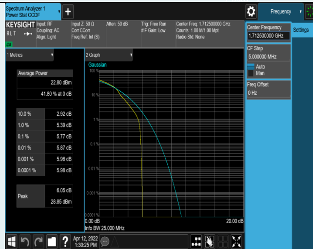
Band4-5MHz-16QAM-19975-1RB#0
