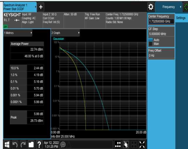
Band4-5MHz-QPSK-20175-25RB#0
