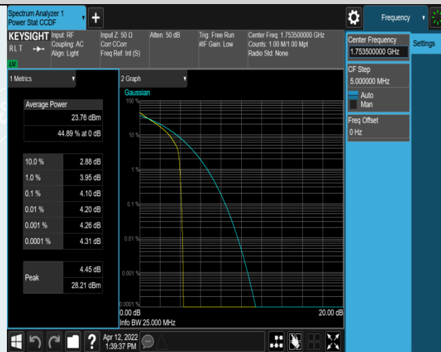
Band4-3MHz-QPSK-20385-1RB#0
