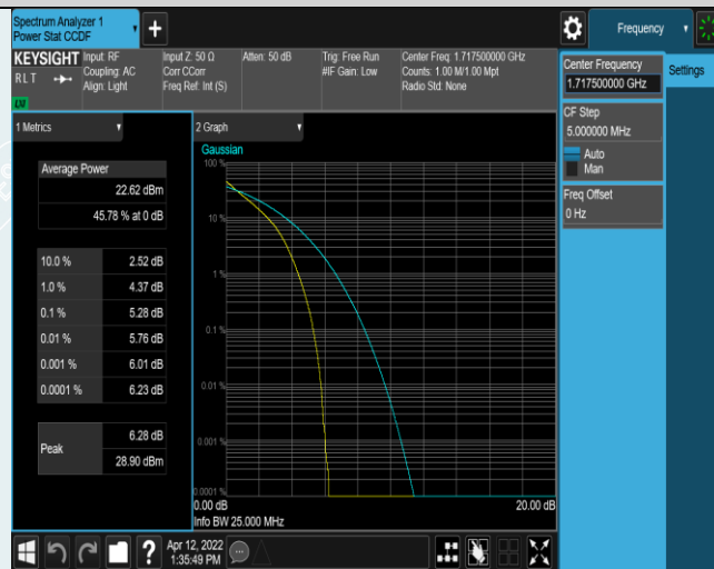
Band4-15MHz-QPSK-20025-75RB#0
