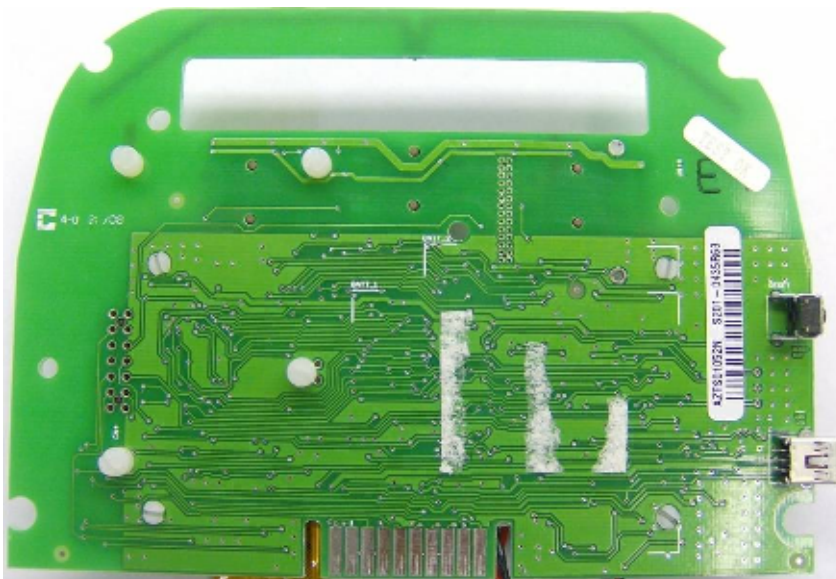
Solder side
