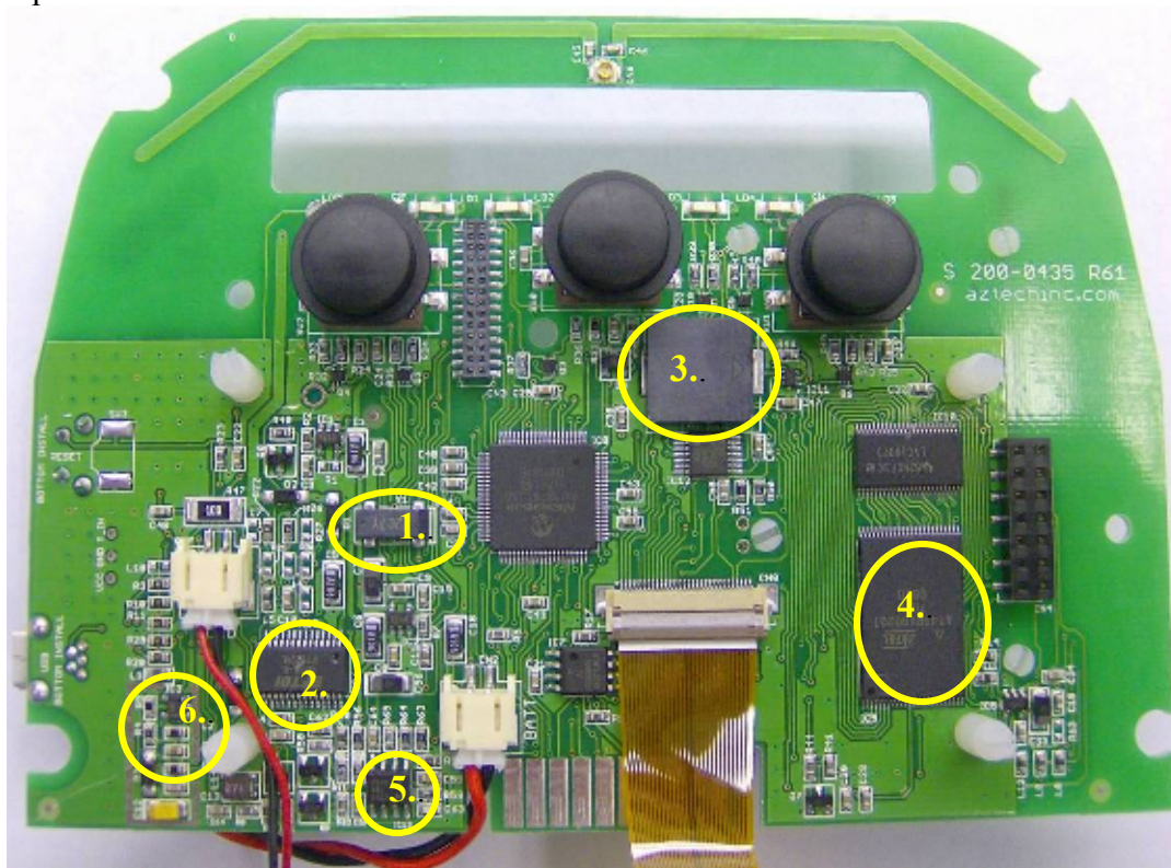
Component Side
