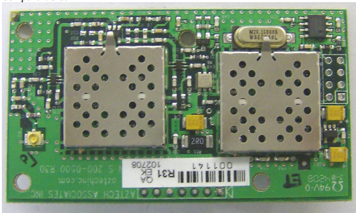
Component Side
