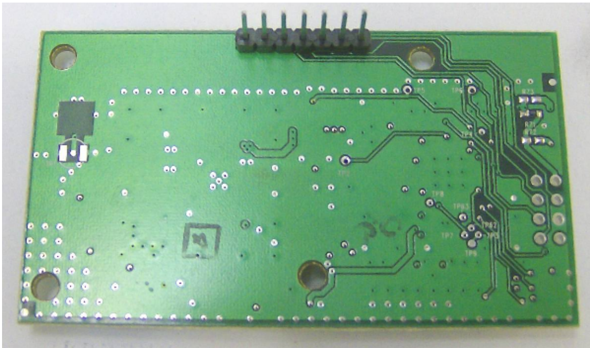
Solder Side
