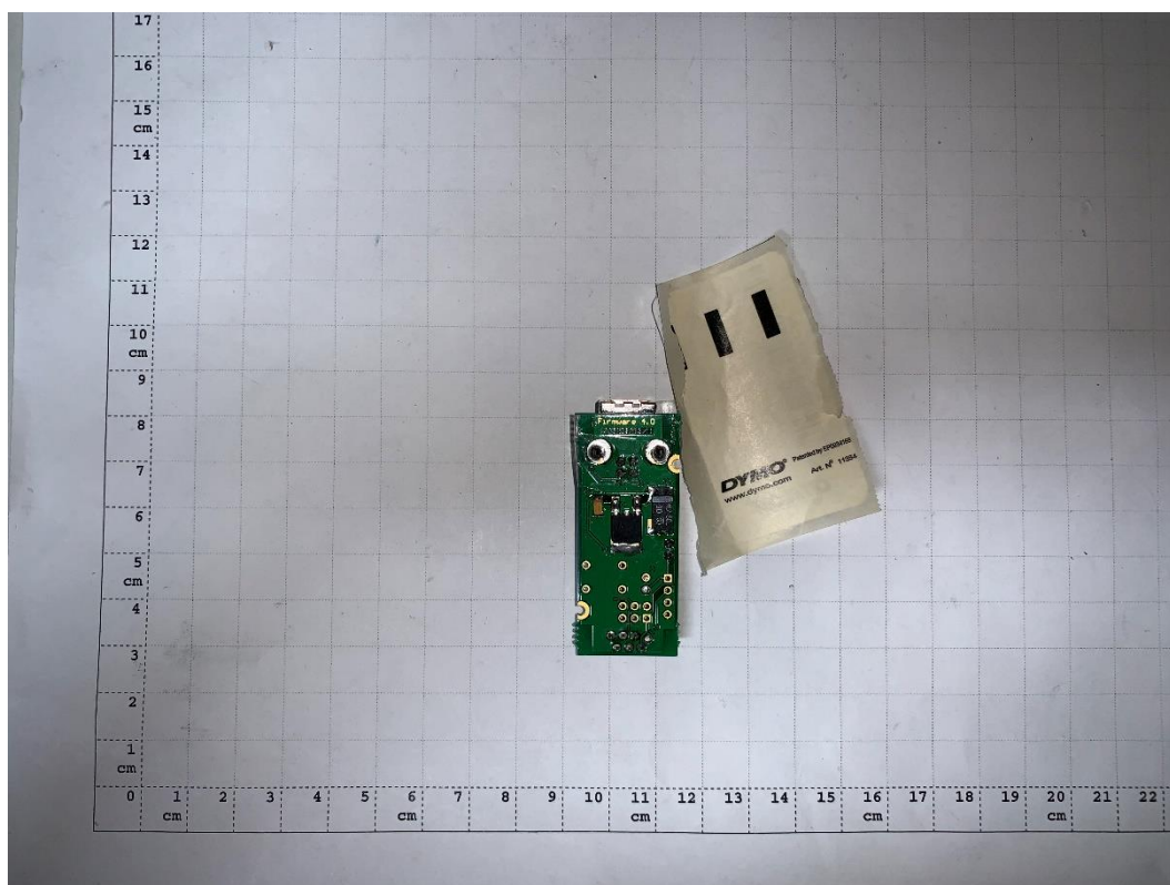
Photograph 23: AE 7, bottom side
