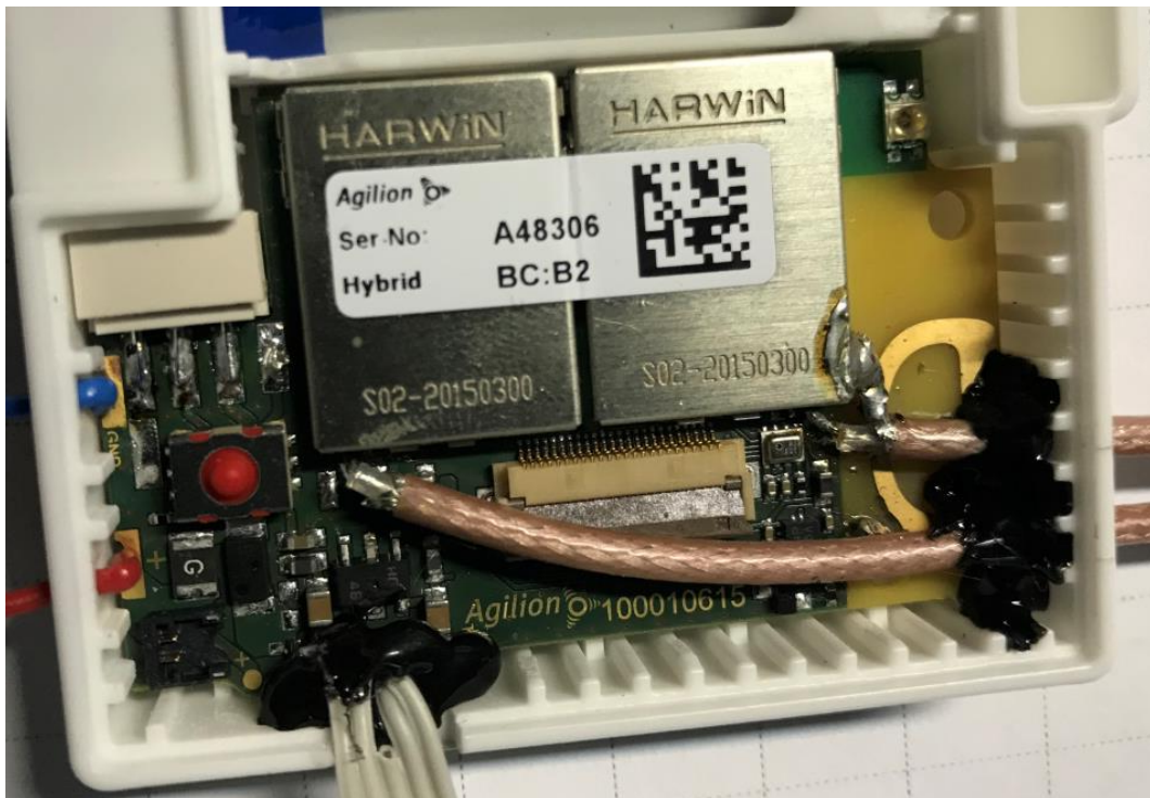
Photograph 5: : EUT B, front close view, circuit board
