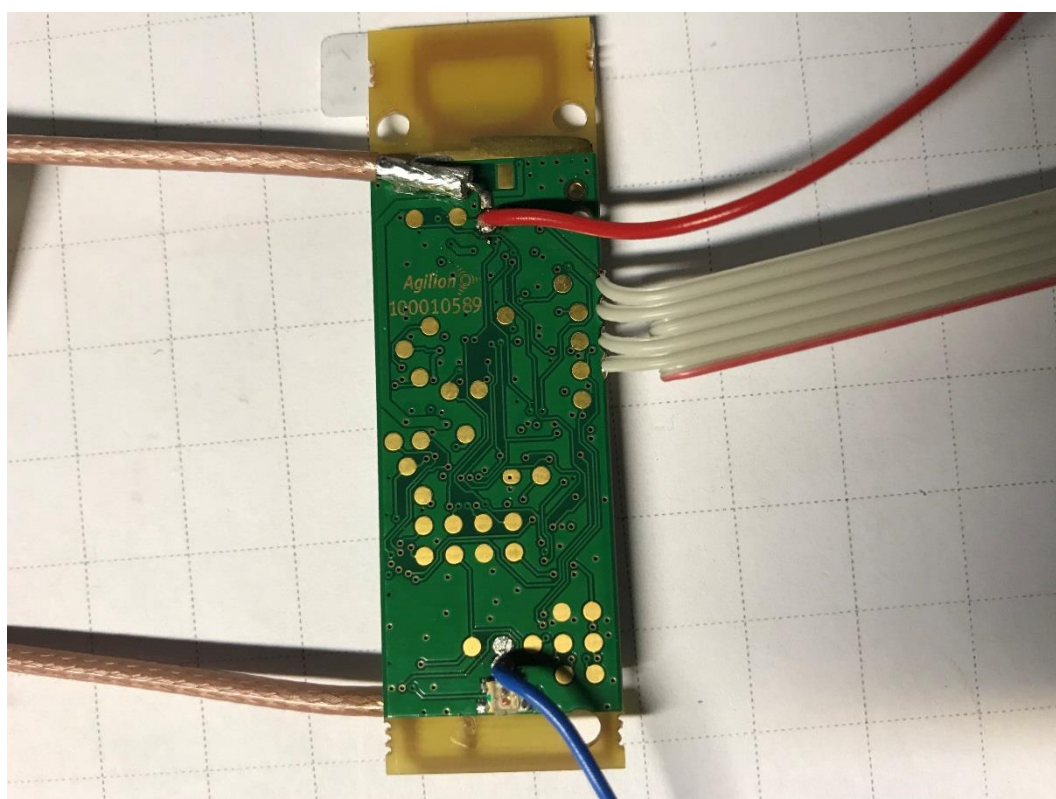
Photograph 2: EUT B, rear-view
