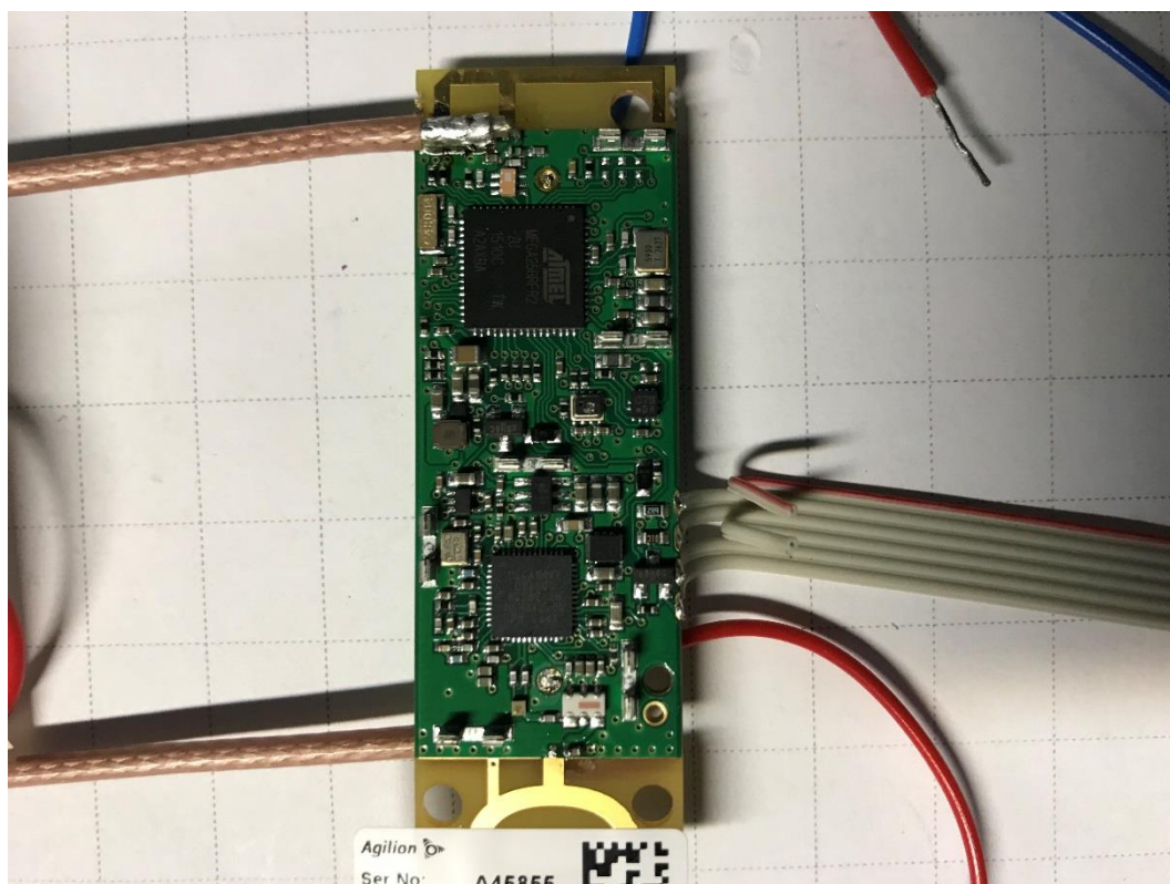
Photograph 1: EUT B, front-view, bottom- UWB antenna, top- 2.4 GHz antenna
