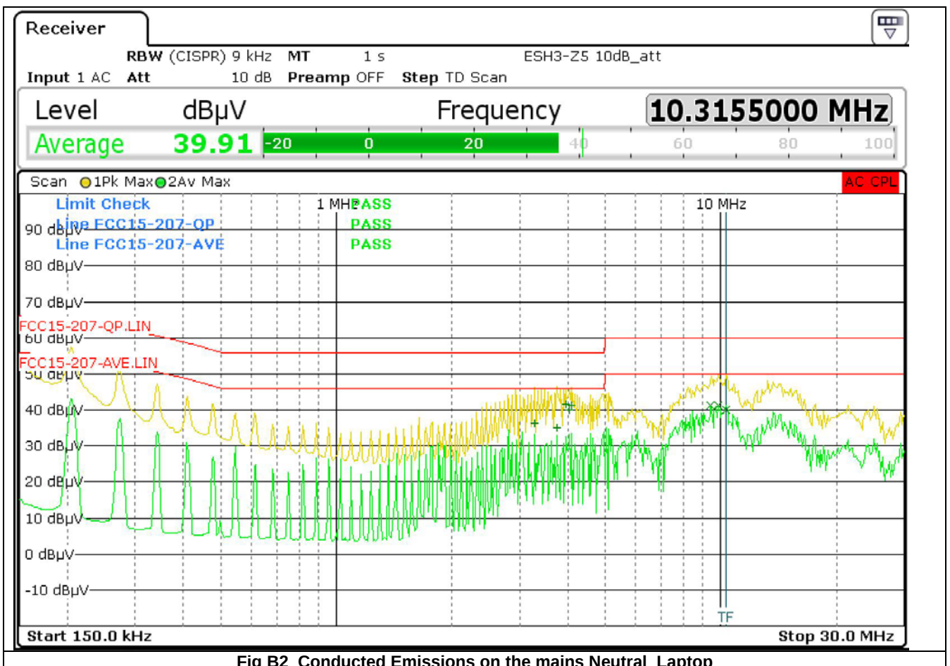
Fig B2 Conducted Emissions on the mains Neutral Laptop
