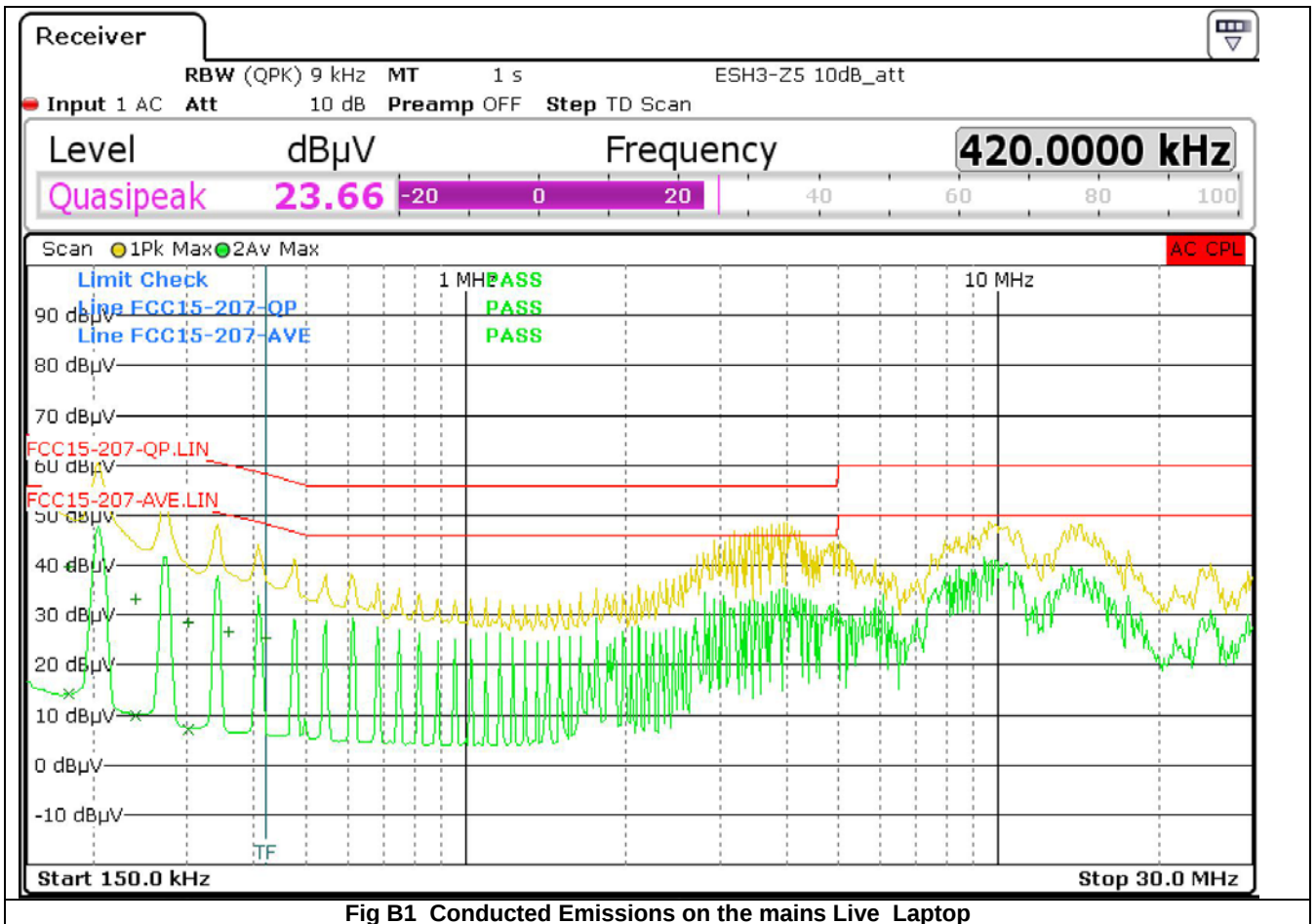
Fig B1 Conducted Emissions on the mains Live Laptop
