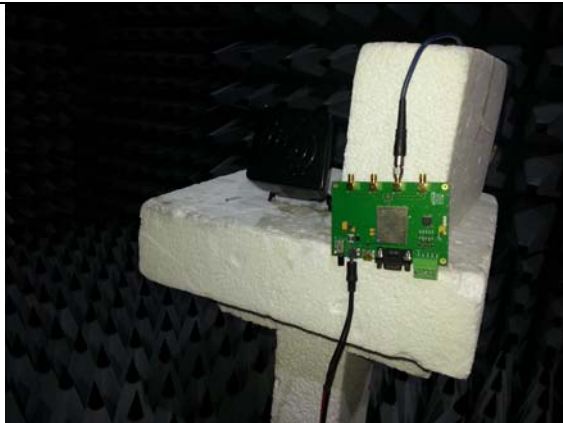
Fig B5 Radiated Emissions
