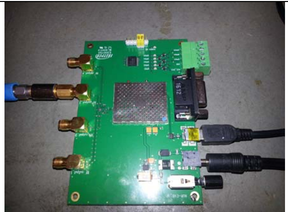
Fig D2 Conducted Emissions antenna port
