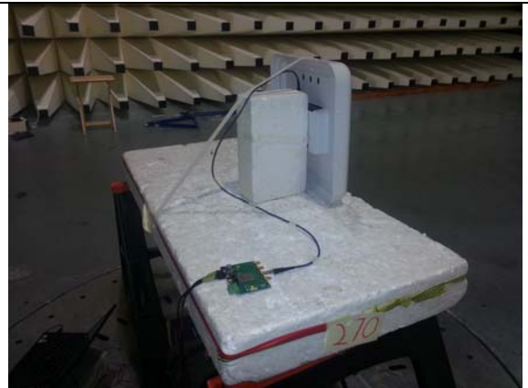
Fig C2 Radiated Emissions
