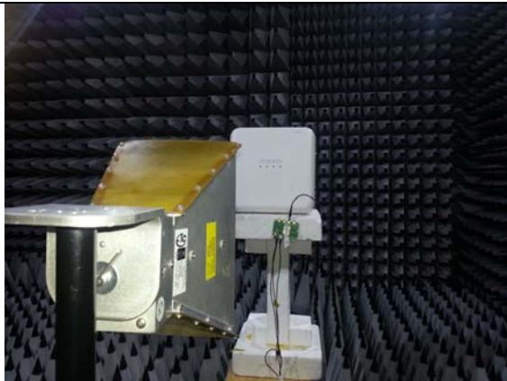
Fig C5 Radiated Emissions
