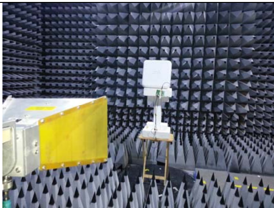
Fig C3 Radiated Emissions
