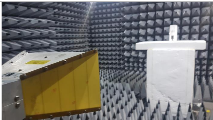
Fig A9 Radiated Emissions above 1GHz
