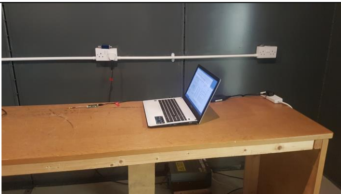
Fig B3 Conducted Emissions mains Laptop
