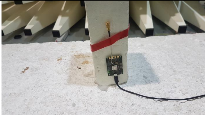
Fig A5 Radiated Emissions EUT close up antenna port terminated
