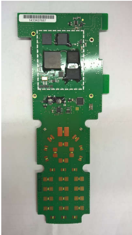
Picture 10. Merlin 805-2C main board top.
