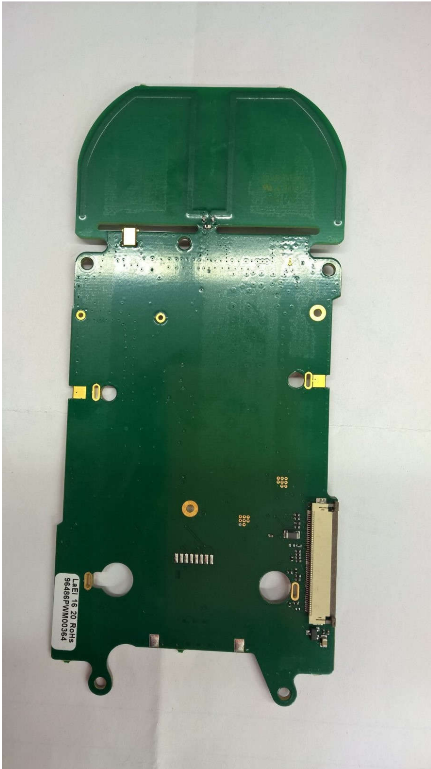
Picture 15. Merlin 805-2C MOD board bottom.
