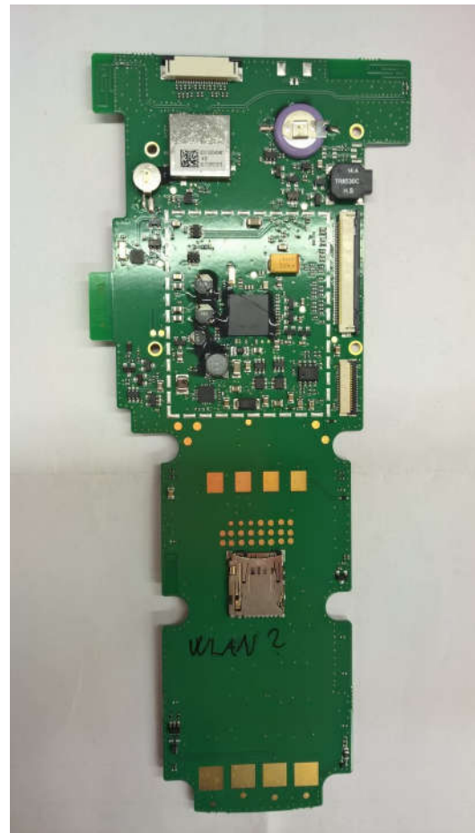
Picture 11. Merlin 805-2C main board bottom.
