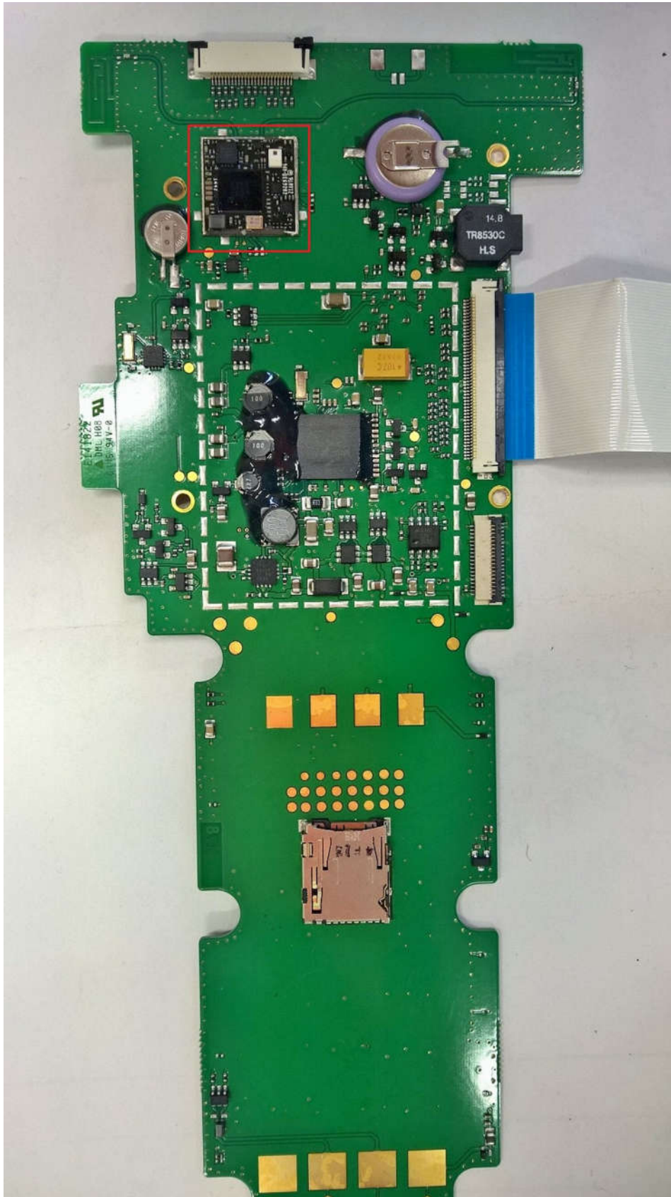
Picture 13. SDC-SSD40NBT module without shield.
