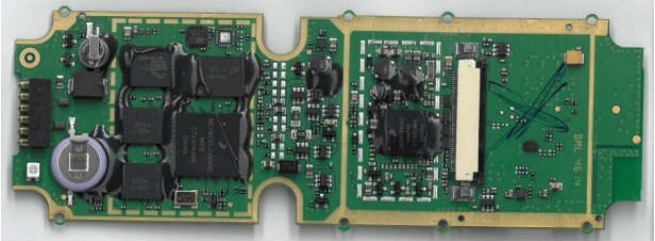
Picture 2: CPU811 board bottom side
