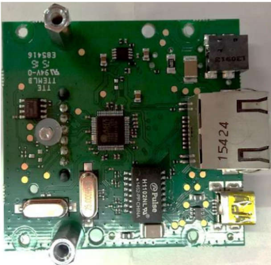
Picture 16: DTC811 board bottom side
