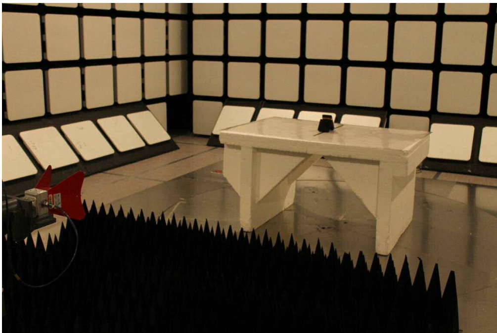
Photograph 2. Radiated Spurious Emissions 1 – 10 GHz
