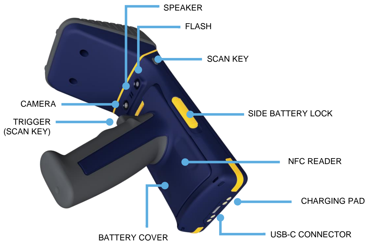
Figure 1-7. Brady HH86 features (back)
