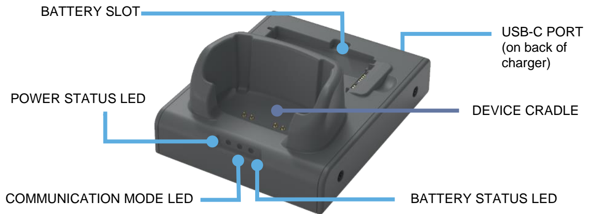
Figure 1-12. Brady HH83 Desktop Charger (single bay)
