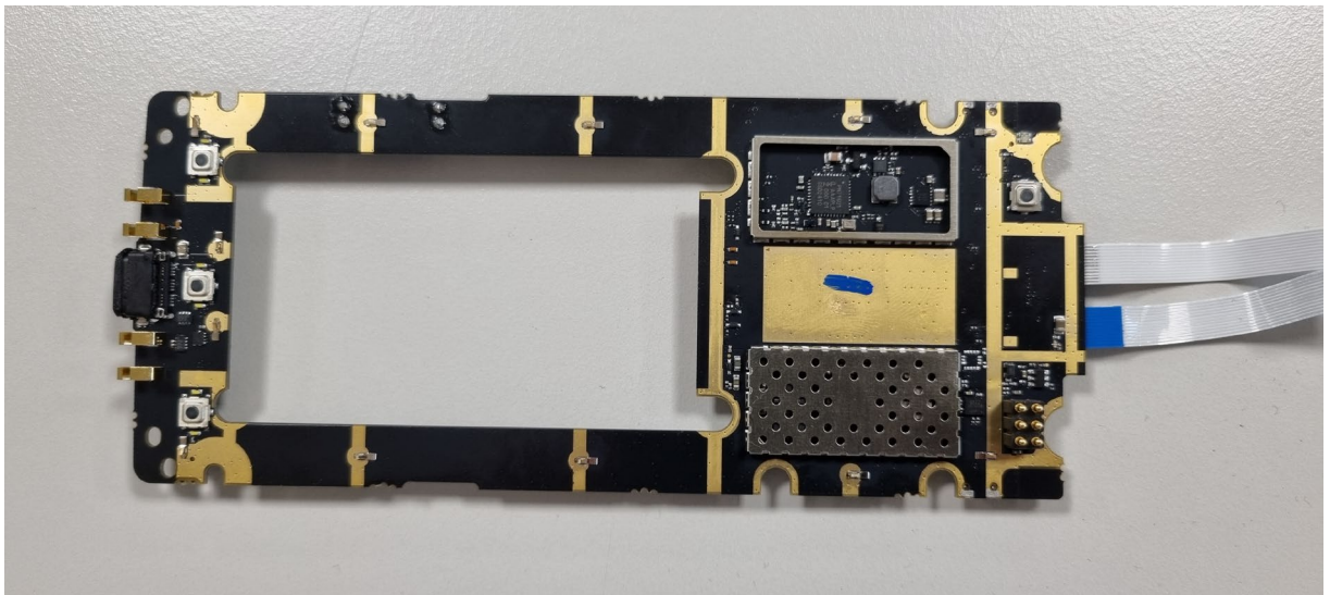
Picture 5. HH86 main unit PWB NFC solution without shield.
