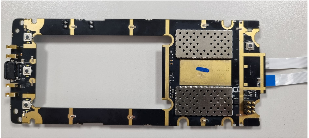
Picture 5. HH86 main unit PWB bottom.
