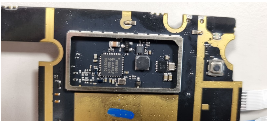
Picture 6. HH86 main unit PWB NFC radio IC close look.
