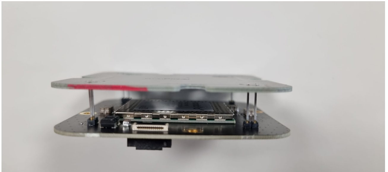
Picture 8. HH86 RFID module + antenna mounted at the top of the module.
