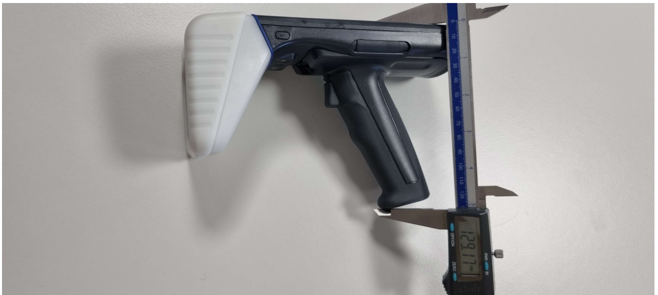
Picture 3 & 4. Right & left side view and size (L) 195.7mm and (H) 129mm
