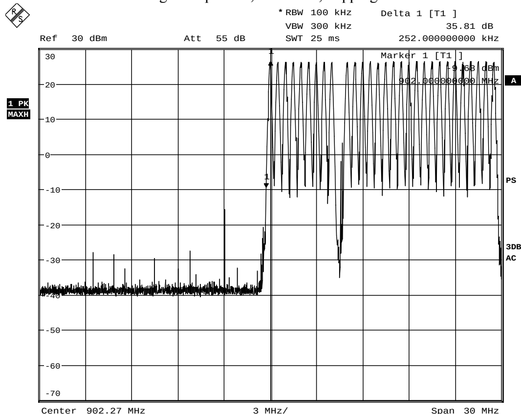
Picture 20: Band edge compliance, channel 1, hopping enabled
