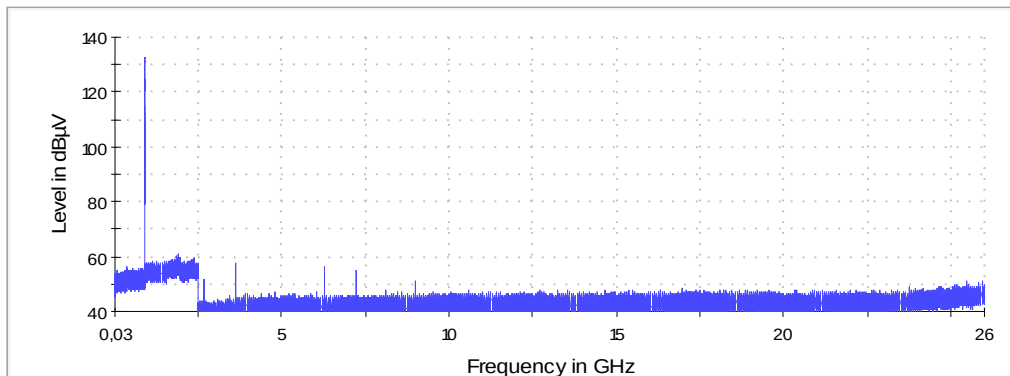
Picture 32: Conducted spurious emissions on antenna port, Channel 1,
