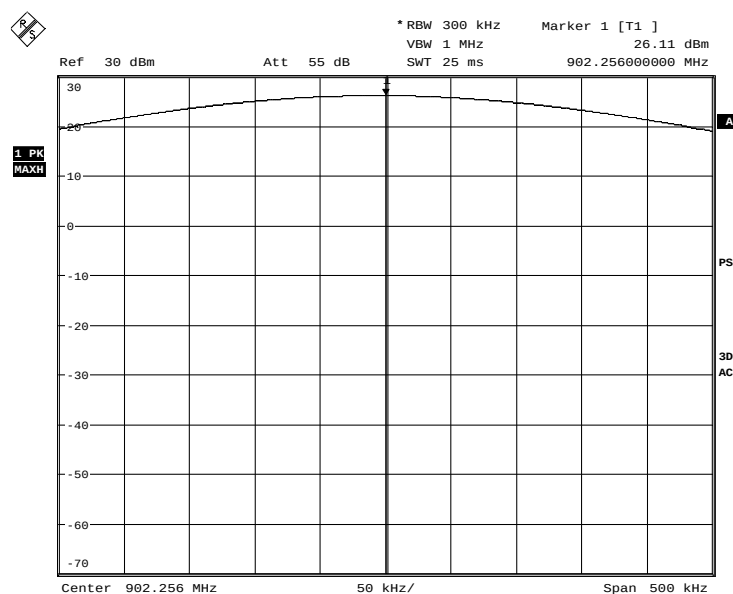
Picture 16: Peak output power, channel 1
