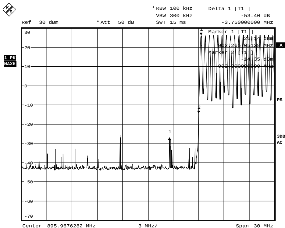
Picture 22: Band edge compliance, channel 1, hopping enabled
