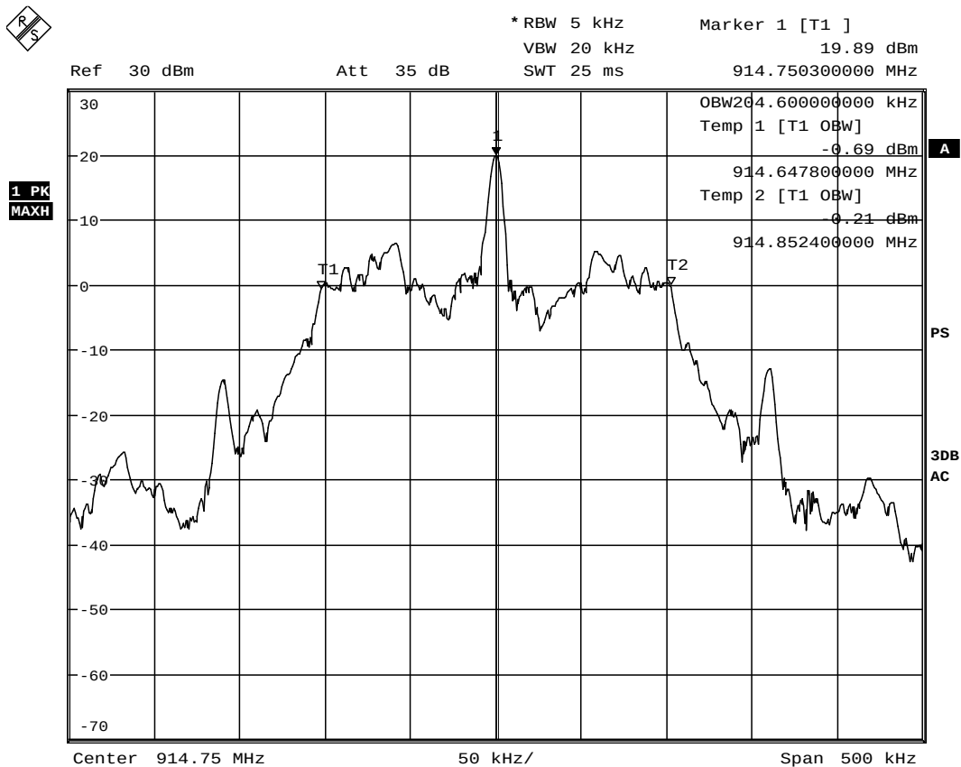
Picture 29: 99% Bandwidth measurement result, ch 26
