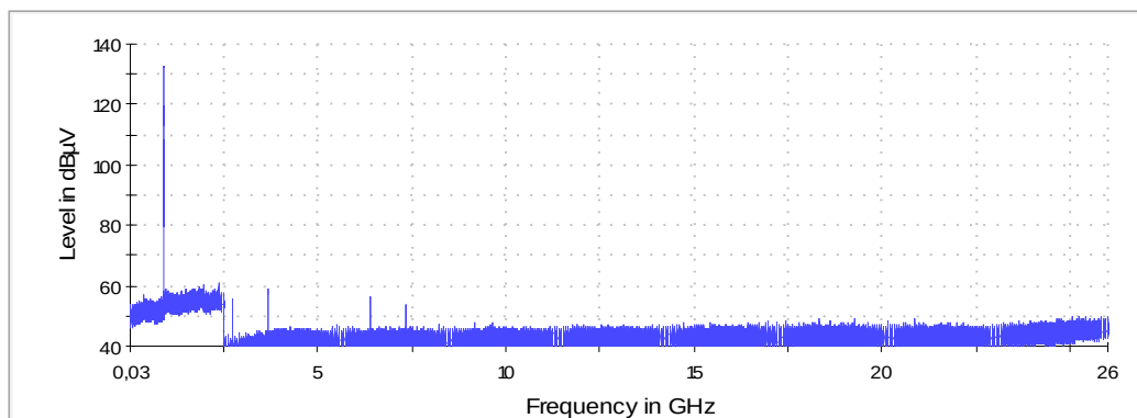
Picture 34: Conducted spurious emissions on antenna port, Channel 52,
