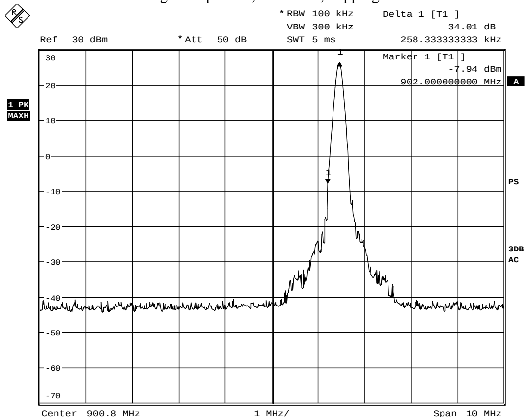
Picture 26: Band edge compliance, channel 0, hopping disabled
