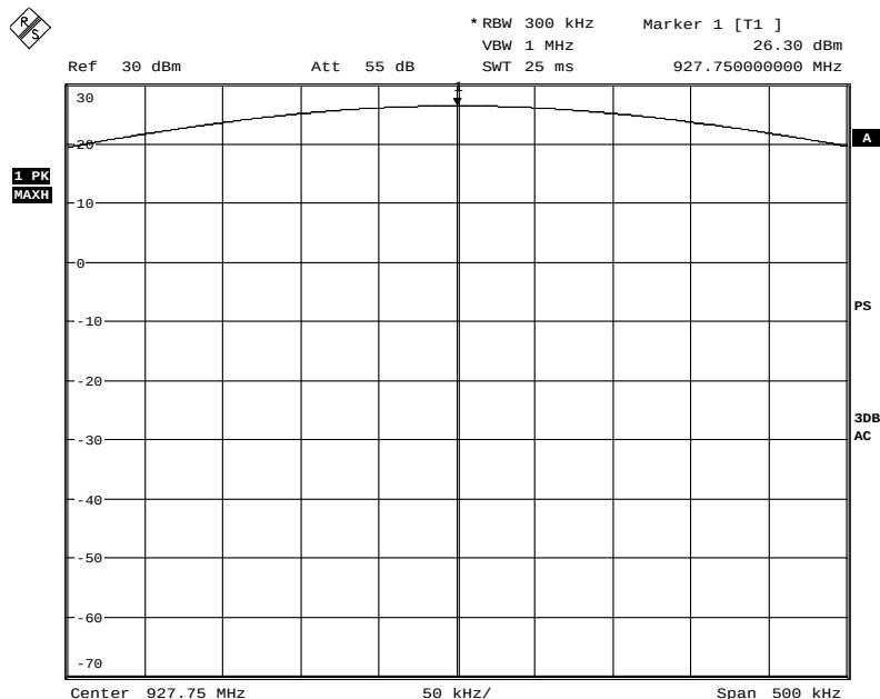
Picture 15: Peak output power, channel 52
