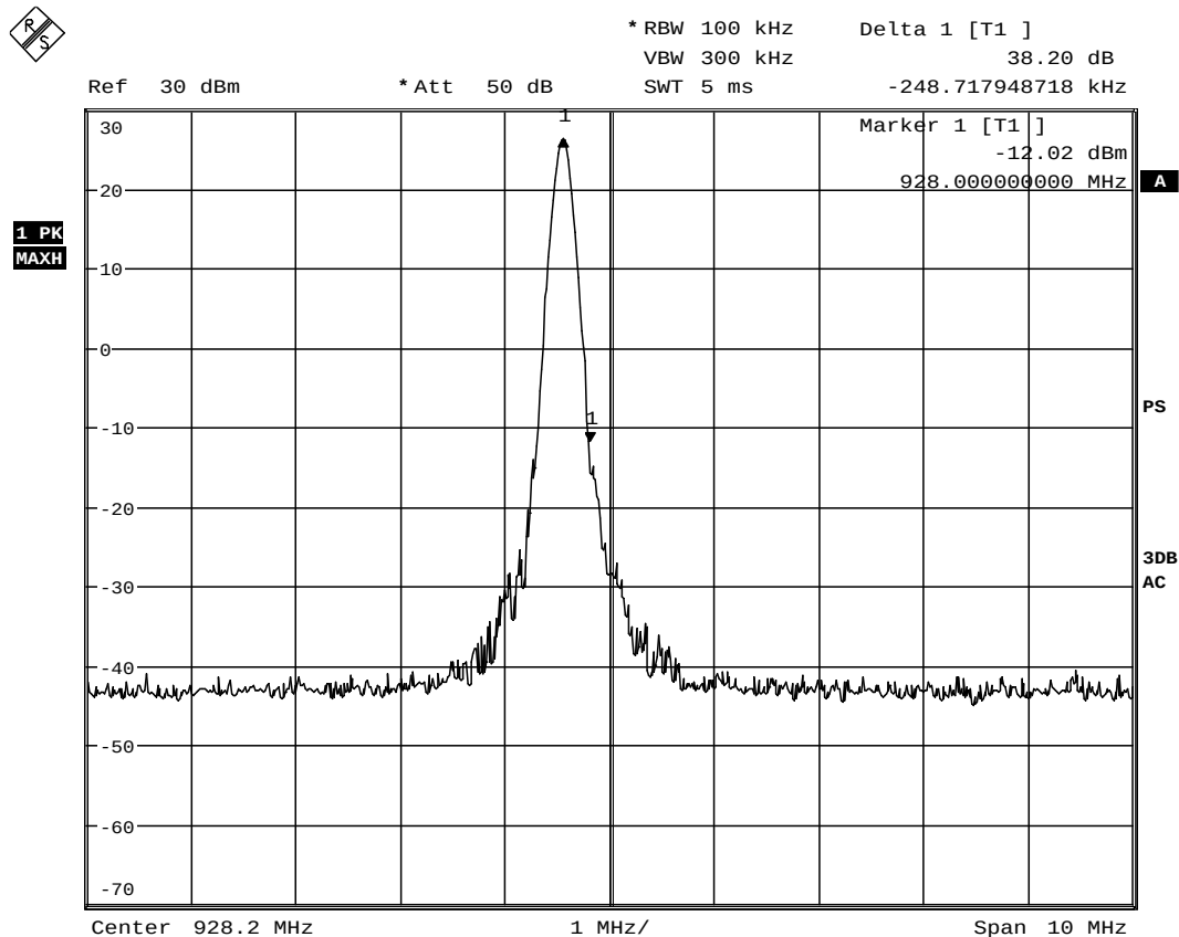
Picture 27: Band edge compliance, channel 52, hopping disabled
