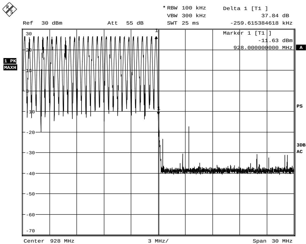
Picture 21: Band edge compliance, channel 52, hopping enabled
