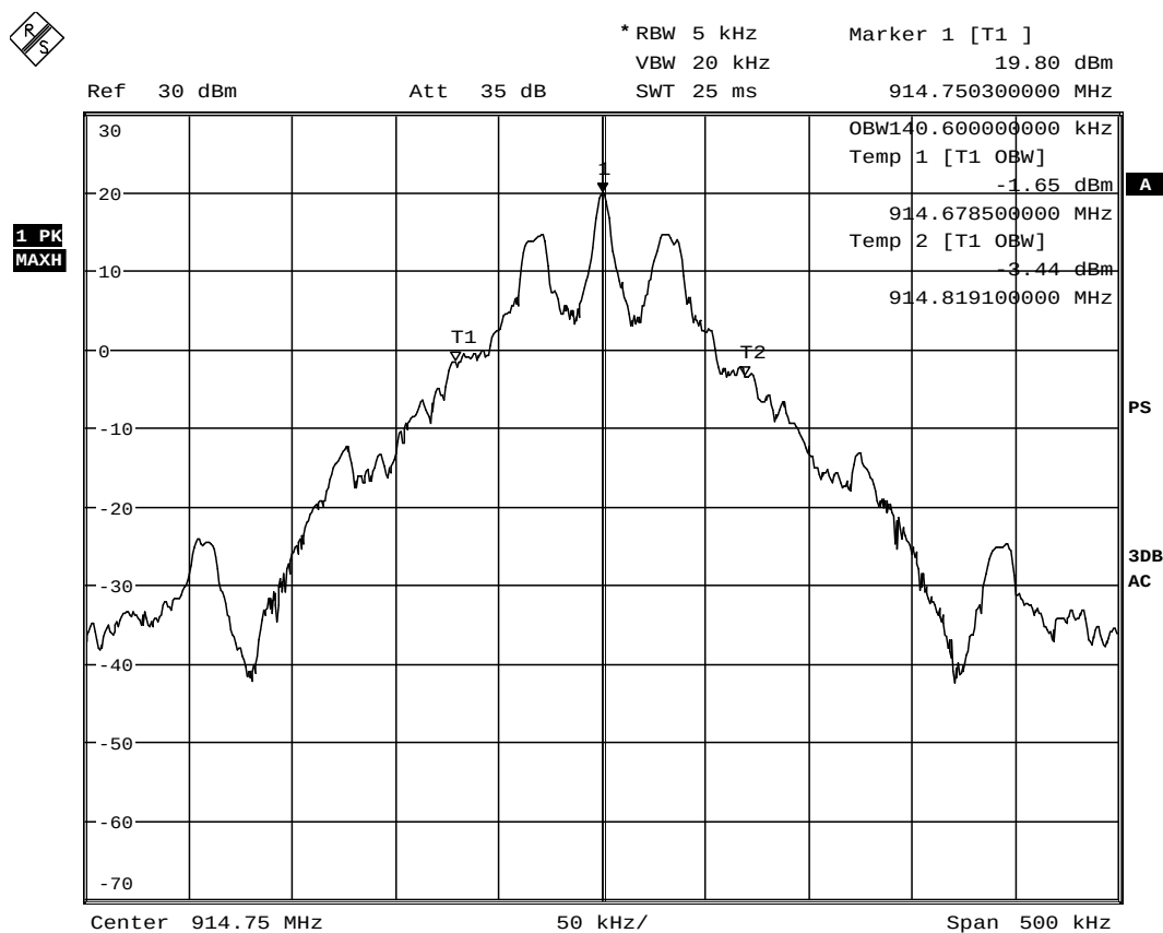
Picture 30: 99% Bandwidth measurement result, ch 26
