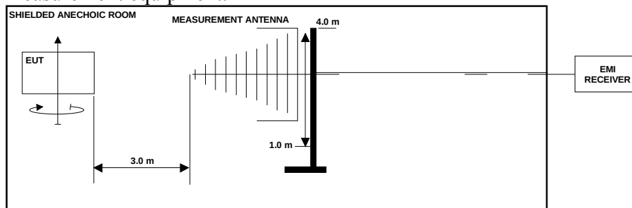
Picture 35: Test setup for radiated spurious emissions measurement 30 MHz - 1 GHz frequencies
