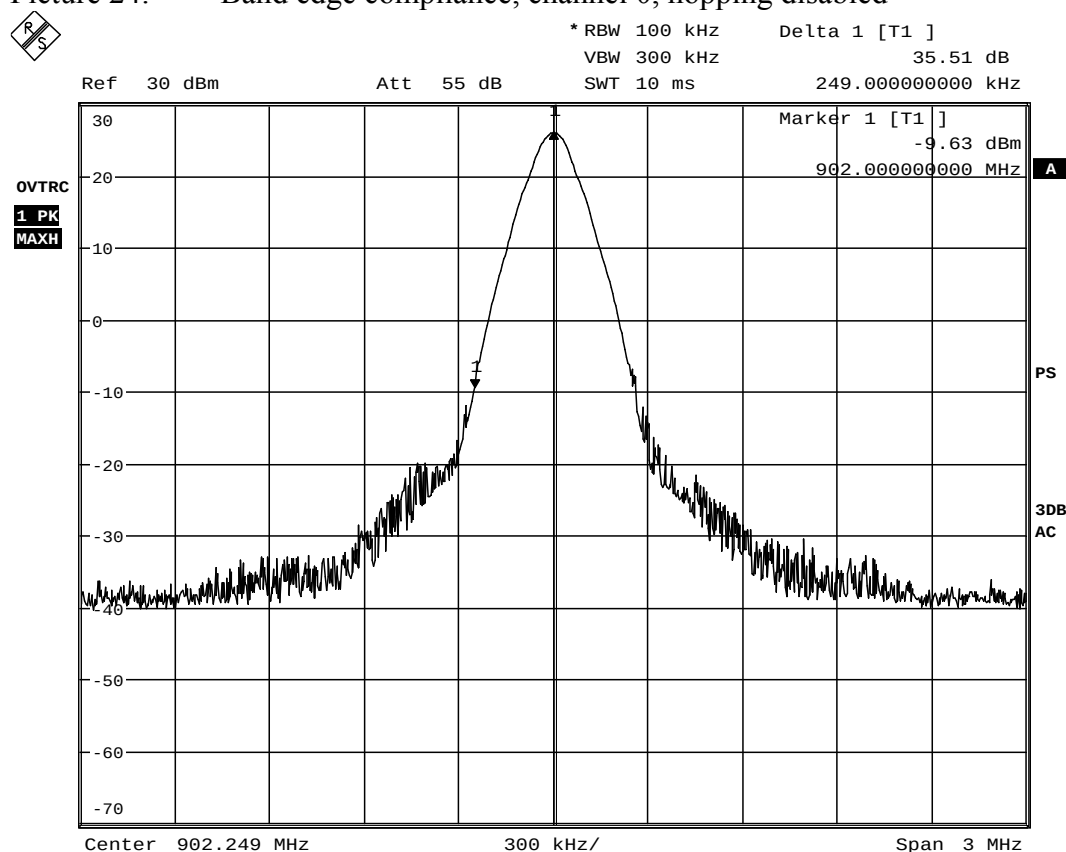
Picture 24: Band edge compliance, channel 0, hopping disabled
