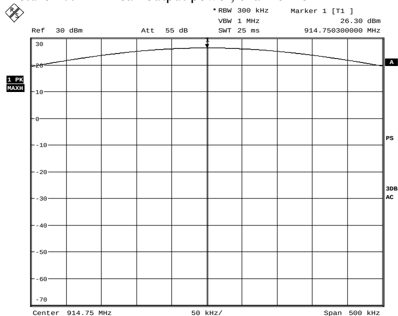
Picture 17: Peak output power, channel 26
