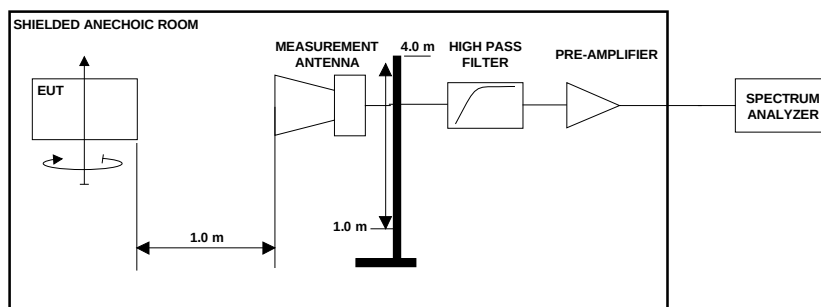
Picture 36: Test setup for radiated spurious emissions measurement 1 GHz – 10 GHz frequencies
