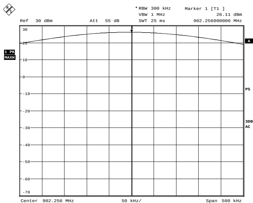
Picture 13: Peak output power, channel 1
