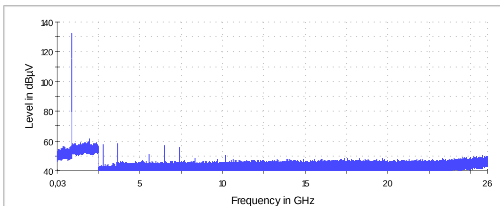
Picture 34: Conducted spurious emissions on antenna port, Channel 52,
