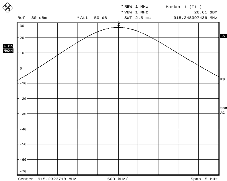
Picture 14: Peak output power, channel 26
