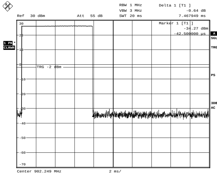
Picture 8: Duration of one transmission on connection state, channel 1
