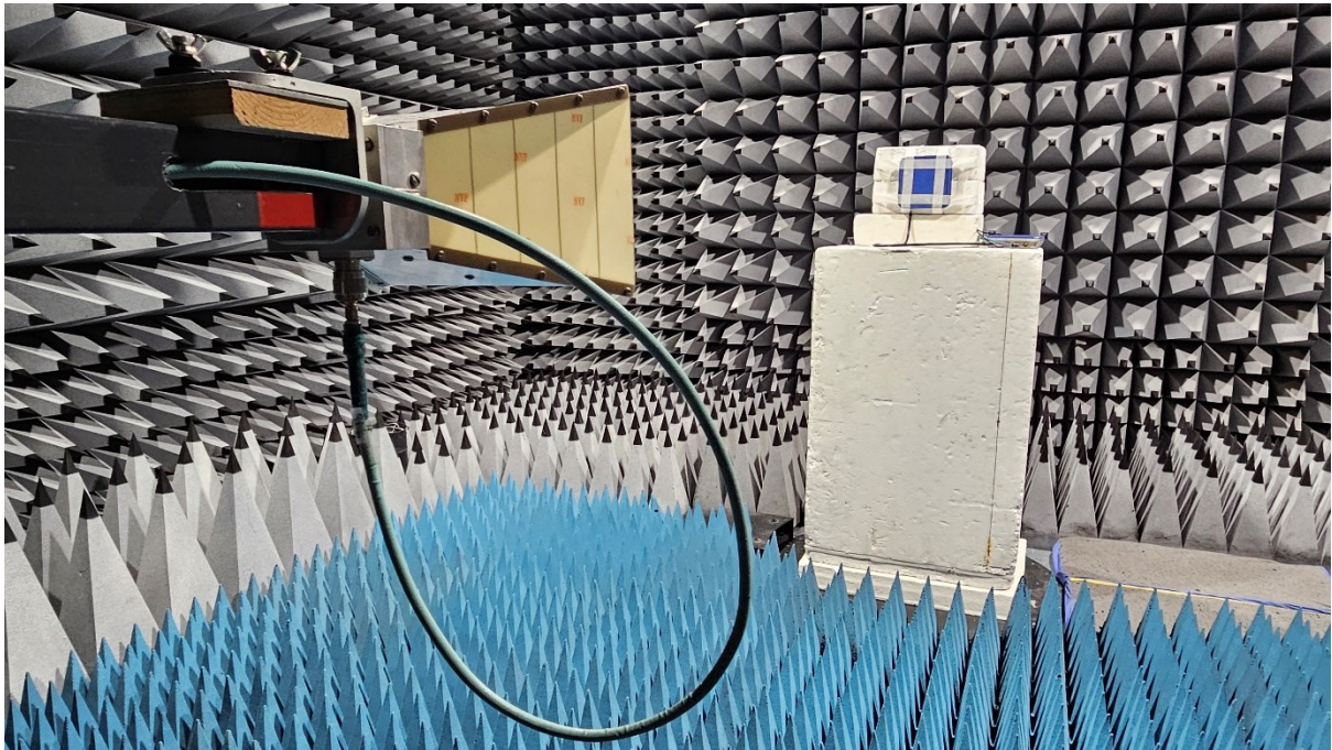
Radiated Emissions 1GHz to 10GHz test with external antenna
