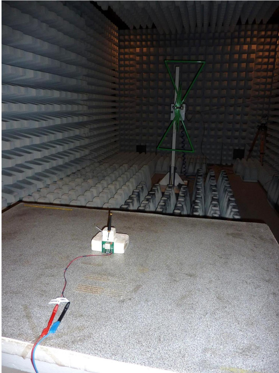
130412_2.JPG: Test setup fully anechoic chamber
