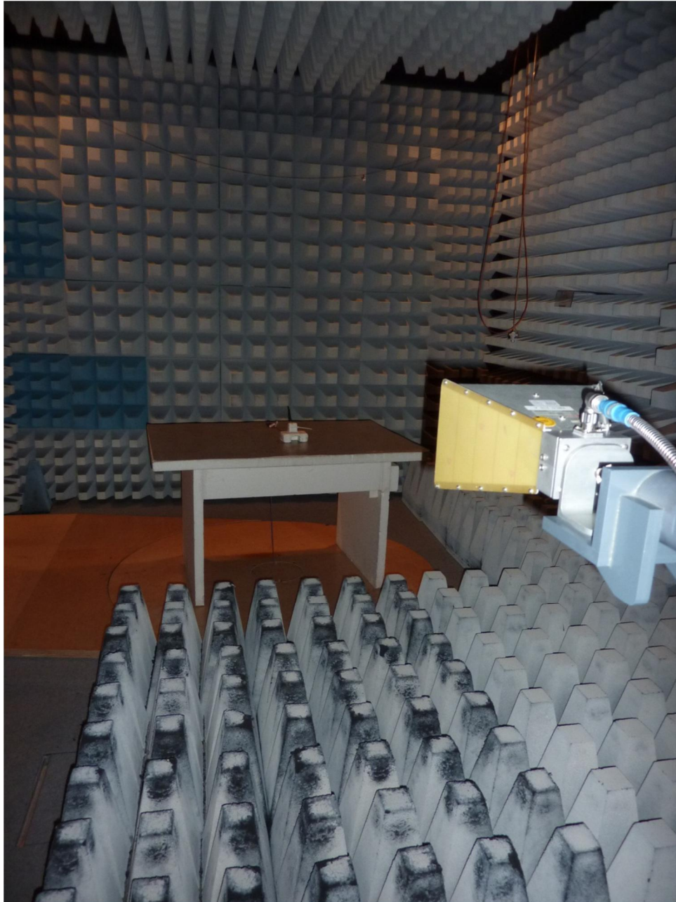
130412_3.JPG: Test setup fully anechoic chamber
