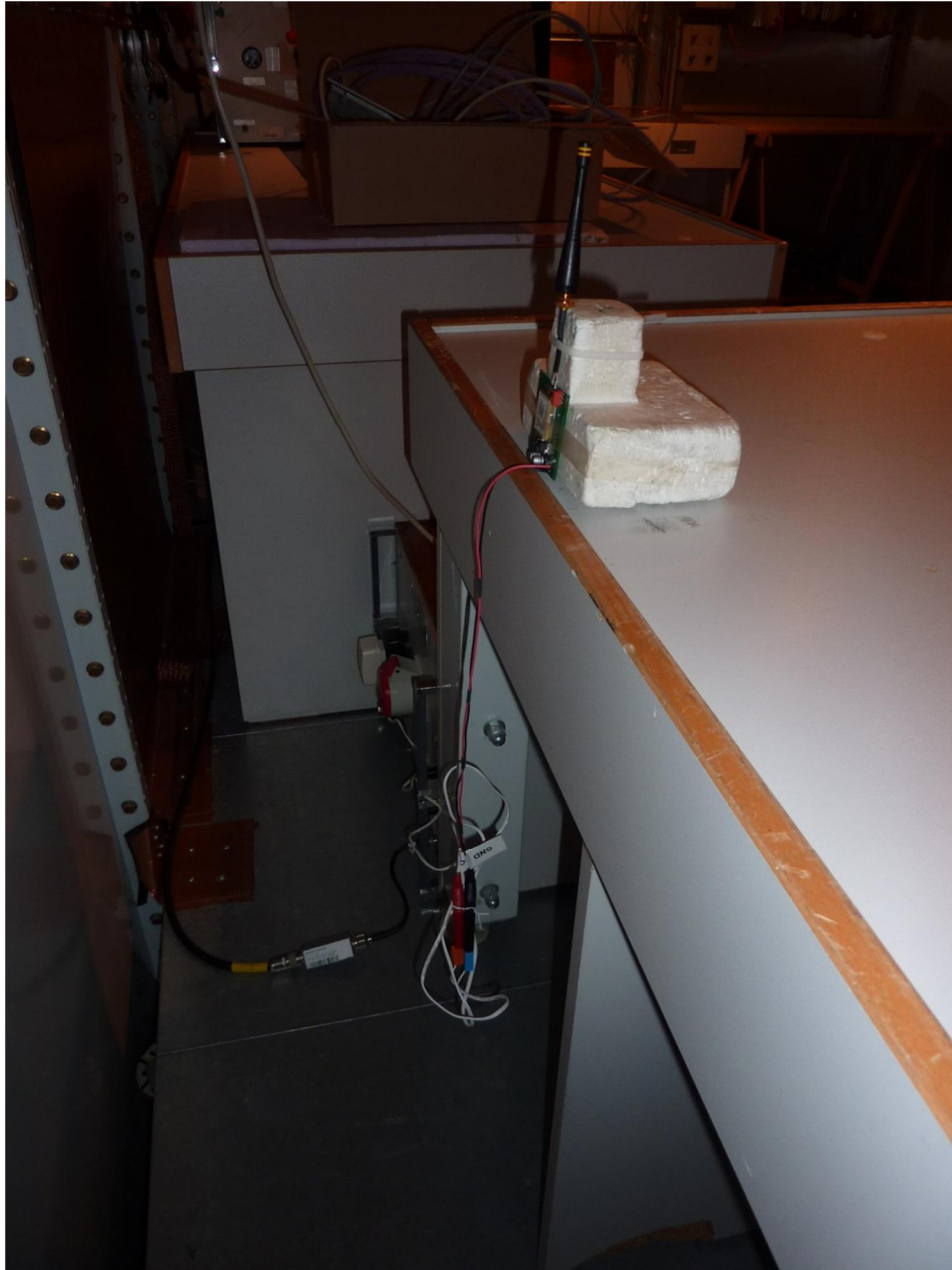
130412_4.JPG: Test setup shielded chamber
