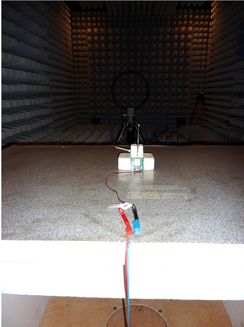
130412_1.JPG: Test setup fully anechoic chamber
