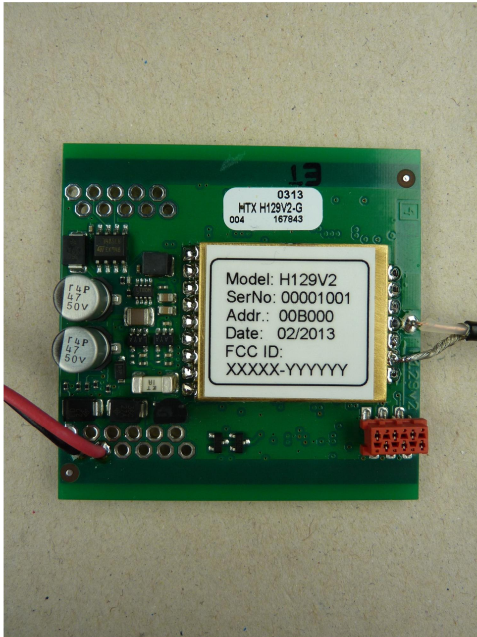
130412_8.JPG: H129V2, bottom and type plate view
