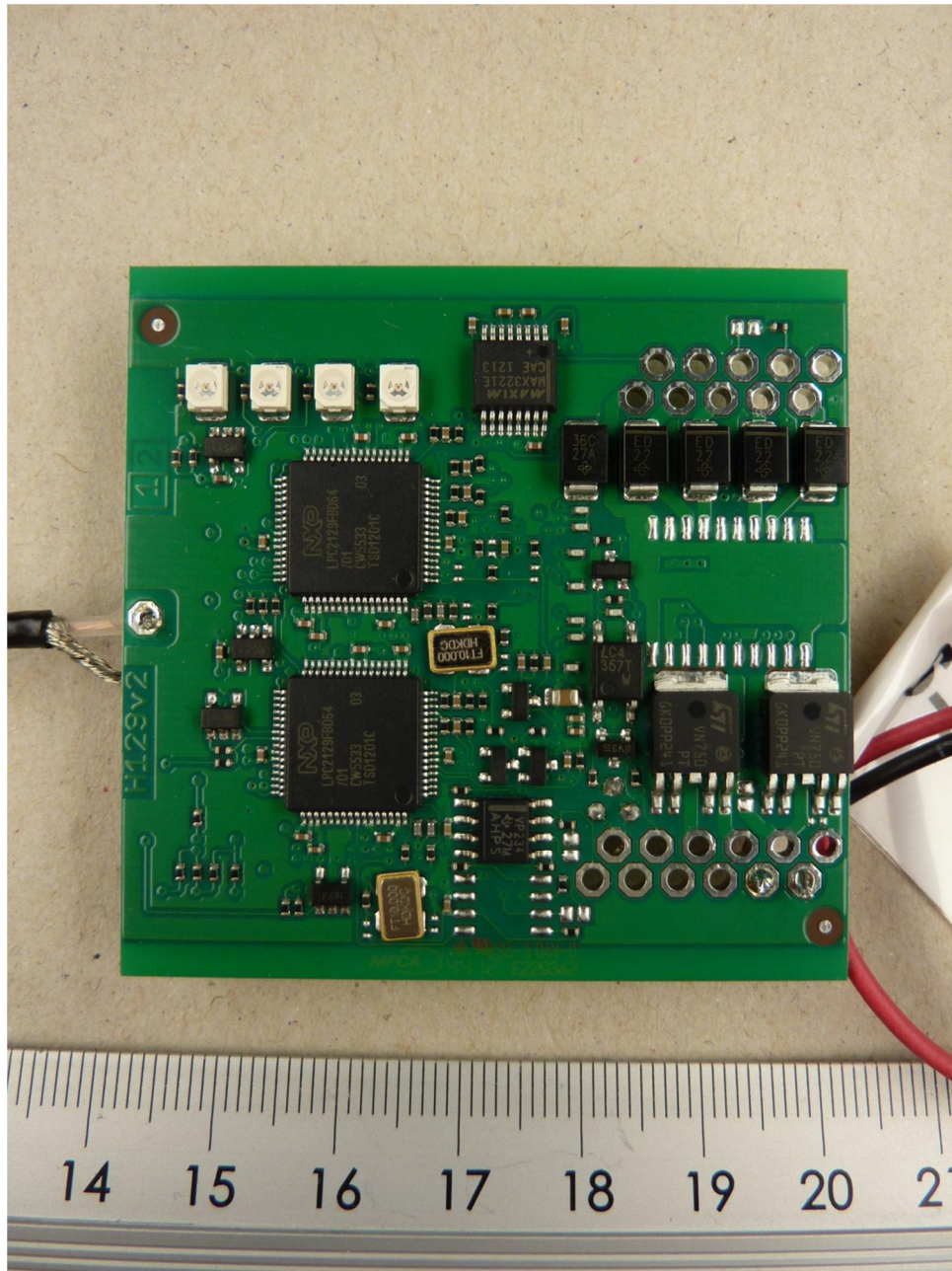
130412_7.JPG: H129V2, top view
