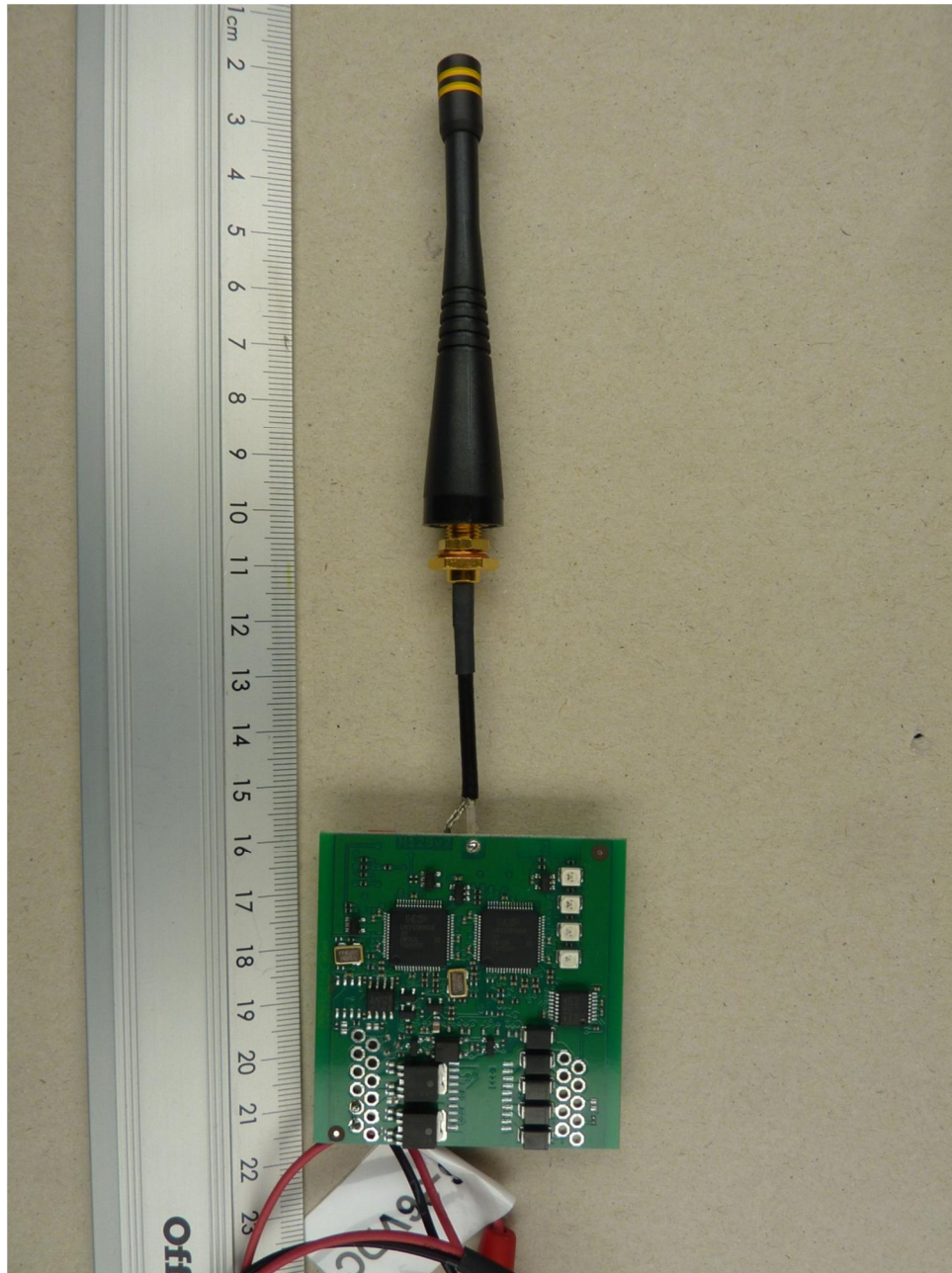
130412_6.JPG: H129V2, top view with mounted antenna
