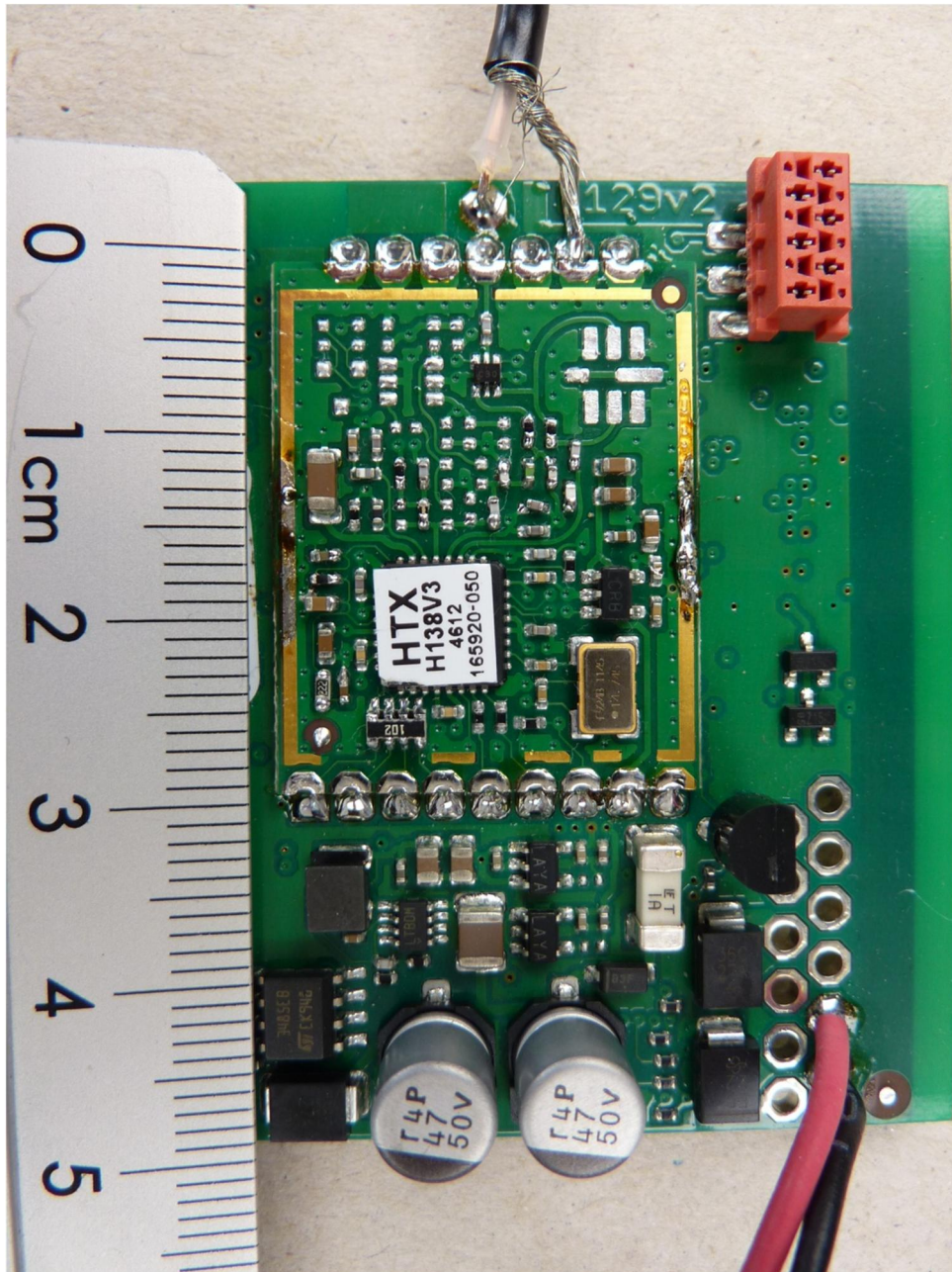
130412_10JPG: H129V2, shielding removed
