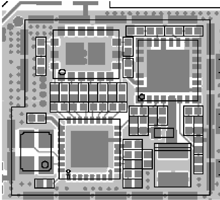
<Figure 5.3> RF Area
