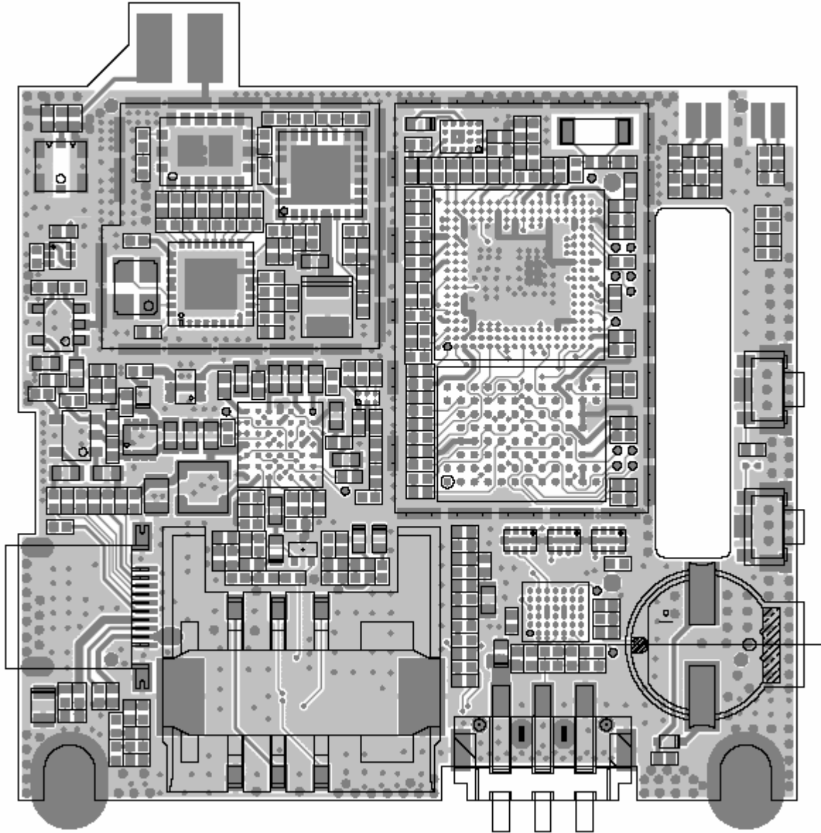
<Figure 5.2> Bottom View
