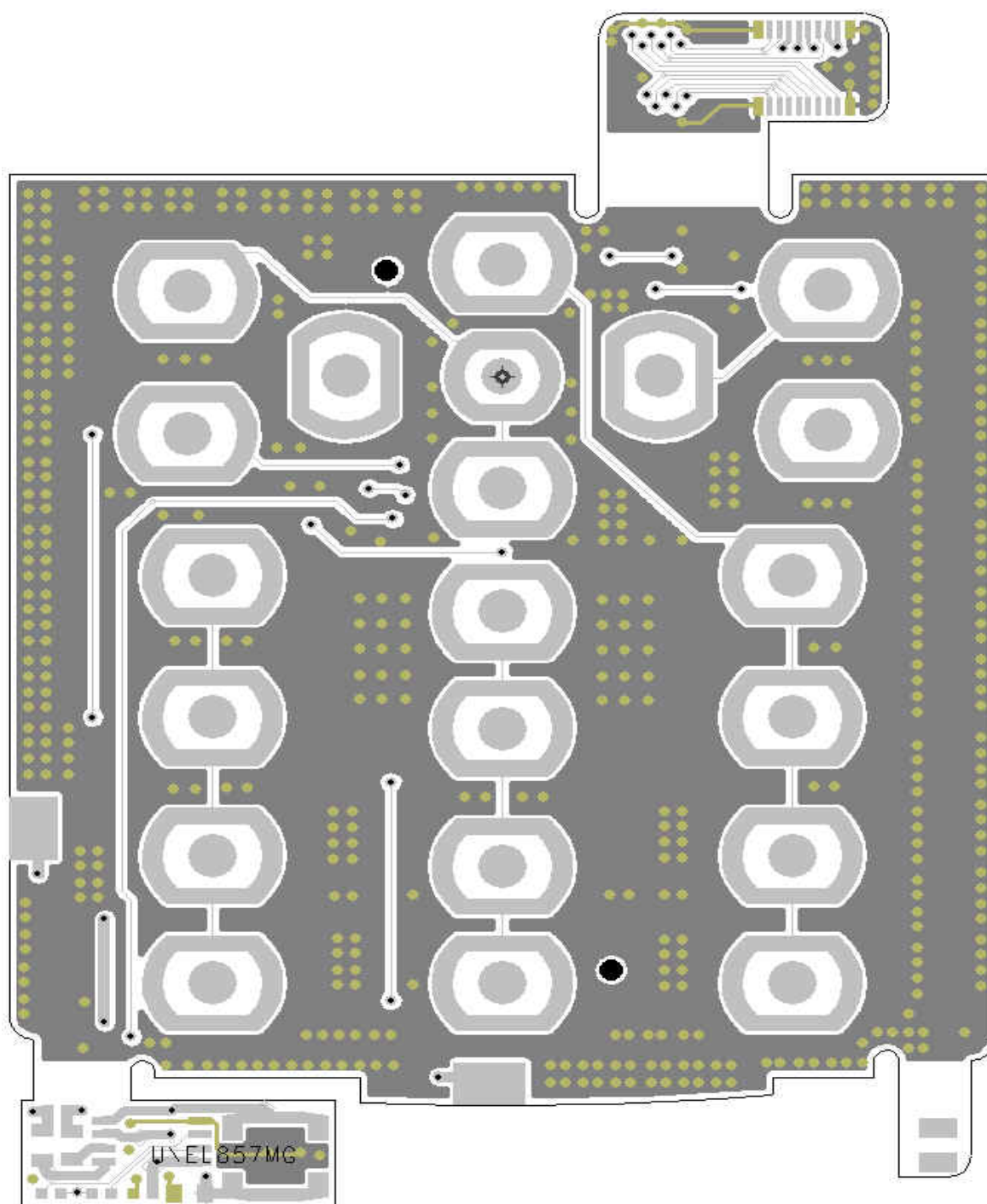
<Figure 5.6> Key Top Area
