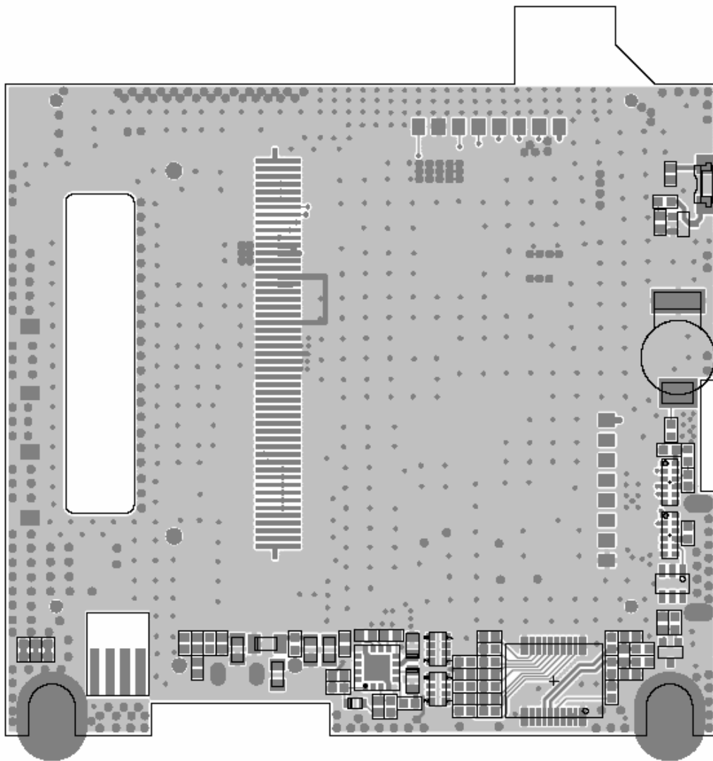
<Figure 5.1> Top View
